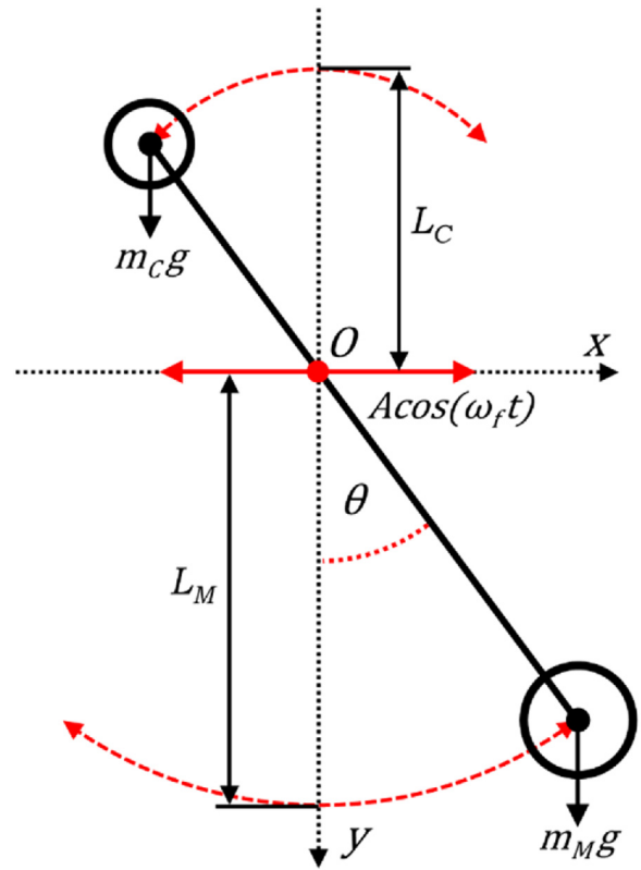
Fig. 1. Schematic of the counterweight pendulum.
