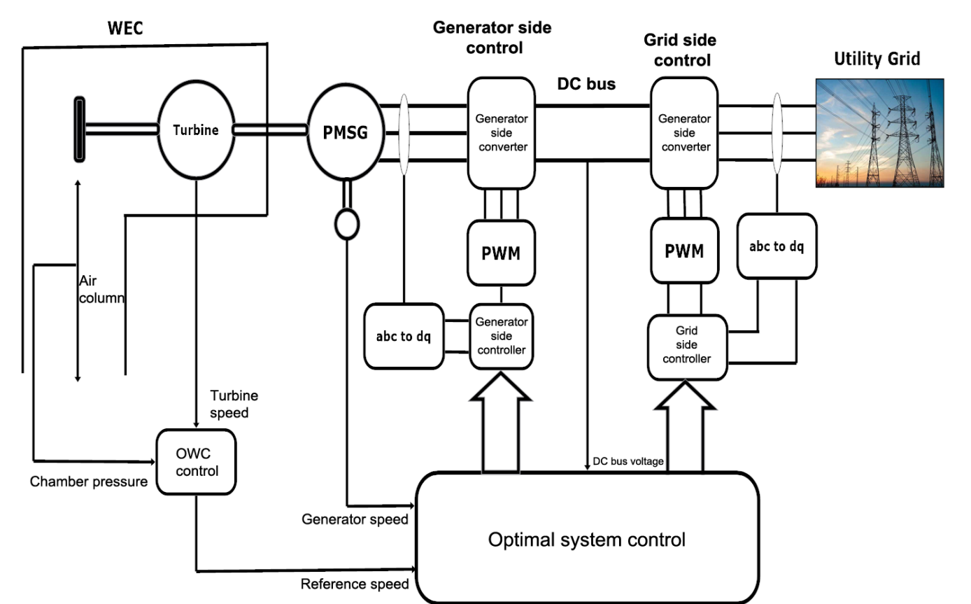
Figure 1. The schematic of the proposed MPPT control system for oscillating water column OWECs.
