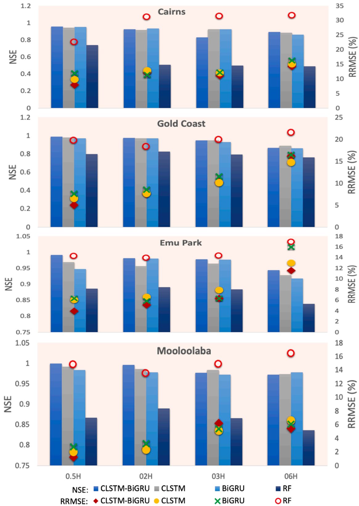
Fig. 7. Comparison of the predictive skill for proposed CLSTM-BiGRU vs. CLSTM, BiGRU and RF models in terms of the relative error: RRMSE (%) and the NSE value within the testing period computed for the multi-step horizons.
