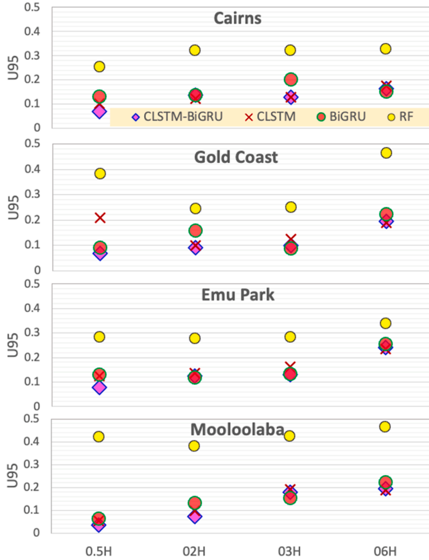
Fig. 9. Comparison of the predictive skill of the proposed CLSTM-BiGRU model using the Expanded Uncertainty (U95) metric against the benchmark CLSTM, BiGRU and RF models for the multi-step forecast horizons.
