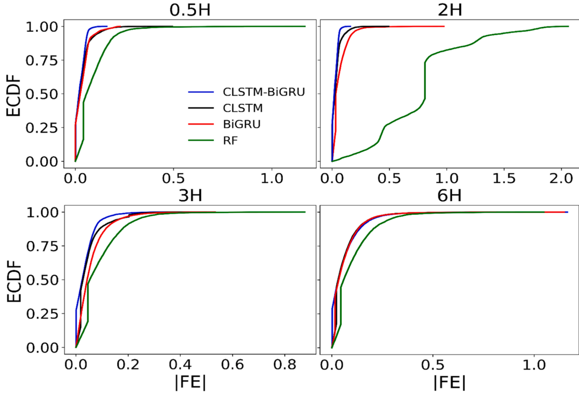
Fig. 8. Empirical cumulative distribution function (ECDF) in absolute forecast error |FE| for the proposed CLSTM-BiGRU vs. CLSTM, BiGRU and RF models for Mooloolaba station presented for multi-step forecast horizons.
