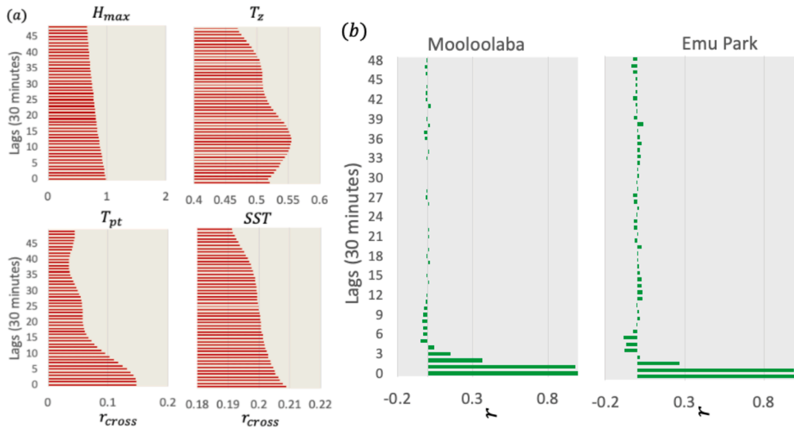
Fig. 3. (a) The correlogram shows the covariance between the objective target ( H_{sig} ) and the predictor ( H_{max} , T_z , T_{pt} , SST ) variables in terms of cross-correlation coefficients ( r_{cross} ), and (b) a partial autocorrelation function (PACF) plot of the H_{sig} time series exploring the antecedent behaviour for Mooloolaba and Emu Park study sites.
