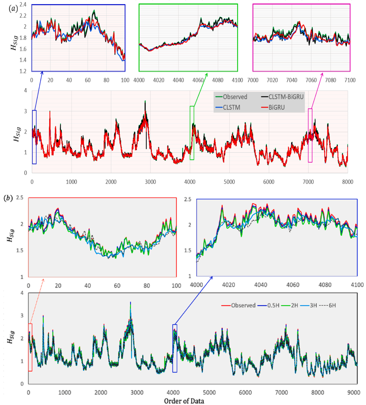
Fig. 11. The time series plot at Mooloolaba study site of: (a) forecasted and observed H_{sig} for the proposed CLSTM-BiGRU model compared with the CLSTM and BiGRU models at 0.5 h forecast horizons, (b) the forecasted and observed H_{sig} generated by the proposed CLSTM-BiGRU model at multi-step forecasting horizons.
