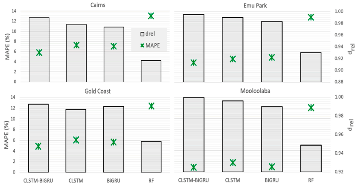
Fig. 4. Comparison of the predictive skill of the proposed CLSTM-BiGRU model vs. CLSTM, BiGRU and RF (benchmark) models in terms of the Mean Absolute Percentage Error (MAPE %) and Relative Index of Agreement ( d_{rel} ) computed in the testing period for 0.5 H forecasting horizon.
