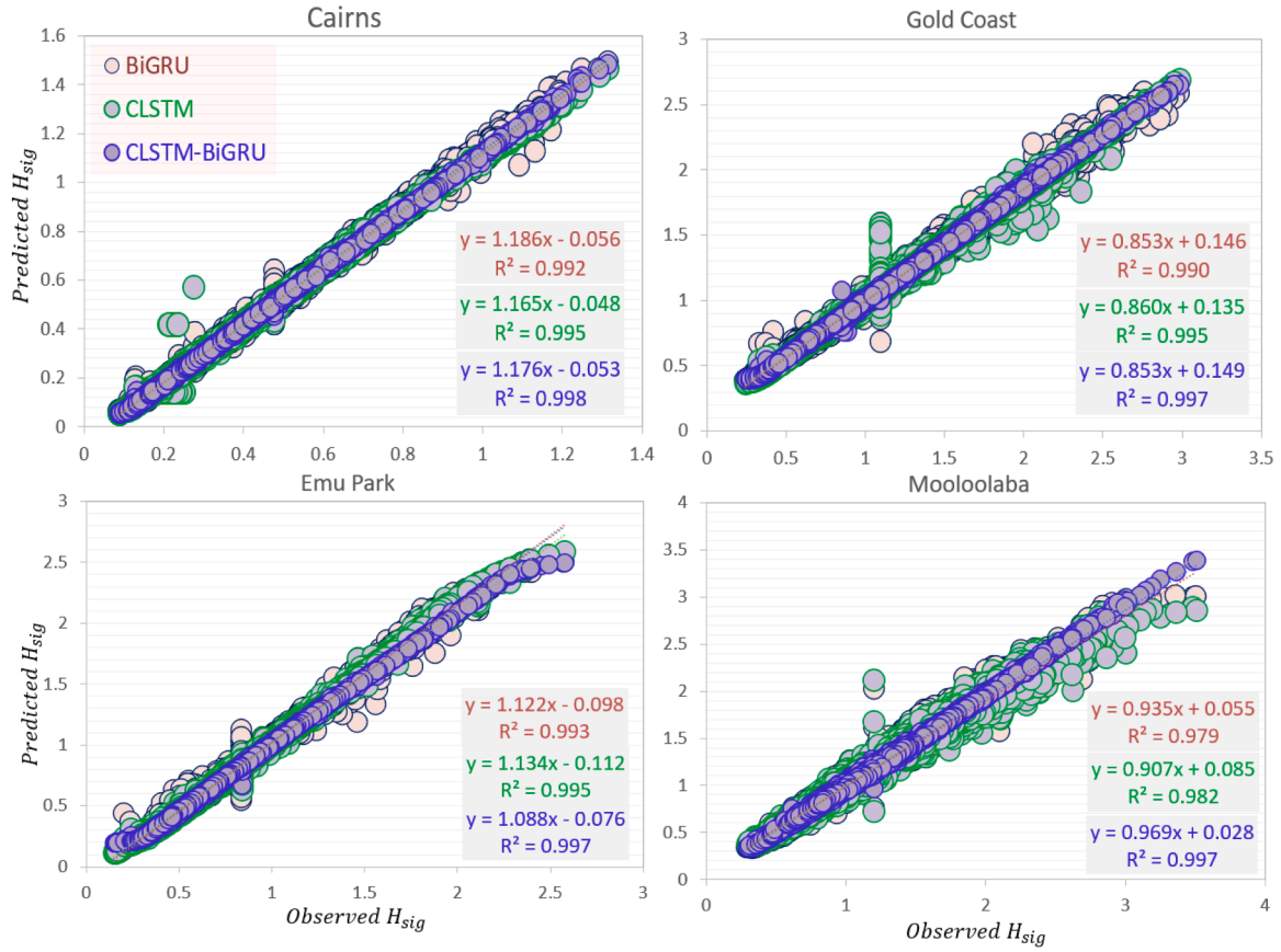
Fig. 6. Scatter plot of forecasted and observed H_{sig} in testing phase at the four stations using the proposed CLSTM-BiGRU vs. CLSTM and BiGRU models for 0.5 H horizon. Least square regression line and coefficient of determination ( R^2 ) with a linear fit is shown in each sub-panel.
