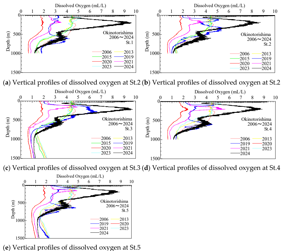
Figure 7. Vertical profiles of dissolved oxygen obtained in our observations of each year are summarized in each observation point.
