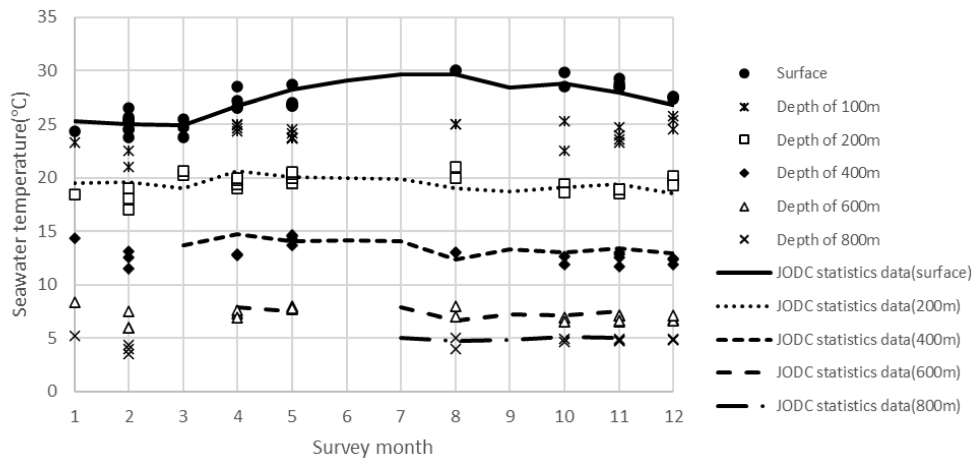
Figure 5. Change in seawater temperature by month including the data from JAMSTEC, CMO, Yeneyama, Tokyo Metropolitan Government, IDEA Consultants, Inc. and JODC.
