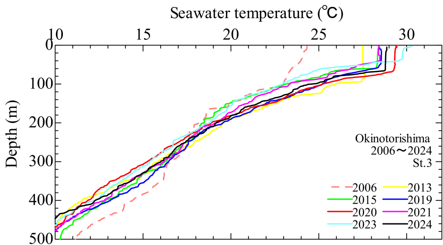
Figure 4. Vertical profiles of seawater temperature zoomed up to surface.
