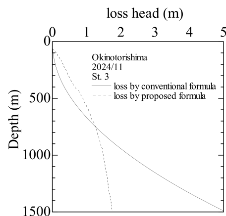
Figure 10. Vertical profiles of density different loss. St.3 in 2024 is used as the representative point for calculation. The solid lines mean result of simple calculation. The dashed lines mean precise calculation.
