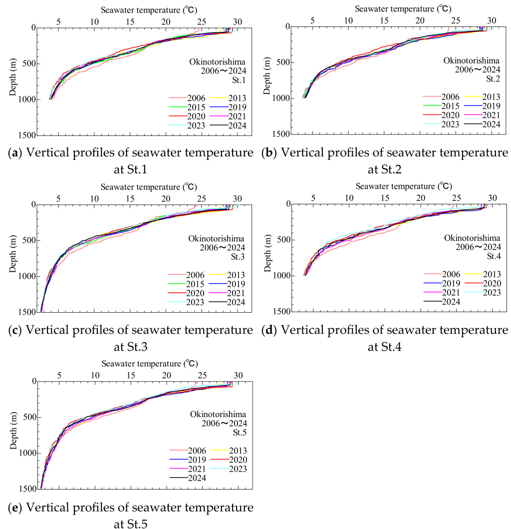
Figure 3. Vertical profiles of seawater temperature obtained in our observations of each year are summarized in each observation point.
