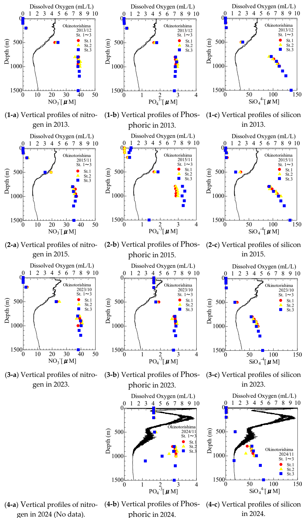
Figure 8. Vertical profiles of inorganic nutrients. Survey of nutrients had been implemented in st.1 to st.3, and limited survey years. Branch numbers are assigned by survey year—type of nutrients. It
