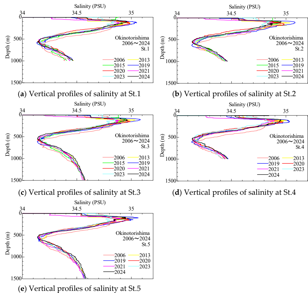
Figure 6. Vertical profiles of salinity obtained in our observations of each year are summarized in each observation point.
