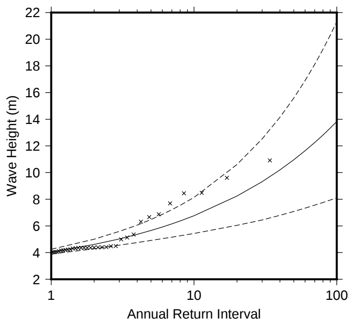
Figure 9 Extreme wave distribution for Tau Island. The crosses represents the wave events that occurred since 1979. The plain line is the statistical distribution that best fit the past wave events. The dotted line show the upper and lower high confidence of the fit, there is a 95% chance that the fitted distribution lie between the two dashed lines.
