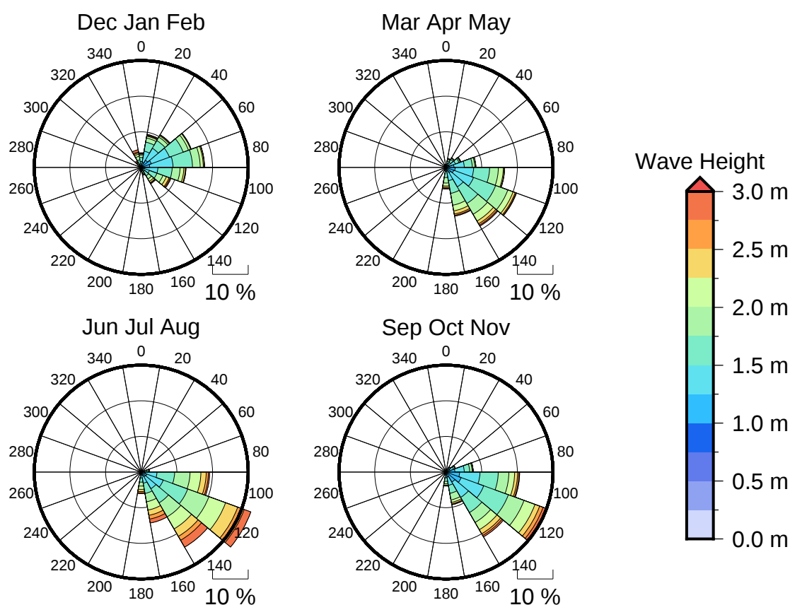
Figure 3 Seasonal wave roses for Tau Island
