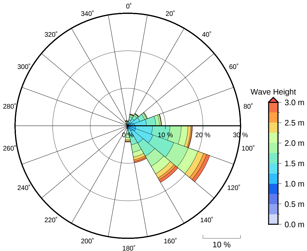
Figure 2 Annual wave rose for Tau Island. Note that direction are where the wave are coming from .
