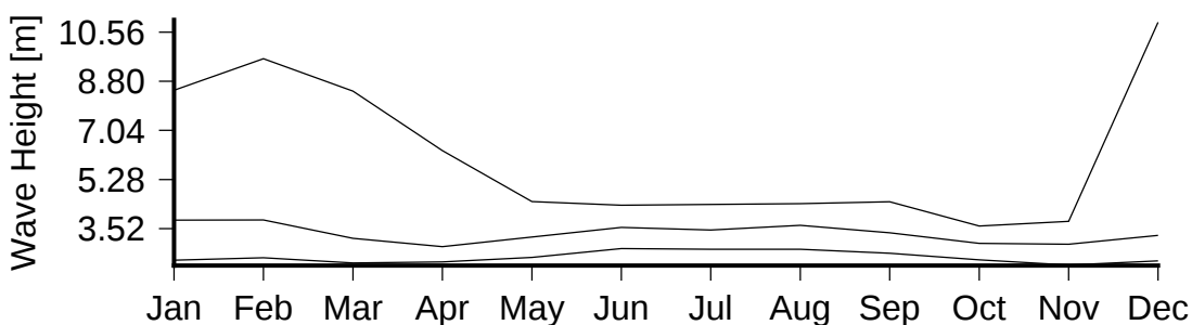
Figure 7 Monthly variation in large waves (90th percentile)(lower curve), severe waves (99th percentile) (middle curve) and the largest wave(upper curve) in Tau Island.
