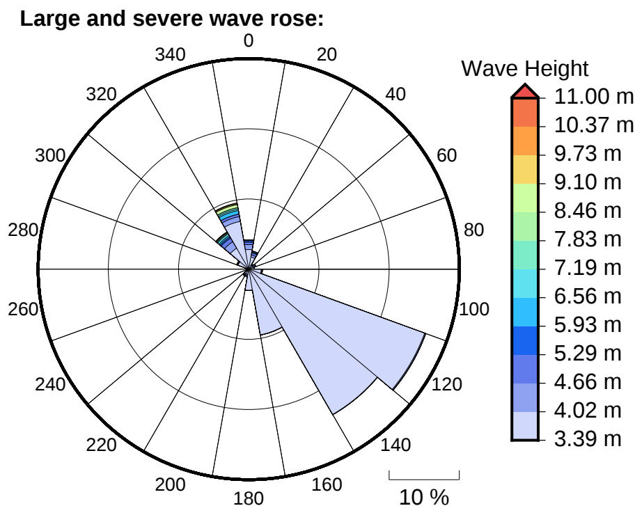
Figure 6 Large, severe and extreme wave roses for Tau Island
