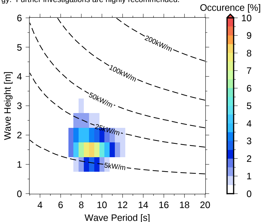
Figure 10 Occurences of sea states in Tau Island .
