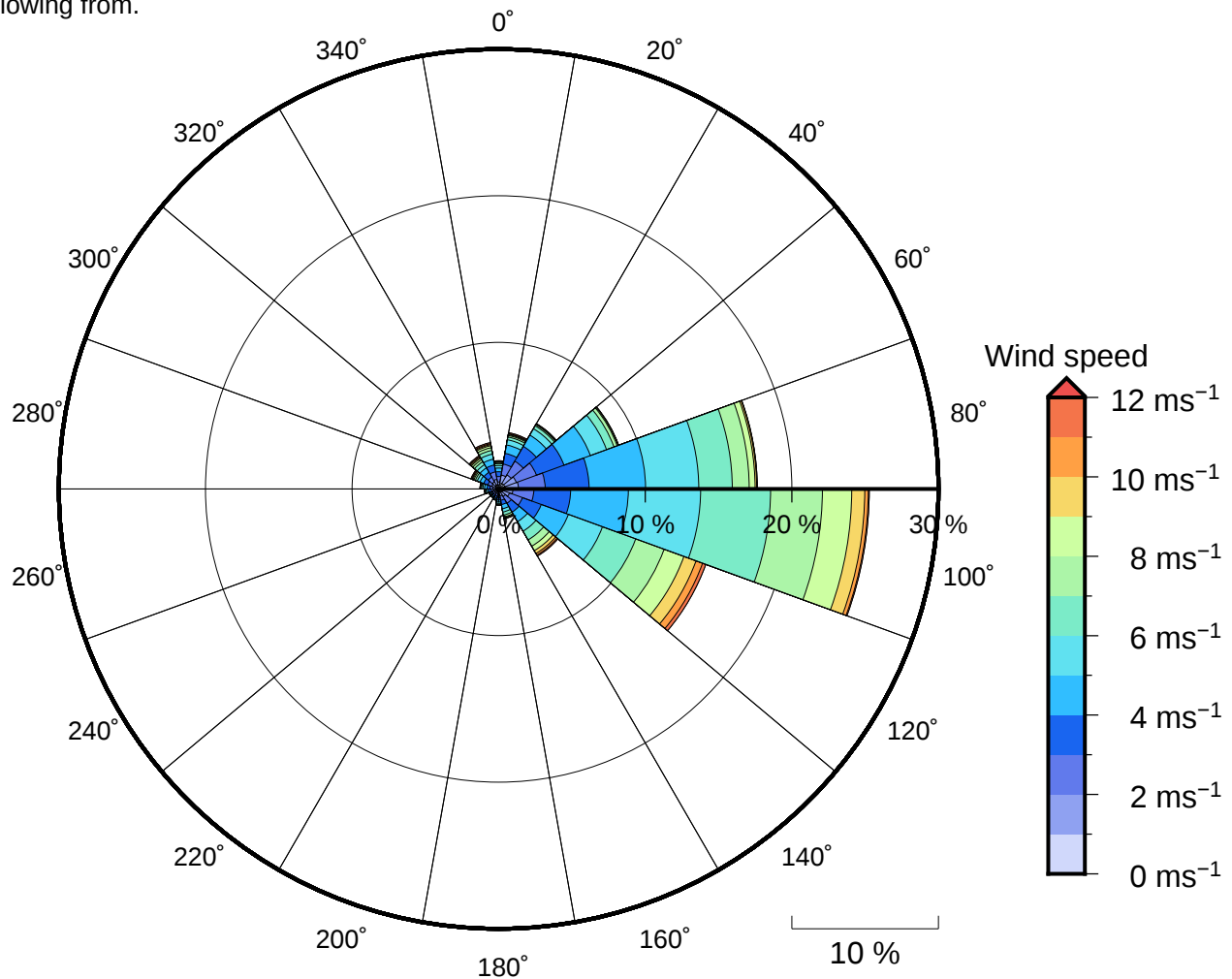
Figure 11 Annual wind rose for Tau Island. Note that directions are where the wind is coming from .
