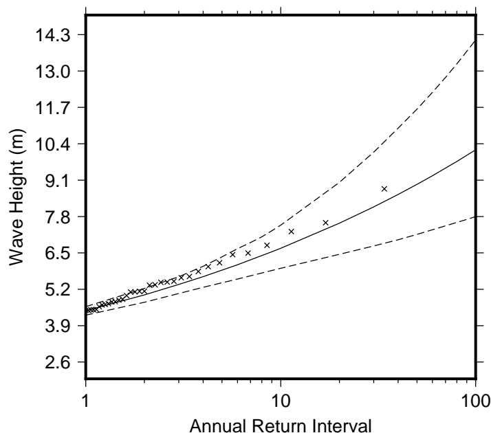
Figure 9 Extreme wave distribution for Avatiu. The crosses represents the wave events that occurred since 1979. The plain line is the statistical distribution that best fit the past wave events. The dotted line show the upper and lower high confidence of the fit, there is a 95% chance that the fitted distribution lie between the two dashed lines.
