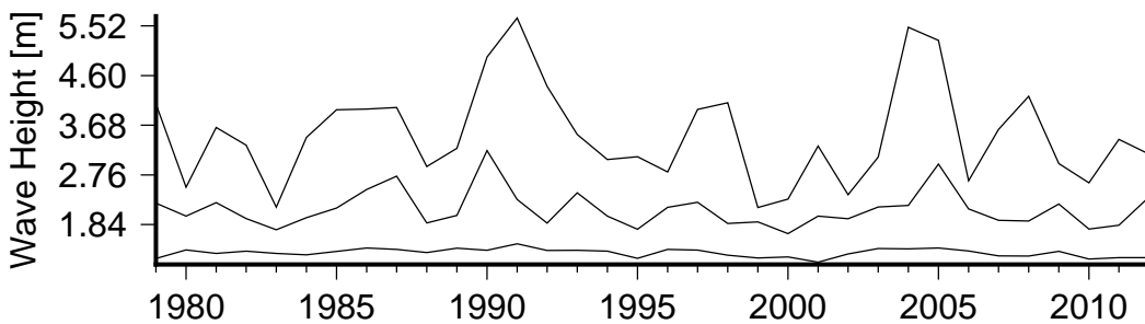
Figure 8 Annual variation in large waves (90th percentile)(lower curve), severe waves (99th percentile) (middle curve) and the largest wave(upper curve) in Black Rock.
