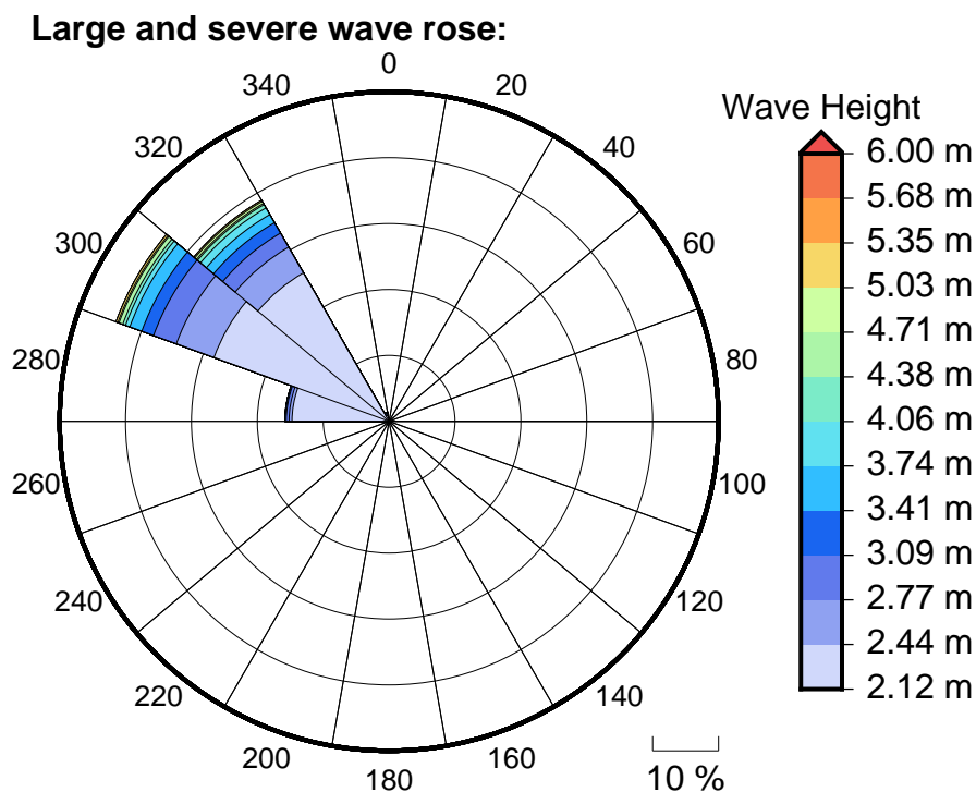
Figure 6 Large, severe and extreme wave roses for Black Rock
