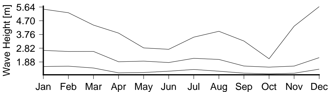
Figure 7 Monthly variation in large waves (90th percentile)(lower curve), severe waves (99th percentile) (middle curve) and the largest wave(upper curve) in Black Rock.
