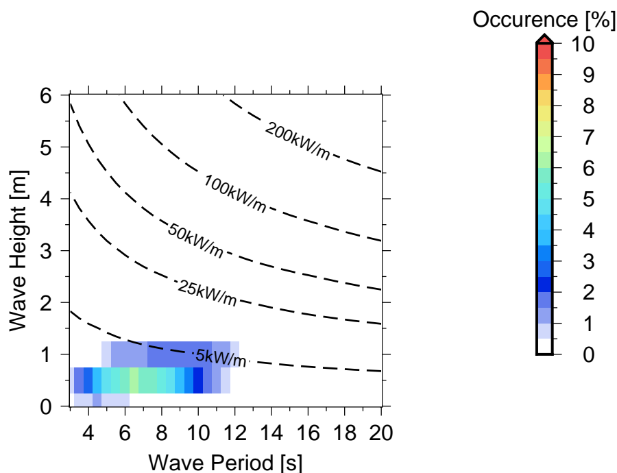
Figure 10 Occurrences of sea states in Black Rock .
