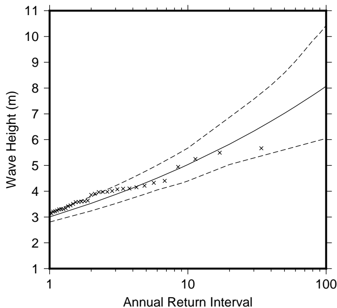
Figure 9 Extreme wave distribution for Black Rock. The crosses represents the wave events that occurred since 1979. The plain line is the statistical distribution that best fit the past wave events. The dotted line show the upper and lower high confidence of the fit, there is a 95% chance that the fitted distribution lie between the two dashed lines.
