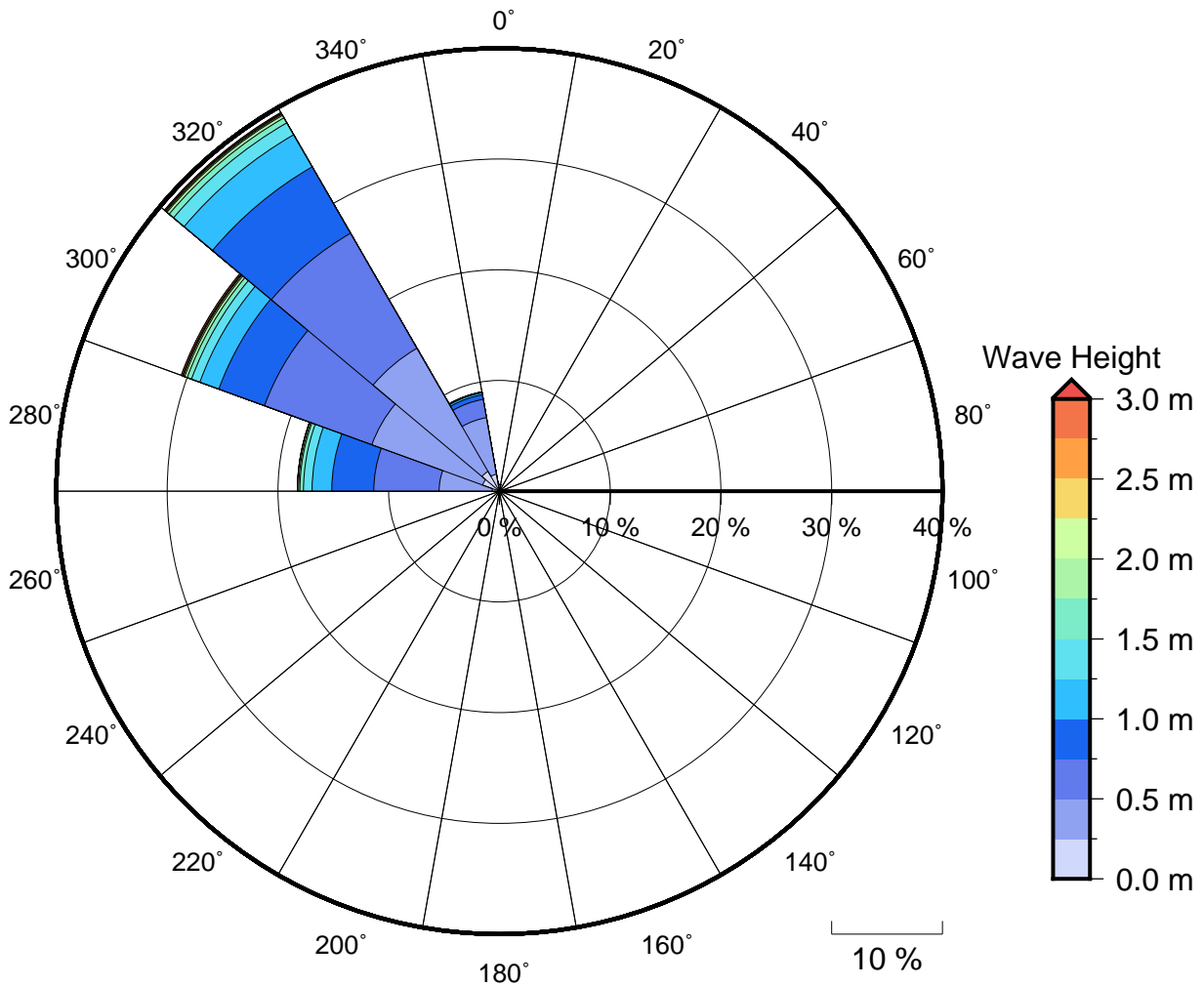
Figure 2 Annual wave rose for Black Rock. Note that direction are where the wave are coming from.
