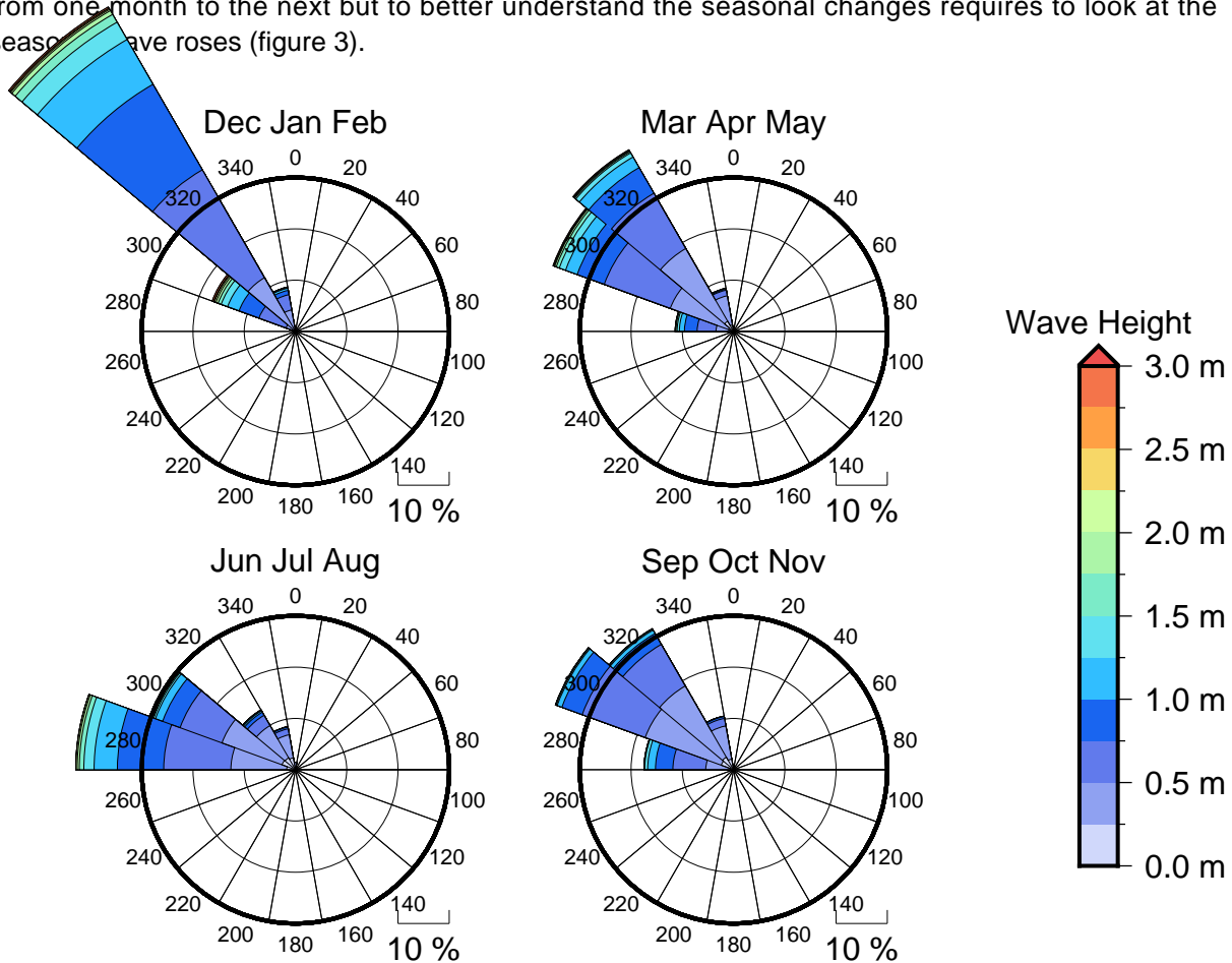
Figure 3 Seasonal wave roses for Black Rock
