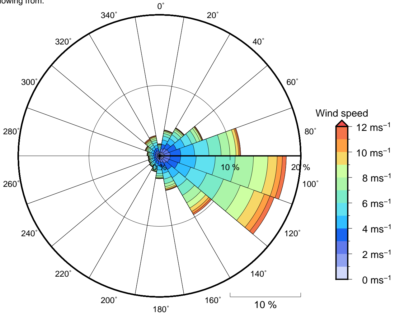
Figure 11 Annual wind rose for Black Rock. Note that directions are where the wind is coming from .
