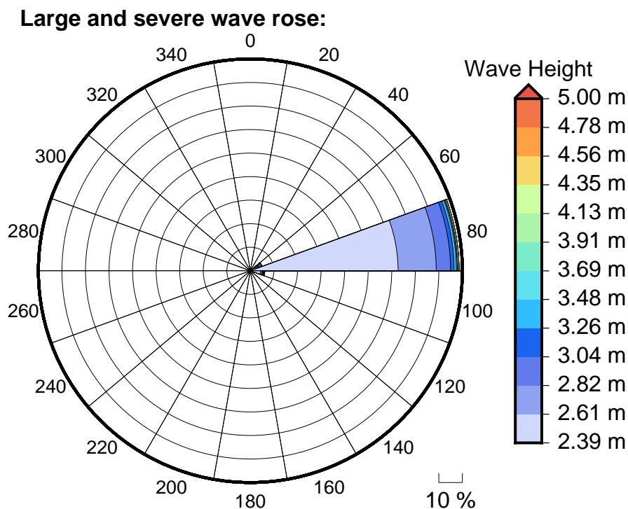
Figure 6 Large, severe and extreme wave roses for Ngatangia passage
