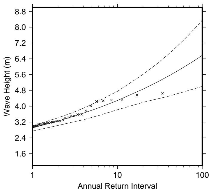
Figure 9 Extreme wave distribution for Ngatangia passage. The crosses represents the wave events that occurred since 1979. The plain line is the statistical distribution that best fit the past wave events. The dotted line show the upper and lower high confidence of the fit, there is a 95% chance that the fitted distribution lie between the two dashed lines.
