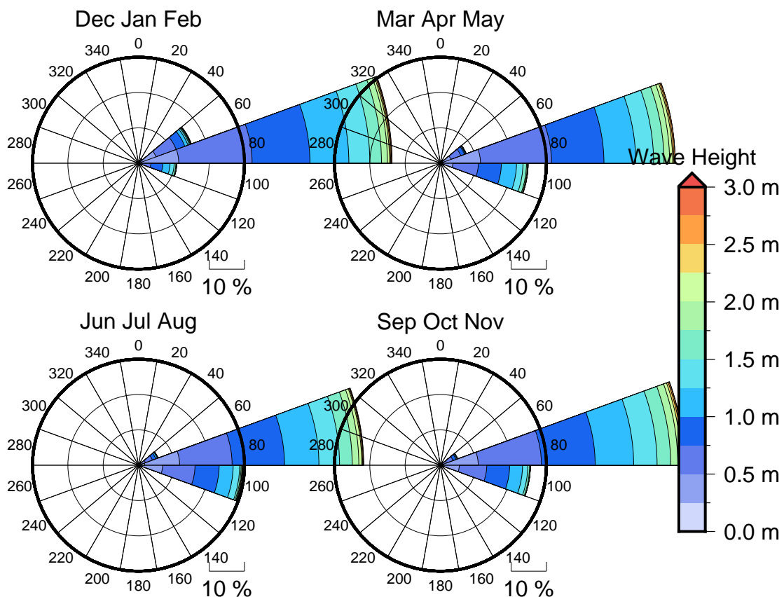
Figure 3 Seasonal wave roses for Ngatangia passage
