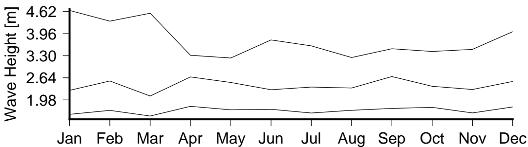
Figure 7 Monthly variation in large waves (90th percentile)(lower curve), severe waves (99th percentile) (middle curve) and the largest wave(upper curve) in Ngatangiiia passage.
