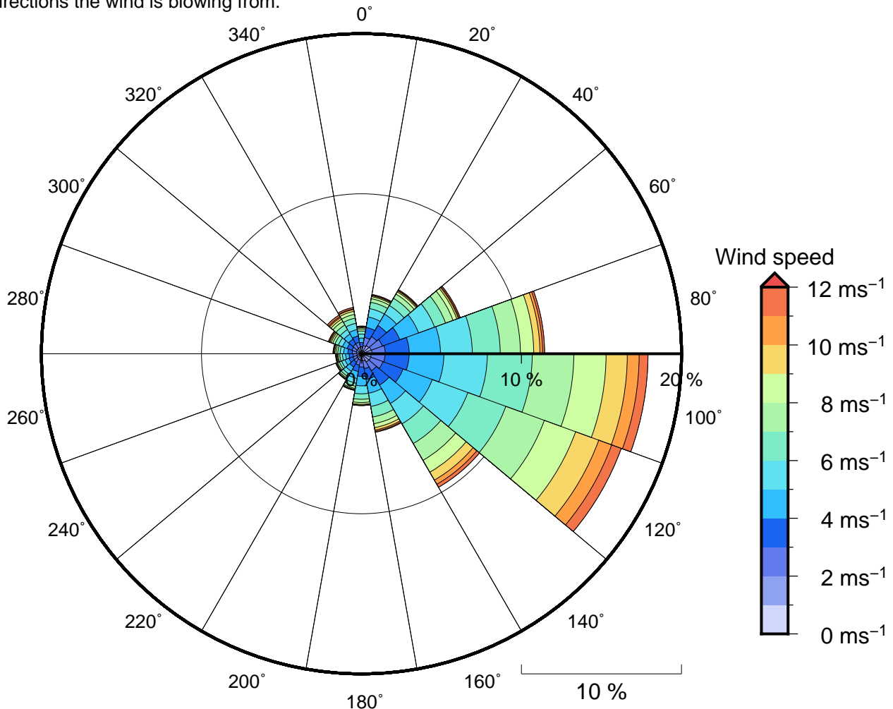
Figure 11 Annual wind rose for Ngatangia passage. Note that directions are where the wind is coming from.
