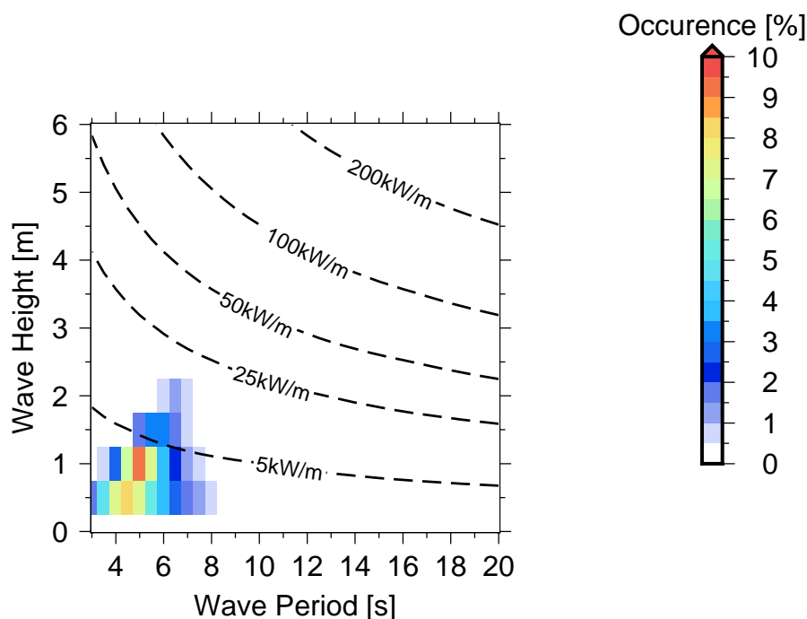
Figure 10 Occurrences of sea states in Ngatangia passage .
