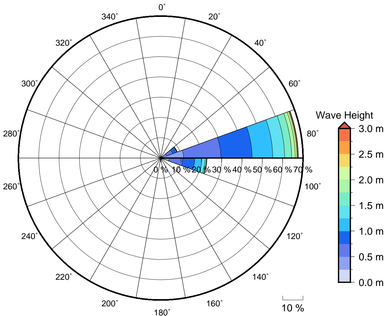
Figure 2 Annual wave rose for Ngatangia passage. Note that direction are where the wave are coming from.
