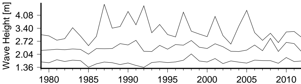
Figure 8 Annual variation in large waves (90th percentile)(lower curve), severe waves (99th percentile) (middle curve) and the largest wave(upper curve) in Ngatangiiia passage.
