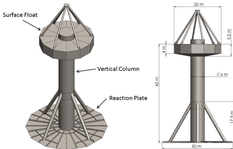
Figure 3: Representation of the RM3 device. (Reference Models for MHK Technology Design, Analysis, and Levelized Cost of Energy (LCOE) Estimates, 2013)
