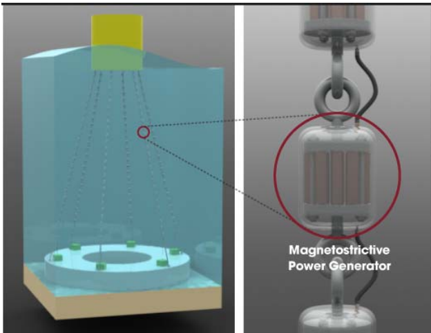
Figure 8: Representation of a prior version of the Oscilla Power iMEC device. [ http://oscillapower.com/wp-content/uploads/2012/02/wavearraythreepanel11.png ].
