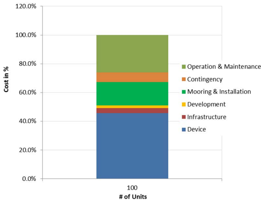
Figure 4: High-Level Cost Breakdown — Point Absorber Technology over a 25 year lifetime.
