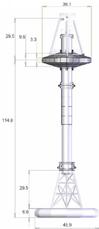
Figure 7: Representation of the Ocean Power Technologies PowerBuoy 150 device (dimensions shown in feet). http://www.oceanpowertechnologies.com/pb150.html
