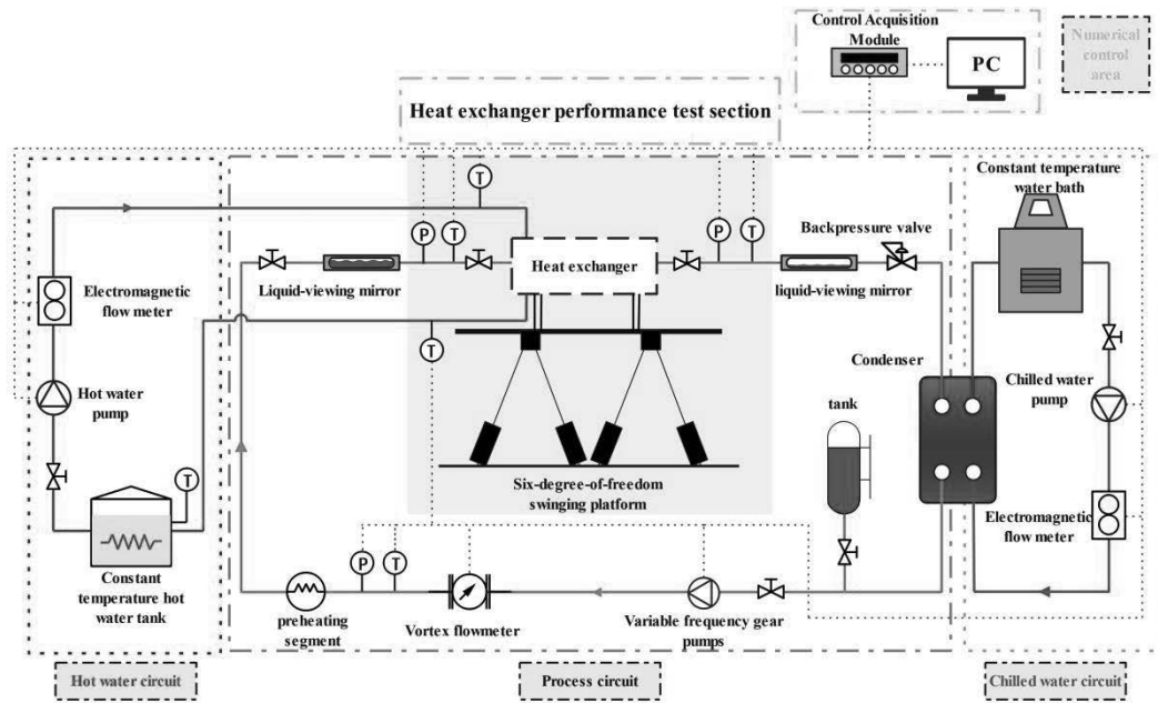
Figure 1(a) Heat exchanger thermal performance testing system
