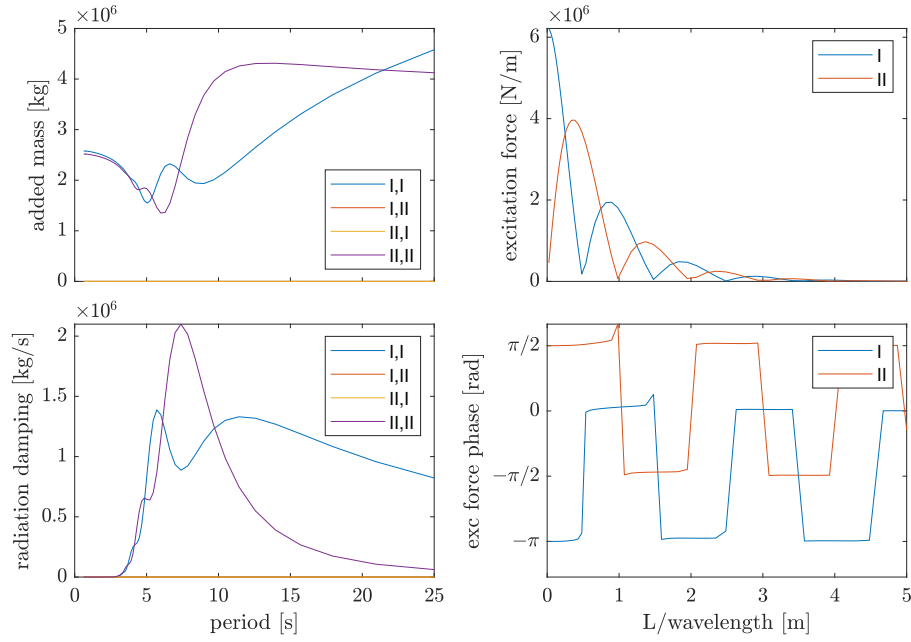
Fig. 7. Added mass, radiation damping, excitation force coefficients, and the phase of the excitation force, for a = 5 m, L = 50 m, d = 10 m, h = 30 m, and p_0 - p_{\text{atm}} = 10 m (of water).
