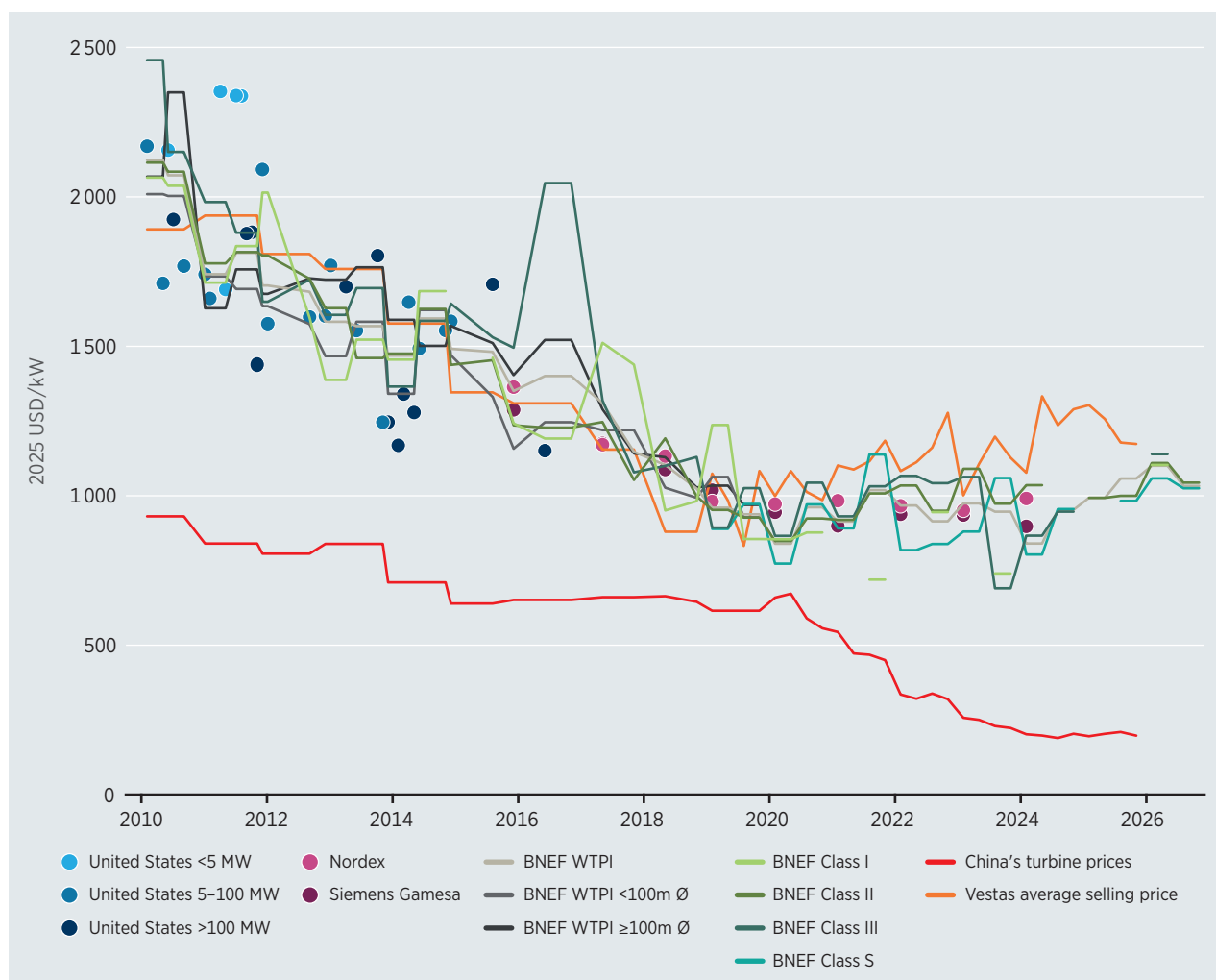
Figure 2.6 Wind turbine price indices and price trends, 2010–2025
