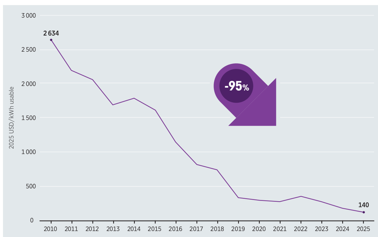
Figure 9.2 TICs of battery energy storage project, 2010–2025
