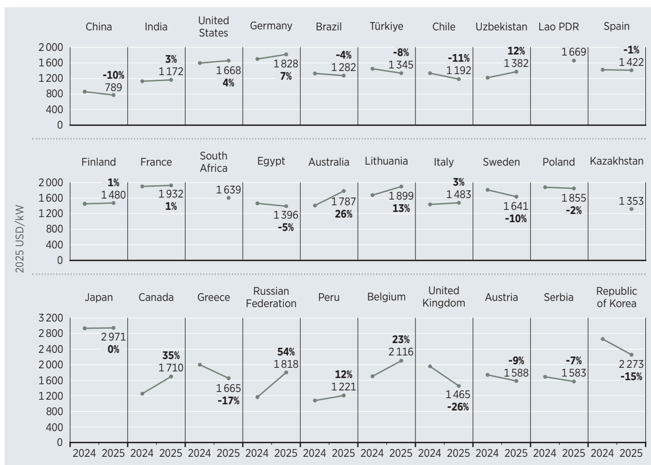
Figure 2.4 Onshore wind weighted-average TICs in selected markets, 2024–2025
