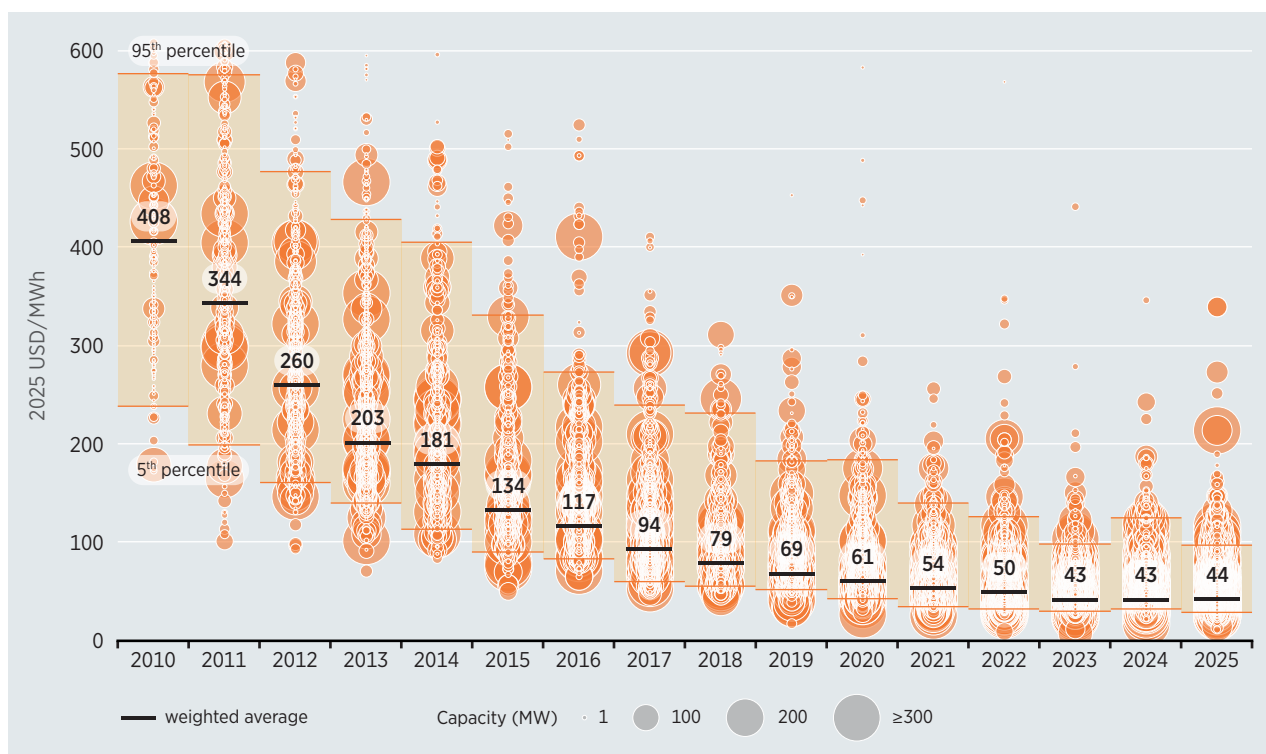
Figure 3.6 LCOE of utility-scale solar PV projects and global weighted-averages, 2010–2025
