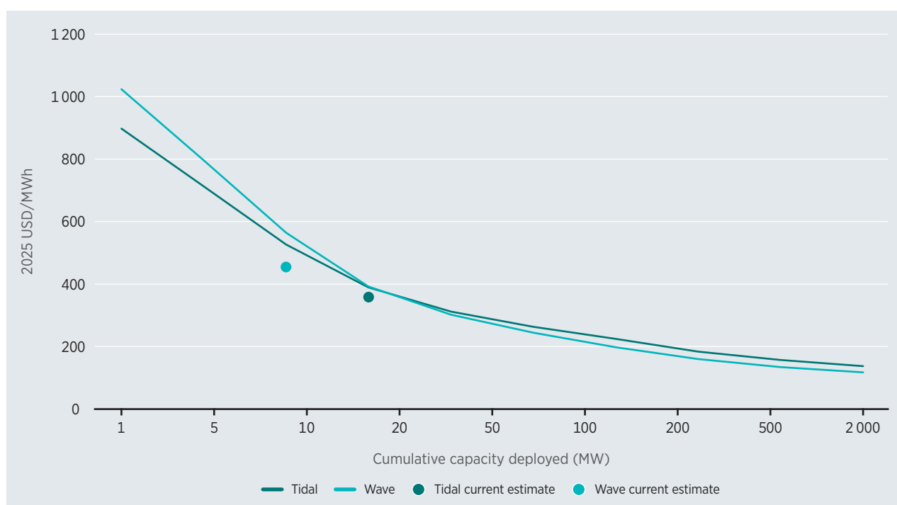
Figure 10.1 Levelised cost of electricity against cumulative deployment in 2025 USD/MWh
