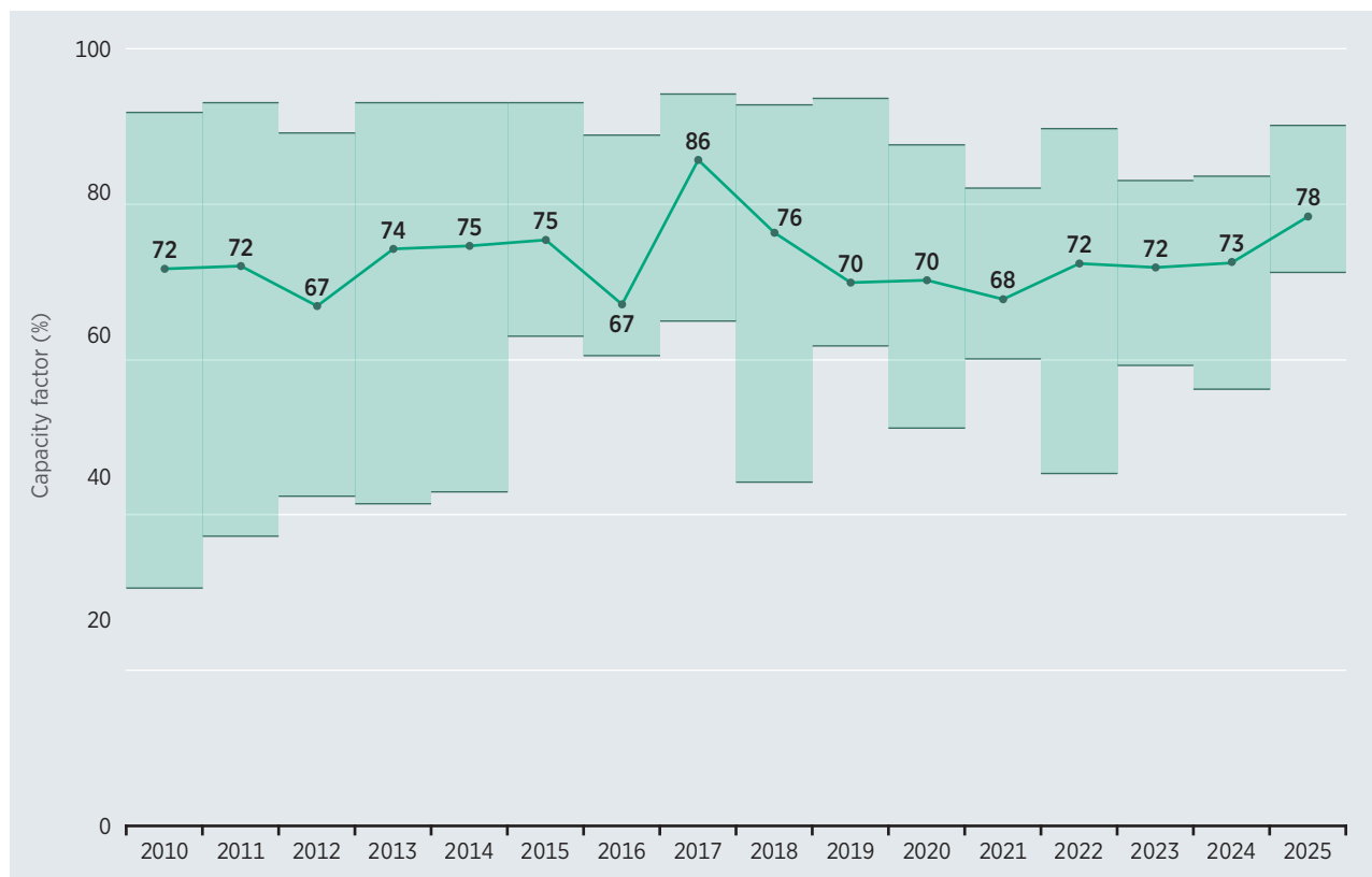
Figure 8.6 Capacity factor of bioenergy projects and global weighted-average, 2010–2025
