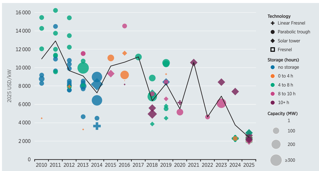
Figure 5.1 TICs for CSP by project size, collector type and amount of storage, 2010–2025
