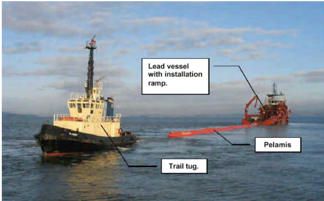
Figure 36 - Pelamis Deployment
