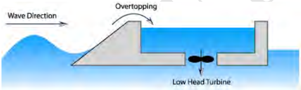
Figure 24 - Overtopping principle
