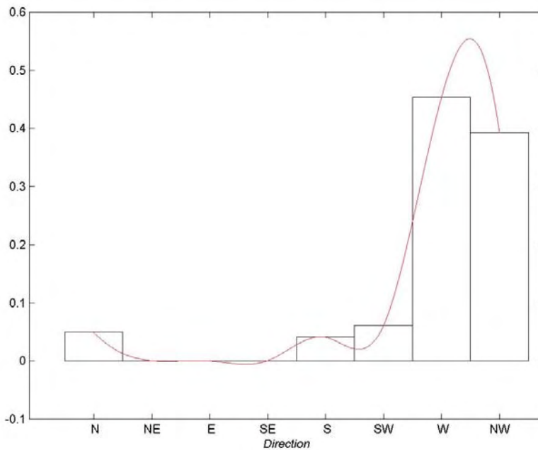
Figure 15 - Directional Distribution of waves in cell 9
