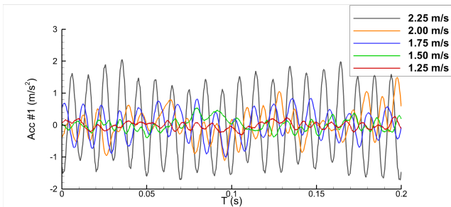
Fig. 20. Time series of accelerometer no. 1 data. Turbine operation at TSR = 2.4 and variable towing speed.
