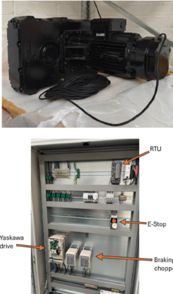
Fig. 4. The generator set (top) and the electrical cabinet (bottom).
