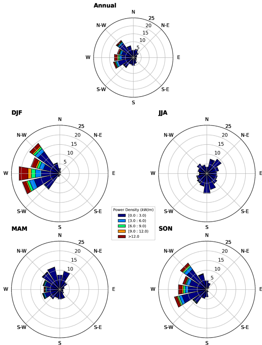
FIGURE 6 | Annual and seasonal wave rise of wave power density at NOITS from the 10-year wave data.
