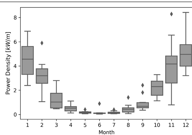
FIGURE 5 | Box-plot of the monthly means of wave power density at the NOITS derived from 10-year wave data. Lines inside box and upper and lower box boundary are median and 75th and 25th percentiles, respectively. Error bars indicate 95% confidence intervals, and diamonds are data falling outside 95% confidence intervals.
