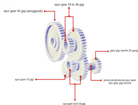
Figure 2. Gearbox Arrangement
