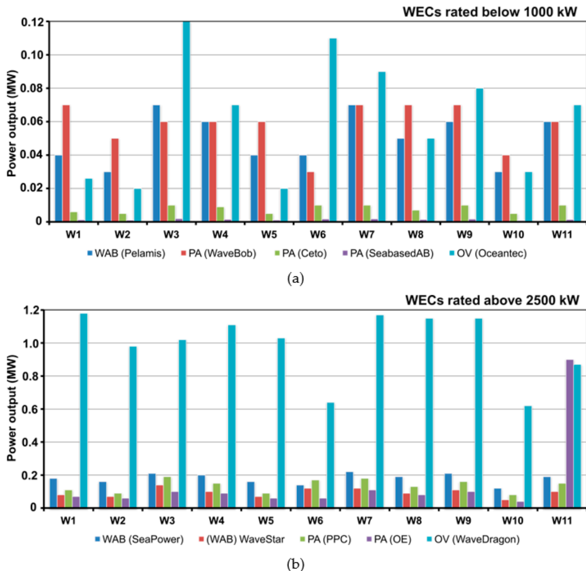
Figure 3. Theoretical power output (in MW) of various WECs for 11 locations. (a) WECs rated below 1000 kW in their power matrix. (b) WECs rated above 2500 kW in their power matrix.
