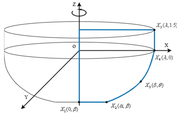
Figure 6. Geometry definition.
