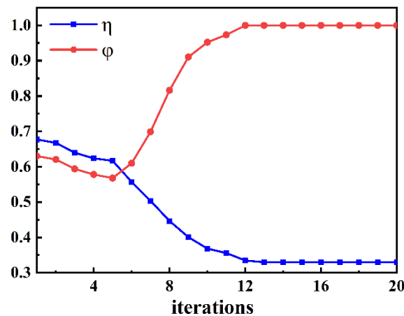
Figure 14. Buoy taper and flatness variation curve.
