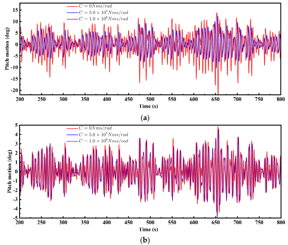
Figure 12. Motion response: (a) buoy pitch motion response; (b) swing-arm system pitch motion response.
