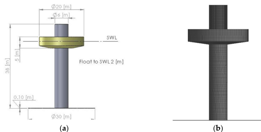
Figure 7. RM3 model: (a) geometric model from Ruehl K et al.; (b) grid model for AQWA frequency domain calculations in this paper.
