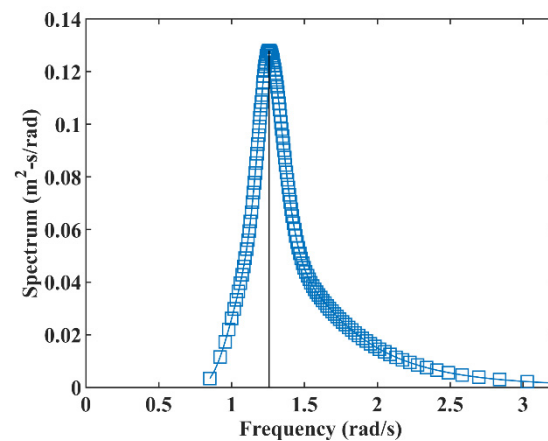
Figure 9. JS spectral density function curve.
