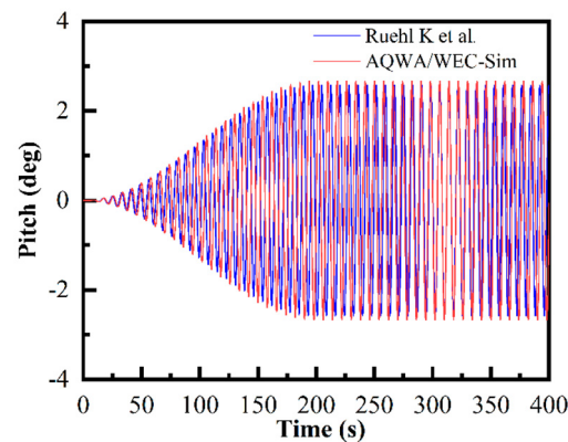
Figure 8. The simulation results compared with the results published by Ruehl K. et al. [43].
