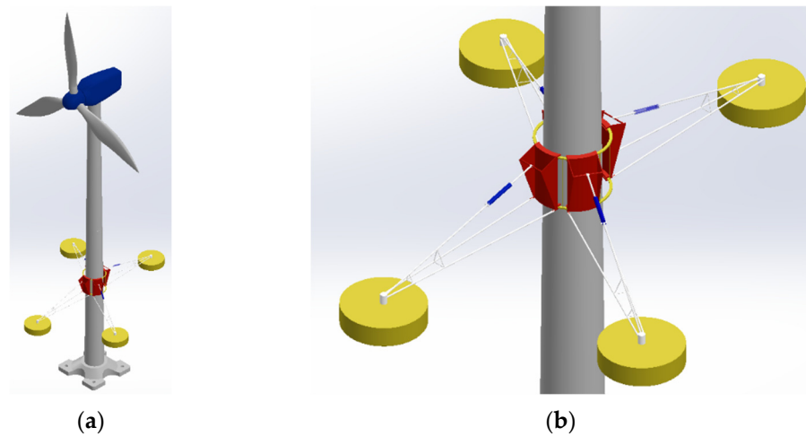
Figure 1. Three-dimensional model of wind and wave combined device: (a) modelling diagram; (b) Partial enlargement diagram.
