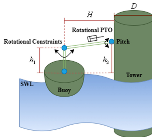
Figure 2. Schematic representation of WEC in pitch motion.
