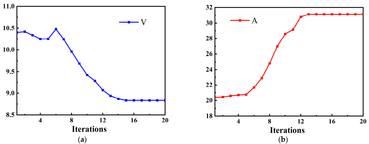
Figure 13. Iterative curves of characteristic parameters: (a) draft volume variation curve; (b) wet surface area variation curve.
