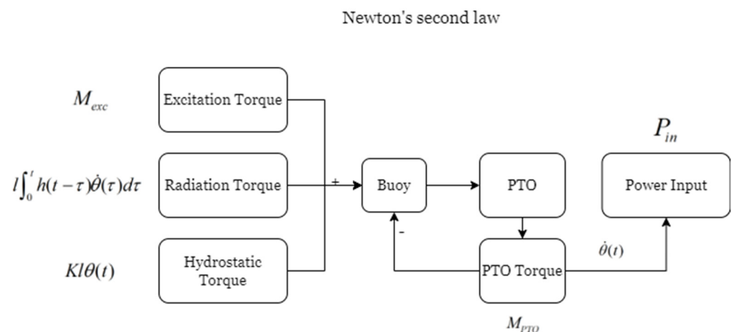
Figure 3. The torque composition analysis of the swing-arm WEC.
