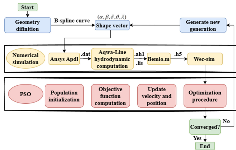
Figure 5. Buoy shape optimization flow chart for the PSO algorithm.
