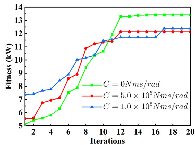
Figure 11. Iterative curve graph.
