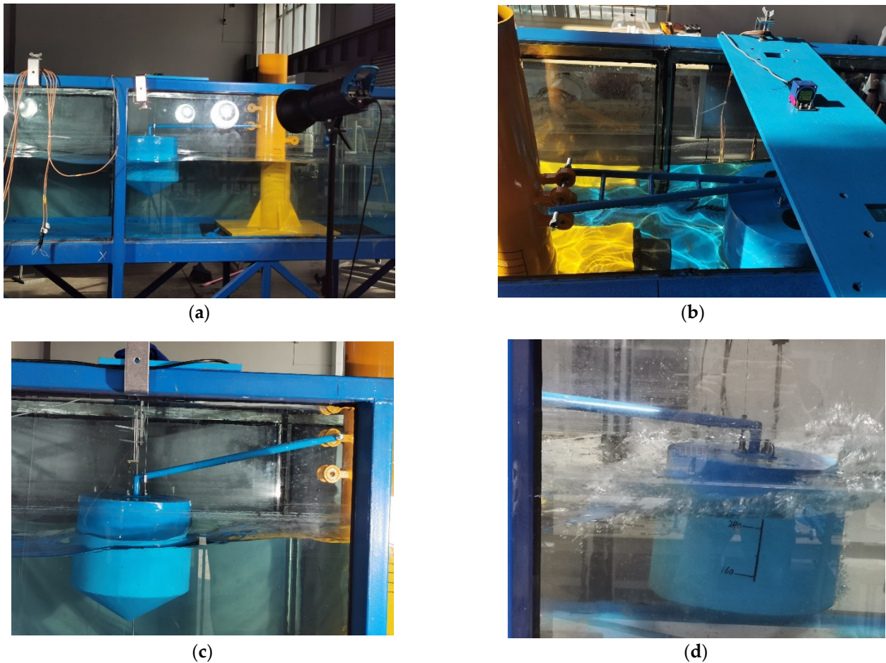
Figure 15. Experimental layouts: (a) high-speed camera setup; (b) Sensor setup; (c) buoy at rest; (d) buoy oscillation State.
