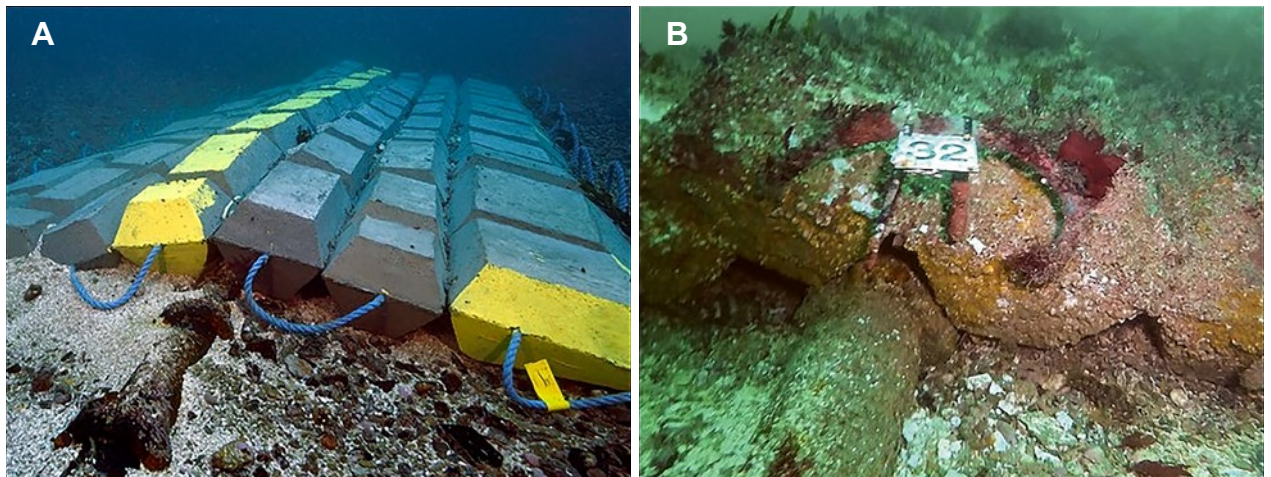
Figure 9. Iron shells and concrete mattresses of iron shells and concrete mattresses used to protect unbundled cable at the Paimpol-Bréhat tidal turbine test site (France) (A) one month after installation; (B) six years later during a video survey. Source: Hemery, 2000.
