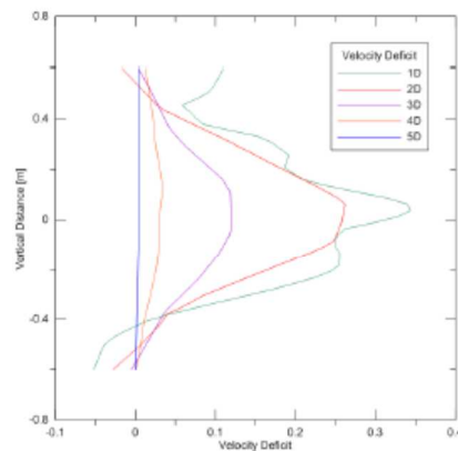
Fig. 2 Velocity Deficit – TSR = 5, V_0 = 1.54 m/s
