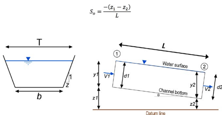
Figure 1. Canal cross-section (left) and profile (right) parameters
