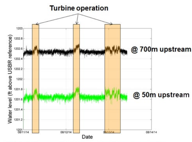
Figure 6. Water level time series at the Roza Canal site, at 50 m and 700 m upstream of the turbine.
