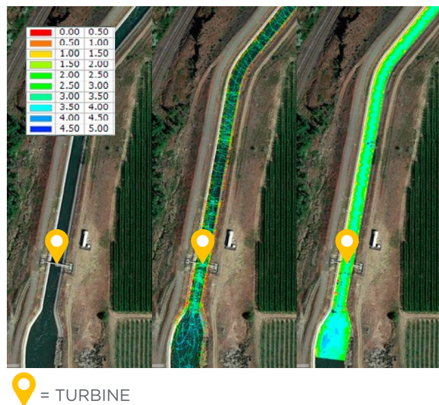
Figure 5. An example of a coarse bathymetric survey using a single-beam echo sounder at the Roza Canal site showing the satellite image with, no data (left), raw data (middle), and the interpolated data (right).
