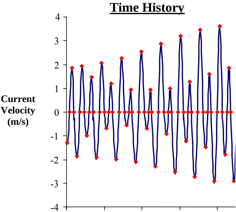
Figure 4-4. Construction of Velocity Time History
