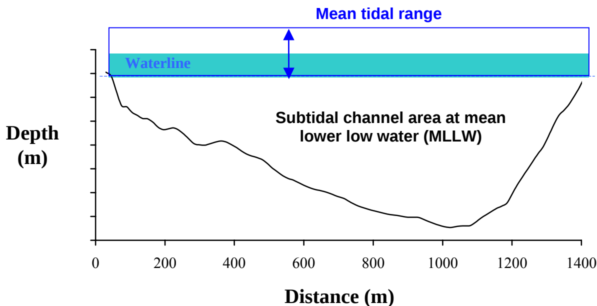
Figure 3-3 Accounting for Tidal Range in Cross-Sectional Area Calculation
