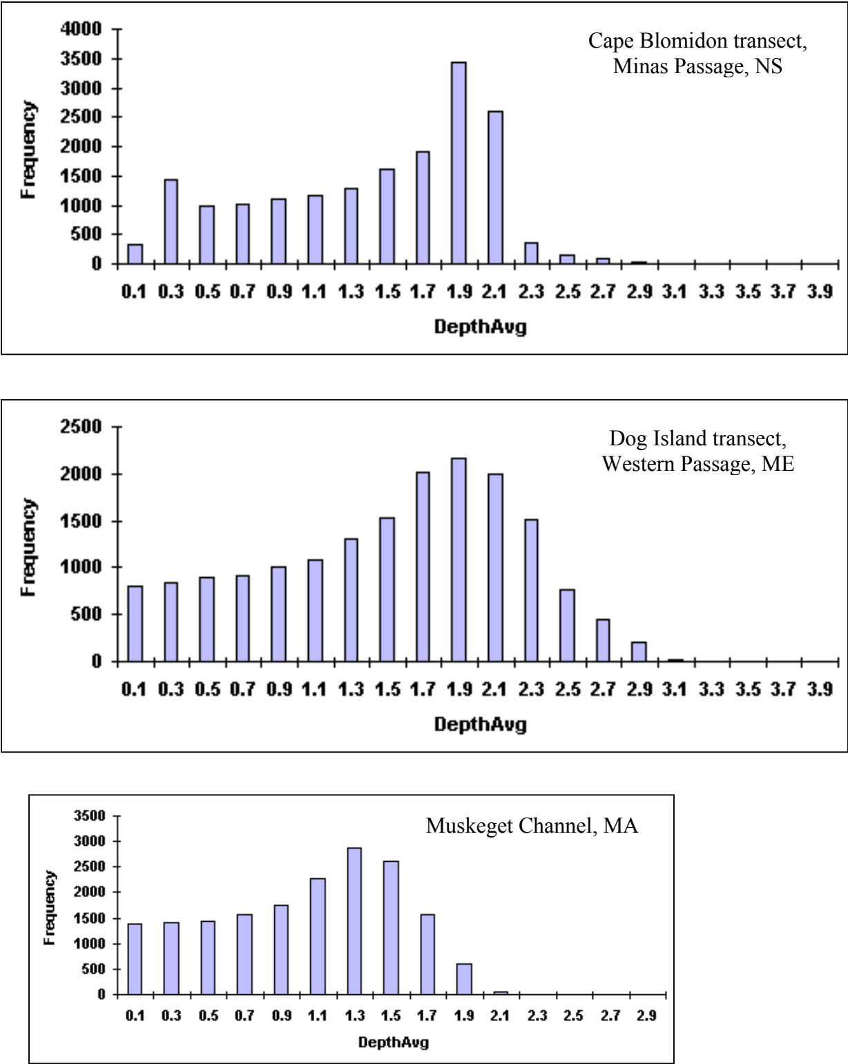
Figure 4-1. Depth-Averaged Tidal Current Speed Probability Distributions for North American East Coast Sites
