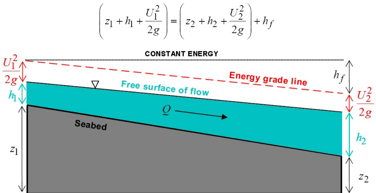
Figure 4-5. Open-Channel Flow Theory: Energy Equation and Definition Sketch
