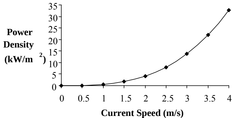
Figure 1-8 Incident Power Density as a Function of Current Speed
