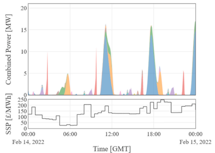
Fig. 9. Sample day of stacked generation from all sites, with energy price (SSP) shown.
