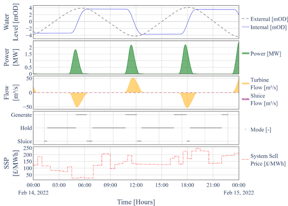
Fig. 6. Sample day of operation – Barry single turbine.
