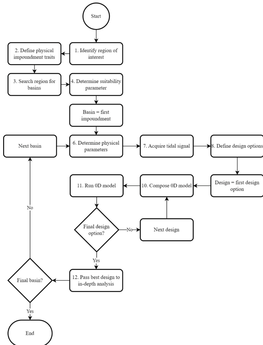
Fig. 2. Flow chart of small tidal range scheme initial assessment process.
