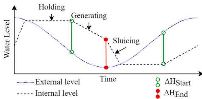
Fig. 1. Example operation of tidal range scheme.
