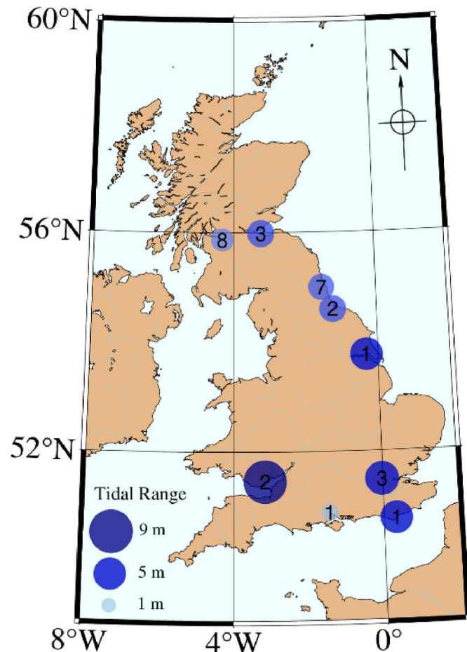
Fig. 3. Number of suitable basins identified around the UK.
