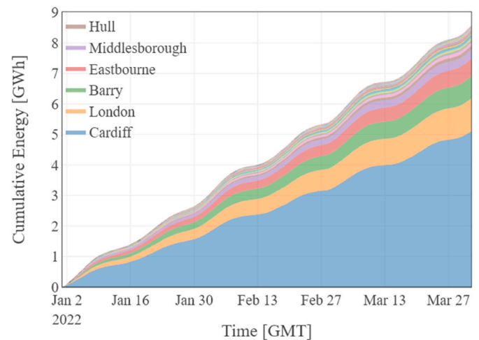
Fig. 8. 2022, three months stacked energy production from assumed tidal dock basins.
