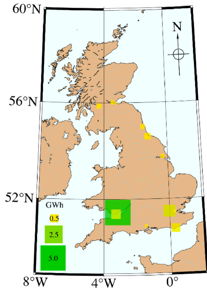
Fig. 7. Maximum three month energy generation, markers scaled and coloured on best output (plotted using Generic Mapping Tools [47]).
