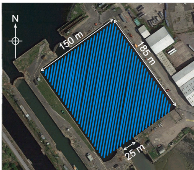
Fig. 5. Barry docks assumed basin (annotated).
