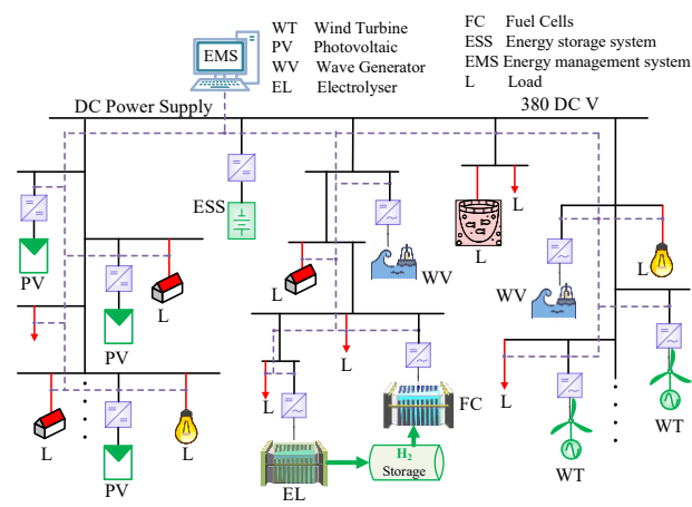
Fig. 1: Schematic of Islanded Hydrogen DC Microgrid (Solid lines: electrical power flow; dashed lines: communication/control links).
