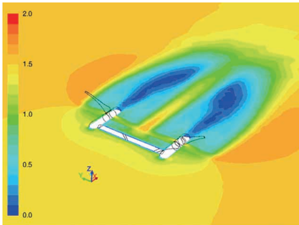
Example of CFD analysis for flow around rotating turbine
