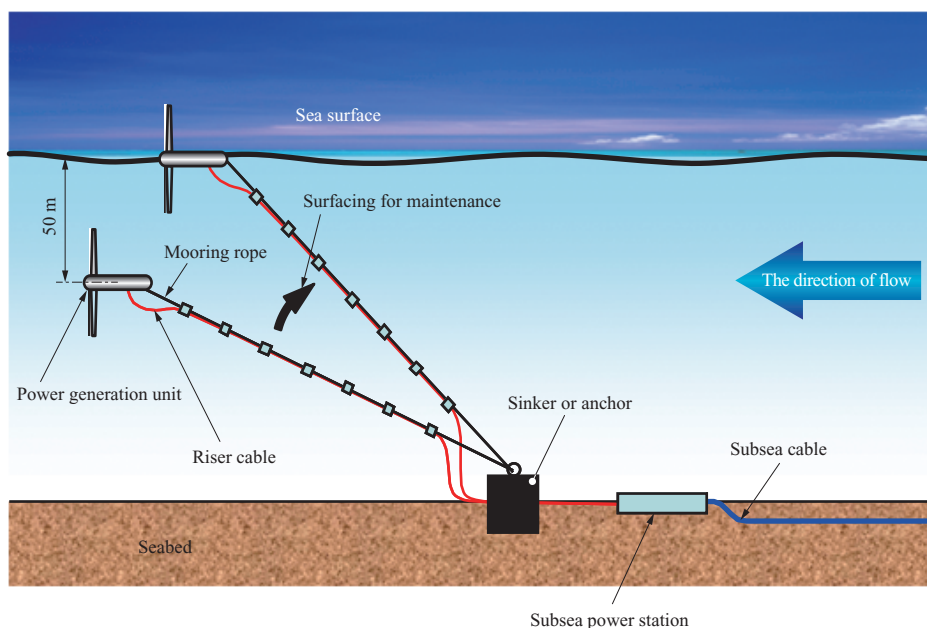
Diagram of floating type ocean current turbine system
