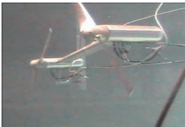
Tank experiment using scale model of floating turbine
