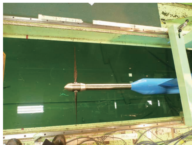
Turbine open test in towing tank
