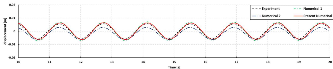
Figure 11. Comparison of cylinder displacement for validation ( B_{PTO} = 200 \text{ Nms} ).
