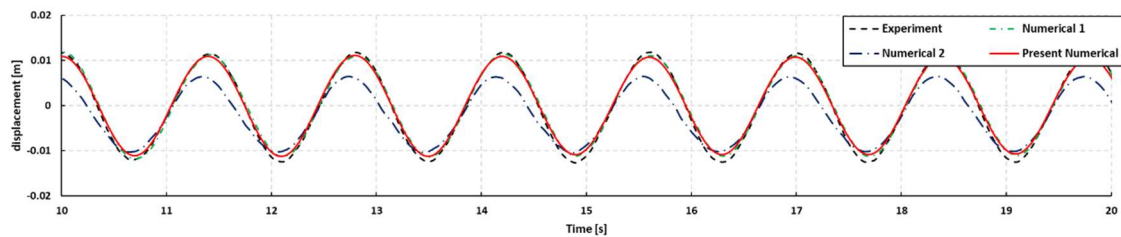
Figure 10. Comparison of cylinder displacement for validation ( B_{PTO} = 100 \text{ Nms} ).
