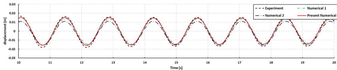
Figure 9. Comparison of cylinder displacement for validation ( B_{PTO} = 50 \text{ Nms} ).
