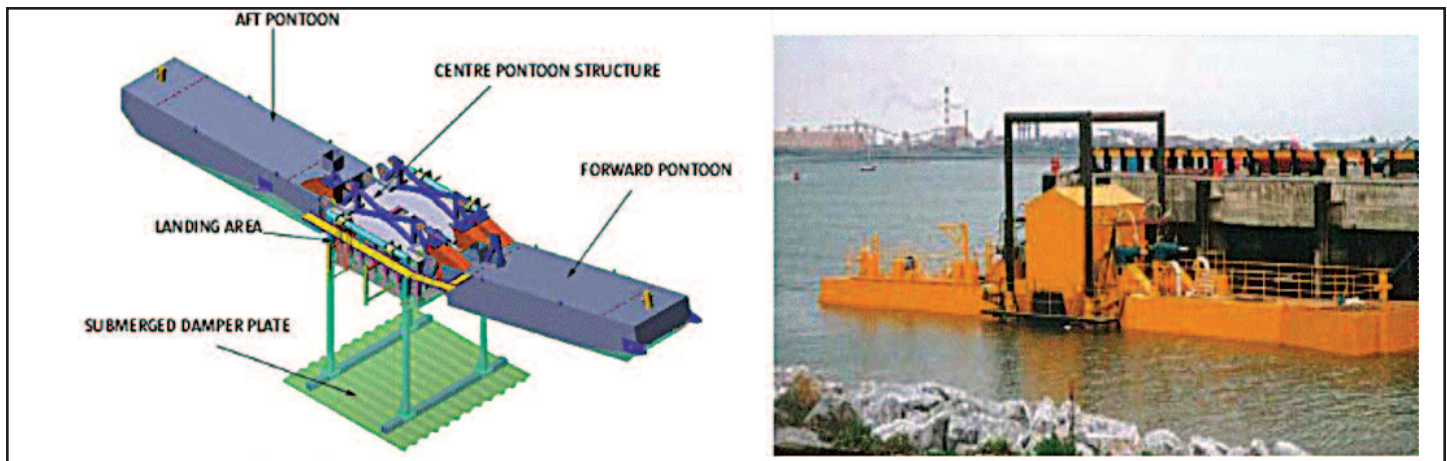
Figure 1. The McCabe Wave Pump
