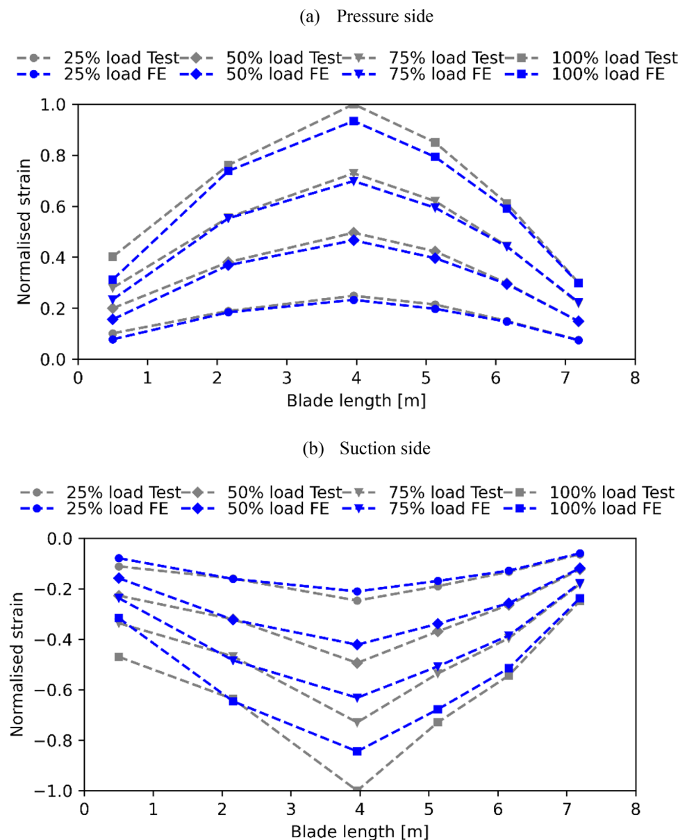
Fig. 10 Normalised blade longitudinal direction strain comparisons along the length of the blade between the testing data and FE results
