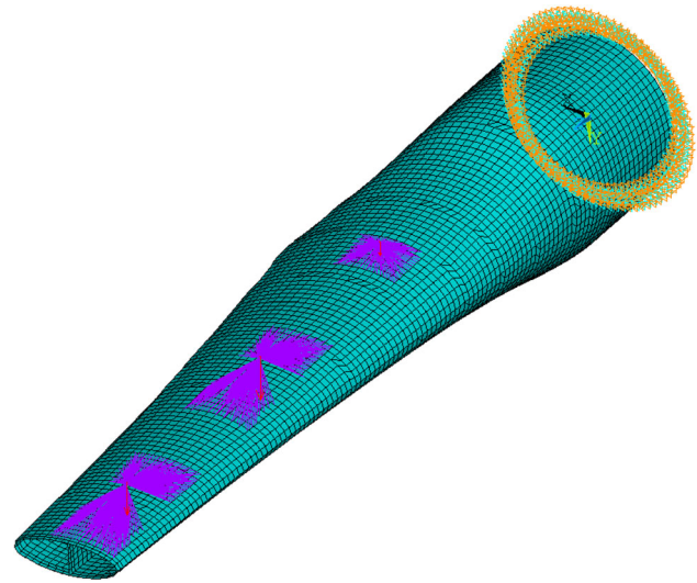
Fig. 6 Finite-element model of the blade
