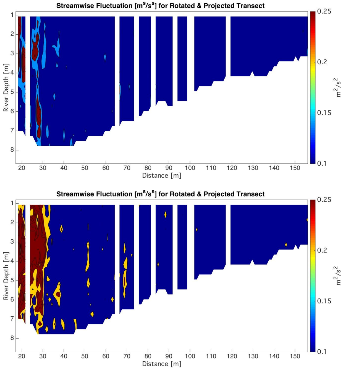
Figure 14. Streamwise fluctuation for each of the four transects from 6 m aft of the RDDP.
