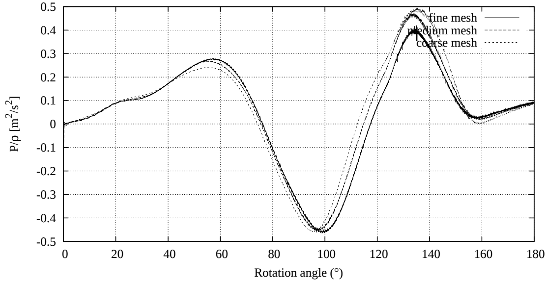
Figure 5.5: Pressure for each mesh at point 3.
