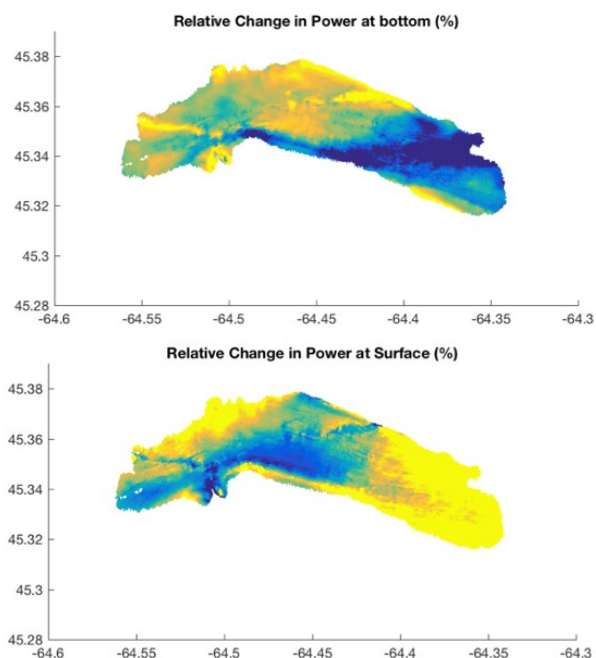
Fig. 15. Change in power if turbine is near bottom (top) or near surface (bottom).
