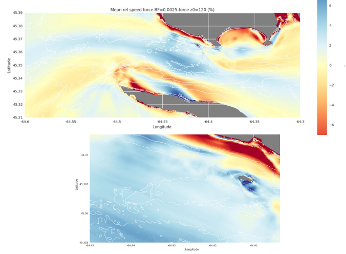
Fig. 7. The relative difference (%) in the mean speed, Acadia-FORCE with constant bottom friction minus variable bottom friction.
