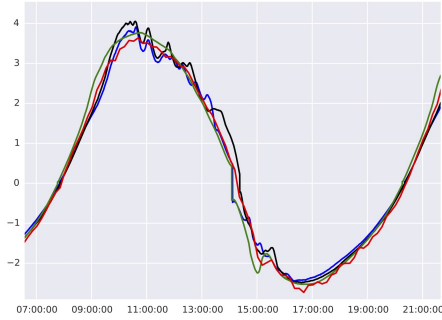
Fig. 12. Time series of the flow for a site in the FORCE region west of the volcanic platform. The red line is 5-minute averaged ADCP data. The blue and black curves are from Acadia-FORCE simulations with bottom-roughness and constant bottom drags. The green curve is from a 3D Acadia-FORCE simulation. The model simulations are sampled at a 10s rate.
