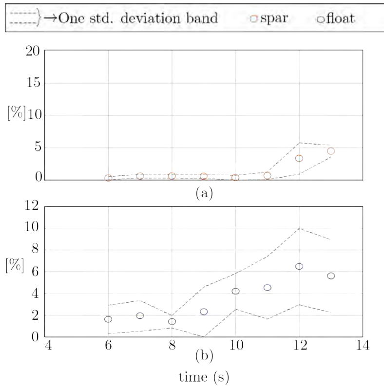
Figure 2.5: Mean standard deviation difference between the Reduced Order Model and WEC-Sim for irregular Waves for (a) spar and (b) float. (The dashed line represents one standard deviation band.)
