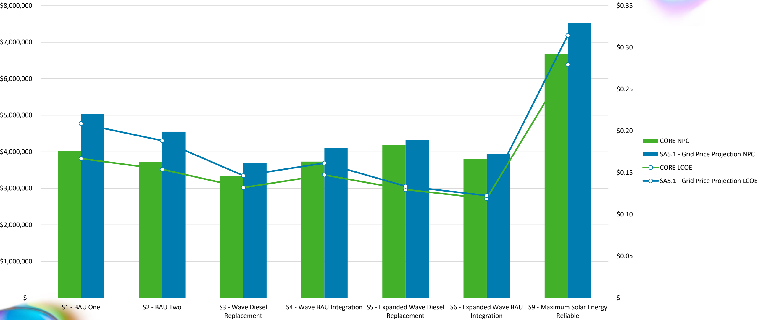
Sensitivity Analysis - Impact of Changing Grid Price (NPC vs LCOE)
