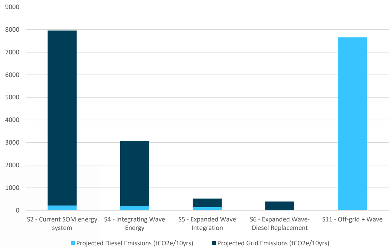
10 Year Emissions Analysis - BAU vs Wave Integration
