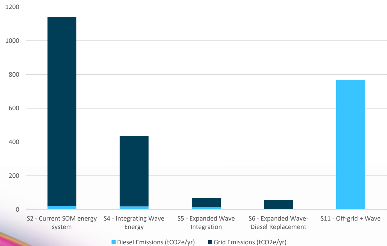
Annual Emissions Analysis - BAU vs Wave Integration
