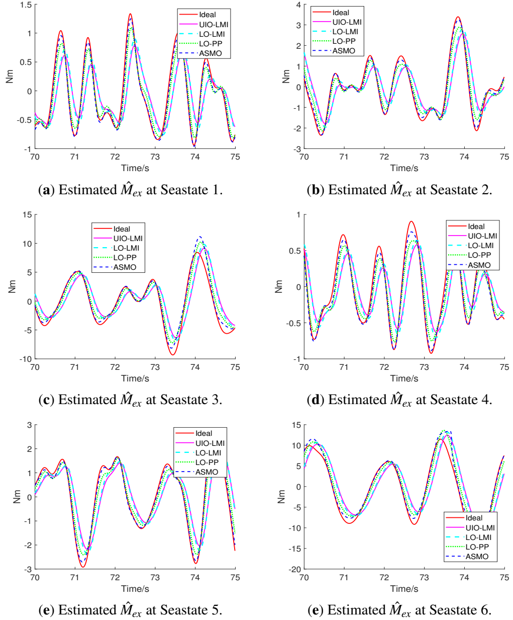
Figure 4.4: Estimated \hat{M}_{ex} from four methods at six sea states.
