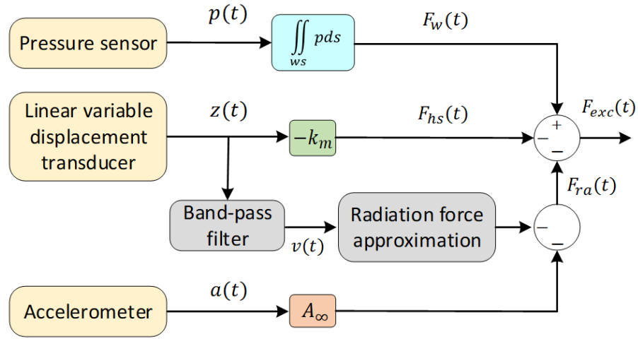
Figure 4.2: Both PAWEC motion and pressure measurements based WEF computation (Guo, 2017).
