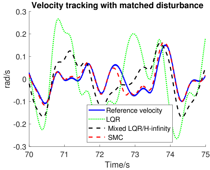
Figure 5.7: Velocity tracking of three methods with added matched disturbance (Seastate 2).
