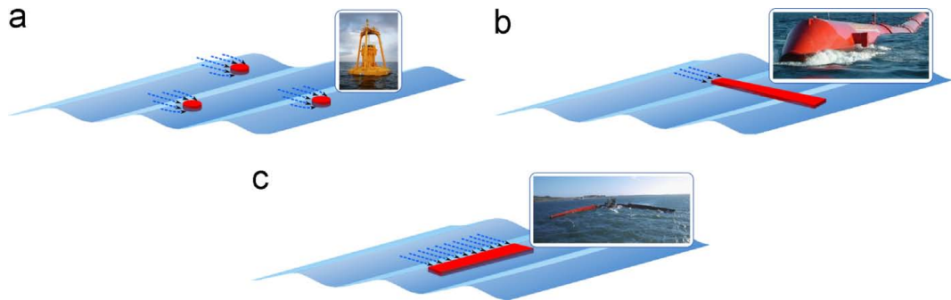
Figure 2.2: The classification by their dimension and orientation (López et al., 2013), including (a) point absorber (PowerBouy OPT), (B) attenuator (Pelamis), (c) terminator (Wave Dragon).
