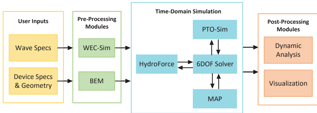
Figure 3.1: WEC-Sim code structure.
