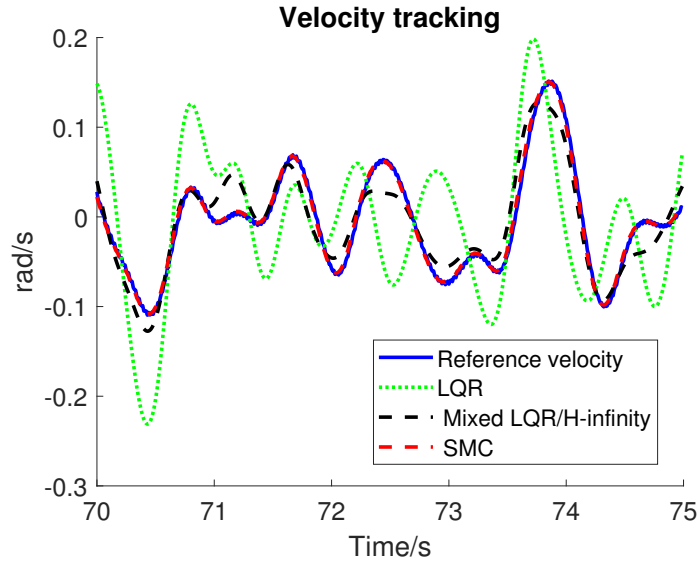
Figure 5.3: Velocity tracking of three methods (Seastate 2).
