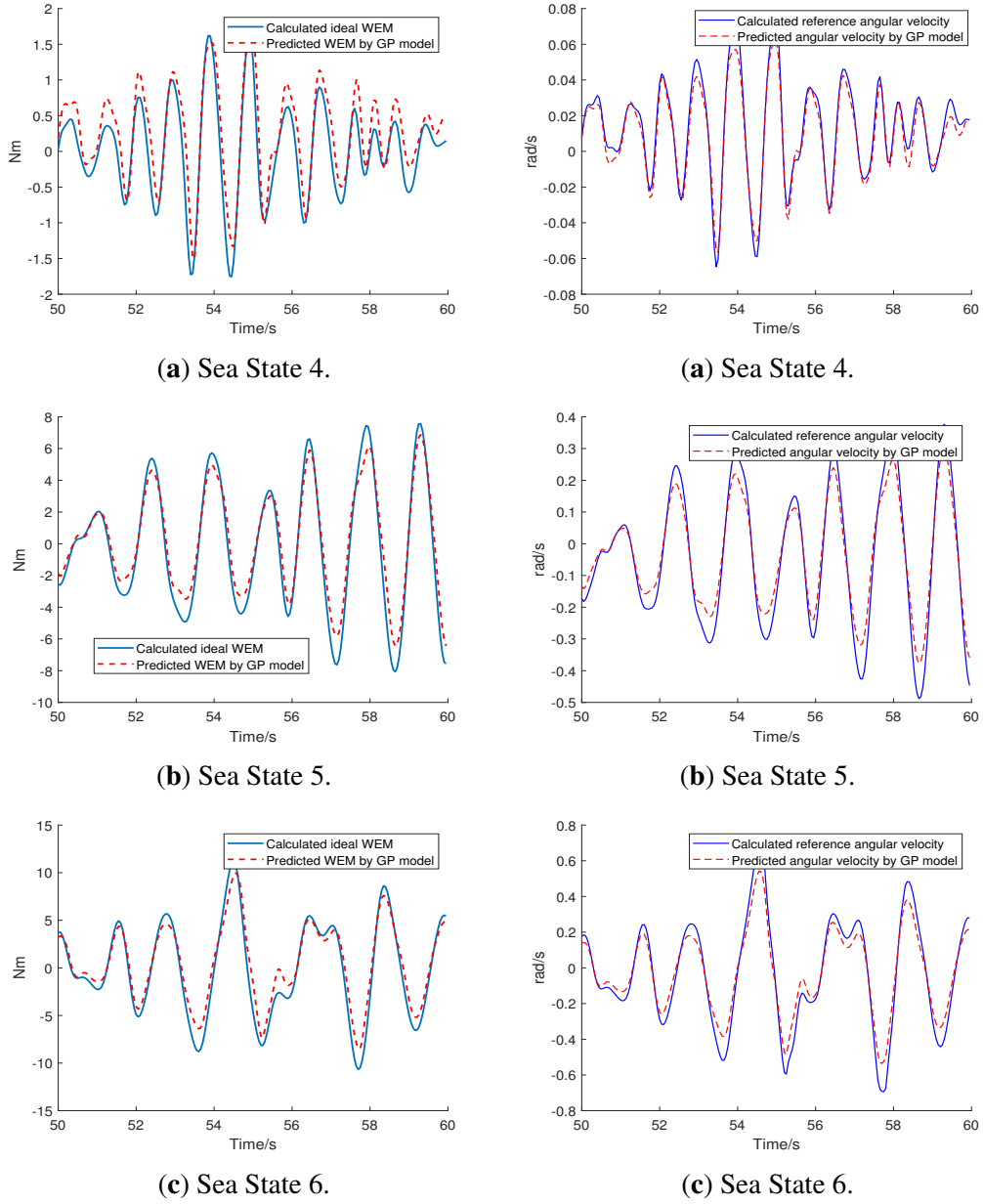
Figure 6.2: Predicted WEM and reference velocity by GP models (three sea states).
