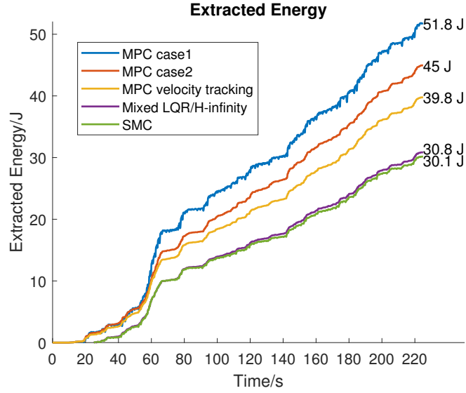
Figure 7.3: Extracted energy from all methods (Seastate 5).
