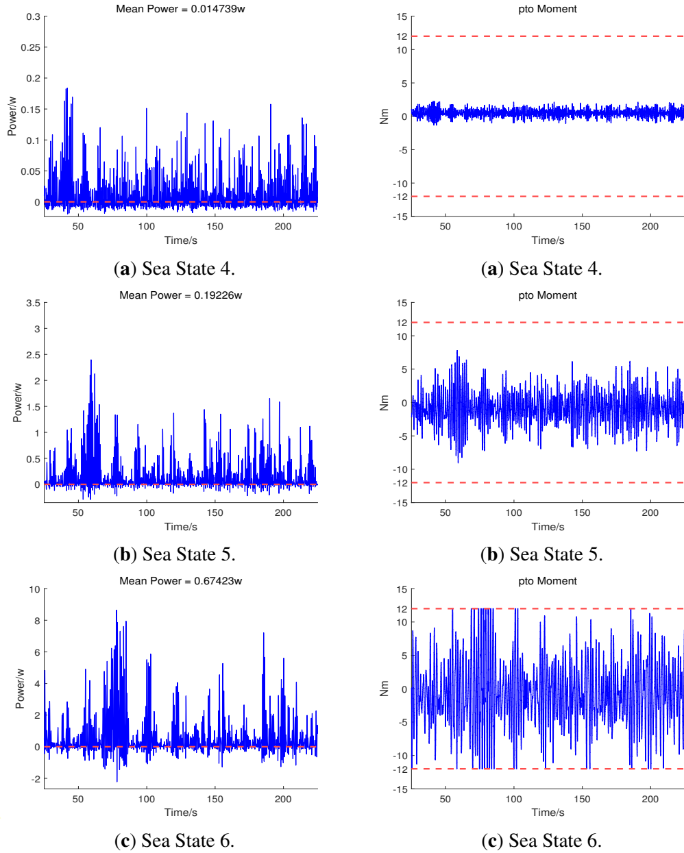
Figure 6.4: Generated instantaneous power and PTO moment (three sea states).
