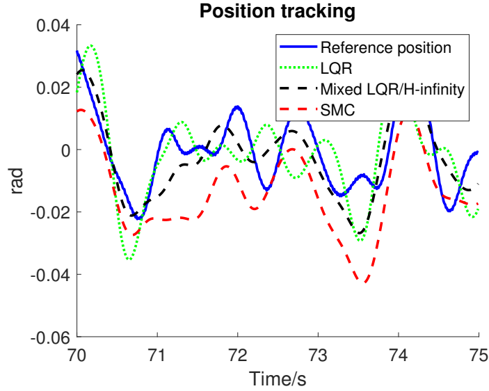
Figure 5.2: Position tracking of three methods (Seastate 2).
