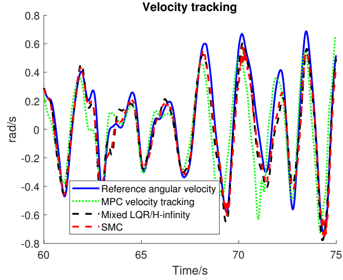
Figure 7.9: Velocity tracking results: (i) MPC, (ii) Mixed LQR/ H_\infty control and (iii) SMC approaches (Seastate 6).
