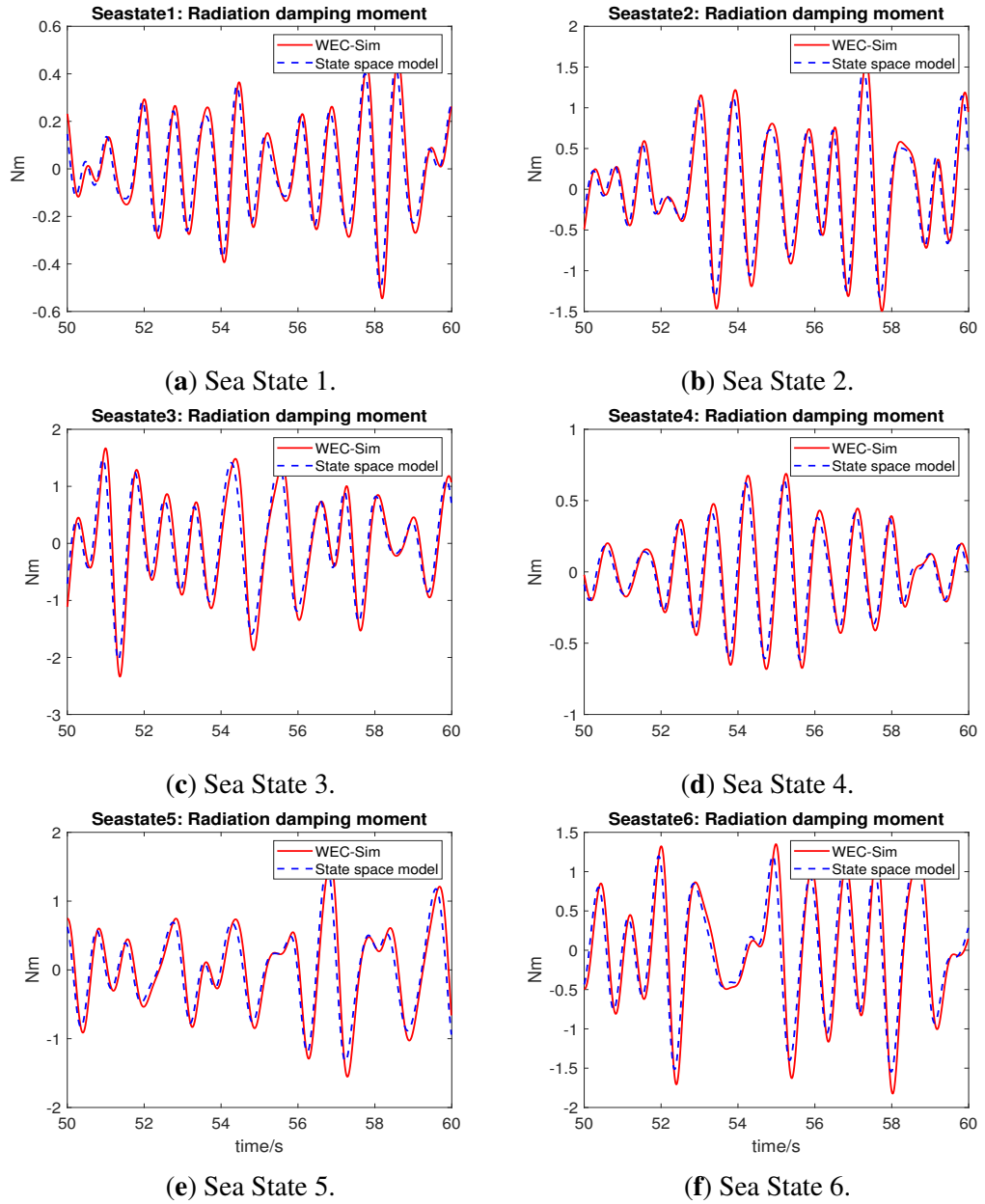
Figure 3.10: Radiation damping moment from WEC-Sim vs state space model approximation.
