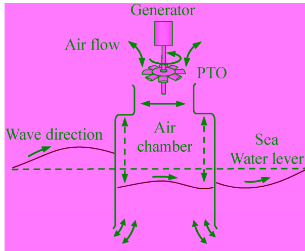
Figure 2.7: The basic structure of oscillating water column WEC (Zhang et al., 2021).
