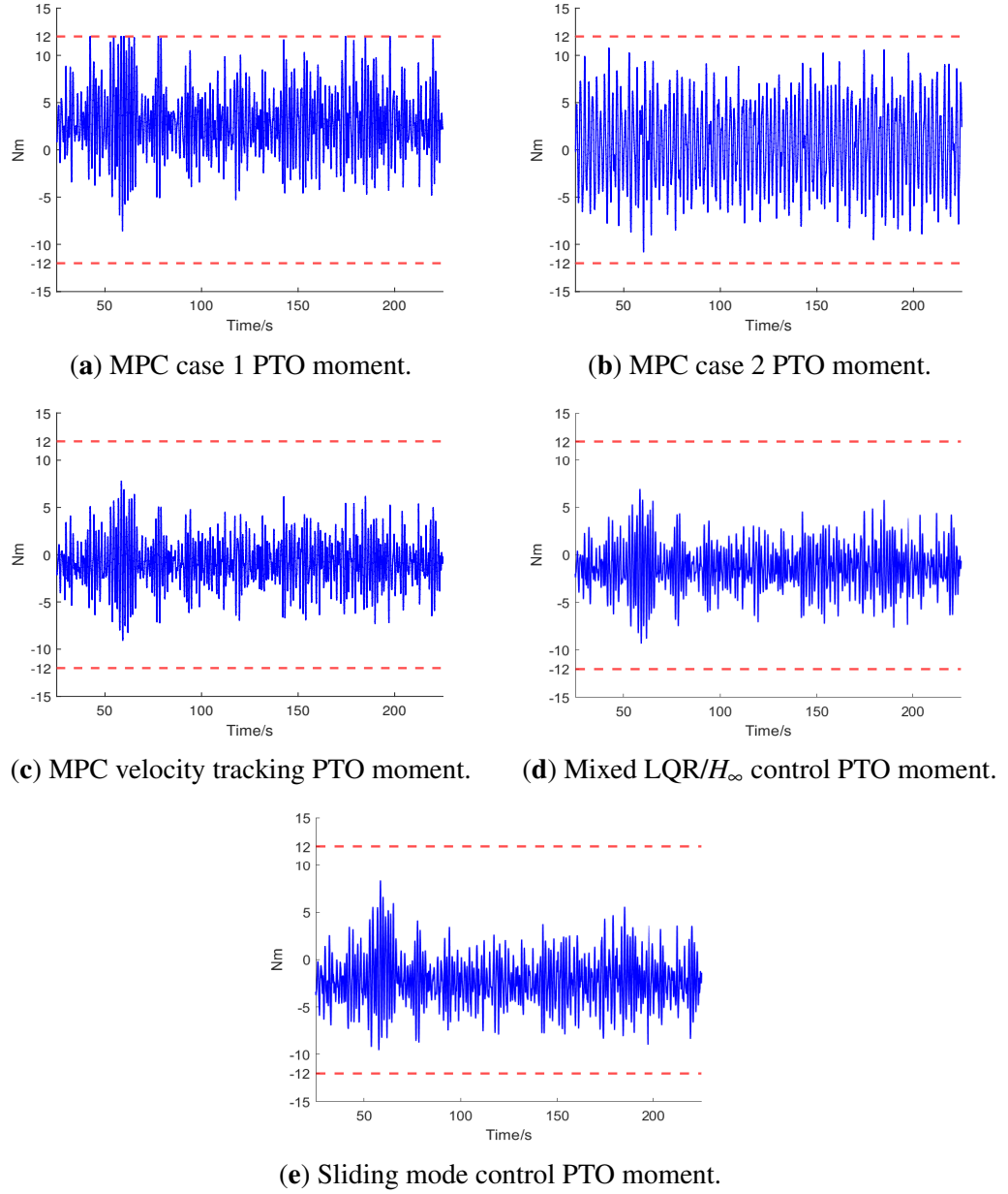
Figure 7.5: PTO moment of all methods (Seastate 5).
