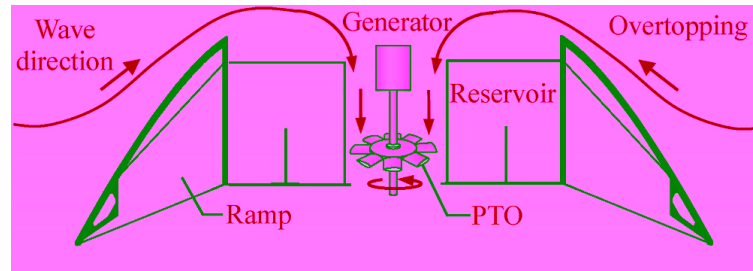
Figure 2.12: The basic working principle of overtopping WEC (Zhang et al., 2021).
