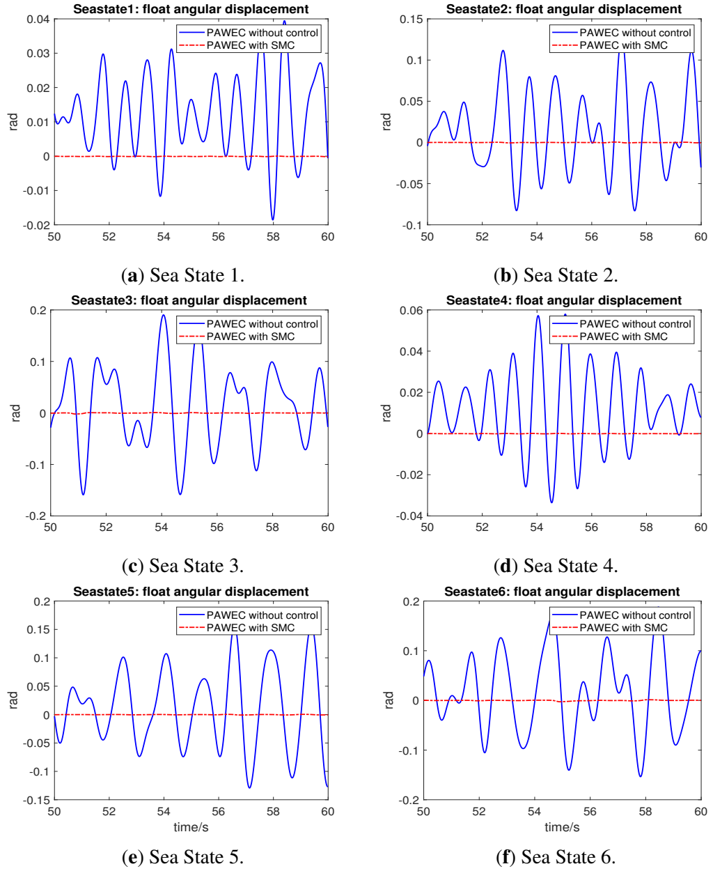
Figure 3.14: Regulation test: the float angular displacement of PAWEC without control or with SMC.
