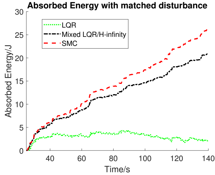
Figure 5.8: Absorbed energy from three methods with added matched disturbance (Seastate 2).
