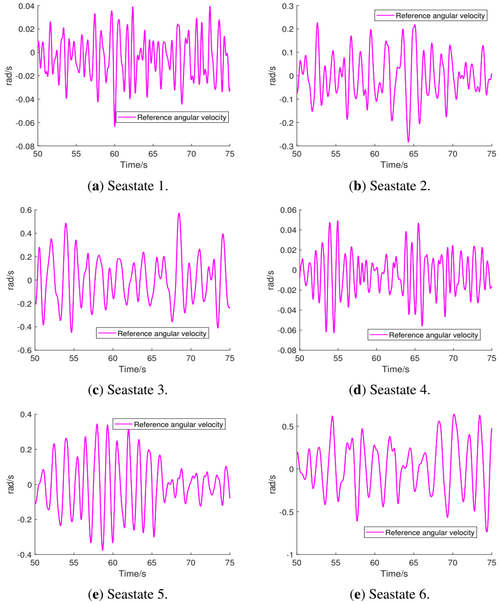
Figure 4.7: Optimal reference angular velocity at six sea states.
