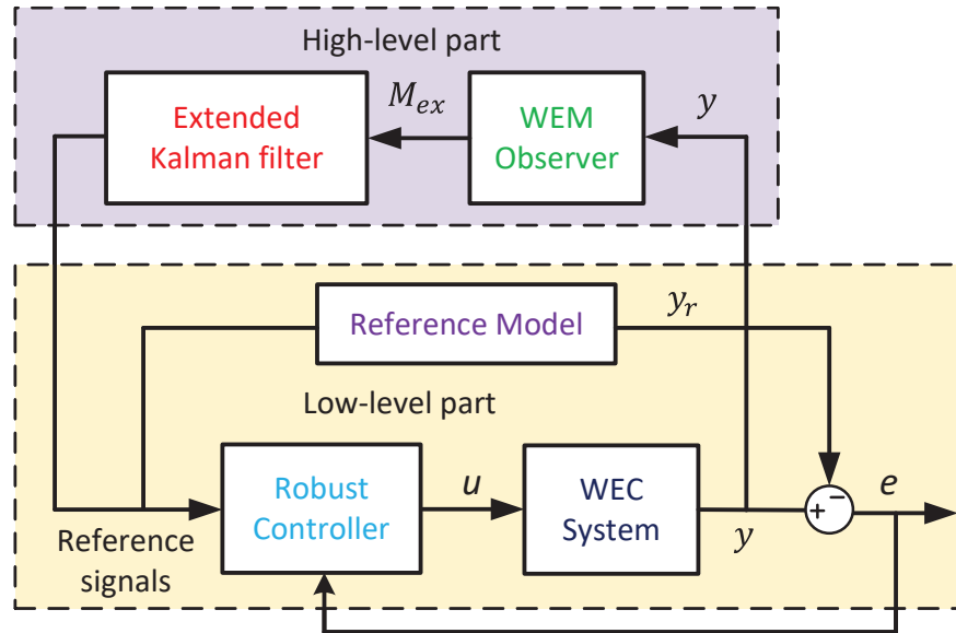
Figure 5.1: Overall tracking structure of model-following control.
