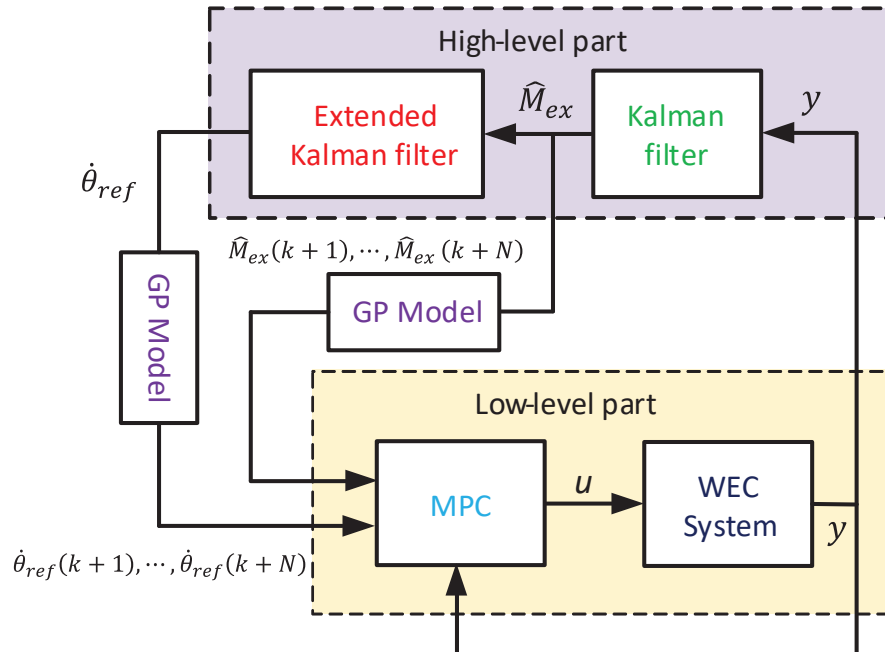
Figure 6.1: Tracking structure of model predictive control.
