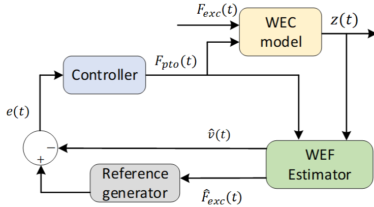
Figure 4.3: The PAWEC motion based way for WEF estimation (Guo, 2017).
