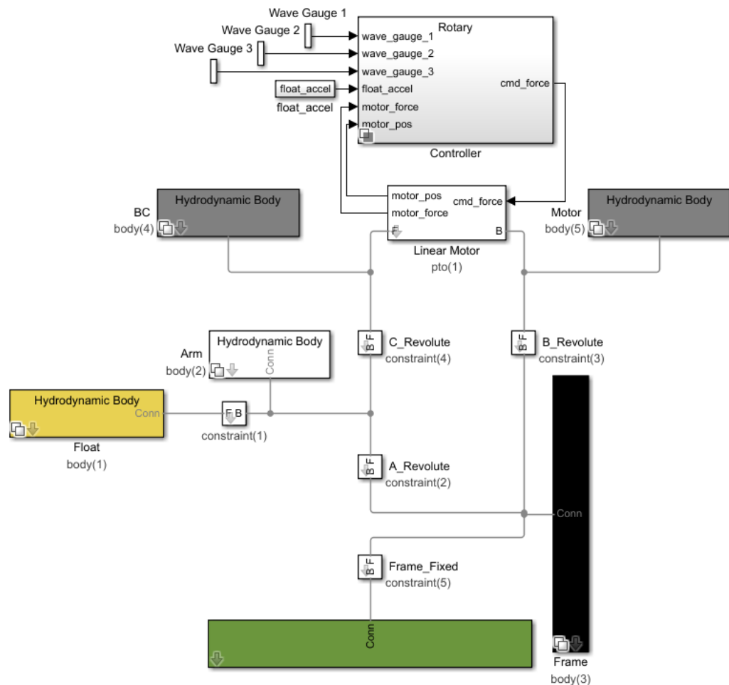
Figure 3.5: The scaled Wavestar Simulink model in WEC-Sim (Tom et al., 2018).
