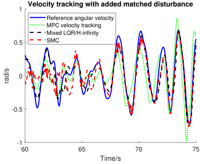
Figure 7.14: MPC velocity tracking, Model-following mixed LQR/ H_\infty control and SMC with matched disturbance (Seastate 6).
