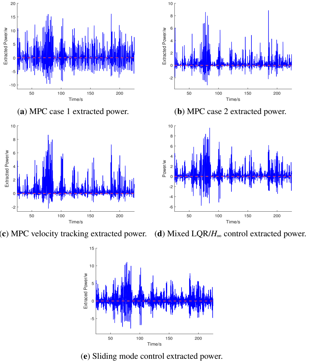
Figure 7.11: Extracted power of all methods (Seastate 6).
