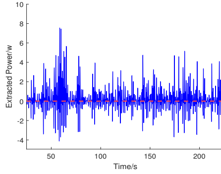
(a) MPC case1 extracted power.
