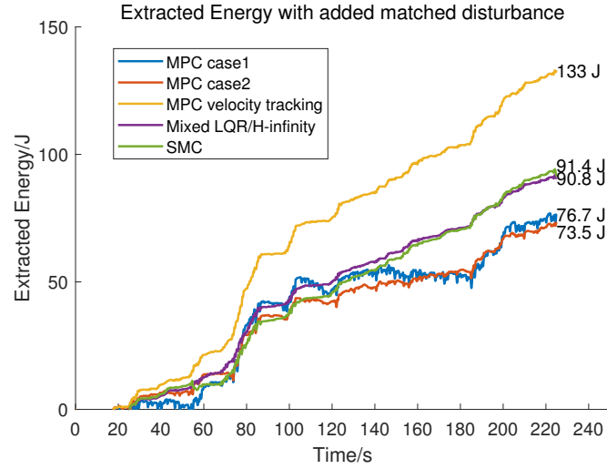
Figure 7.13: Extracted energy with added matched disturbance from all methods (Seastate 6).
