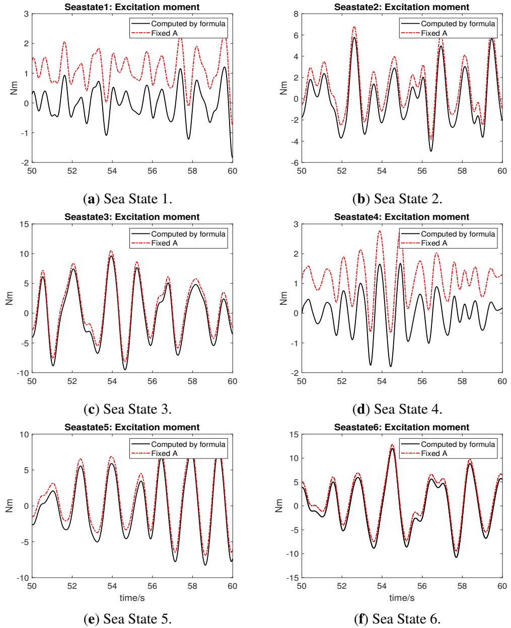
Figure 3.8: Wave excitation moment measured at fixed point A vs computed moments for six sea states.
