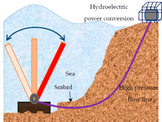
Figure 2.14: The basic illustration of oscillating wave surge WEC (Farrok et al., 2020).
