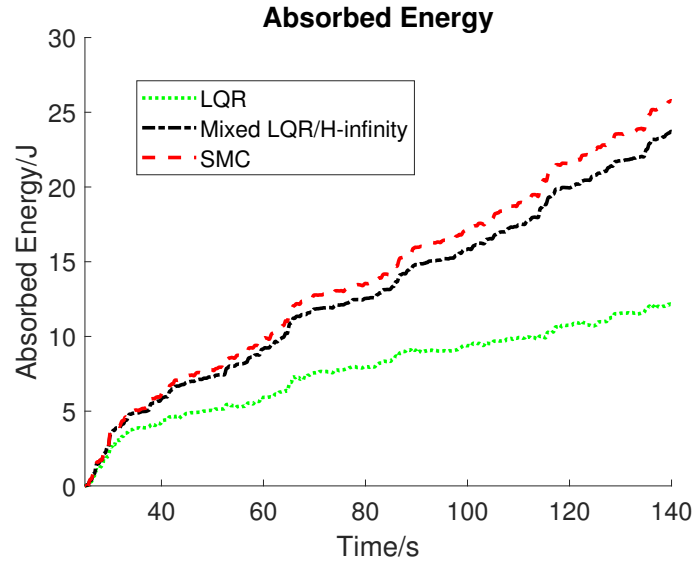
Figure 5.5: Absorbed energy from three methods (Seastate 2).
