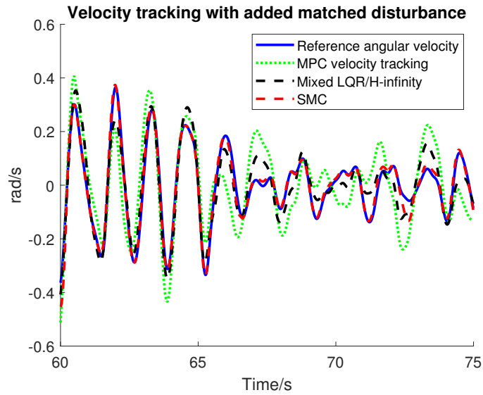
Figure 7.7: MPC velocity tracking, Model-following mixed LQR/ H_\infty control and SMC with matched disturbance (Seastate 5).
