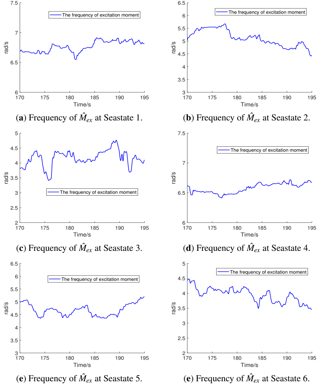
Figure 4.6: Instantaneous frequency of \hat{M}_{ex} at six sea states.
