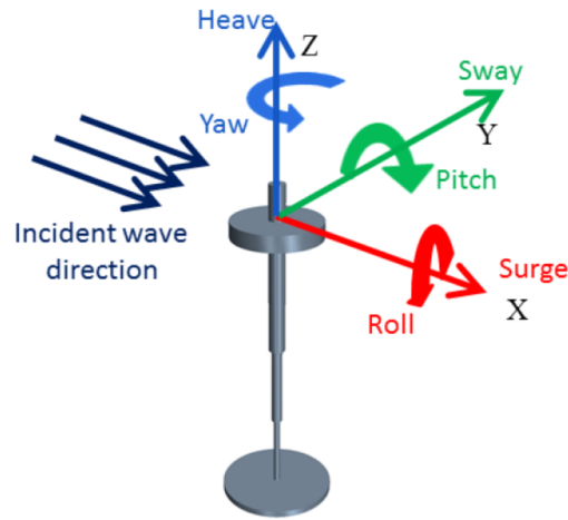
Figure 3.2: WEC-Sim Coordinate System (NREL and Sandia, 2014).
