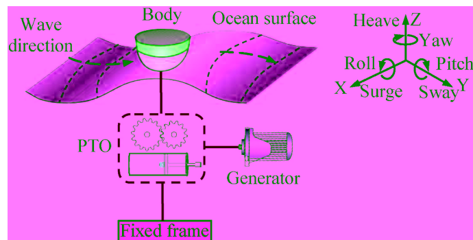
Figure 2.11: The basic idea of floating structure type WEC (Zhang et al., 2021).
