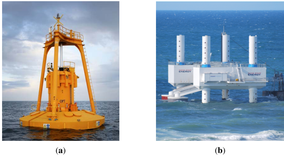
Figure 2.3: Single and array PAWEC schemes, (a) PowerBouy OPT WEC (Artal-Sevil et al., 2018), (b) Wavestar prototype WEC (Kramer et al., 2011).
