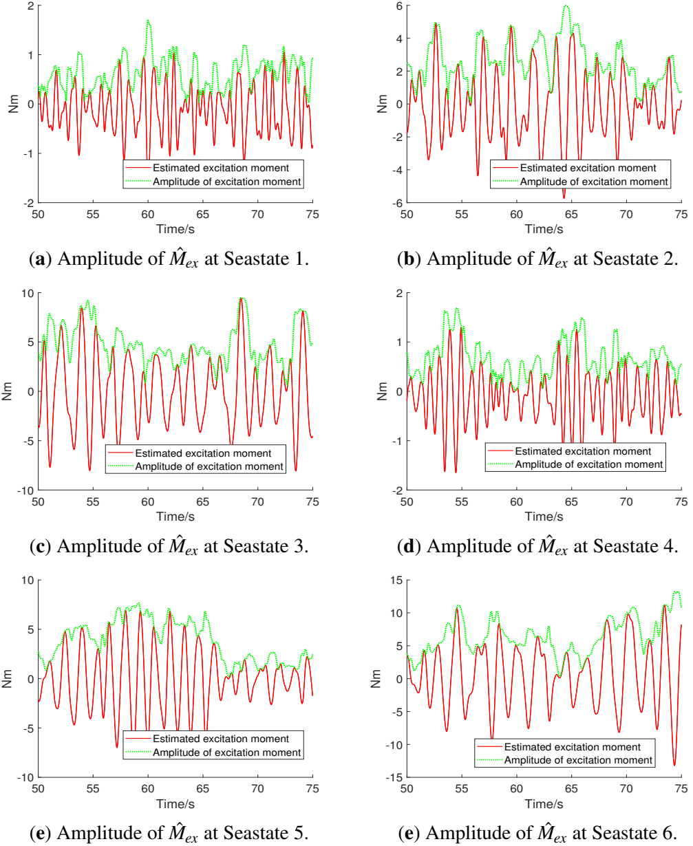
Figure 4.5: Instantaneous amplitude of \hat{M}_{ex} at six sea states.
