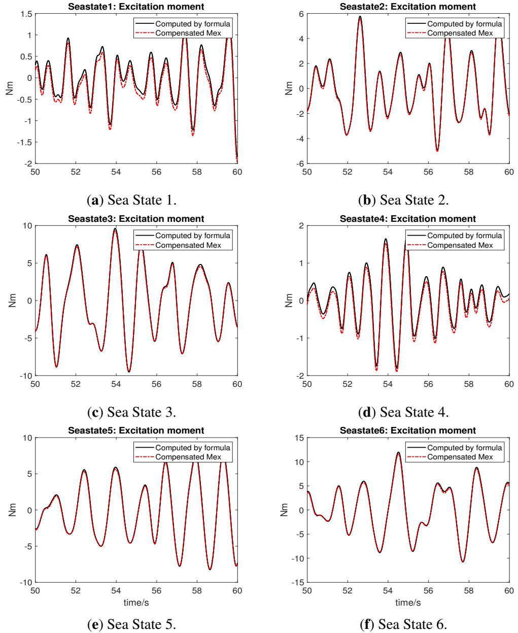
Figure 3.9: Wave excitation moment being compensated vs computed by Equation (3.25) for six sea states.
