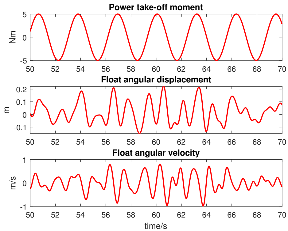
Figure 3.12: Sinusoidal signal of PTO moment test (Seastate 5).
