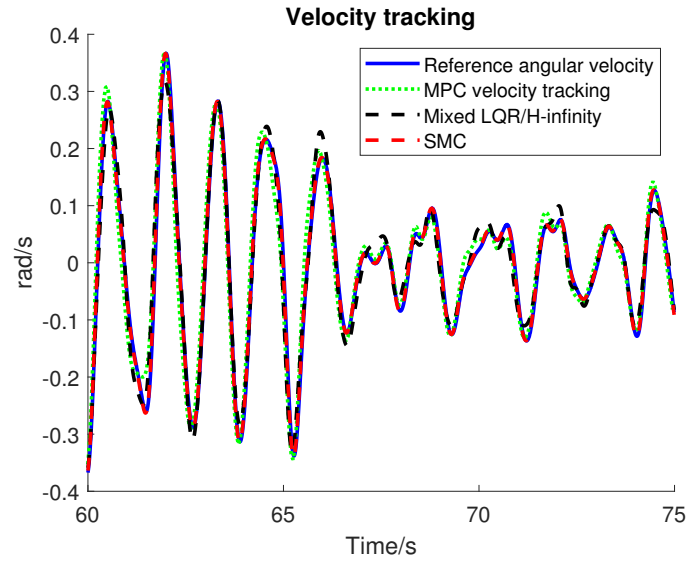
Figure 7.2: Velocity tracking results: (i) MPC, (ii) Mixed LQR/ H_\infty control and (iii) Model-following SMC approaches (Seastate 5).
