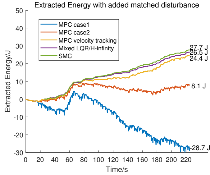
Figure 7.6: Extracted energy with added matched disturbance from all methods (Seastate 5).
