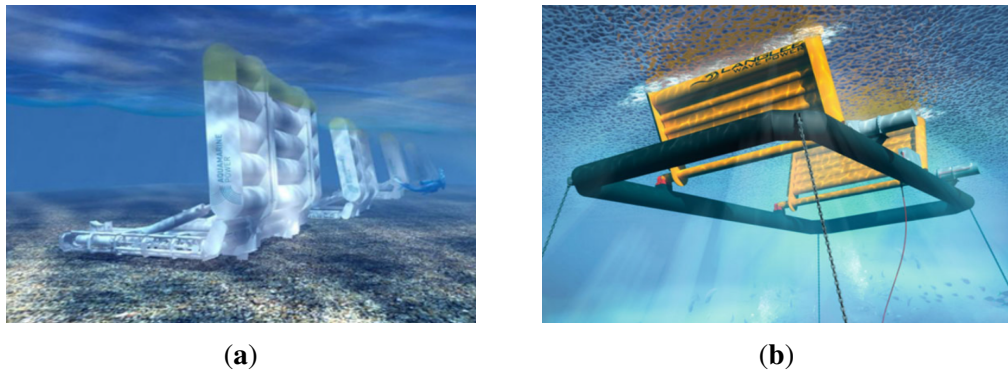
Figure 2.15: The structure of OWS WECs, (a) Oyster WEC (Oyster, 2012), (b) Langlee WEC (Pecher and Kofoed, 2017).
