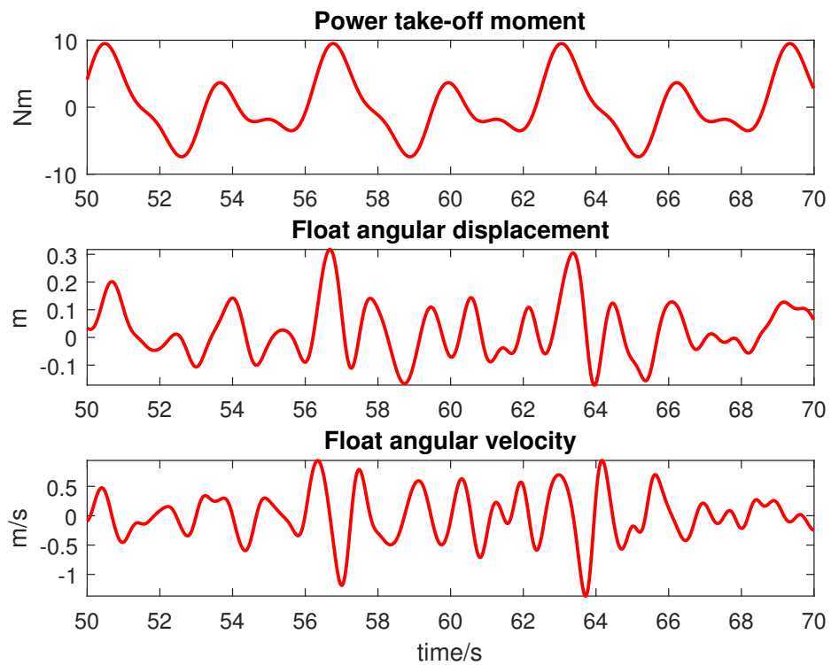
Figure 3.13: Multi-sine signal of PTO moment test (Seastate 5).
