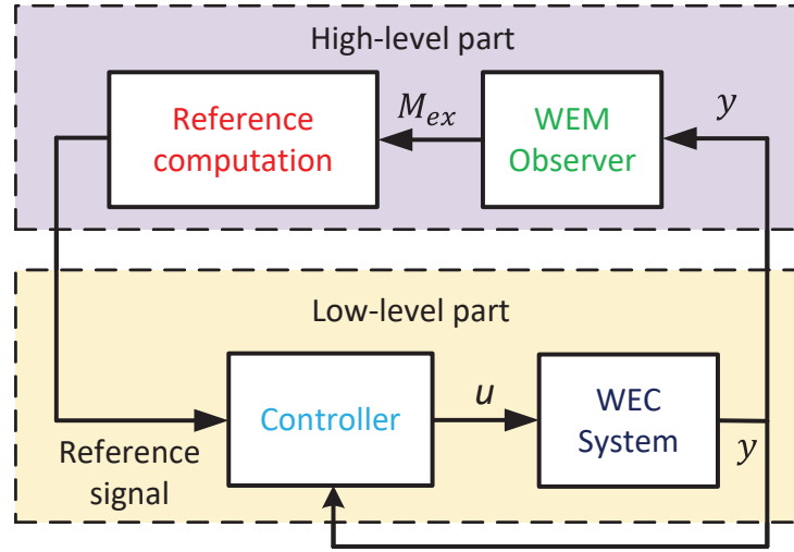
Figure 1.5: Selected hierarchical tracking structure for the whole WEC control system.
