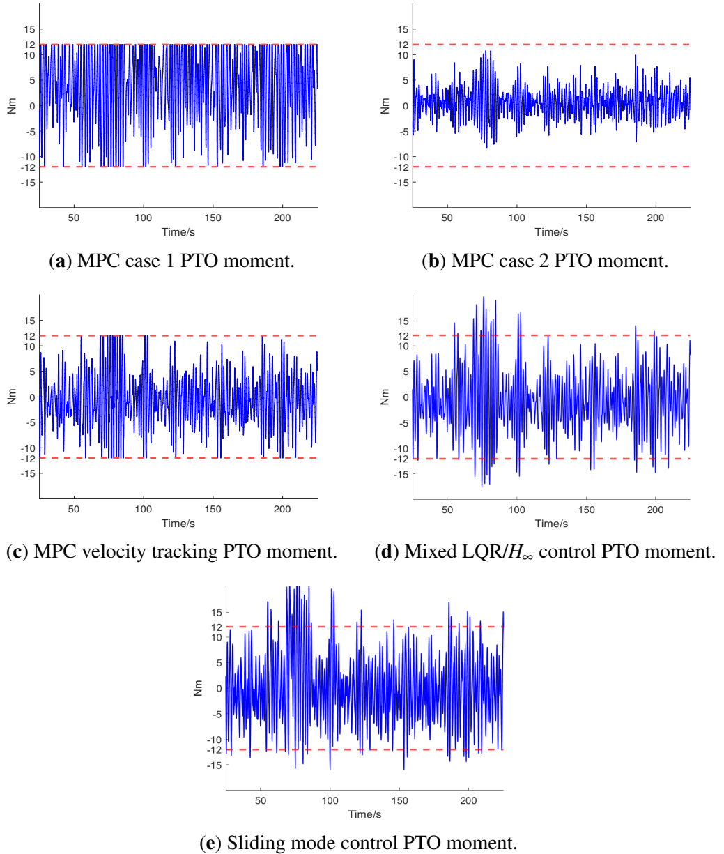
Figure 7.12: PTO moment of all methods (Seastate 6).
