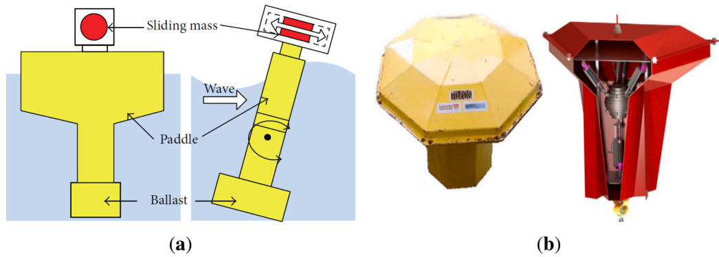
Figure 2.4: The other special designed PAWECs, (a) PS frog MK 5 WEC (Taylor et al., 2002; Faizal et al., 2014), (b) TALOS WEC (Aggidis and Taylor, 2017).
