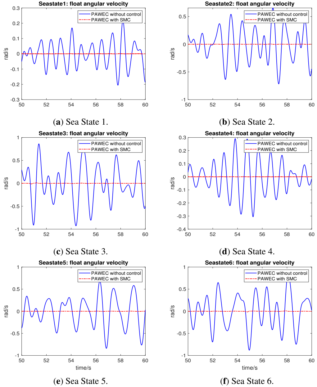
Figure 3.15: Regulation test: the float angular velocity of PAWEC without control or with SMC.
