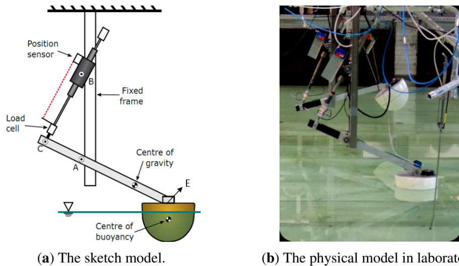
Figure 3.4: The scaled Wavestar-prototype PAWEC device (Peña-Sanchez, 2020).
