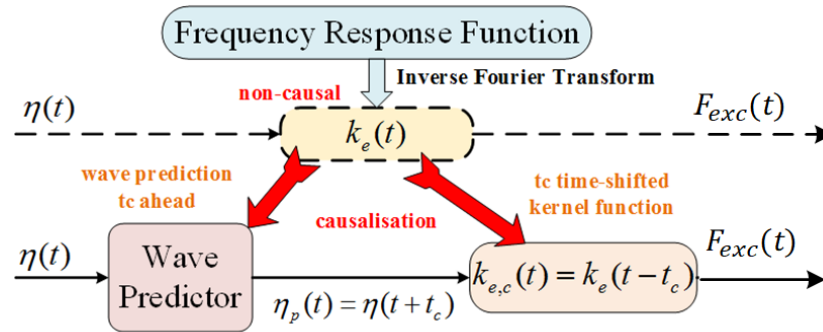
Figure 4.1: The wave elevation-based approach for WEF calculation (Guo, 2017).
