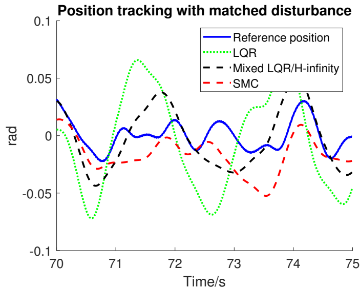
Figure 5.6: Position tracking of three methods with added matched disturbance (Seastate 2).
