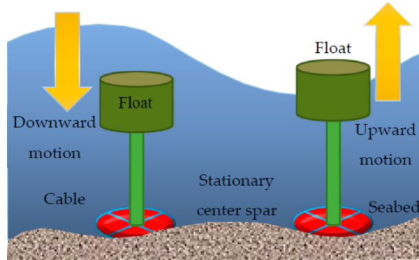
Figure 2.9: The sketch of submerged pressure differential WEC (Farrok et al., 2020).
