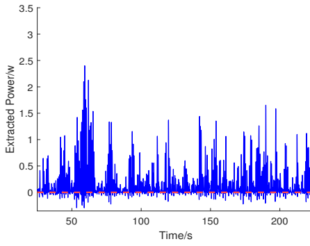
(c) MPC velocity tracking extracted power.
