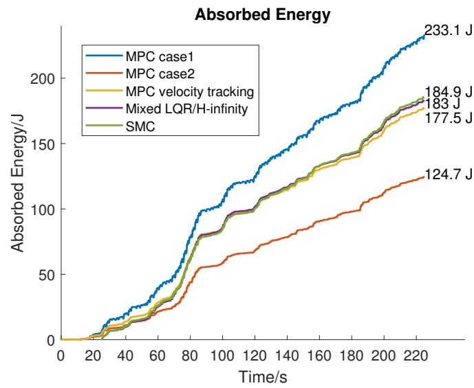
Figure 7.8: Absorbed energy from all methods (Seastate 6).
