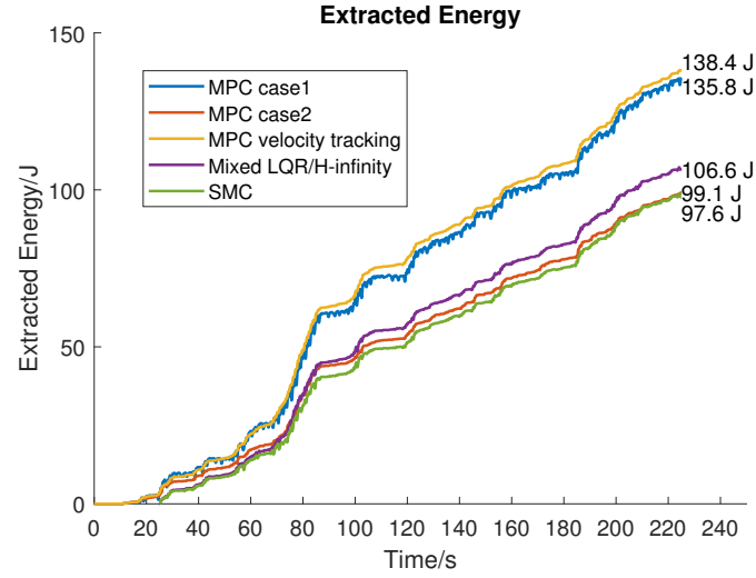
Figure 7.10: Extracted energy from all methods (Seastate 6).
