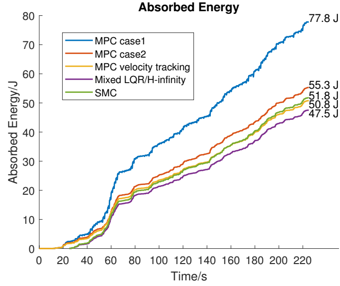
Figure 7.1: Absorbed energy from all methods (Seastate 5).
