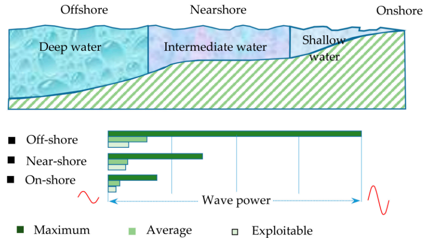
Figure 2.1: The classification by their deployment locations (Farrok et al., 2020).
