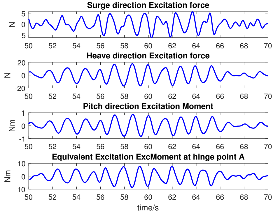
Figure 3.11: The components of wave excitation force in surge, heave, pitch directions and equivalent excitation moment at hinge point A (Seastate 5).
