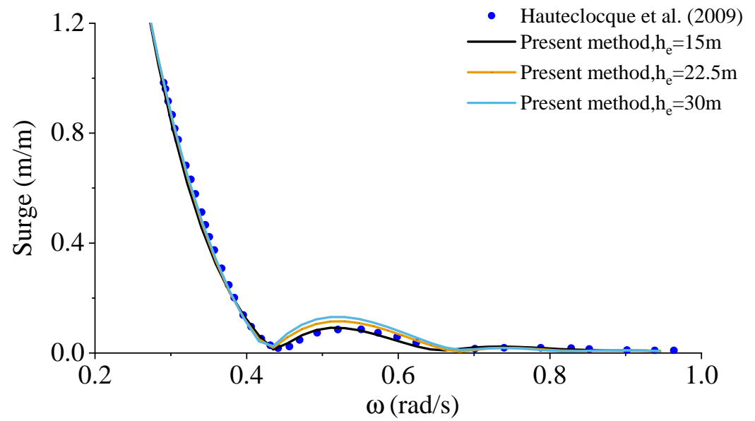
Figure 4. Comparison of surge RAOs between present method with h_e = 15, 22.5 and 30 m and solutions from Hauteclocque et al. [23] for incident wave with \theta = 0 deg for an LNG ship over a sloping seabed.
