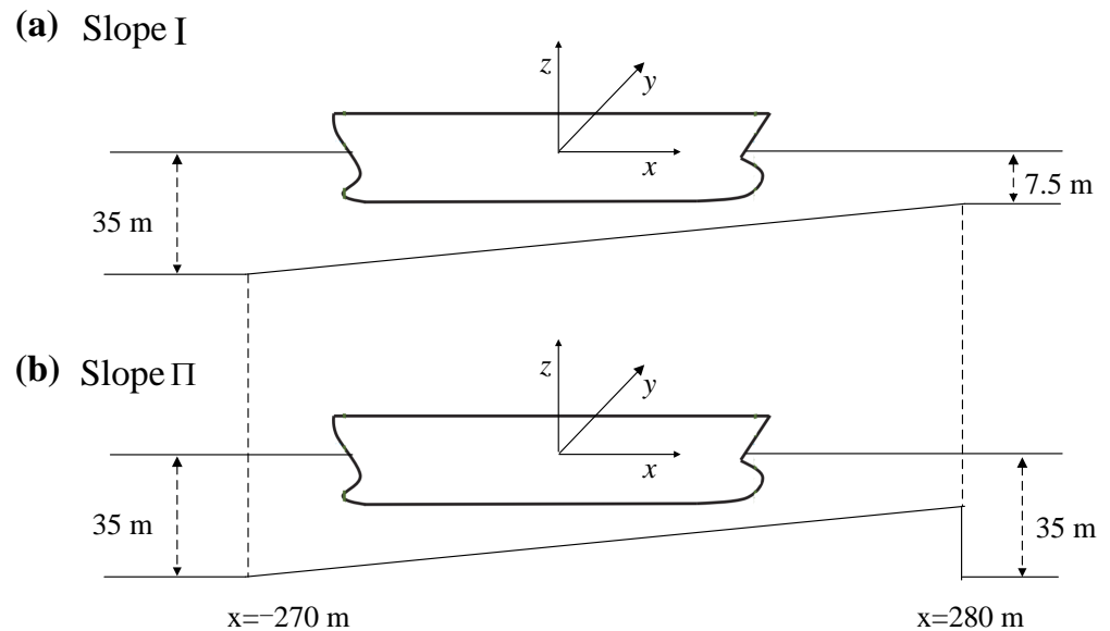
Figure 8. Configurations of the sloped bottom used to demonstrate a comparison with the experimental results from Buchner [21].
