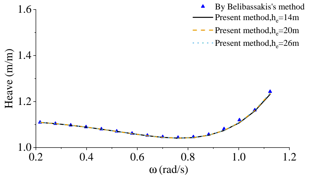
Figure 17. Comparison of heave RAOs between present method with h_e = 14, 20 and 26 m and numerical results using Belibassakis [24]’s method for an oblique wave with \theta = 30 deg for a hemisphere over an undulating seabed.
