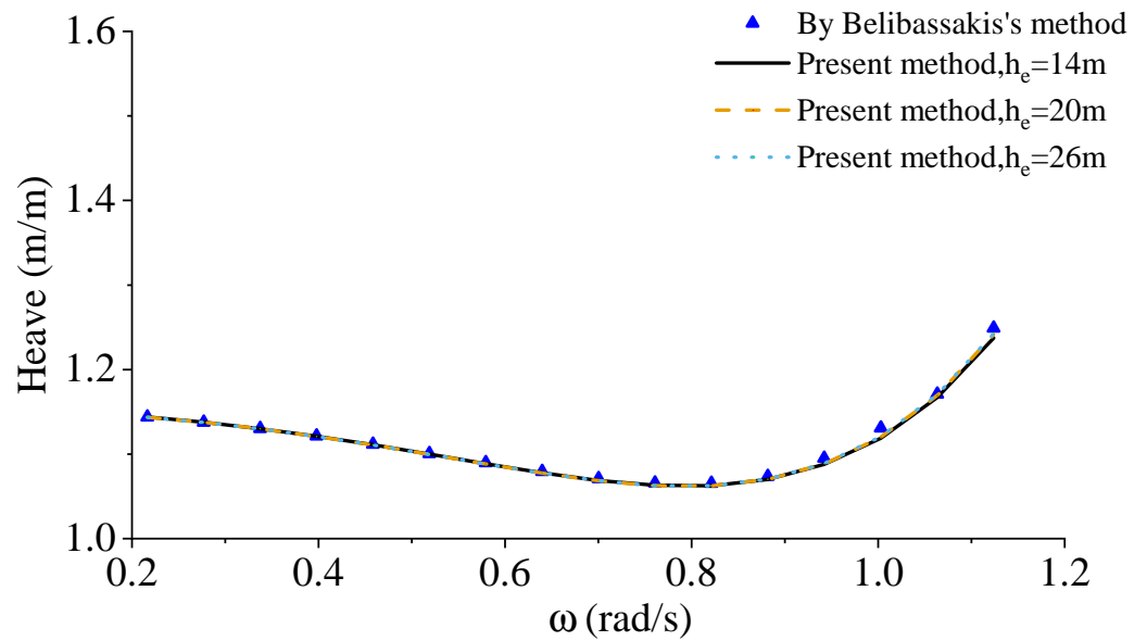
Figure 14. Comparison of heave RAOs between present method with h_e = 14, 20 and 26 m and numerical results using Belibassakis [24]’s method for an incident wave with \theta = 0 deg for a floating hemisphere over a sloping bottom.
