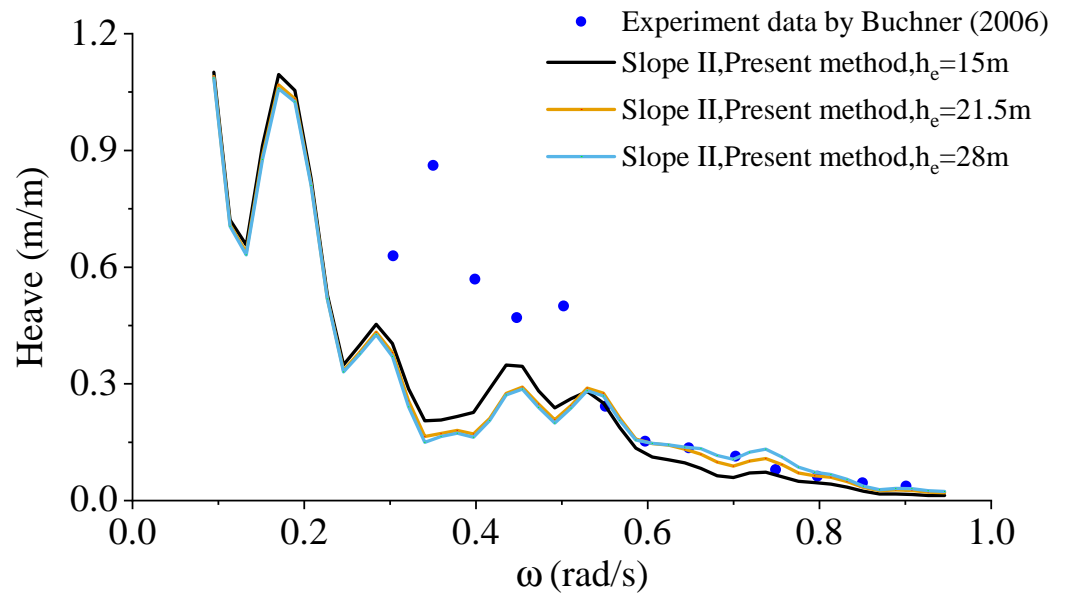
Figure 12. Comparison of heave RAOs between the present method with h_e = 15, 21.5 and 28 m over Slope II and experimental results from Buchner [21] for an incident wave with \theta = 0 deg for an LNG ship.
