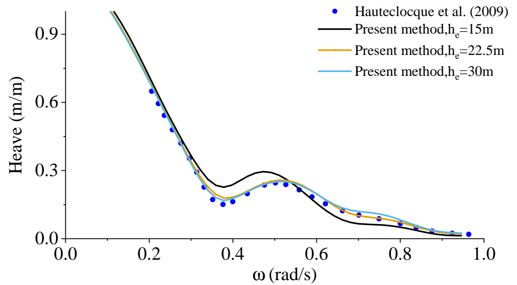
Figure 7. Comparison of heave RAOs between present method with h_e = 15, 22.5 and 30 m and solutions from Hauteclocque et al. [23] for an oblique wave with \theta = 15 deg for an LNG ship over a sloping seabed.
