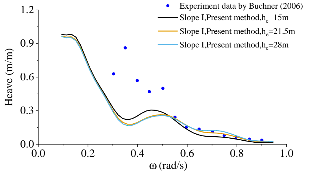
Figure 10. Comparison of heave RAOs between present method with h_e = 15, 21.5 and 28 m over Slope I and experimental results from Buchner [21] for an incident wave with \theta = 0 deg for an LNG ship.
