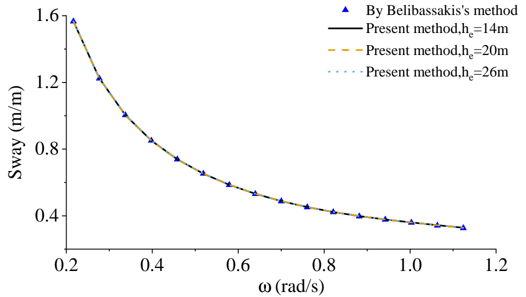
Figure 16. Comparison of sway RAOs between present method with h_e = 14, 20 and 26 m and numerical results using Belibassakis [24]’s method for an oblique wave with \theta = 30 deg for a hemisphere over an undulating seabed.
