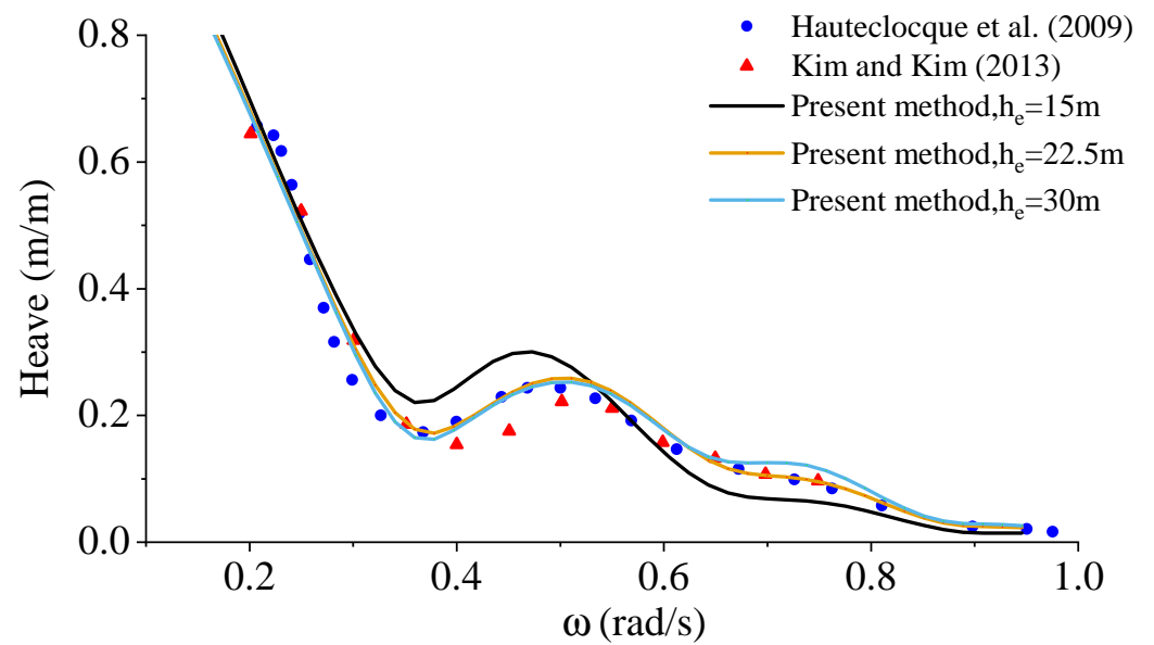
Figure 5. Comparison of heave RAOs between present method with h_e = 15, 22.5 and 30 m and numerical results from Hauteclocque et al. [23], Kim and Kim [28] for incident wave with \theta = 0 deg for an LNG ship over a sloping seabed.
