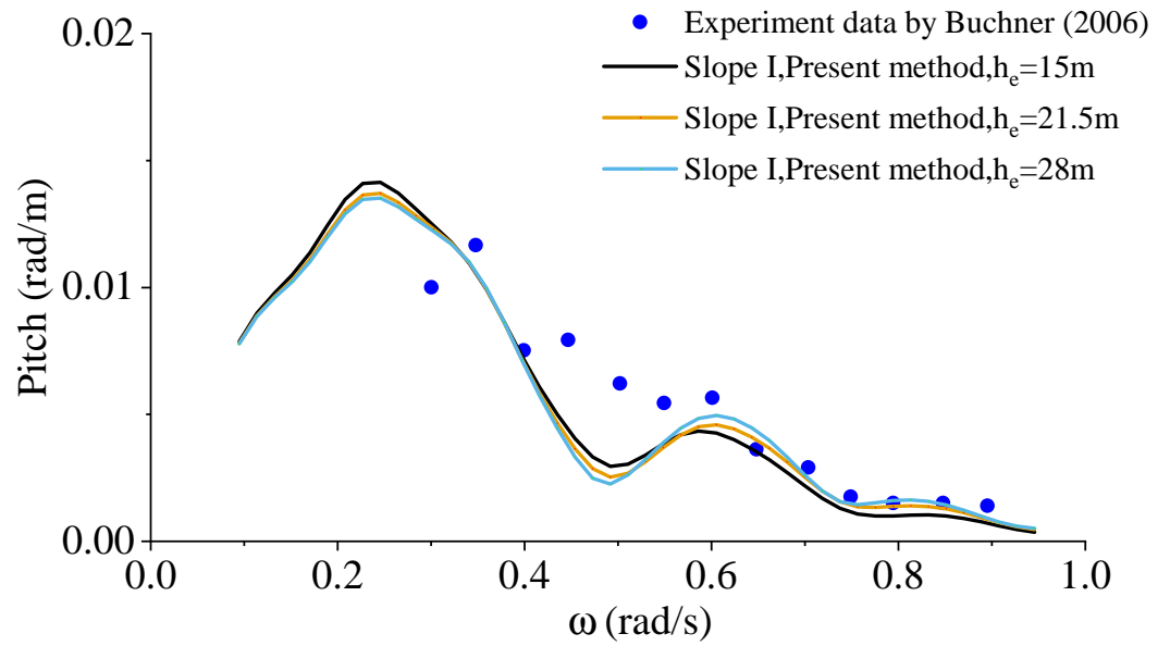
Figure 9. Comparison of pitch RAOs between present method with h_e = 15, 21.5 and 28 m over Slope I and experimental results from Buchner [21] for an incident wave with \theta = 0 deg for an LNG ship.
