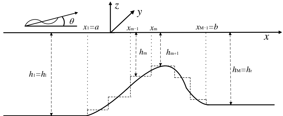
Figure 3. Approximation of the sloping seabed by shelves.
