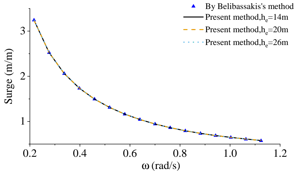
Figure 15. Comparison of surge RAOs between present method with h_e = 14, 20 and 26 m and numerical results using Belibassakis [24]’s method for an oblique wave with \theta = 30 deg for a hemisphere over an undulating seabed.
