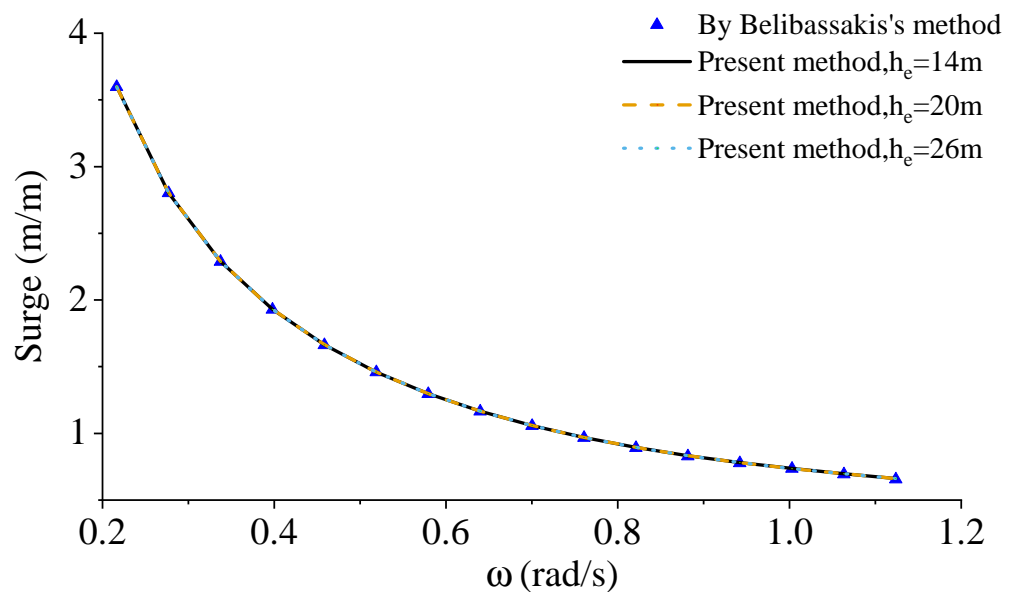
Figure 13. Comparison of surge RAOs between present method with h_e = 14, 20 and 26 m and numerical results using Belibassakis [24]’s method for incident wave with \theta = 0 deg for a hemisphere over an undulating seabed.
