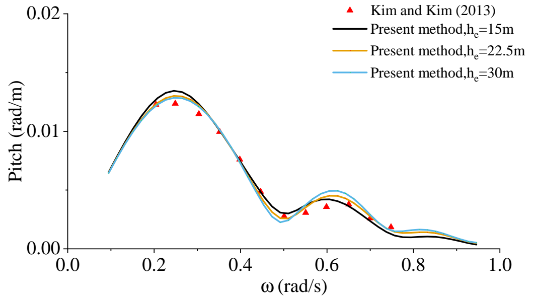
Figure 6. Comparison of pitch RAOs between present method with h_e = 15, 22.5 and 30 m and solutions from Kim and Kim [28] for incident wave with \theta = 0 deg for an LNG ship over a sloping seabed.
