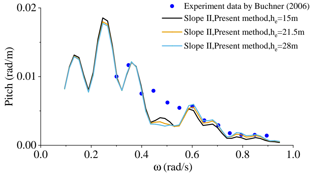
Figure 11. Comparison of pitch RAOs between present method with h_e = 15, 21.5 and 28 m over Slope II and experimental results from Buchner [21] for an incident wave with \theta = 0 deg for an LNG ship.
