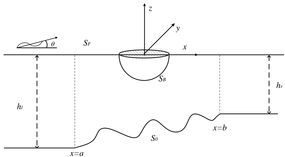
Figure 2. Wave–body hydrodynamic interaction over a sloping bottom.
