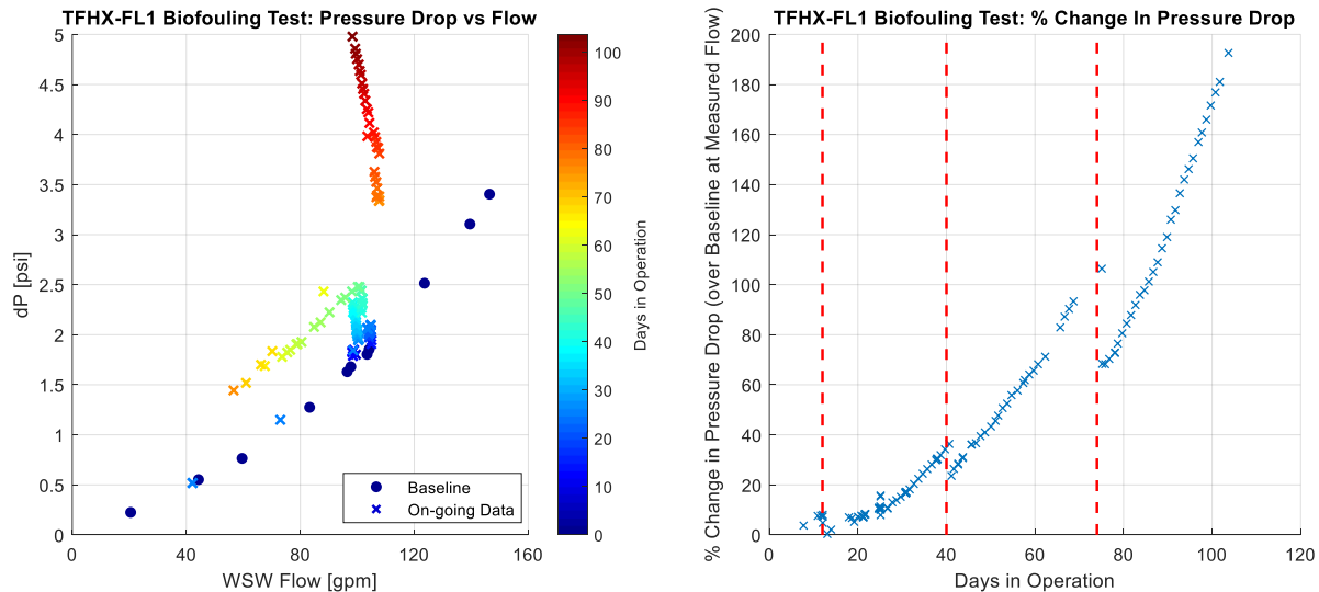
Figure 49. TFHX-FL1 biofouling test change in pressure drop over time.
