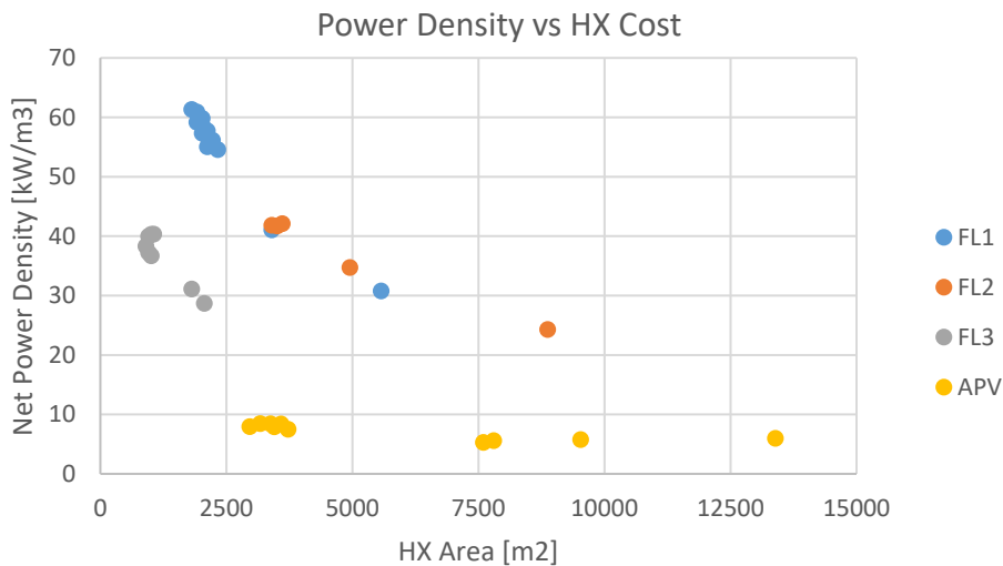
Figure 46. Net power density versus heat exchanger area for a fixed cold water pipe size and seawater flow rates.
