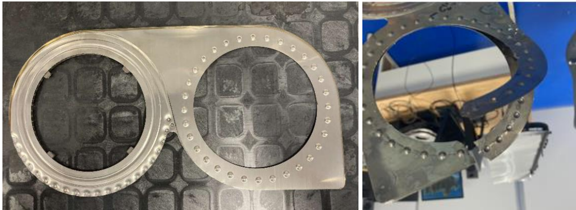
Figure 17. (left) FL3 spacers for condenser and evaporator testing. (right) The external fluid opening of several spacers was found to have rotated out of position and a few were also torn after testing.
