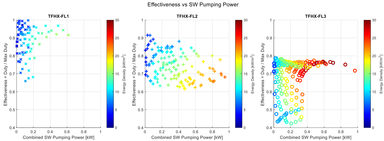
Figure 41. Effectiveness depends on duty and seawater pumping power.
