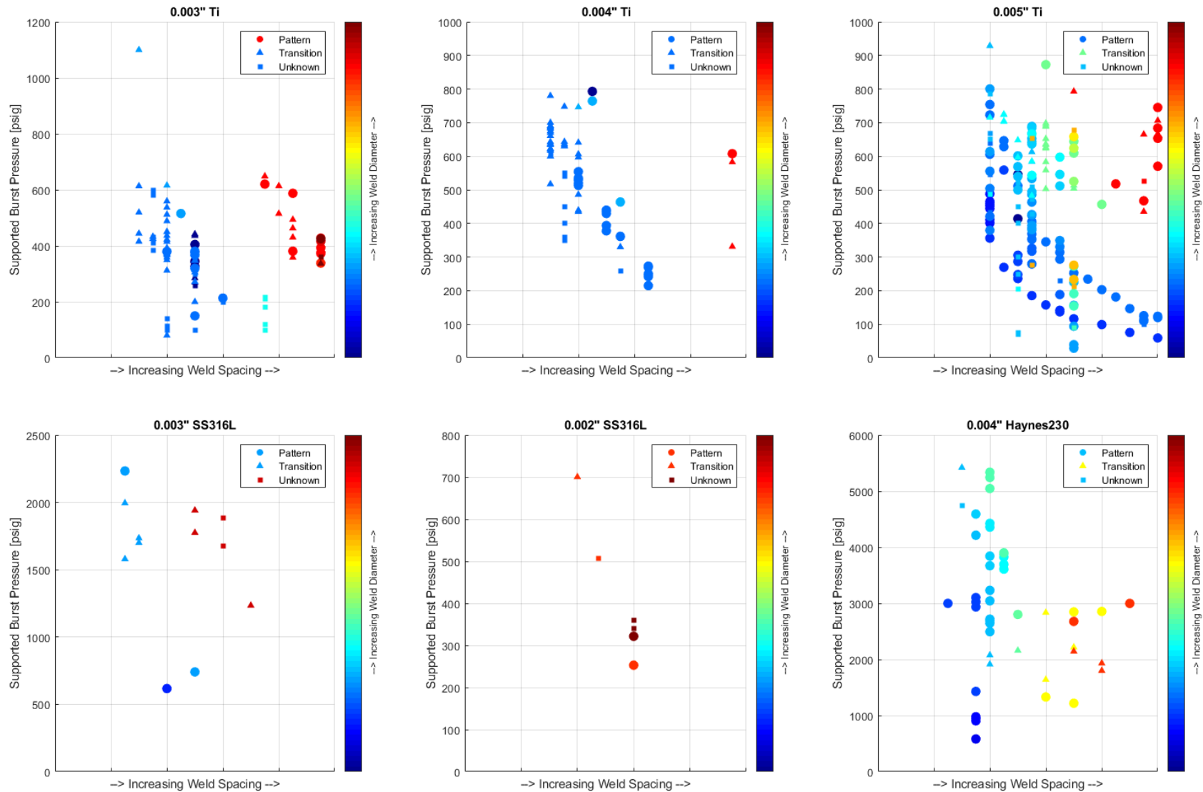
Figure 3. Supported burst pressure dependence on weld spacing, weld diameter, material, and foil thickness.
