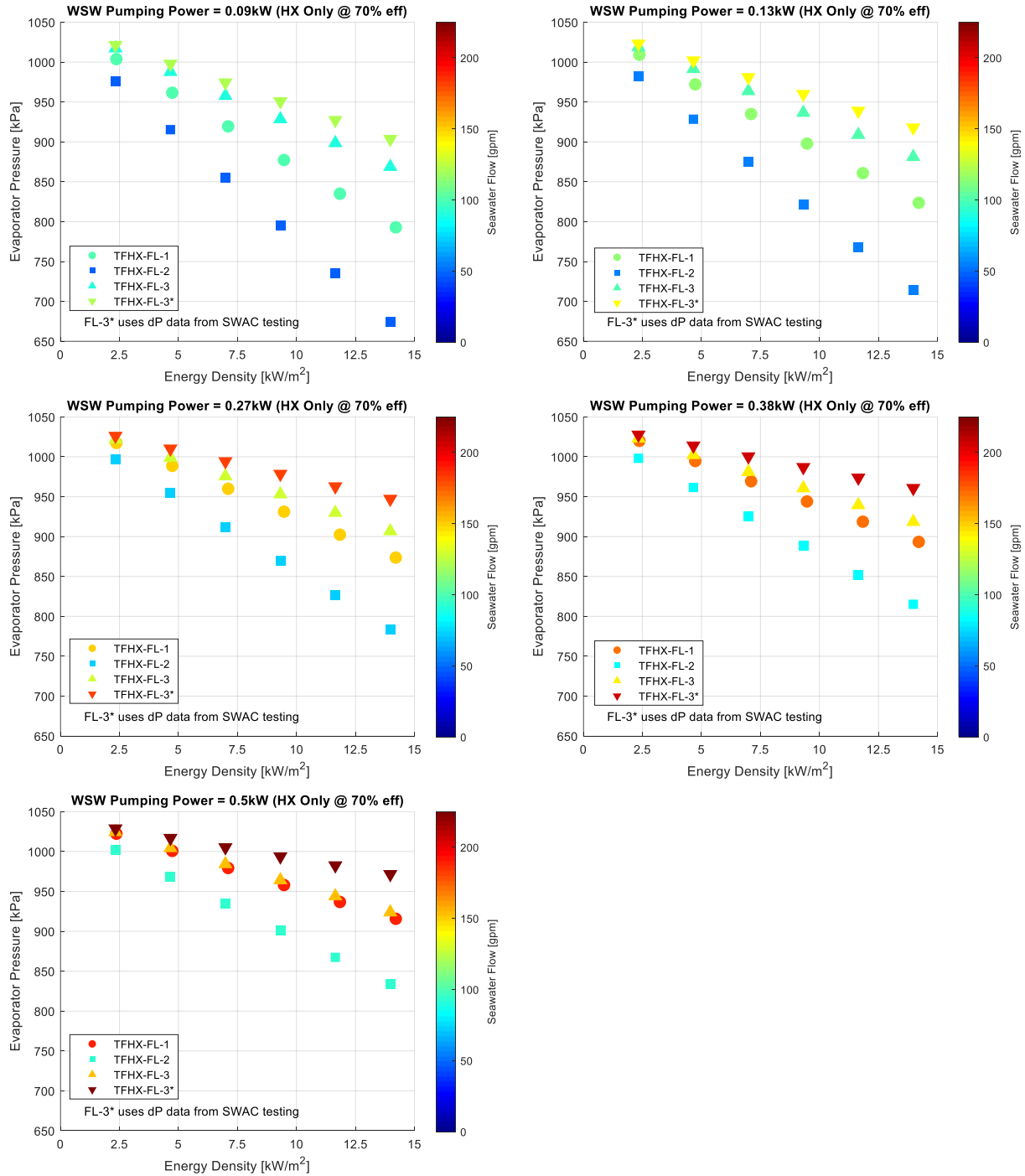
Figure 40. Comparison of evaporator operating pressure versus energy density for warm seawater temperature = 26.5^\circ\text{C} at different seawater pumping powers (through the heat exchanger only).
