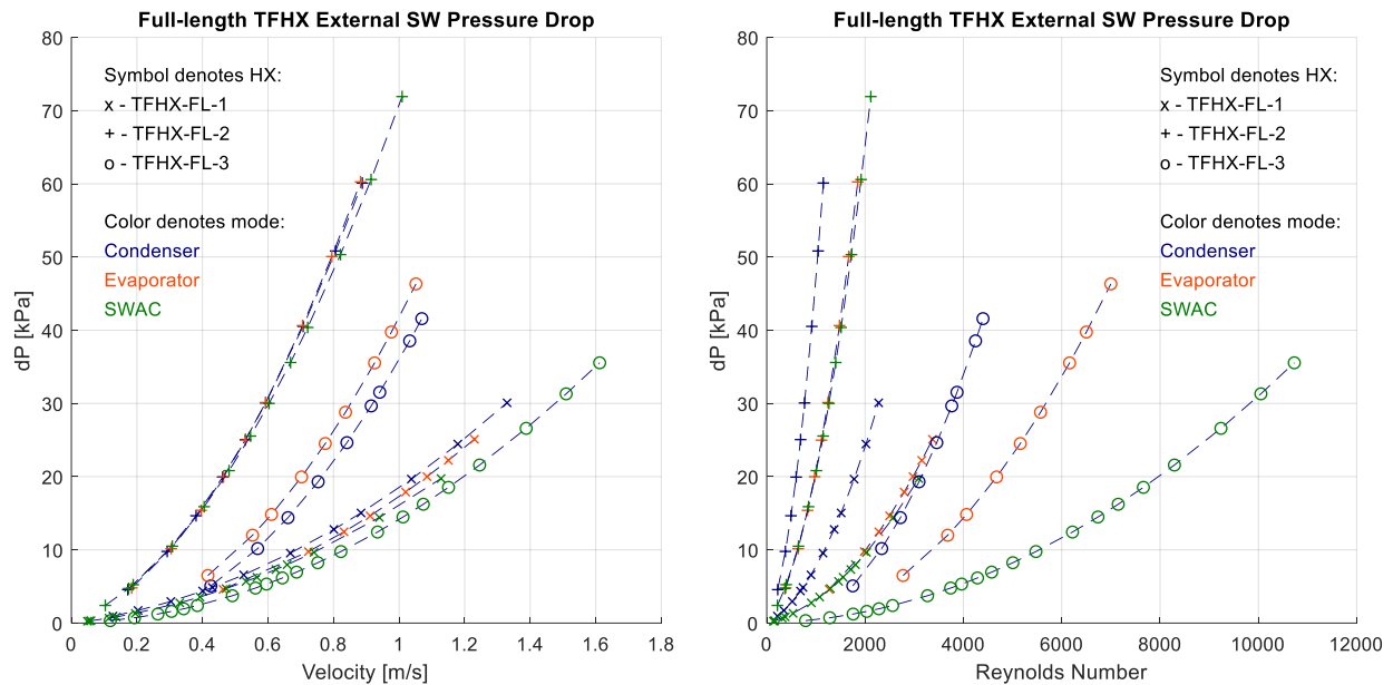
Figure 19. Seawater pressure drop for all three TFHX units. The FL3 SWAC data set is taken after the torn external spacers were removed.
