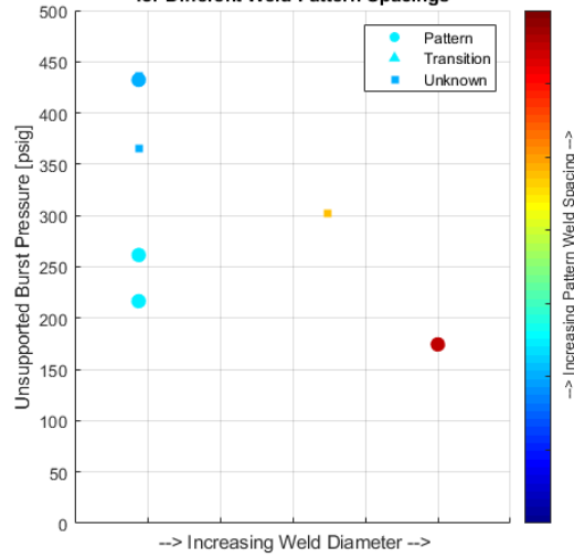
0.005" Ti Unsupported Burst Pressure vs Weld Diameter for Different Weld Pattern Spacings
