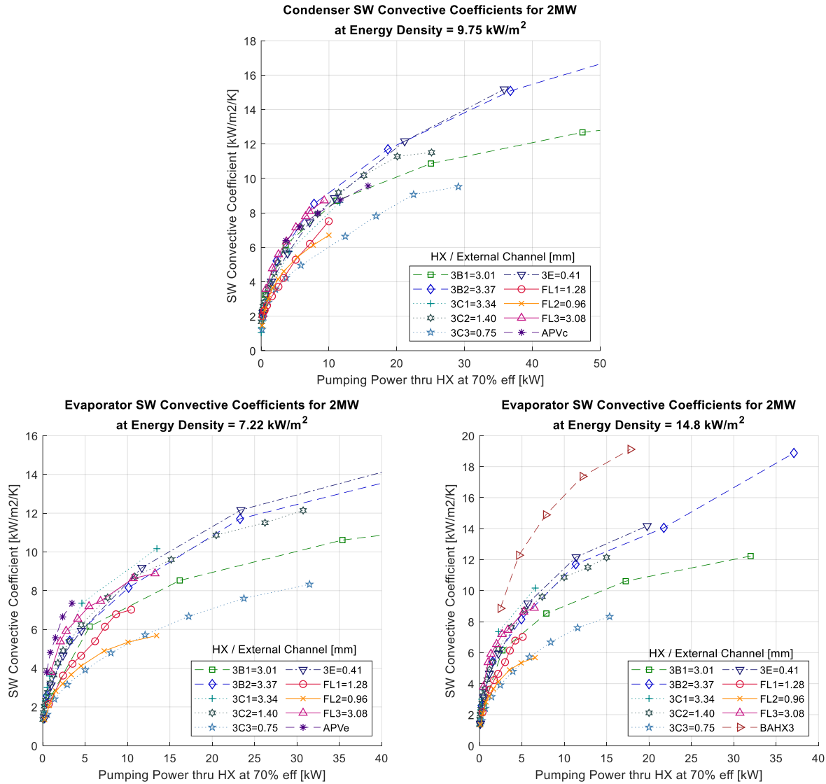
Figure 36. Comparison of external seawater convective coefficients versus pumping power through the heat exchanger. TFHXs are scaled up to a 2MW unit at the same energy density as previously tested APV or BAHX heat exchangers.
