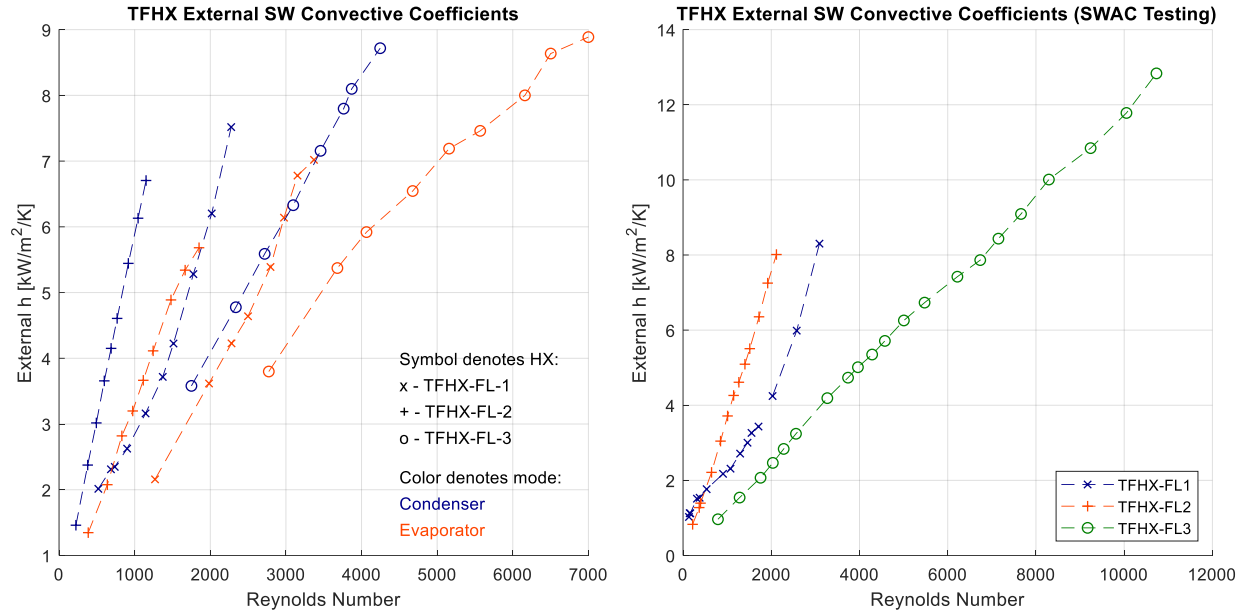
Figure 35. At the same Reynolds number, the smaller channel in FL2 had higher convective coefficients.
