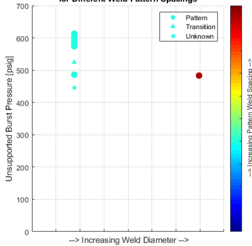
0.004" Ti Unsupported Burst Pressure vs Weld Diameter for Different Weld Pattern Spacings
