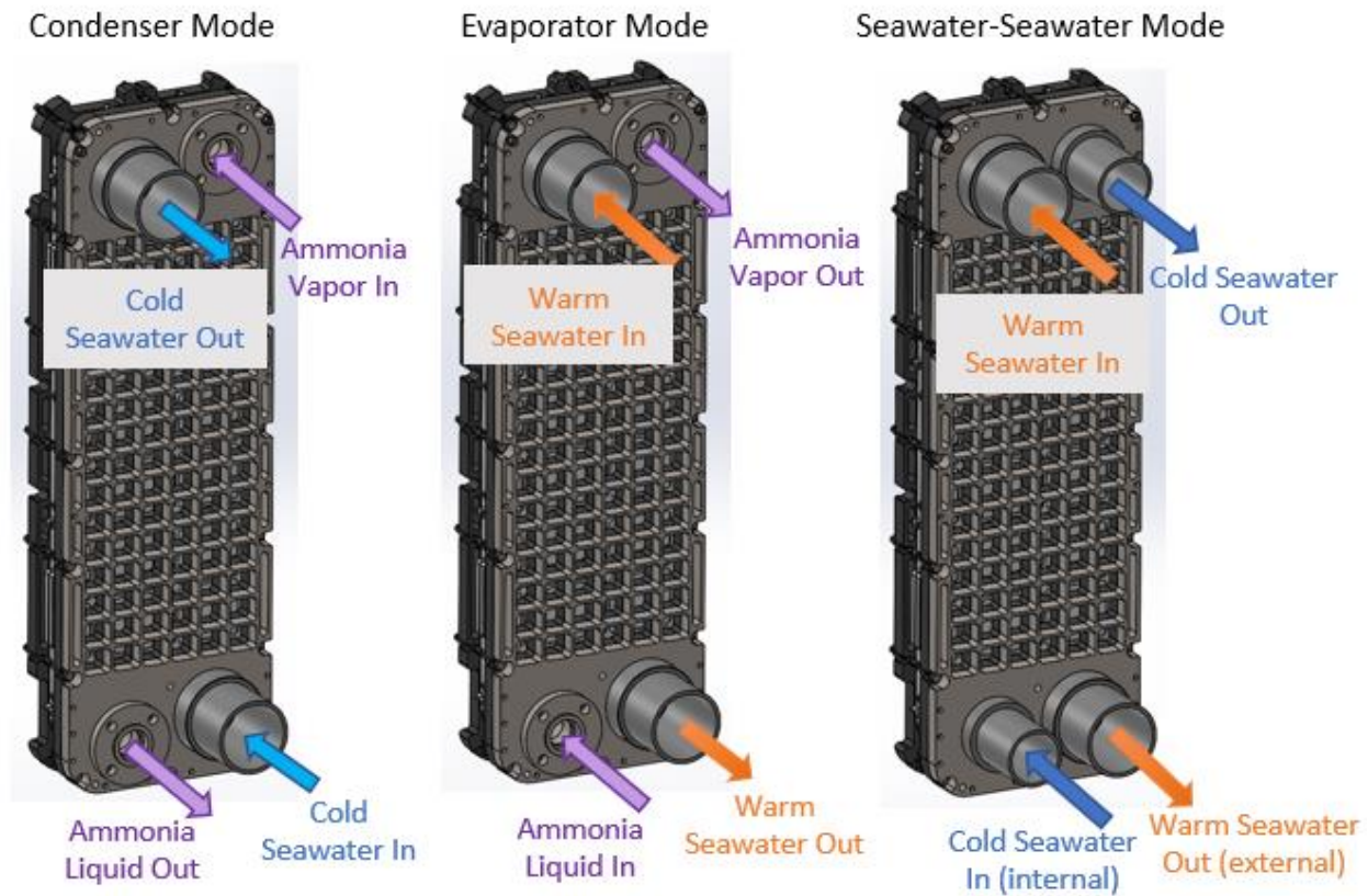
Figure 16. Full-length TFHX module configured for counterflow condenser, evaporator, and seawater-seawater (SWAC) testing.
