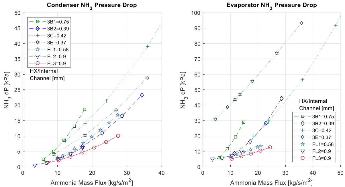
Figure 25. Comparison of ammonia-side pressure drop to previous TFHX units.
