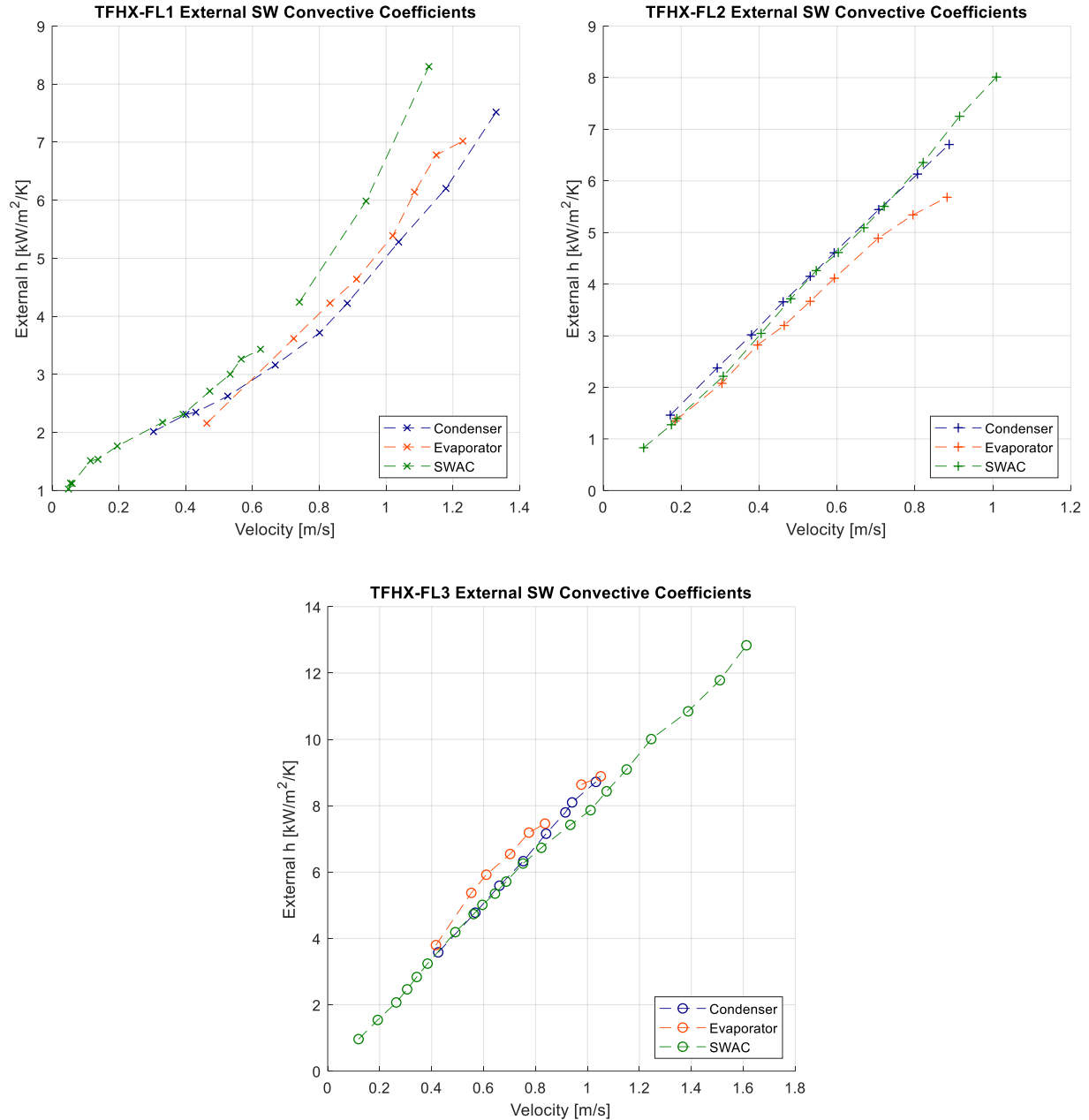
Figure 34. Seawater-side convective coefficients calculated individually for each configuration showed strong agreement.
