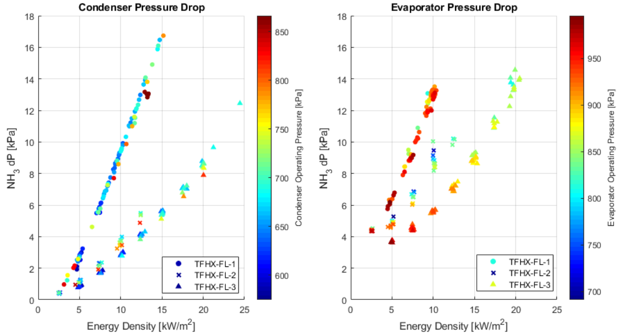
Figure 24. Ammonia-side pressure drop in condenser and evaporator mode.
