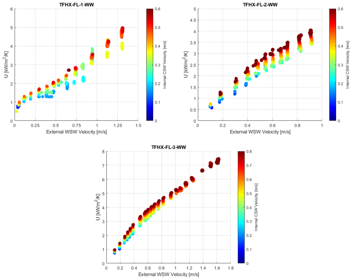
Figure 30. SWAC testing U -values.
