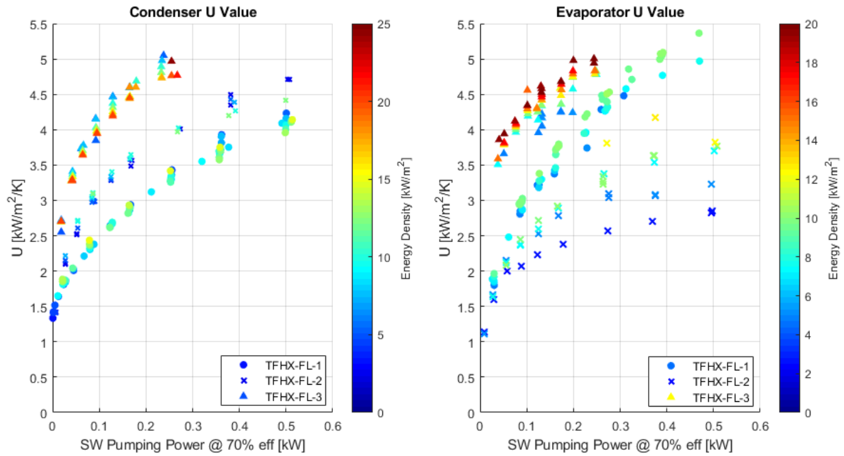
Figure 28. U-value versus seawater pumping power for different energy densities.
