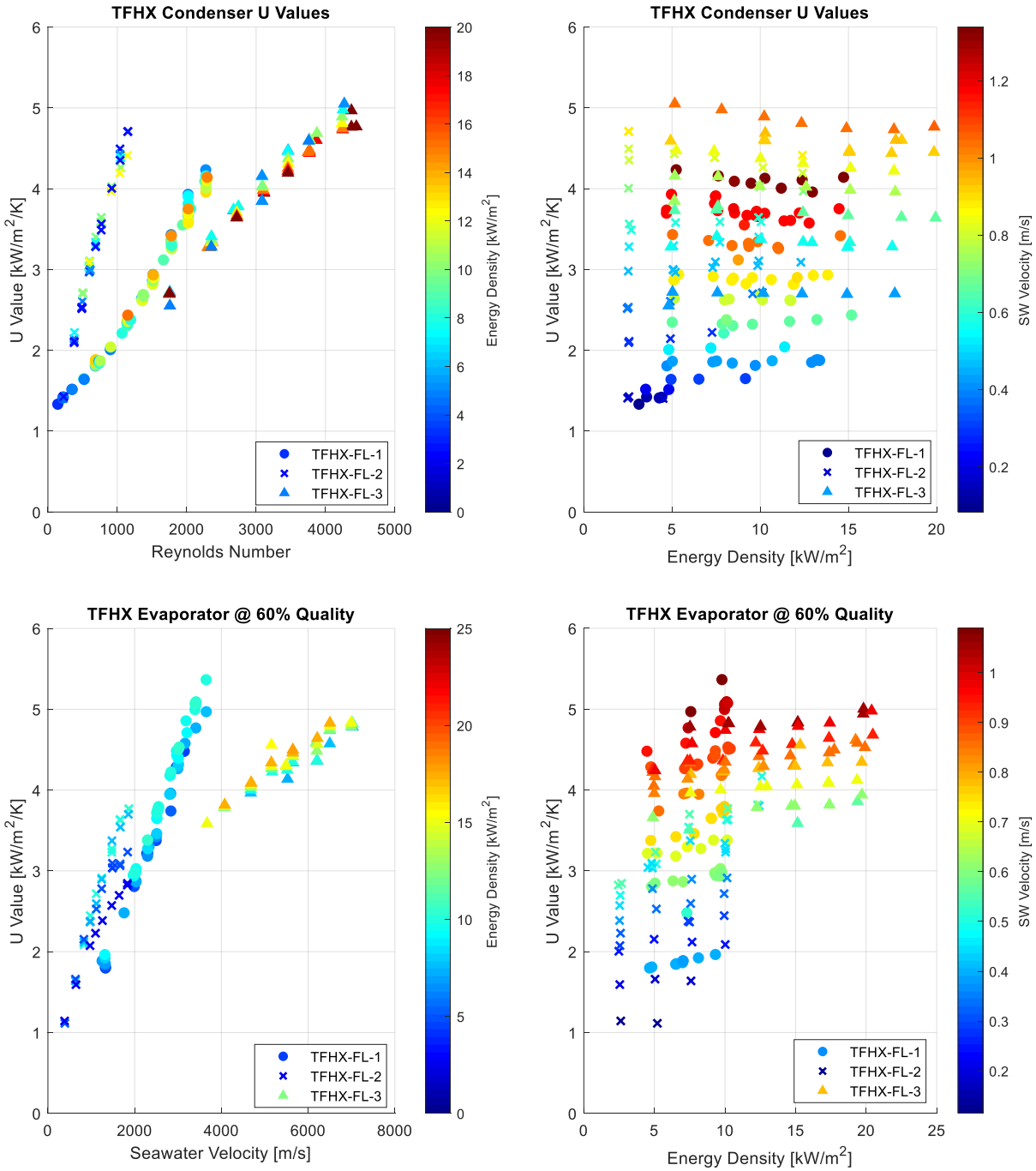
Figure 26. Effect of seawater velocity and energy density on U-value for TFHX units in condenser and evaporator mode.
