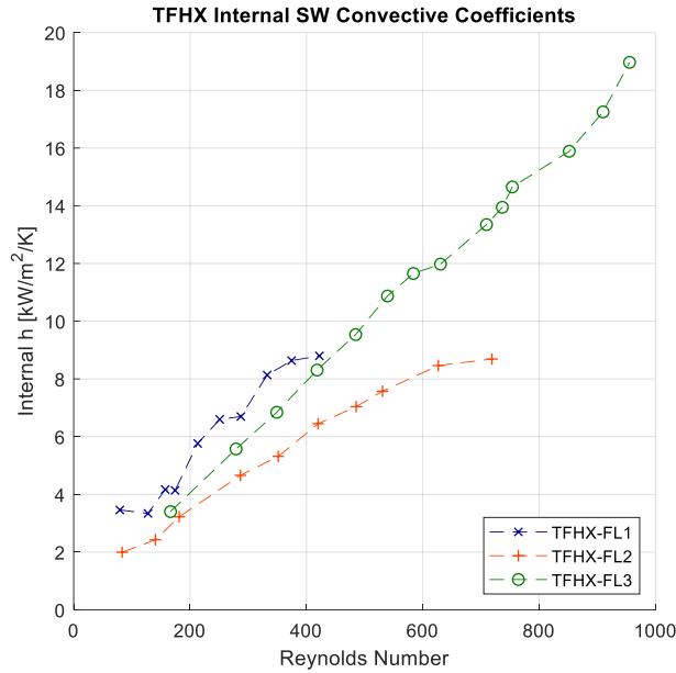
Figure 37. Internal seawater convective coefficients from SWAC testing.
