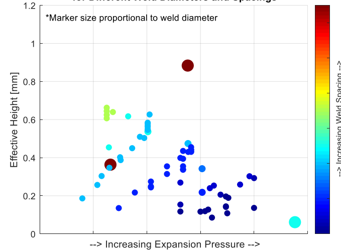
0.005" Ti Effective Channel Size vs Expansion Pressure for Different Weld Diameters and Spacings
