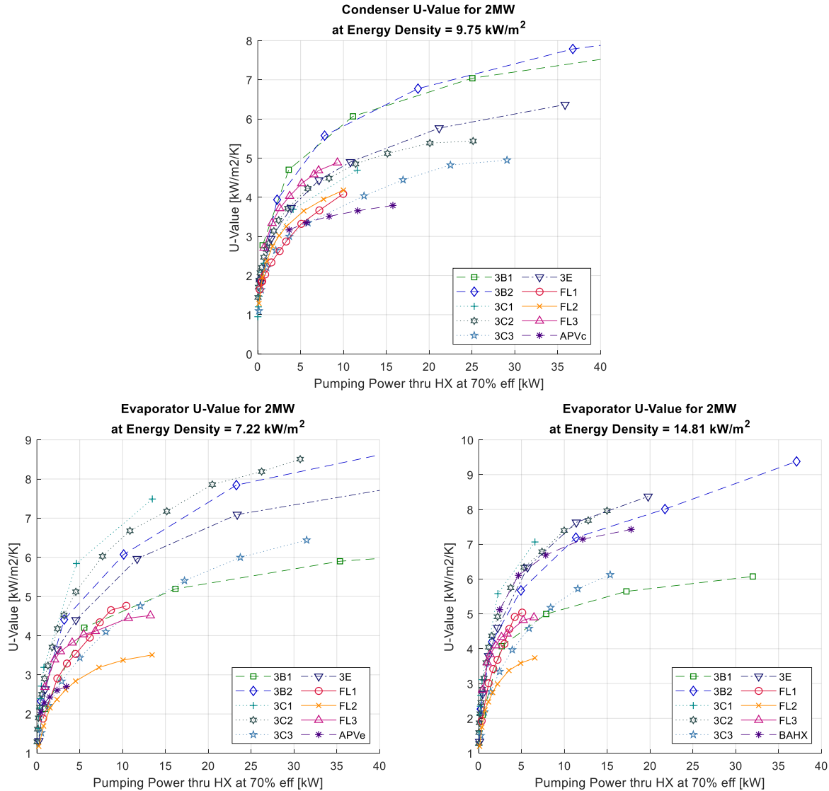
Figure 29. Comparison of U-value vs pumping power with TFHX units scaled to 2MW duty at the same energy density as other 2MW heat exchangers.
