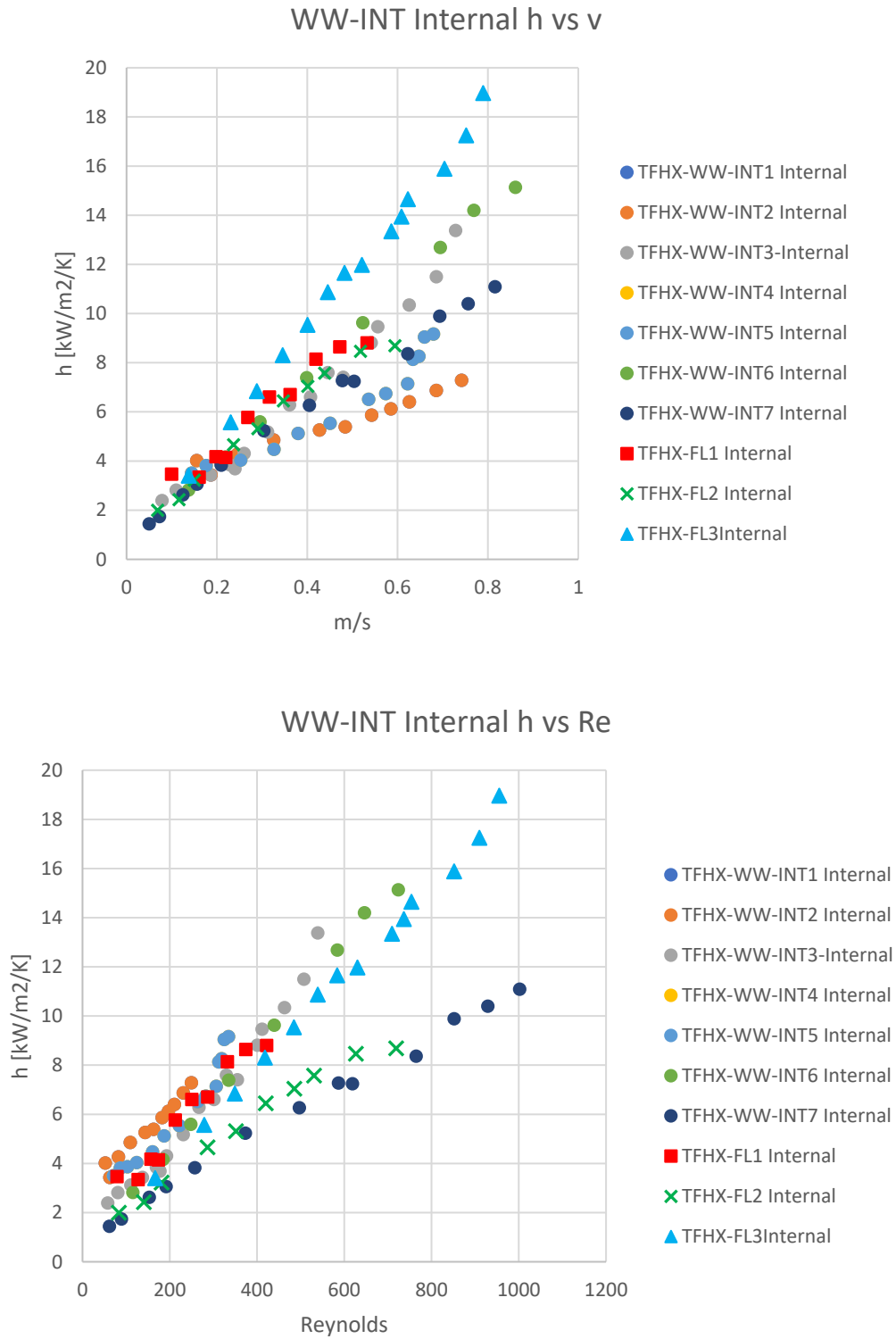
Figure 38. Internal convective coefficient comparison with previous SWAC testing results.
