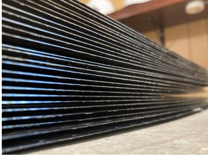
Figure 14. Cut edges on the commissioned cutting station are relatively smooth and do not require a post-cut manual deburring step.
