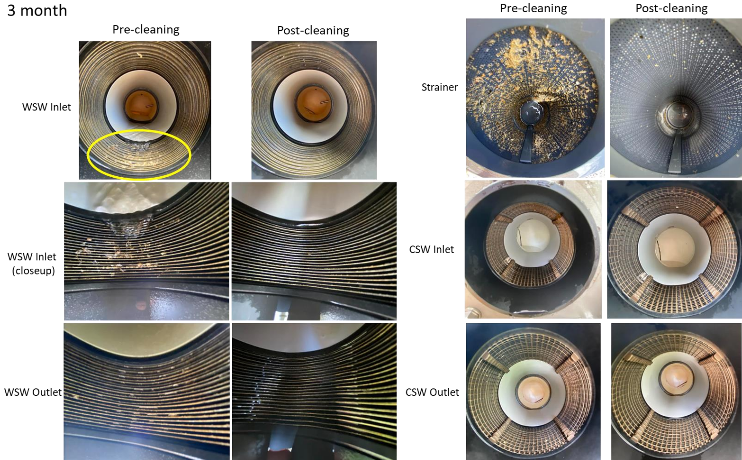
Figure 51. Pre- and post-cleaning images after 1, 2, and 3 months of testing.
