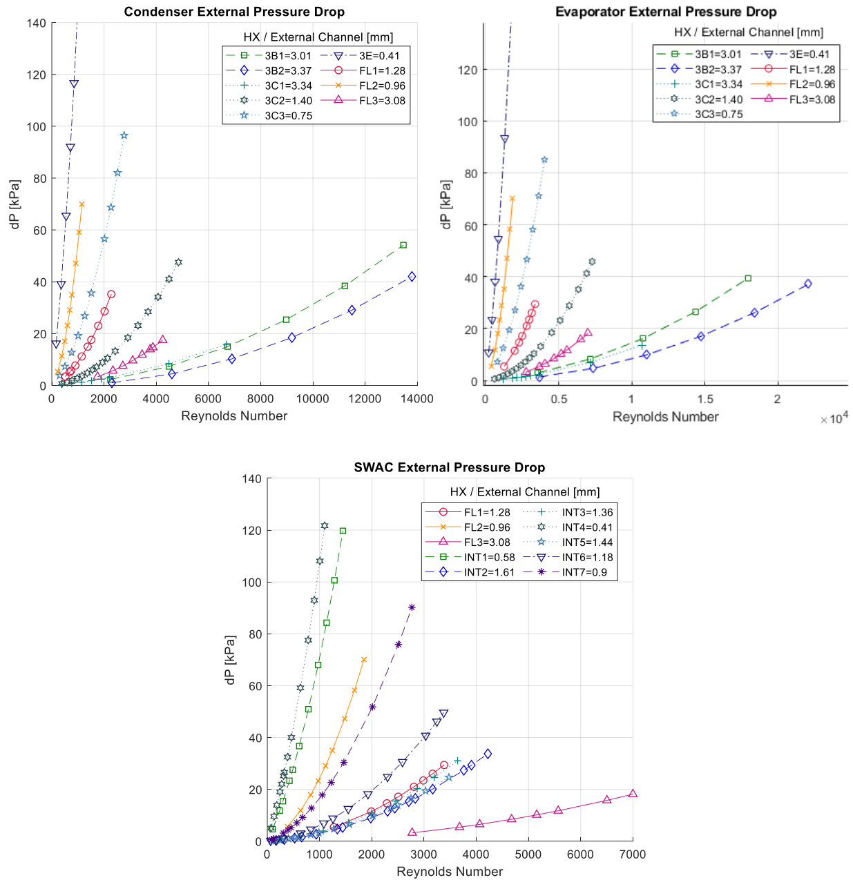
Figure 22. External seawater pressure drop comparison to previous TFHX designs.
