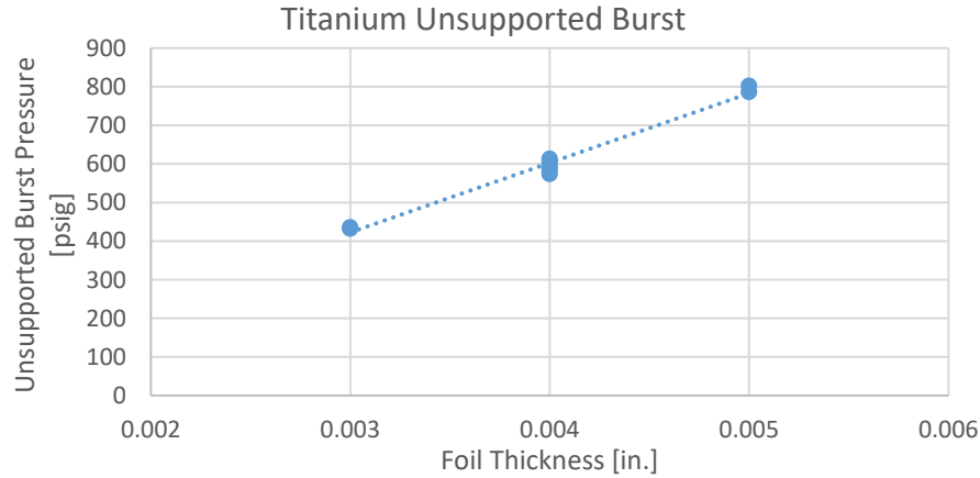
Figure 5. Unsupported burst pressure of 0.003", 0.004", and 0.005" with the same weld pattern design.
