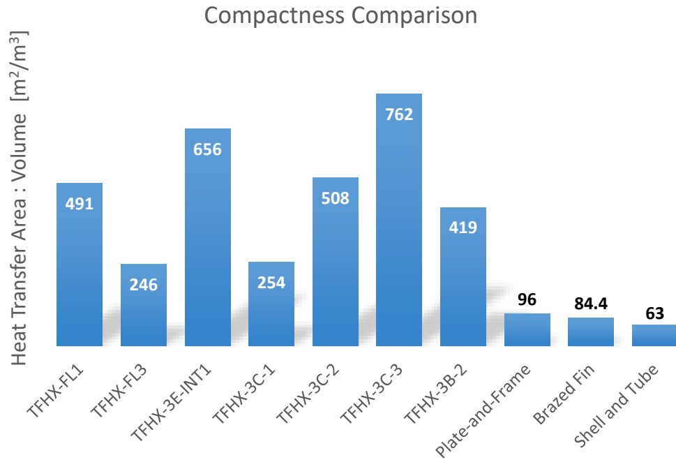
Figure 42. TFHX heat exchangers have more heat transfer area per volume compared to the previously tested plate-frame (APV), brazed fin (BAHX3), and shell and tube (ETHX) heat exchangers
