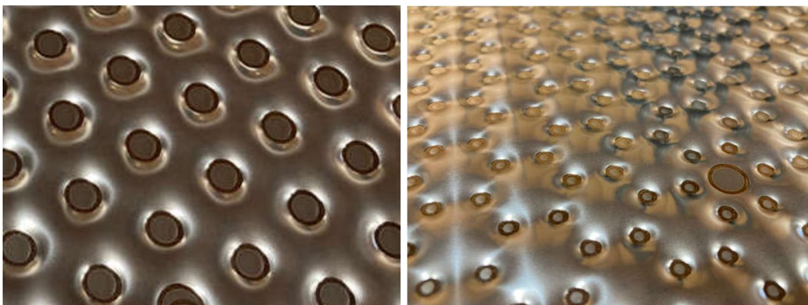
Figure 1. Triangular pattern (left) and hexagonal pattern (right). The hexagonal pattern enables larger internal channels.
