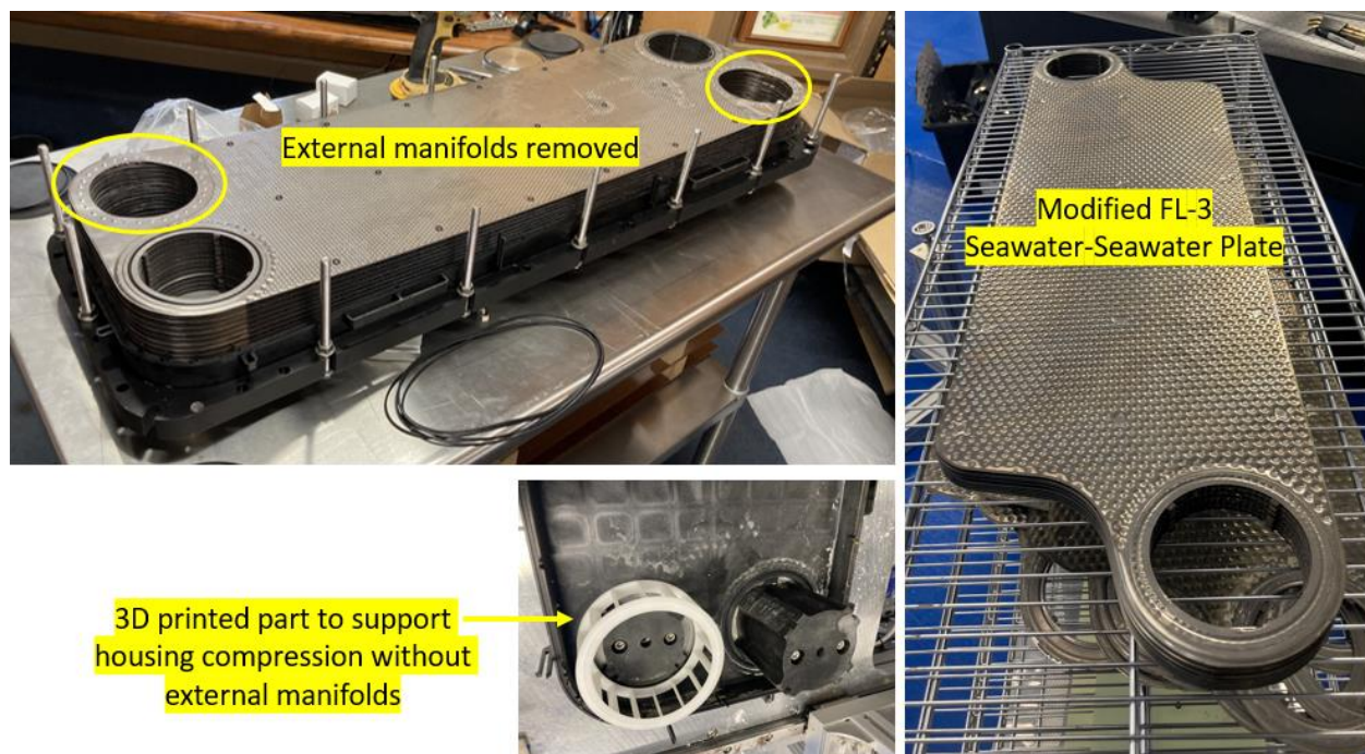
Figure 18. Modifications to remove external manifolds in FL3 SWAC plates. Circular spacers were required for internal manifolds but were less likely to rotate out of position.
