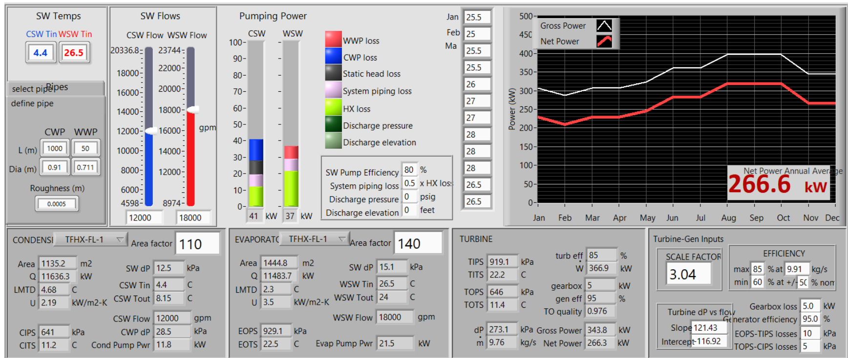
Figure 44. Screenshot of OTEC Power Calculator using TFHX FL1.
