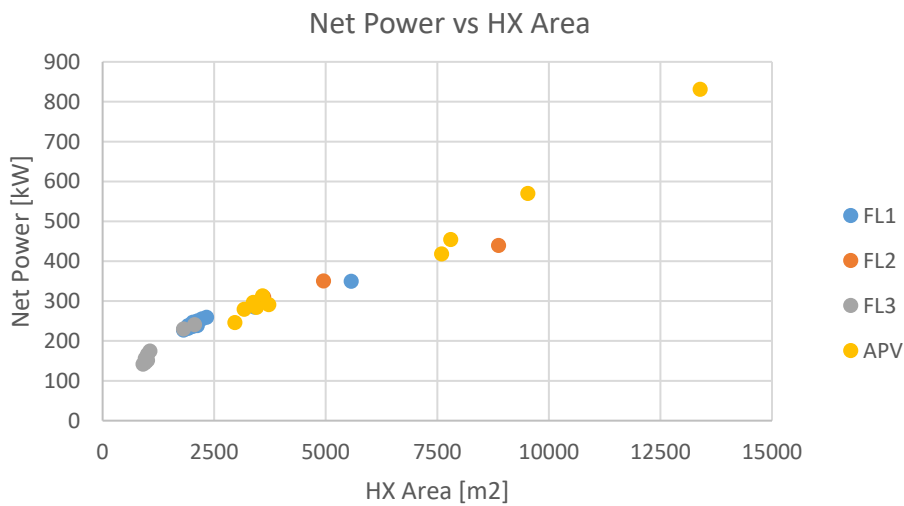
Figure 45. Net power vs HX area for fixed cold and warm seawater flow rates.
