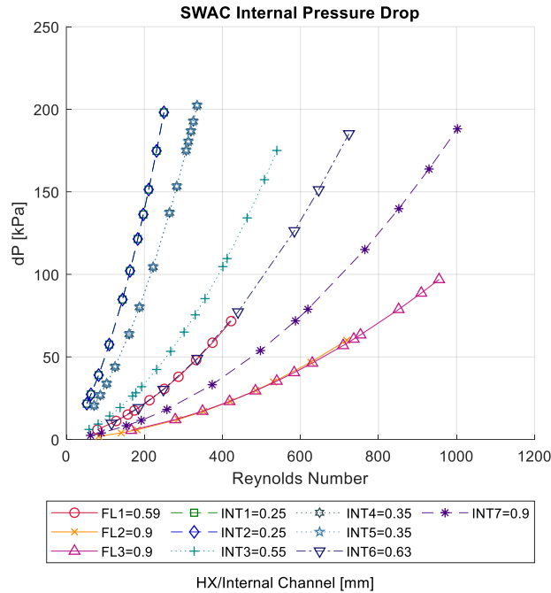
Figure 23. Internal seawater pressure drop compared to previous SWAC units.
