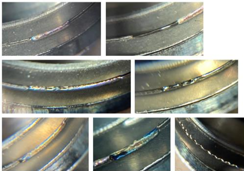
Figure 15. Visual inspection of welds performed using different parameters and shield gas flow rates reveals significant differences in weld quality. Smooth silver welds are preferred.
