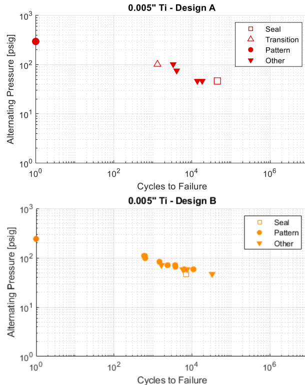
Figure 6. Fatigue life of two different 0.005" Ti plate designs.
