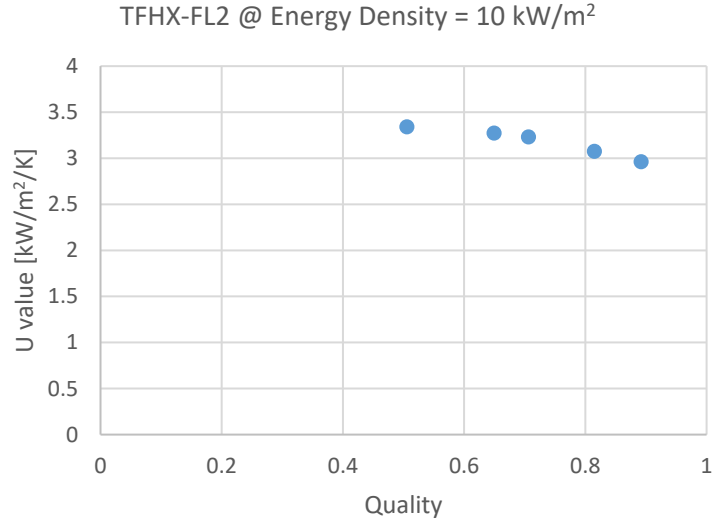
Figure 27. Effect of quality on U-value.
