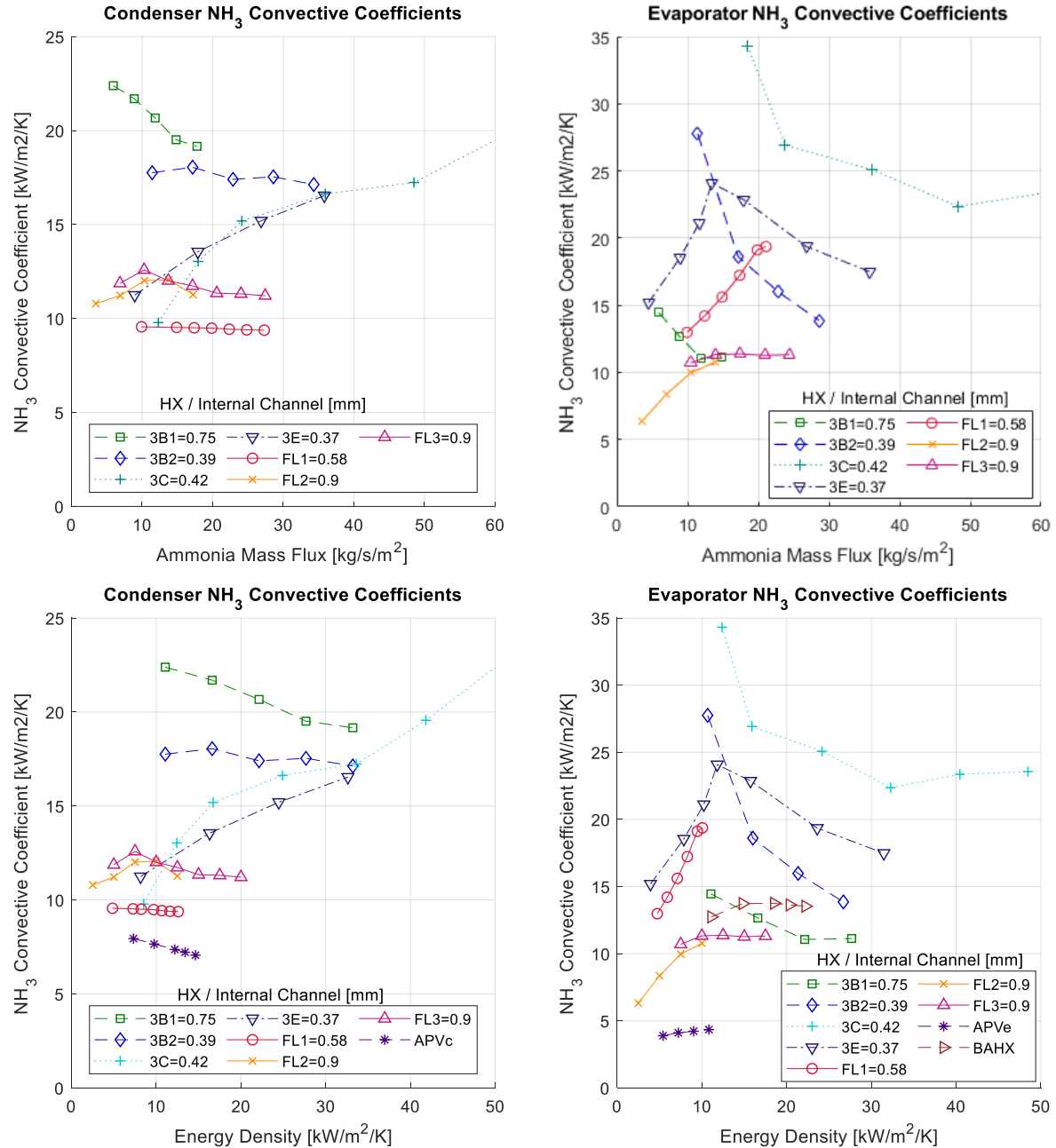
Figure 33. Comparison of ammonia convective coefficients with previous heat exchangers.
