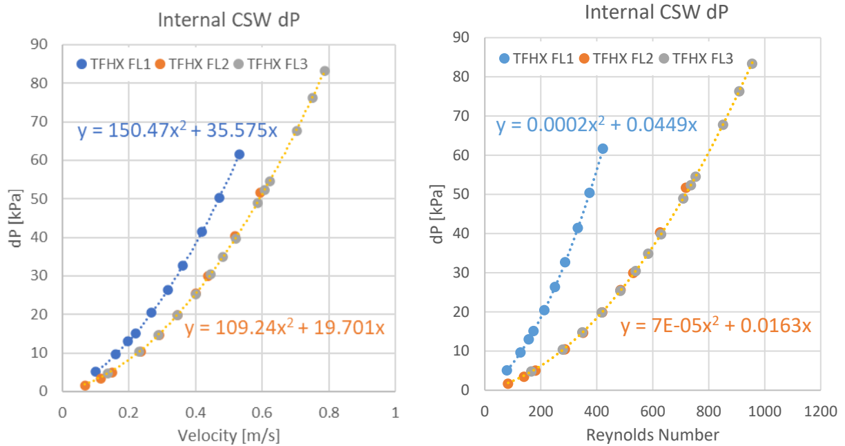
Figure 21. Internal seawater pressure drop for three TFHX designs.
