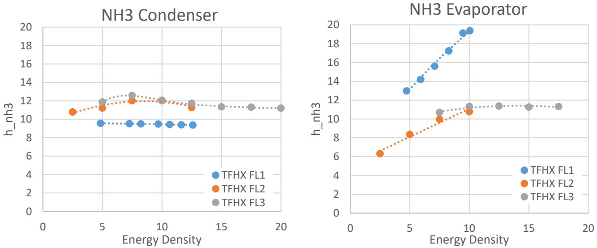
Figure 32. Ammonia-side convective coefficients for condenser and evaporator.
