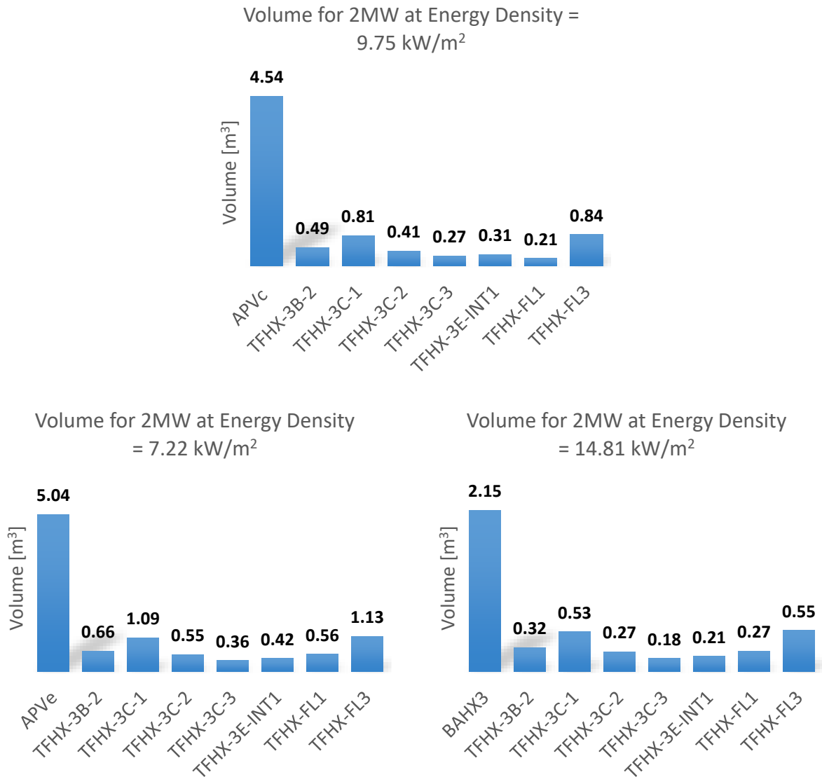
Figure 43. Comparison of volume required for 2MW of duty at various energy densities. Energy density was selected to match previously tested heat exchangers.
