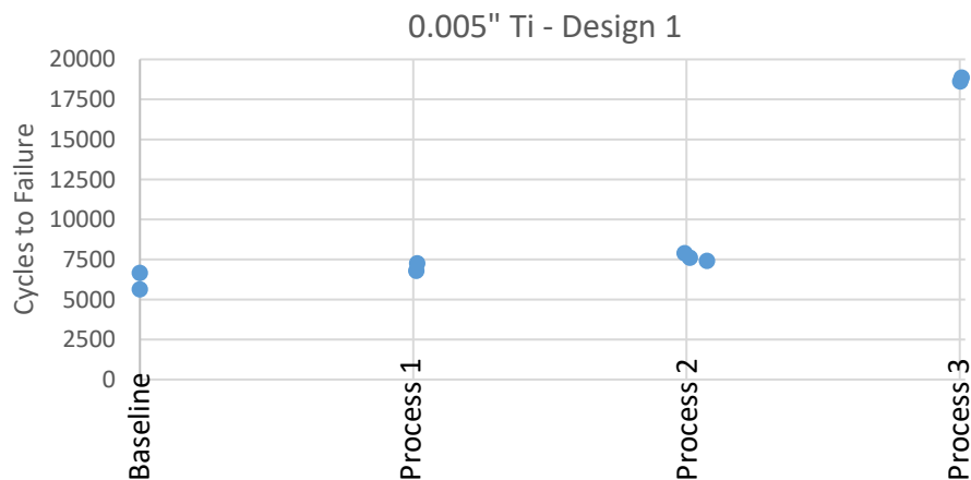
Figure 7. Fatigue life for baseline and three different process steps for 0.005" Ti plate.
