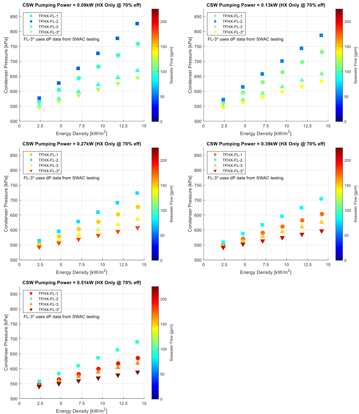
Figure 39. Comparison of condenser operating pressure versus energy density for cold seawater temperature = 6°C at different seawater pumping powers (through the heat exchanger only).
