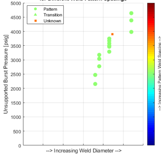
0.004" Ti Unsupported Burst Pressure vs Weld Diameter for Different Weld Pattern Spacings
