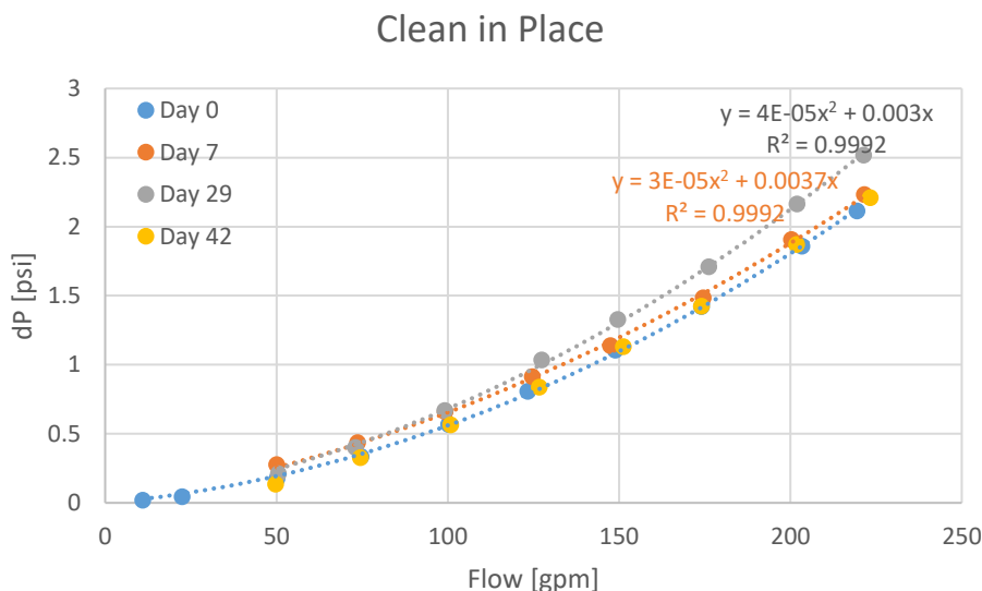
Figure 44. Pressure drop test for clean-in-place prototype.
