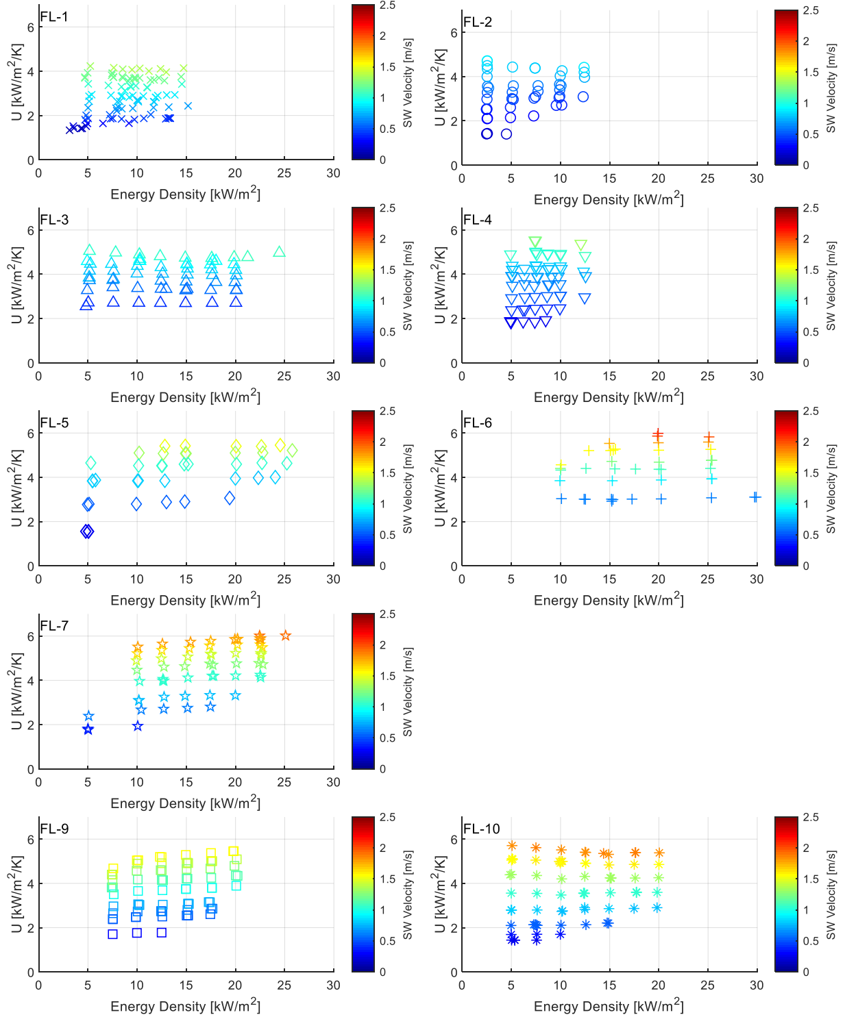
Figure 24. Condenser U -value vs energy density.
