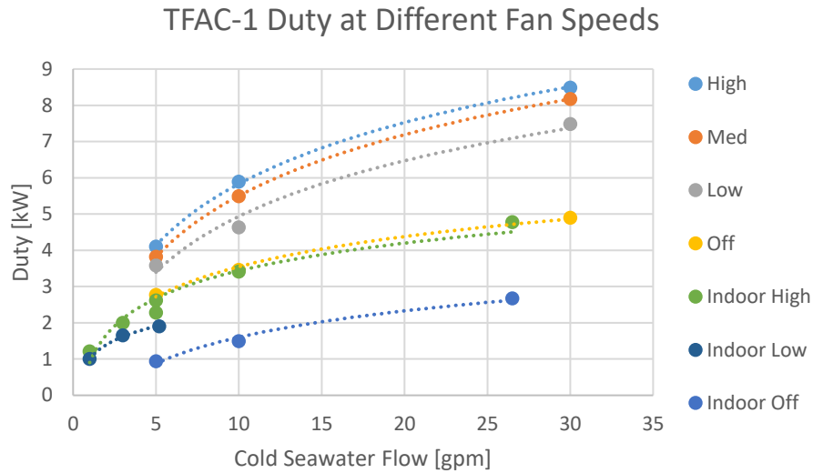
Figure 10. Duty vs seawater flow for different fan speeds.
