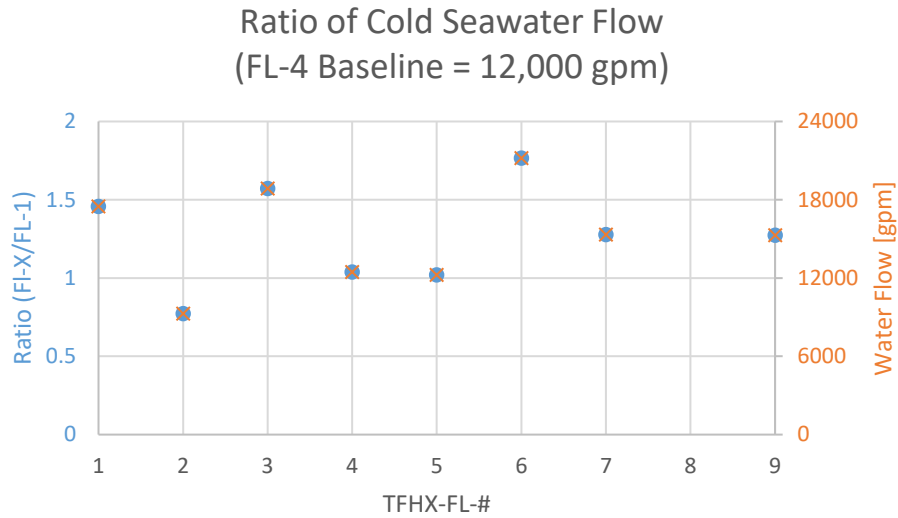
Figure 36. Ratio of optimized warm seawater flow rate compared to baseline TFHX-FL-4.
