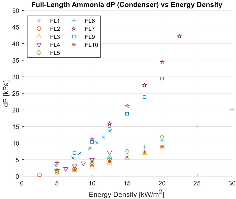
Figure 19. Ammonia pressure drop in condenser mode.
