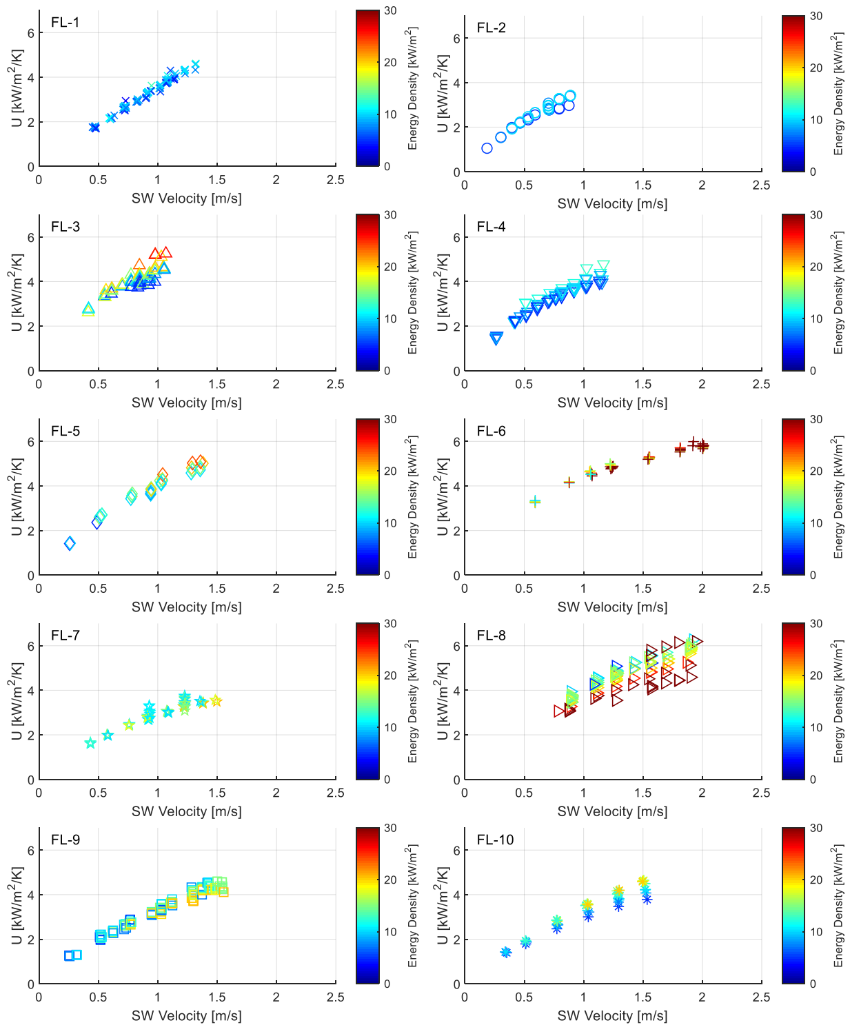
Figure 21. Evaporator U-value vs seawater velocity.
