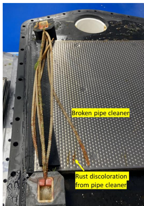
Figure 45. Broken pipe cleaner and rust stains on plates.
