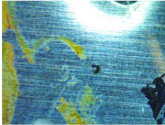
Figure 7. Pit in 0.002" SS316L foil along with rust spots.
