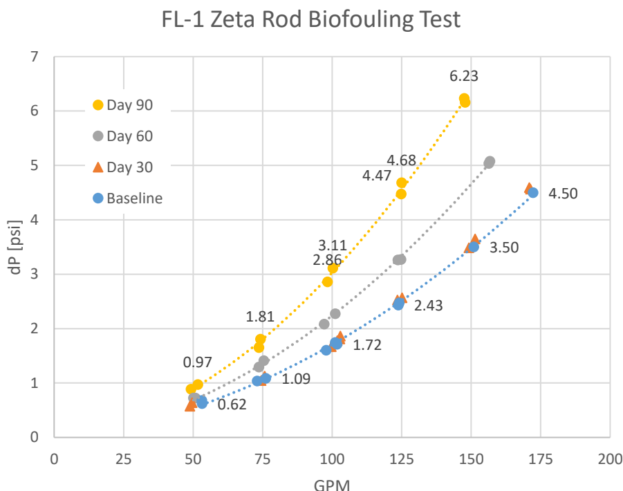
Figure 39. Zeta Rod test: Pressure drop vs flow.
