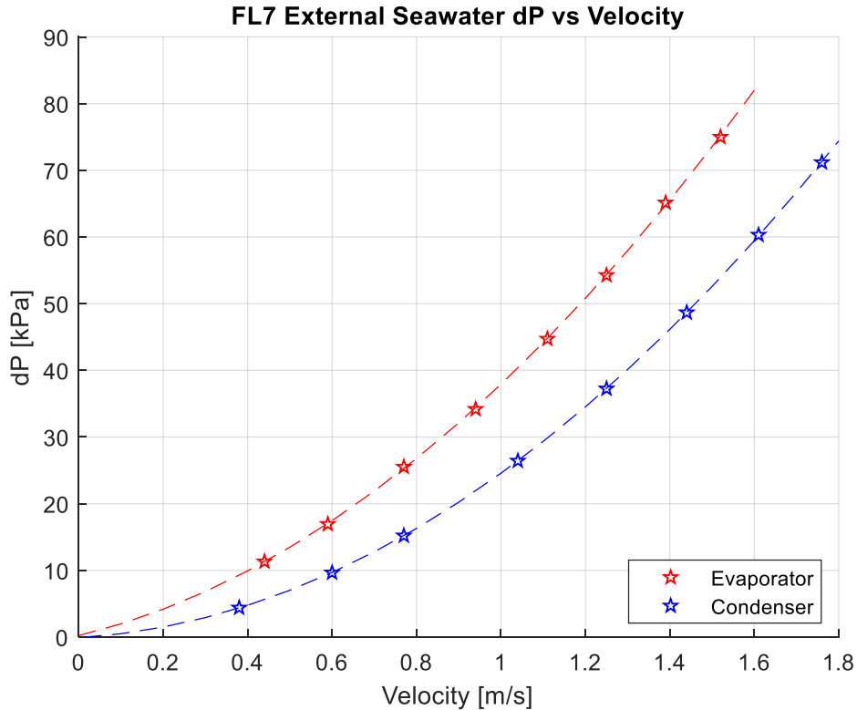
Figure 18. Substantial discrepancy in seawater pressure drop between condenser and evaporator tests.
