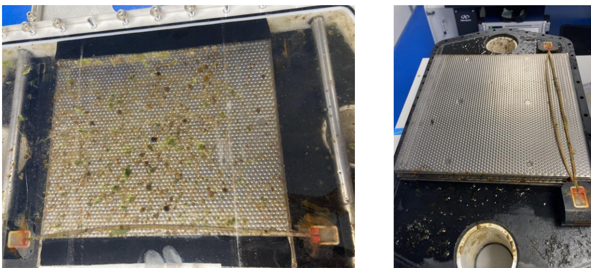
Figure 43. (left) Biofouling on the cover and first plate but not on the second plate (right).
