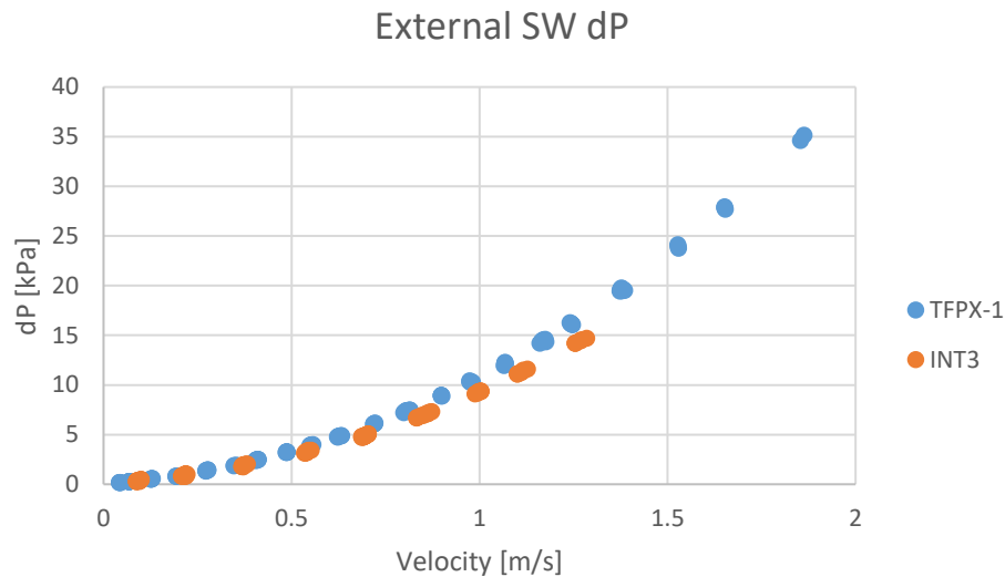
Figure 13. External dP vs velocity, INT3 and TFPX1 have external channel sizes = 1.36mm.
