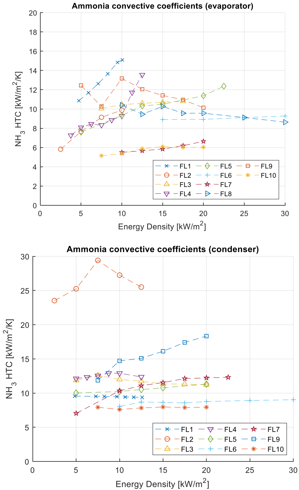
Figure 27. Ammonia-side convective coefficients for condenser and evaporator.
