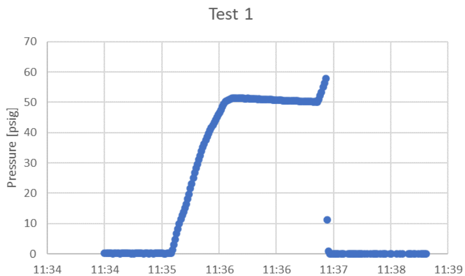
Figure 6. External pressure during first test. The module housing failed at 59 psig.
