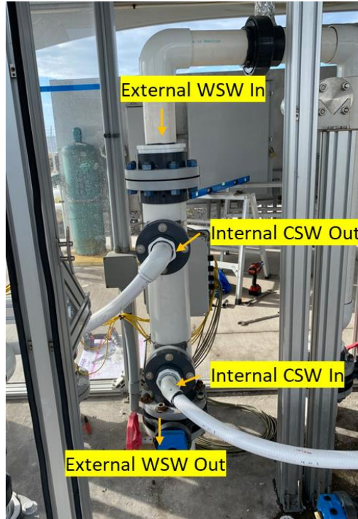
Figure 11. TFPX installed in the 100 kW Test Station.
