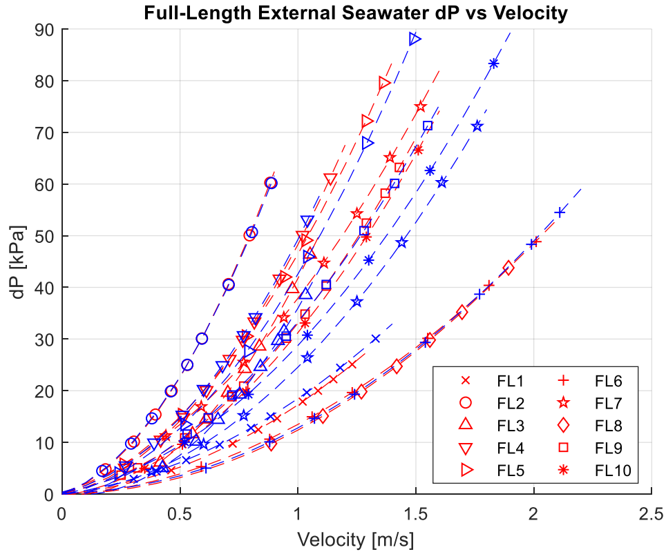
Figure 17. Seawater pressure drop for all ten TFHX units. Evaporator data is in red and condenser data is in blue.
