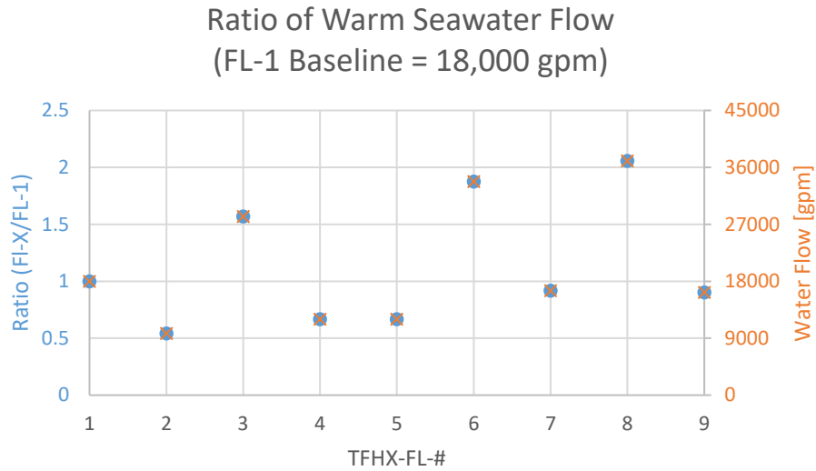
Figure 34. Ratio of optimized warm seawater flow rate compared to baseline TFHX-FL-1.
