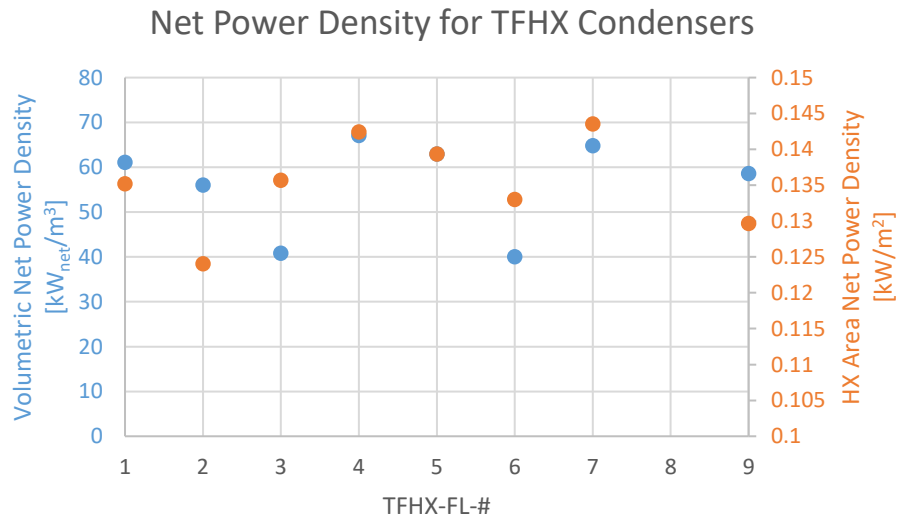
Figure 35. Comparison of net power density for different TFHX condensers.
