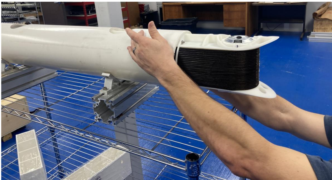
Figure 2. Inserting TFPX plate stack into pipe.
