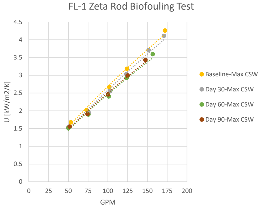
Figure 40. Zeta rod test: U-value vs flow.
