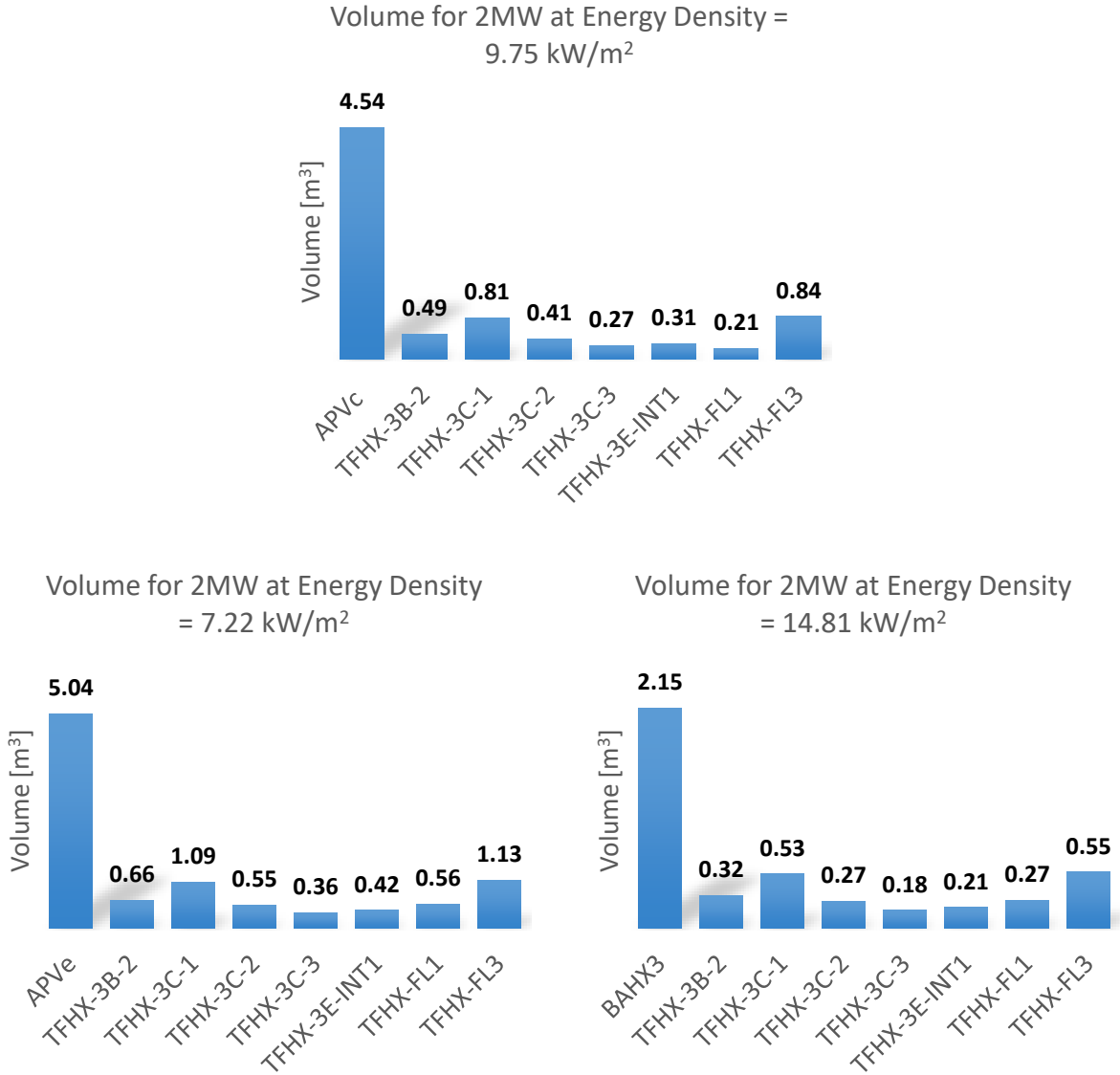
Figure 31. Comparison of volume required for 2MW of duty at various energy densities. Energy density was selected to match previously tested heat exchangers.
