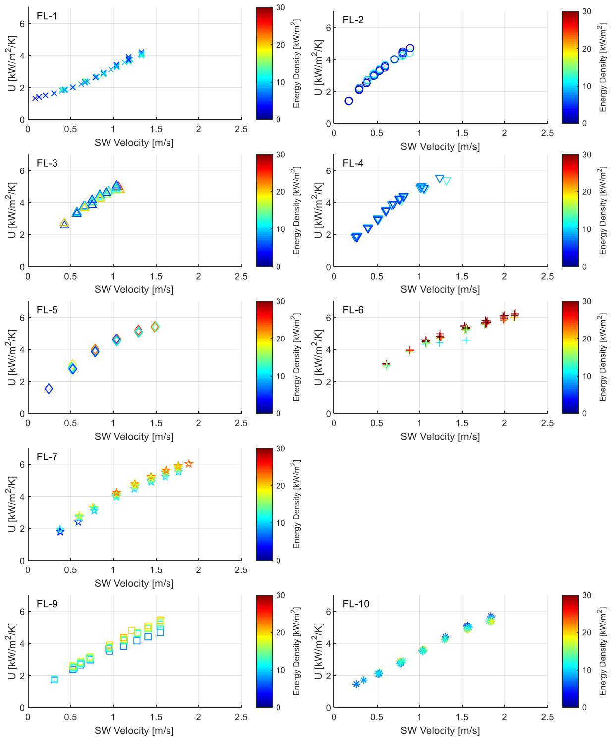
Figure 22. Condenser U -value vs seawater velocity.
