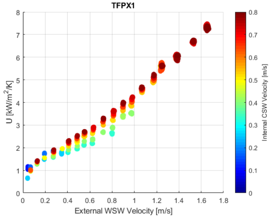
Figure 14. TFPX-1 overall heat transfer coefficient.
