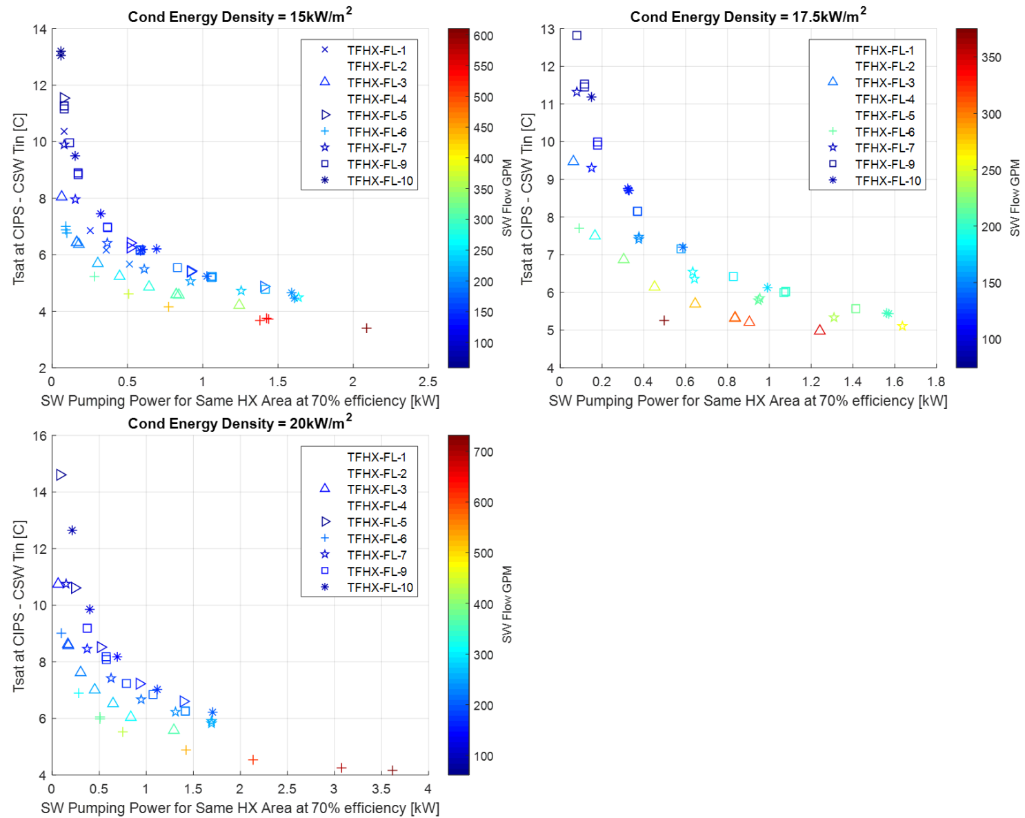
Figure 29. Condenser approach temperature vs pumping power at different energy densities.
