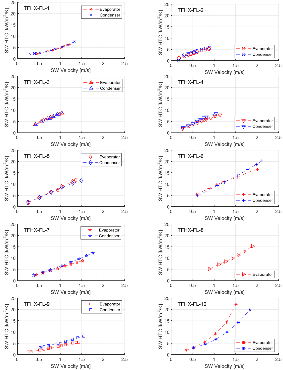
Figure 25. Seawater-side convective coefficients calculated individually for each configuration showed strong agreement.
