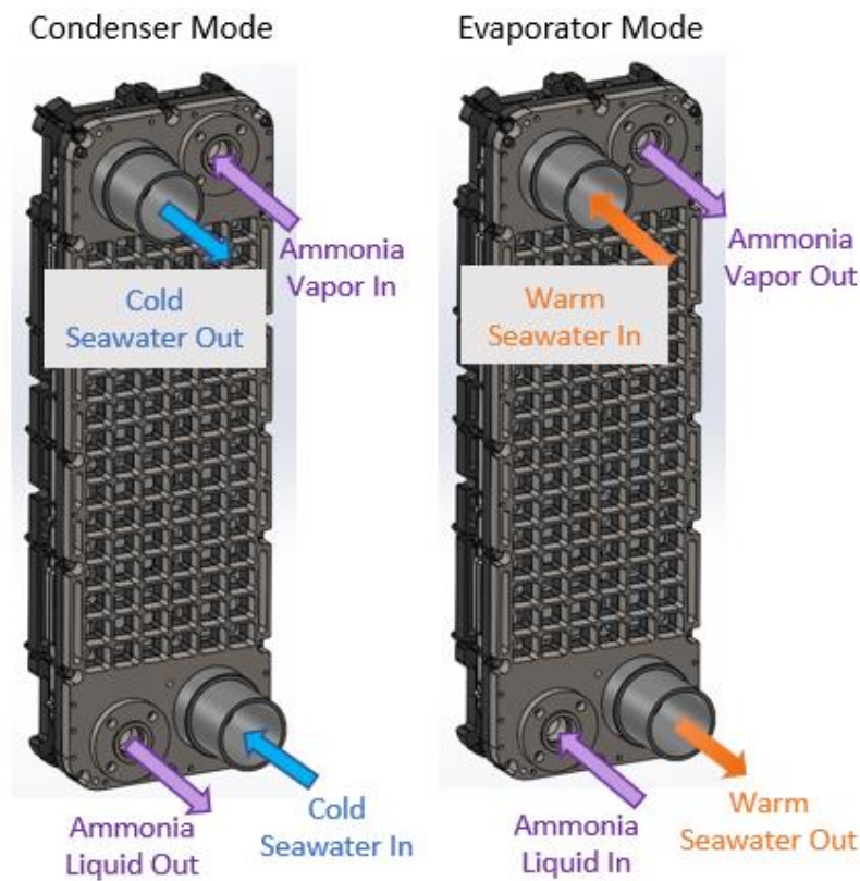
Figure 16. Full-length TFHX module configured for counterflow condenser and evaporator testing.
