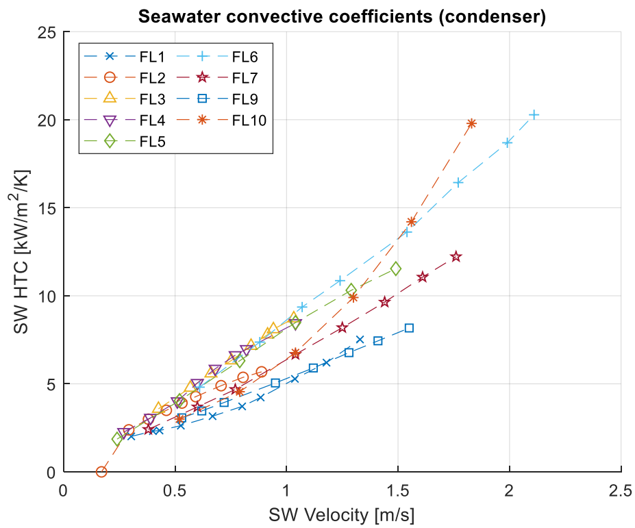
Figure 26. External seawater convective coefficients for all ten TFHX designs.
