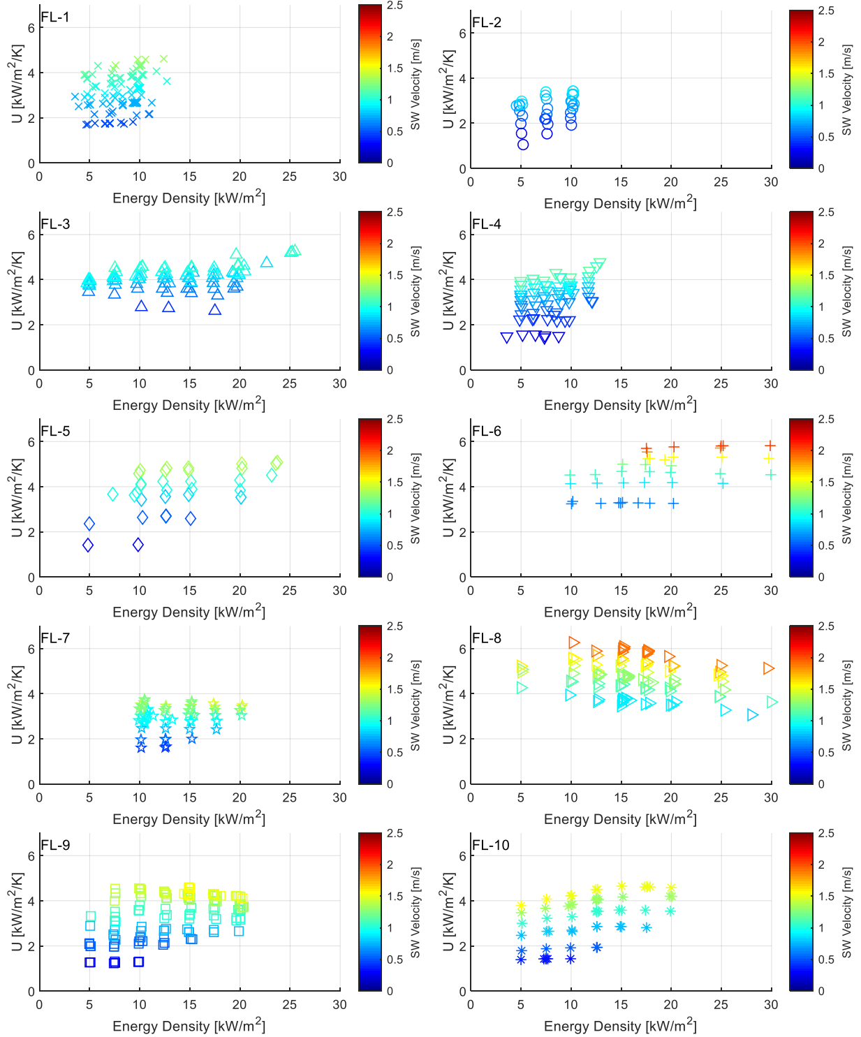
Figure 23. Evaporator U -value vs energy density.
