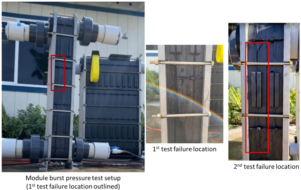
Figure 5. Module pressure test setup and failure locations for each of two tests.
