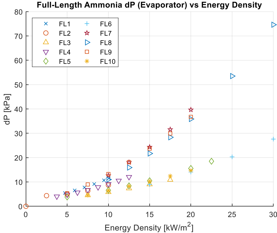
Figure 20. Ammonia pressure drop in evaporator mode.
