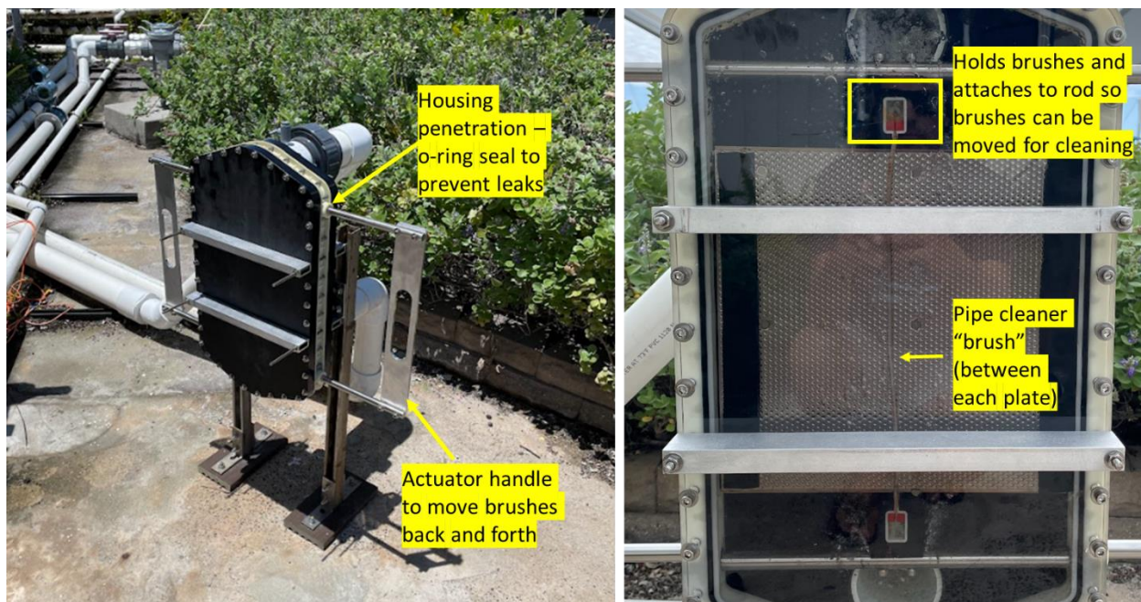
Figure 42. Clean in place prototype installed in Biofouling Test Station.
