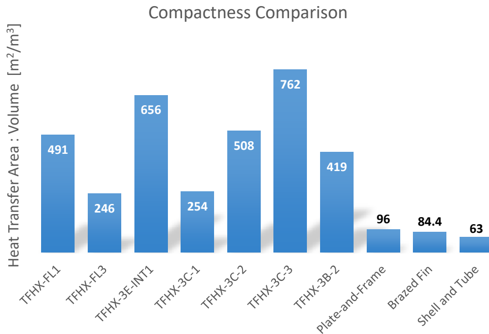
Figure 30. TFHX heat exchangers have more heat transfer area per volume compared to the previously tested plate-frame (APV), brazed fin (BAHX3), and shell and tube (ETHX) heat exchangers
