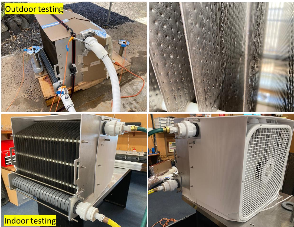
Figure 9. TFAC test setup.
