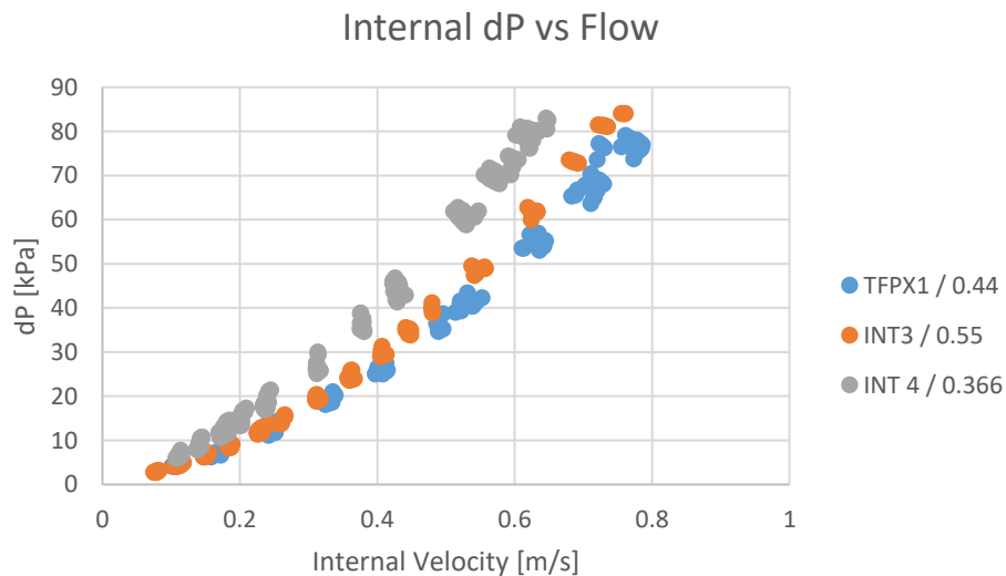
Figure 12. Internal dP vs velocity. The internal channel sizes of the INT units were slightly different than TFPX1.
