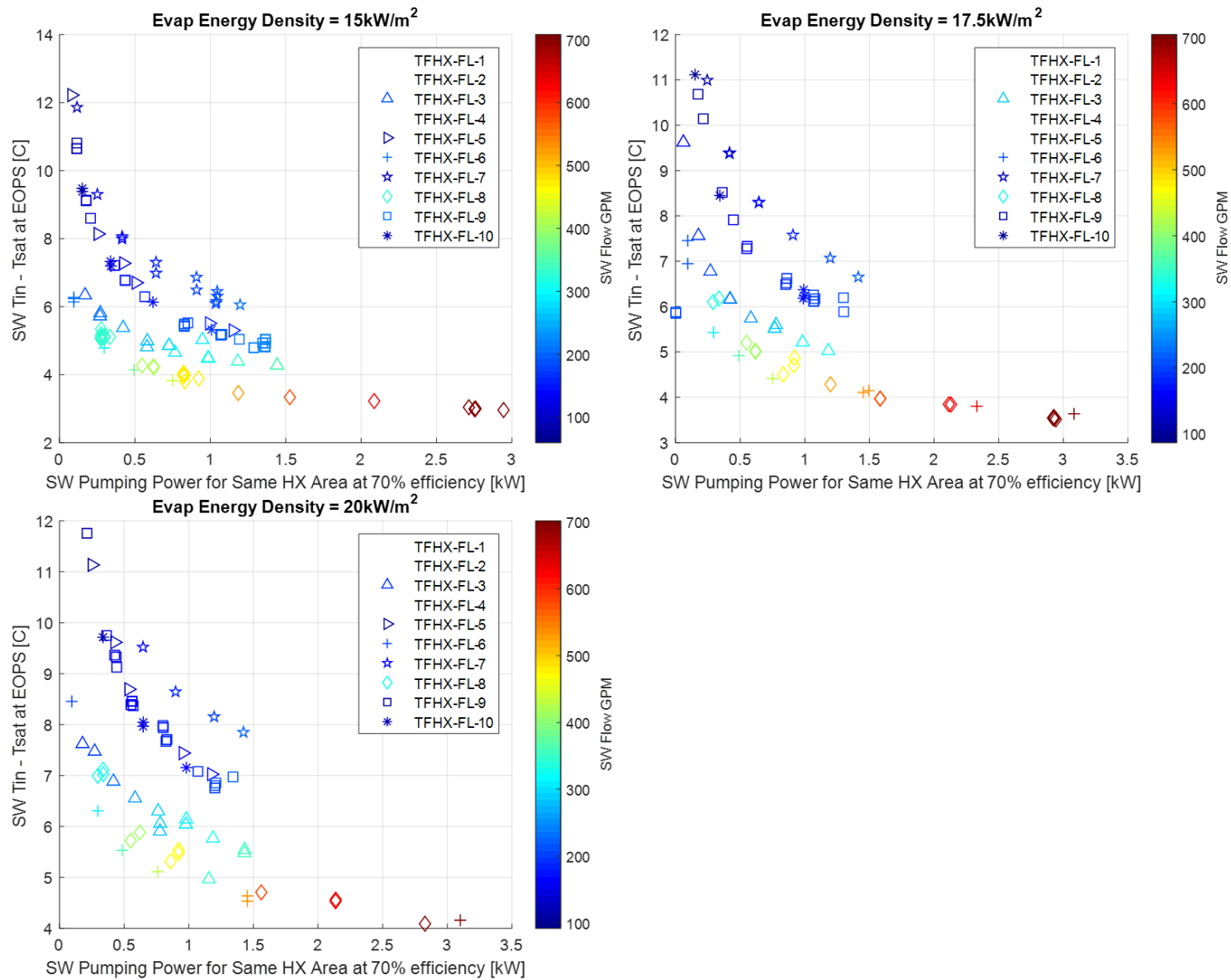
Figure 28. Evaporator approach temperature vs pumping power at different energy densities.
