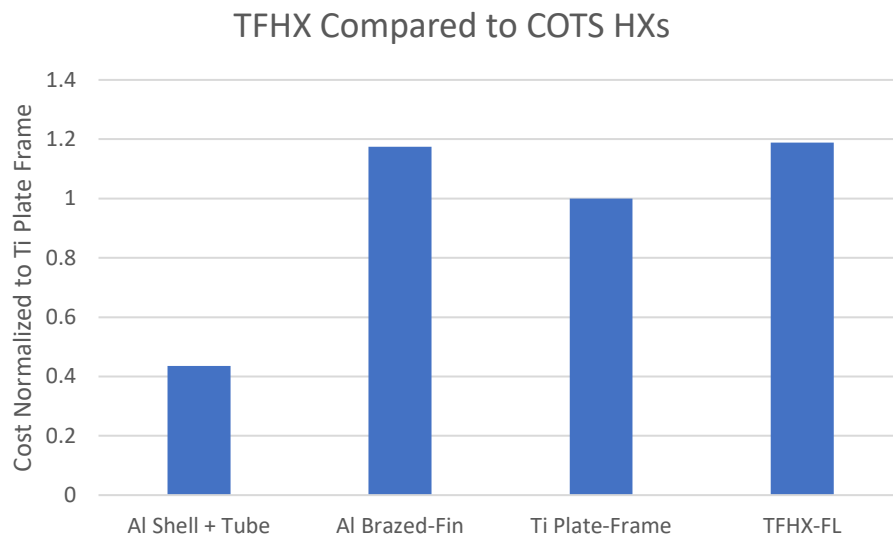
Figure 8. TFHX costs compared to COTS heat exchangers.
