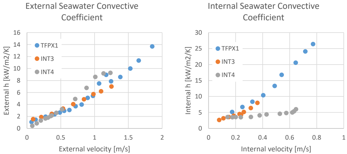
Figure 15. TFPX internal and external convective coefficients.
