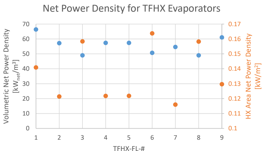
Figure 33. Comparison of net power density for different TFHX evaporators.
