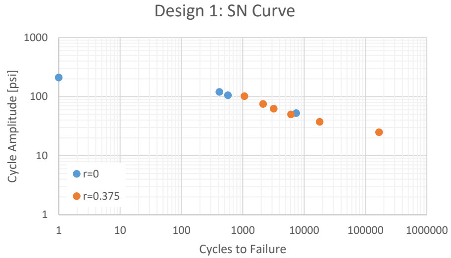
Figure 37. Design 1 SN curve.
