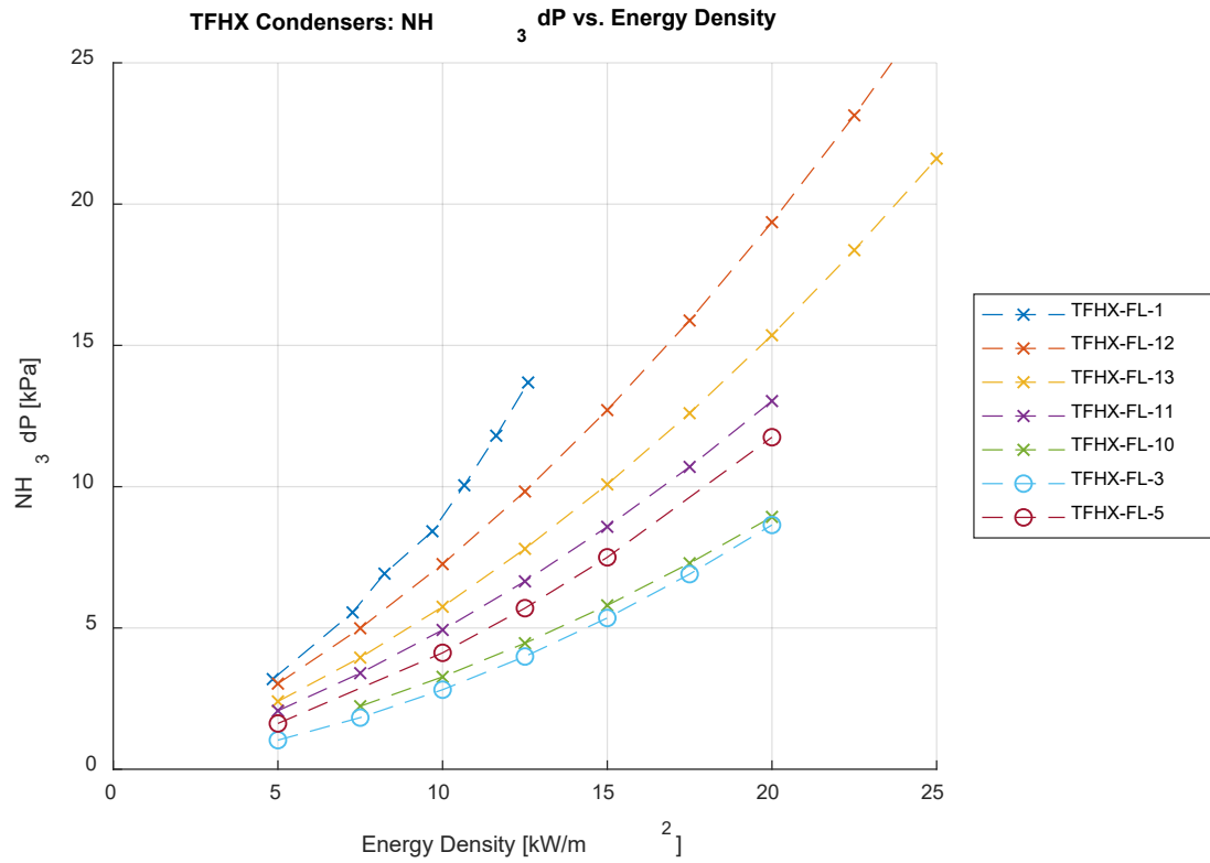
Figure 5. Ammonia pressure drop versus energy density for all 12-plate TFHX units.
