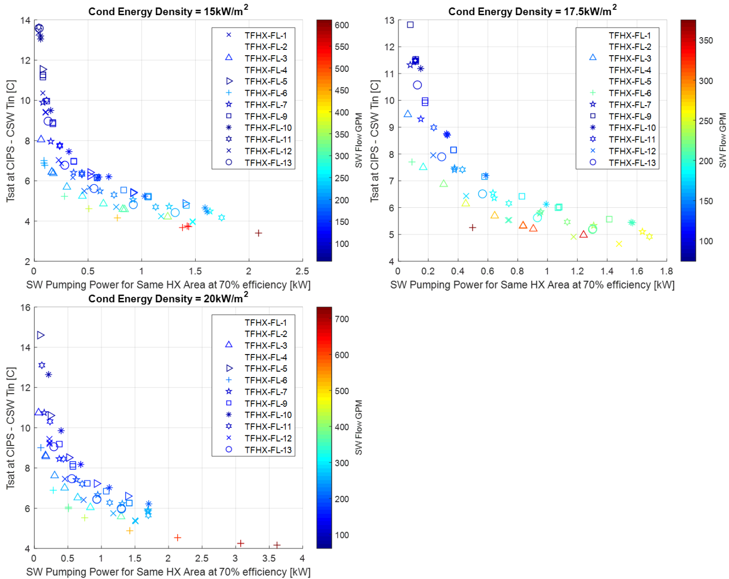
Figure 14. Condenser approach temperature vs pumping power at different energy densities.
