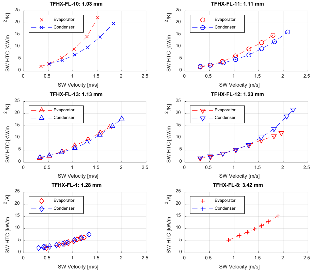
Figure 8. Seawater-side convective coefficients for TFHX units with different internal channel sizes and plate spacings. External channel size is shown after the unit number.
