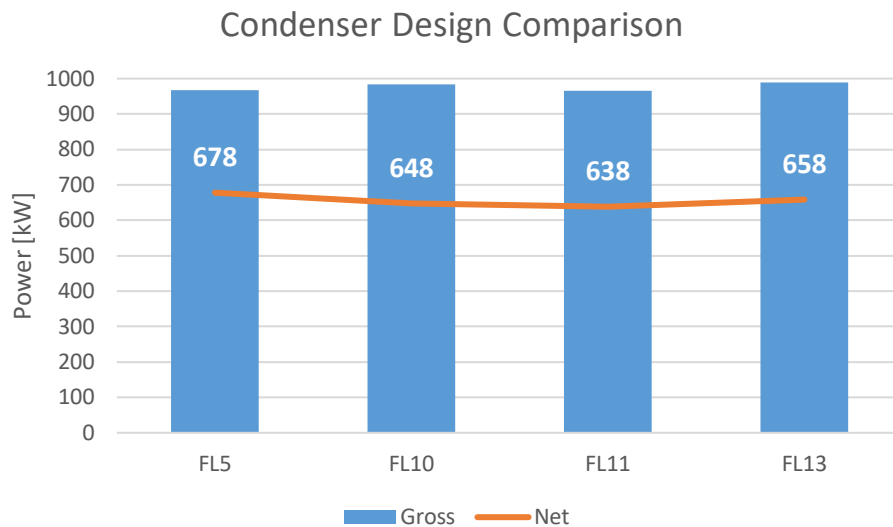
Figure 18. Comparison of condenser designs in OTEC system.
