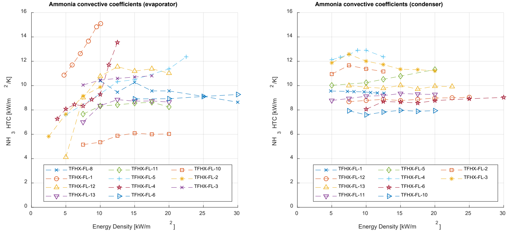
Figure 12. Ammonia-side convective coefficients for evaporator and condenser. TFHXs are listed from smallest ammonia effective channel (TFHX-FL8/-FL1) to largest (TFHX-FL3).
