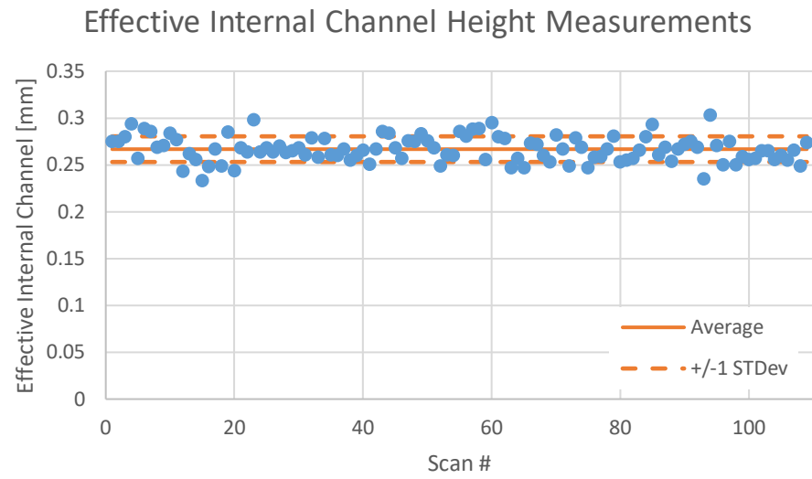
Figure 22. Effective internal channel size measurements on 10 plates.
