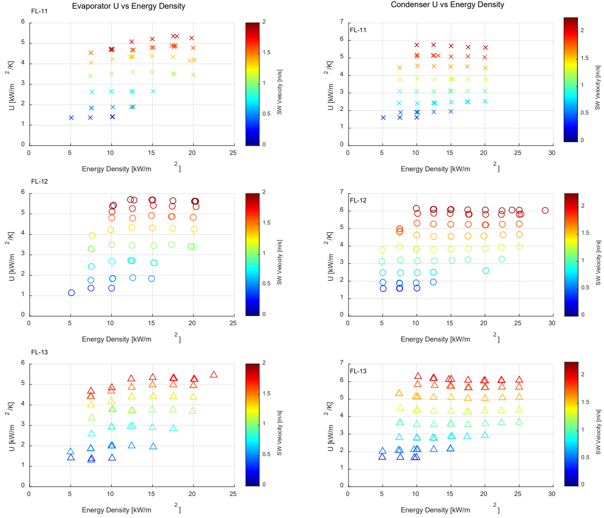
Figure 7. U-value vs energy density.
