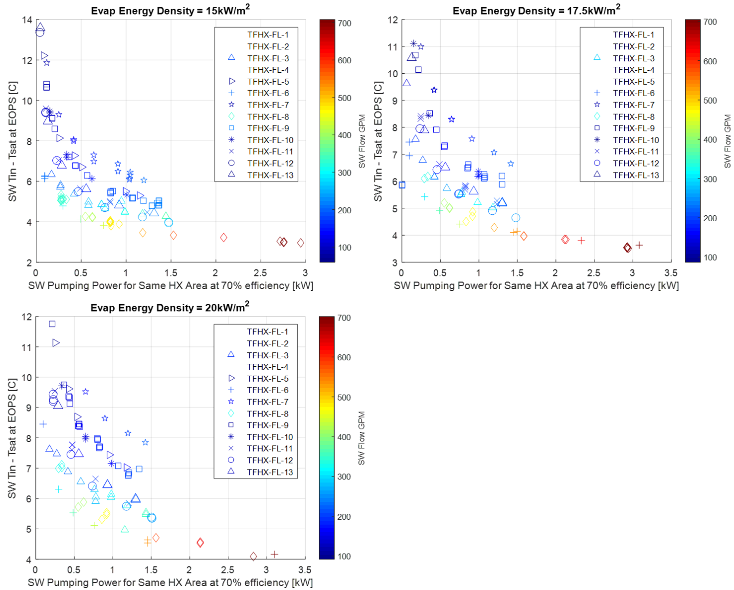
Figure 13. Evaporator approach temperature vs pumping power at different energy densities.
