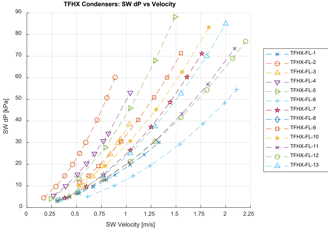
Figure 4. Seawater pressure drop for all tested TFHX units.
