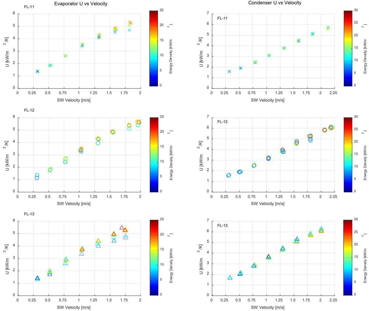
Figure 6. U-value vs seawater velocity.
