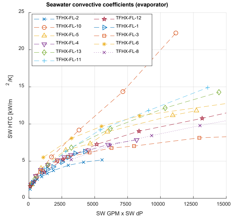
Figure 10. Evaporator seawater convective coefficients. TFHX units are listed from smallest seawater channel (TFHX-FL2) to largest (TFHX-FL8)
