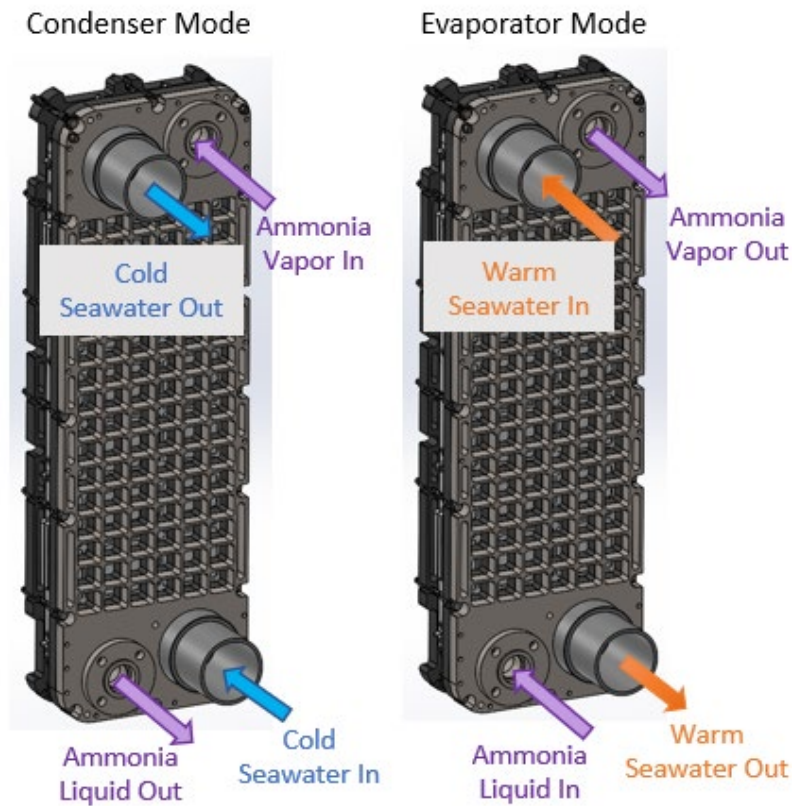
Figure 2. Full-length TFHX module configured for counterflow condenser and evaporator testing.
