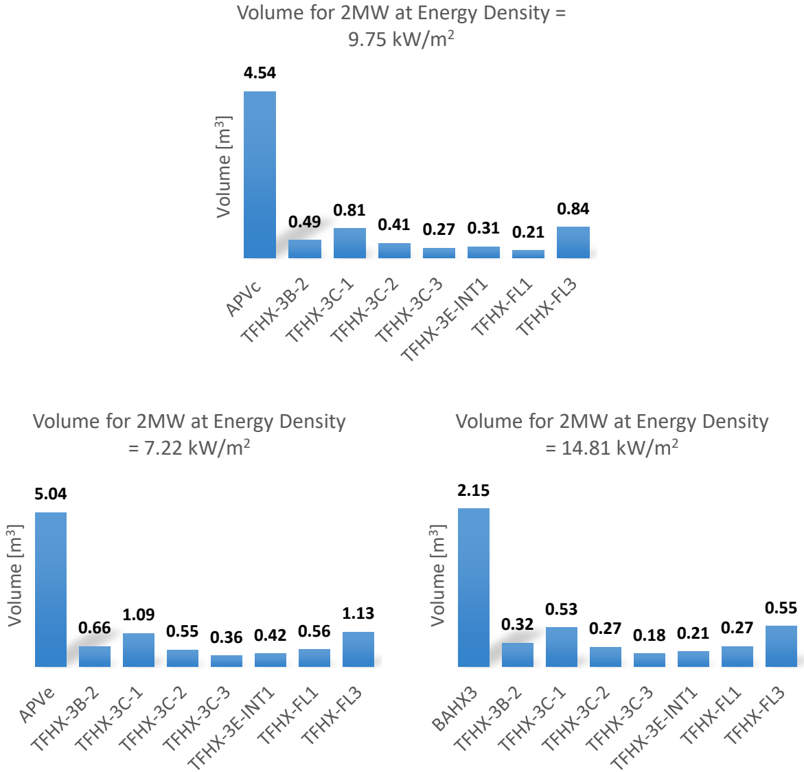
Figure 16. Comparison of volume required for 2MW of duty at various energy densities. Energy density was selected to match previously tested heat exchangers.
