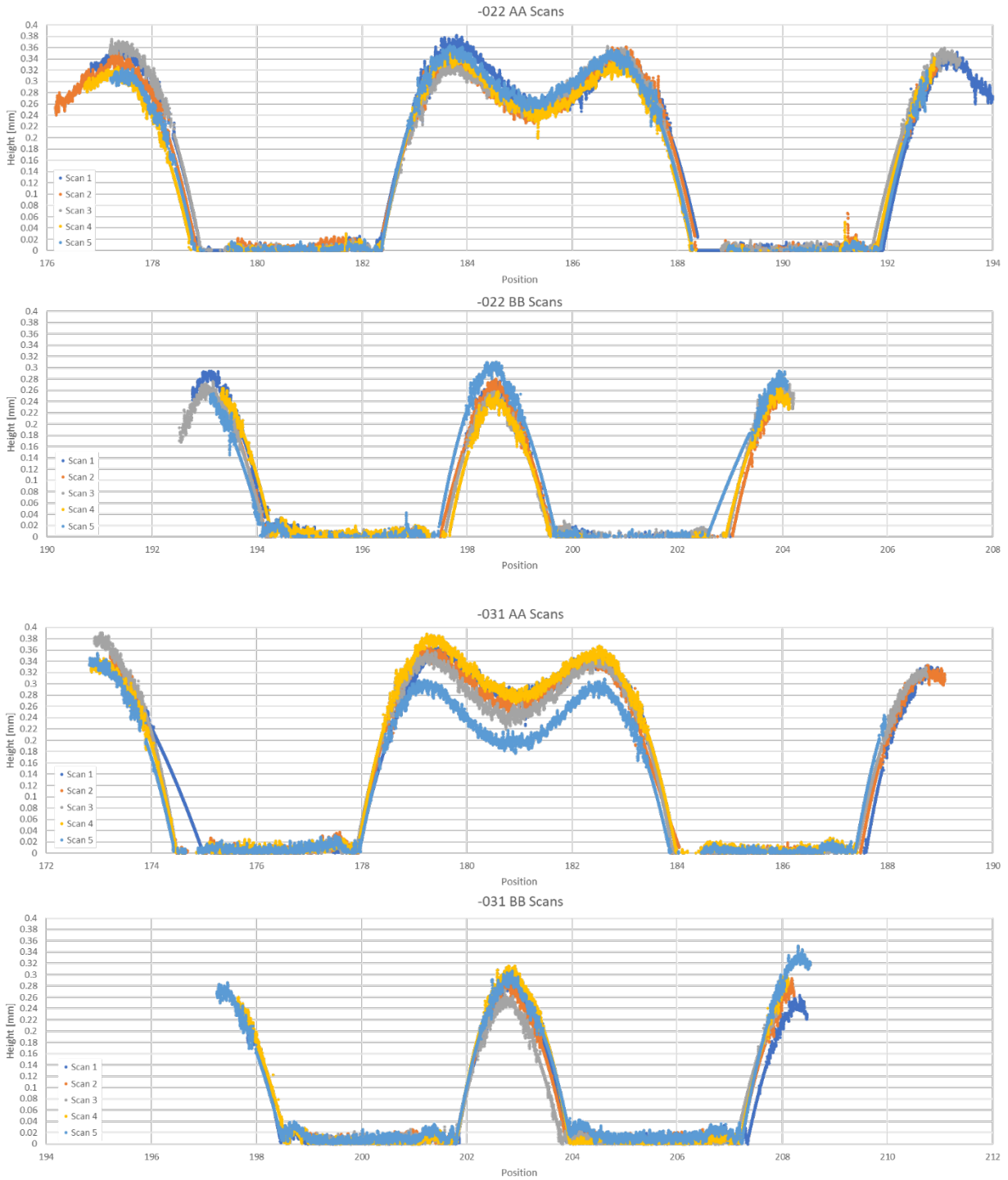
Figure 23. Overlay of line scans on two plates. 10 scans were performed on each plate; 5 scans across the A-A profile and 5 scans across the B-B profile.
