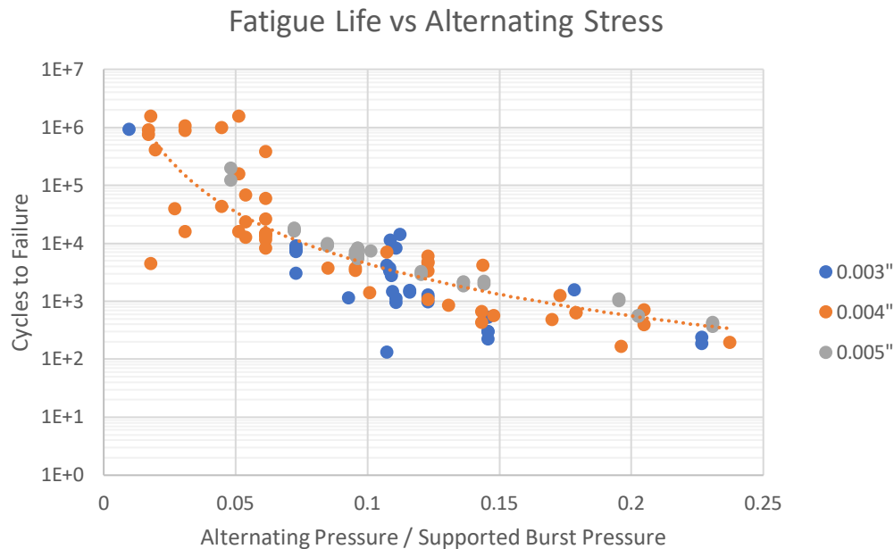
Figure 19. Cycles to failure vs ratio of alternating pressure amplitude/supported burst pressure. Data from 0.003" and 0.004" samples are from different plate shapes and mostly transition / seal weld failures. 0.005" data shows pattern failures only.
