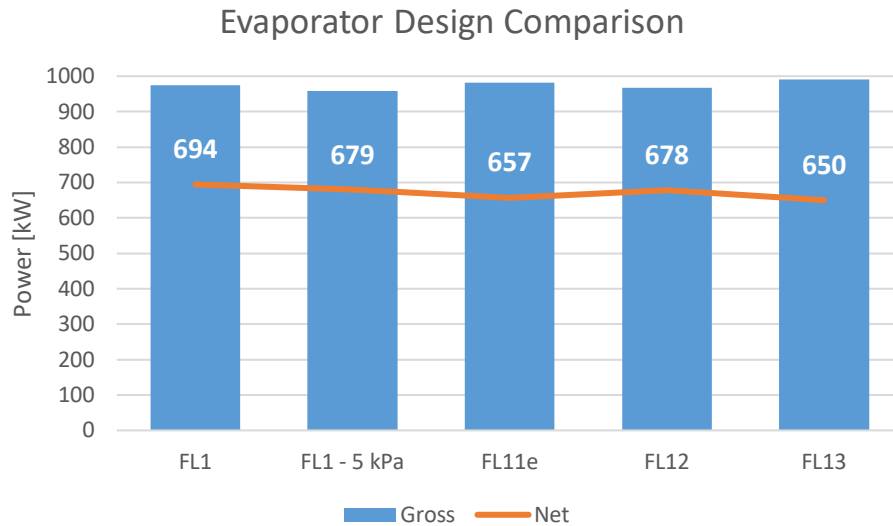
Figure 17. Comparison of evaporator designs in OTEC system.
