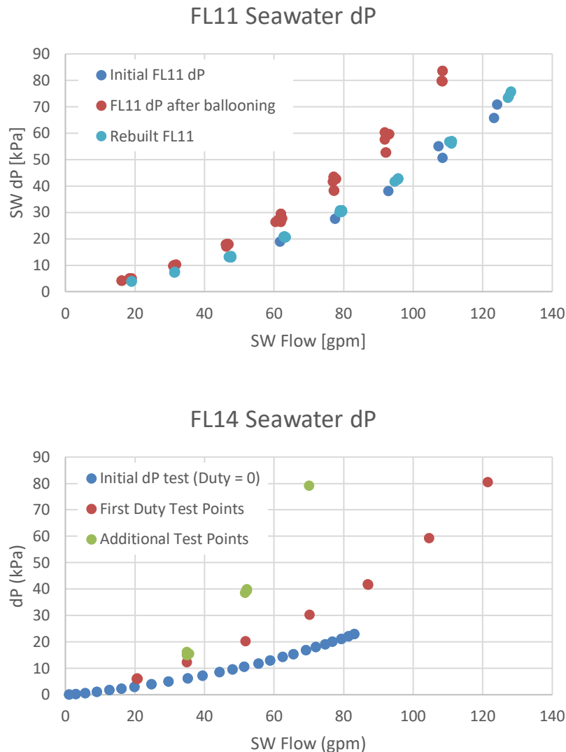
Figure 3. Substantial discrepancy in seawater pressure drop between initial and subsequent data points in FL11 and FL14. Upon disassembly, several plates had expanded areas between the internal and external seal welds which blocked off some of the seawater flow area.
