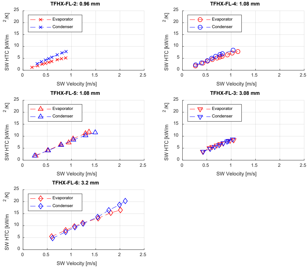
Figure 9. Seawater-side convective coefficients for TFHX units with the same weld design but different expansion pressures. External (seawater) channel size is shown after the unit number.
