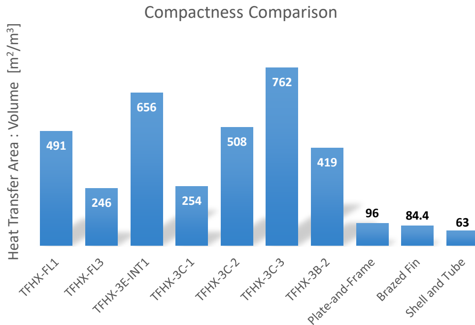
Figure 15. TFHX heat exchangers have more heat transfer area per volume compared to the previously tested plate-frame (APV), brazed fin (BAHX3), and shell and tube (ETHX) heat exchangers
