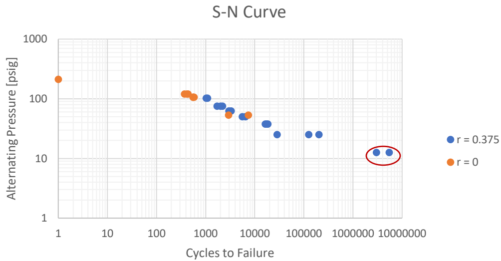
Figure 21. S-N Curve for 0.005" sample at two different stress conditions, r = 0 and r = 0.375 .
