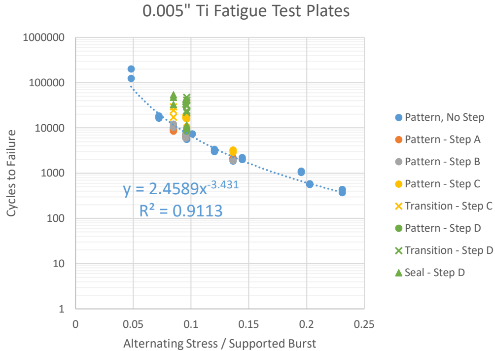
Figure 20. Effect of variation on additional fabrication step and alternating pressure on failure weld and cycles to failure.
