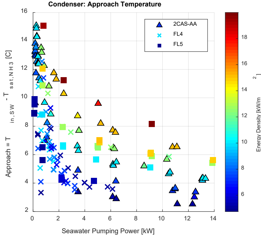
Figure 22. Condenser approach temperature.
