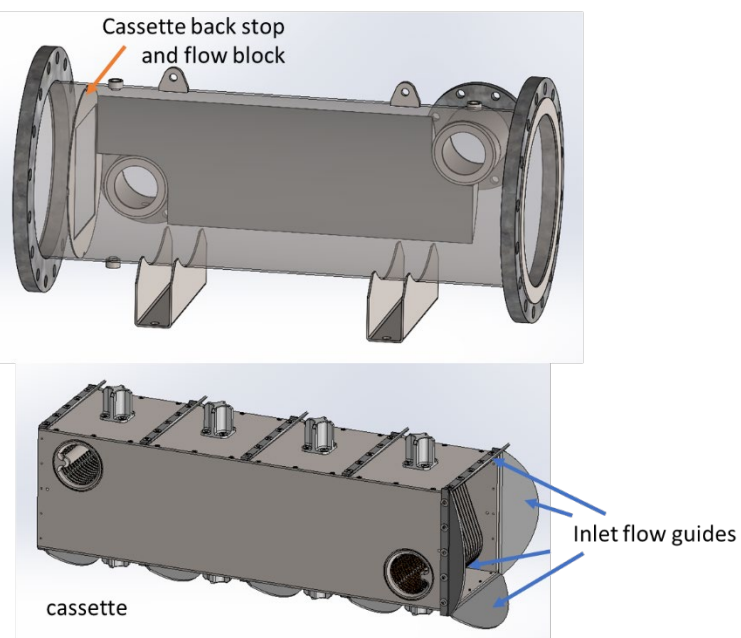
Figure 26. TFPX housing and cassette.
