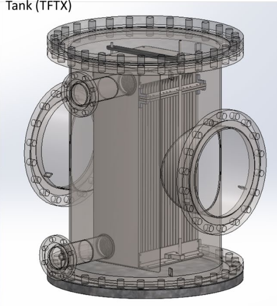
Tank (TFTX)
