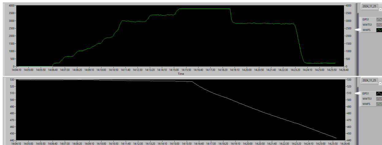
Figure 3. (top) Incrementally increasing warm seawater flow through the TFHX evaporator. (bottom) Depressurization on the ammonia side indicates a loss of sealing which coincides with plate shift that started between 3000-3800 gpm.
