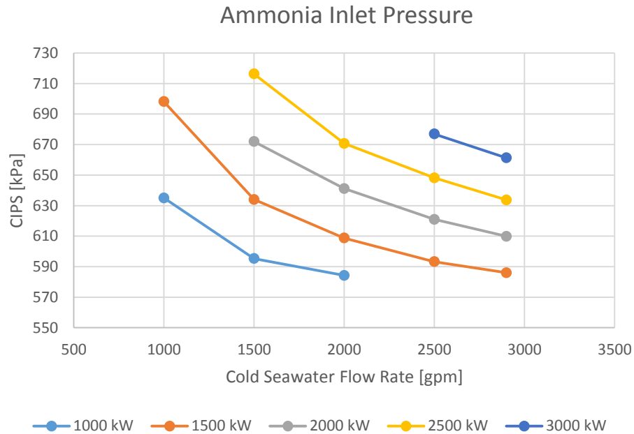
Figure 3-6. Ammonia absolute pressure at condenser inlet
