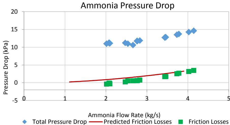
Figure 3-14. Ammonia-side frictional losses.
