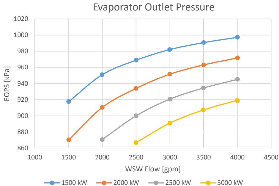
Figure 3-15. Ammonia absolute pressure at evaporator outlet increases with increasing seawater flow rates.
