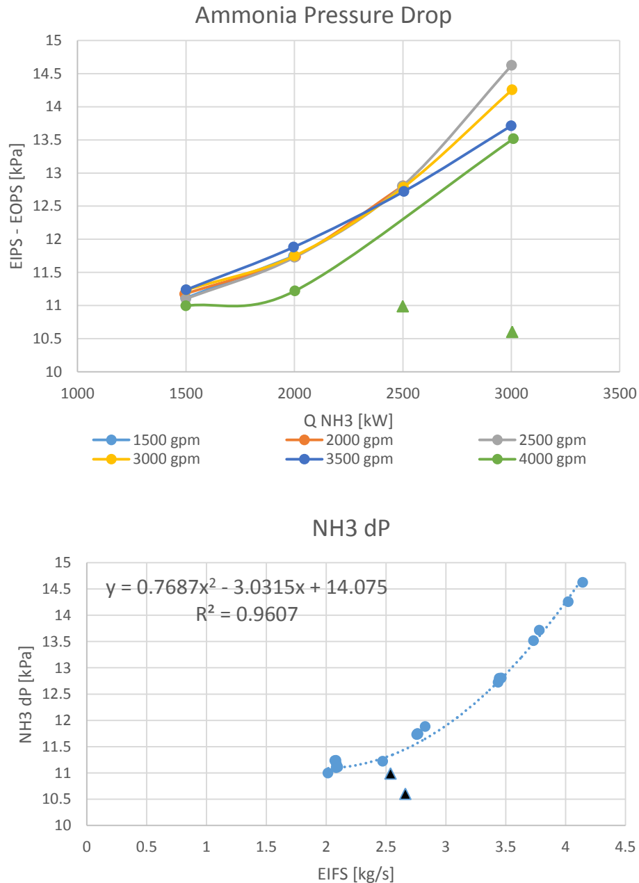
Figure 3-13. Ammonia-side pressure drop. Triangle data points were collected at higher quality than the other points. Since quality effects were not specifically tested, the high quality points are considered outliers, shown for completeness but not included in analysis.
