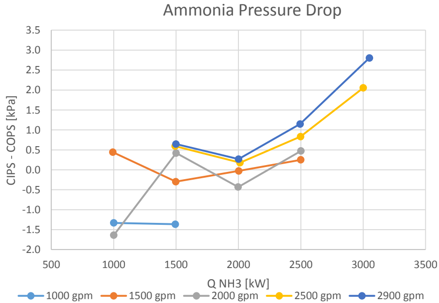
Figure 3-5. Ammonia-side pressure drop
