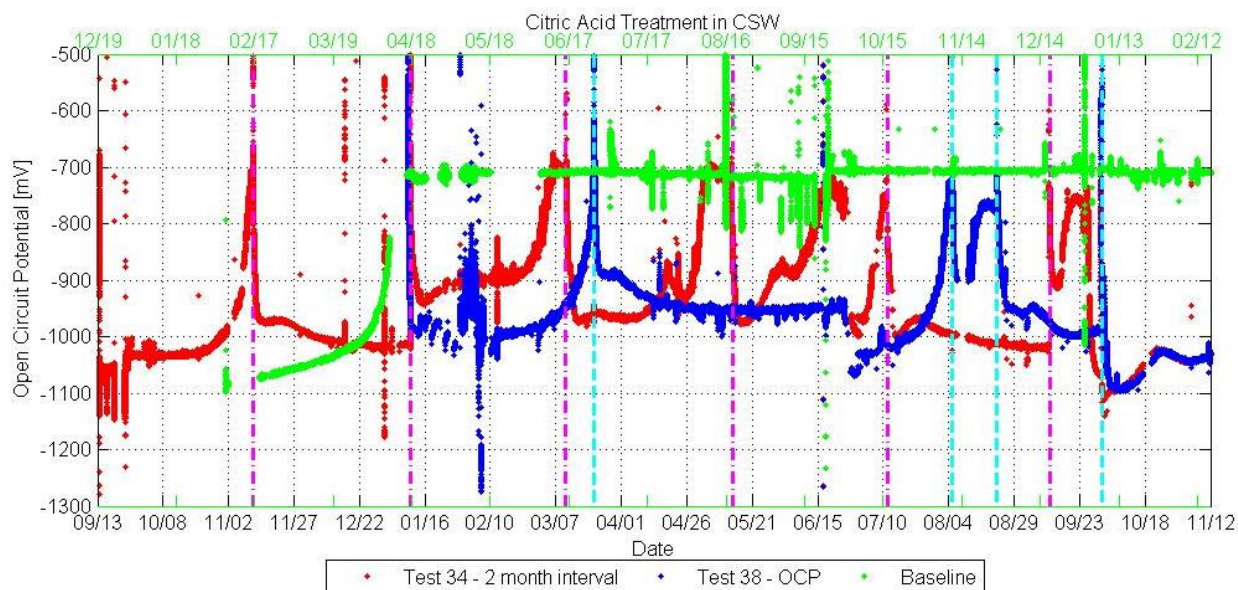
Figure 4-15. Citric acid treatments in CSW. Test 34 2-month treatment dates are indicated by magenta lines and Test 38 OCP-based treatment dates are indicated by cyan lines. Only the first 425 days of exposure are shown for the baseline coupon (actual date is on upper x-axis in green). Treatments have been successful in lowering OCP to between -900 mV and -1000 mV. Test 38 was in stagnant fresh water for several hours due to a flow disruption on 10/1/14.
