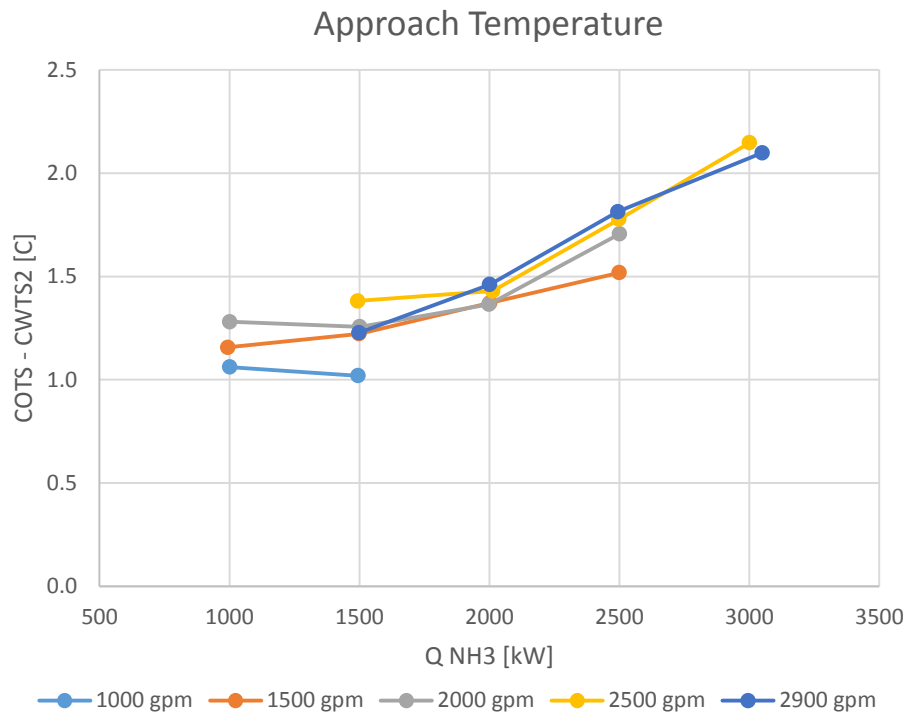
Figure 3-7. Approach temperature
