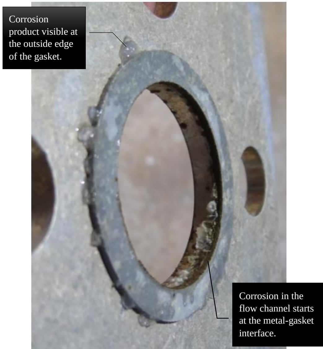
Figure 4-20. In-line sample showing corrosion in the flow channel starting at the metal-gasket interface and on the outside edge of the gasket.
