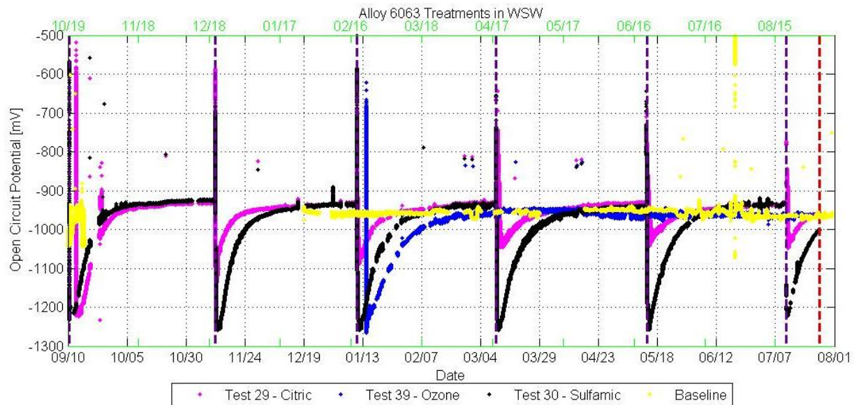
(a) Alloy 6063-T52 coupons in WSW. Treatment intervals are 2 months; dates are indicated by purple dashed lines. No ozone treatment was performed on 3/14/2014. Only first 325 days of exposure are shown for the baseline coupon (actual date is on upper x-axis in green). Treatment coupons were removed on 7/25/2014 (red line). Baseline coupon is still installed.
