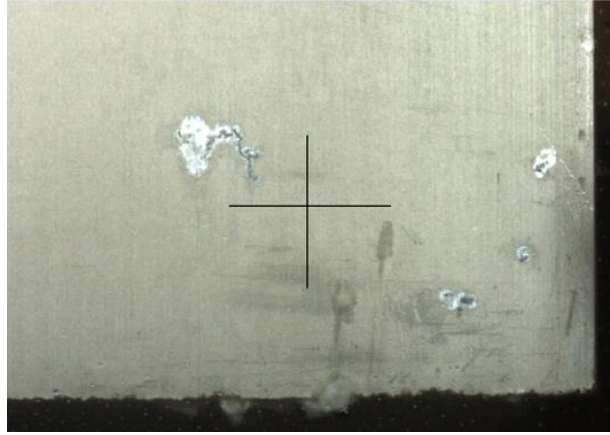
Figure 4-16. After eight months of exposure, pits and corrosion product buildup were observed on the trailing edge of the sample receiving citric acid treatment every two months.
