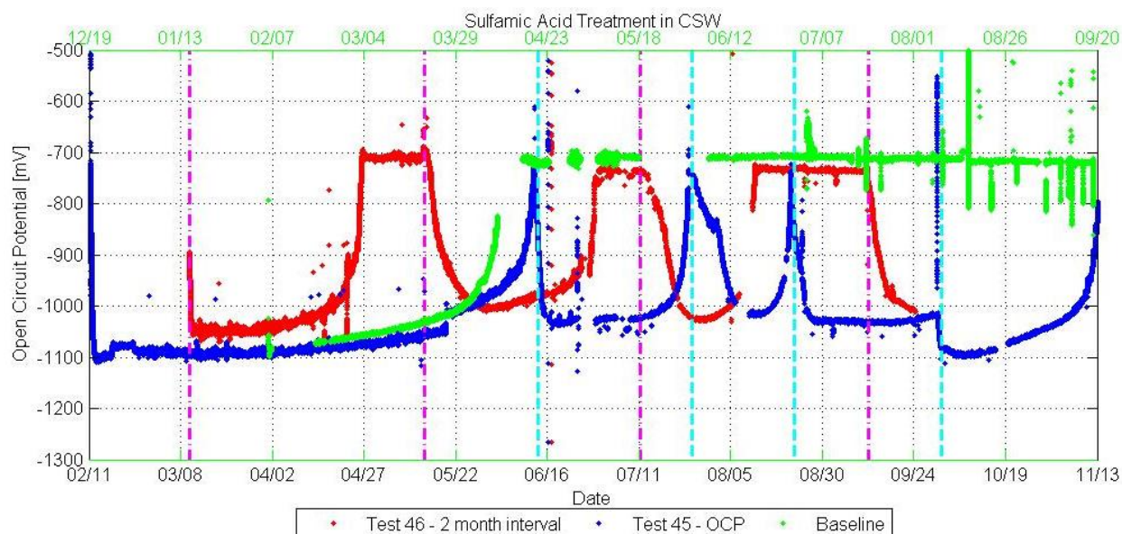
Figure 4-13. Sulfamic acid treatment in CSW. Test 46 2-month treatment dates are indicated by magenta lines and Test 45 OCP-based treatment dates are indicated by cyan lines. Only the first 275 days of exposure are shown for the baseline coupon (actual date is on upper x-axis in green). Treatments have been successful in lowering OCP to \sim -1000 mV. Test 45 was in stagnant fresh water for several hours due to a flow disruption on 10/1/14.
