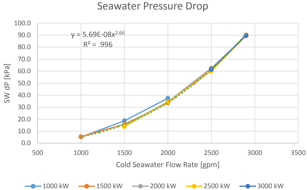
Figure 3-4. Seawater-side pressure drop
