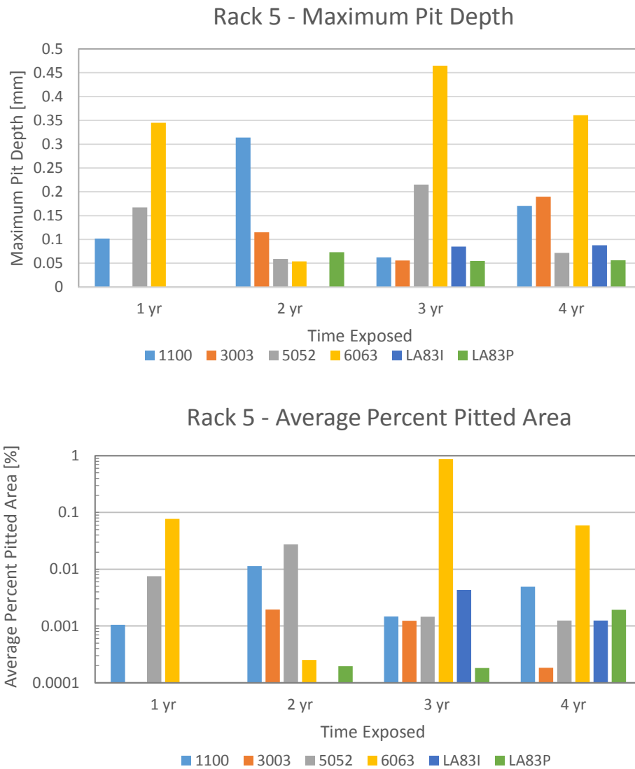
Figure 4-9. Maximum pit depth and average percent pitted area (per alloy, per exposure time) for WSW pre-treated samples exposed to CSW.
