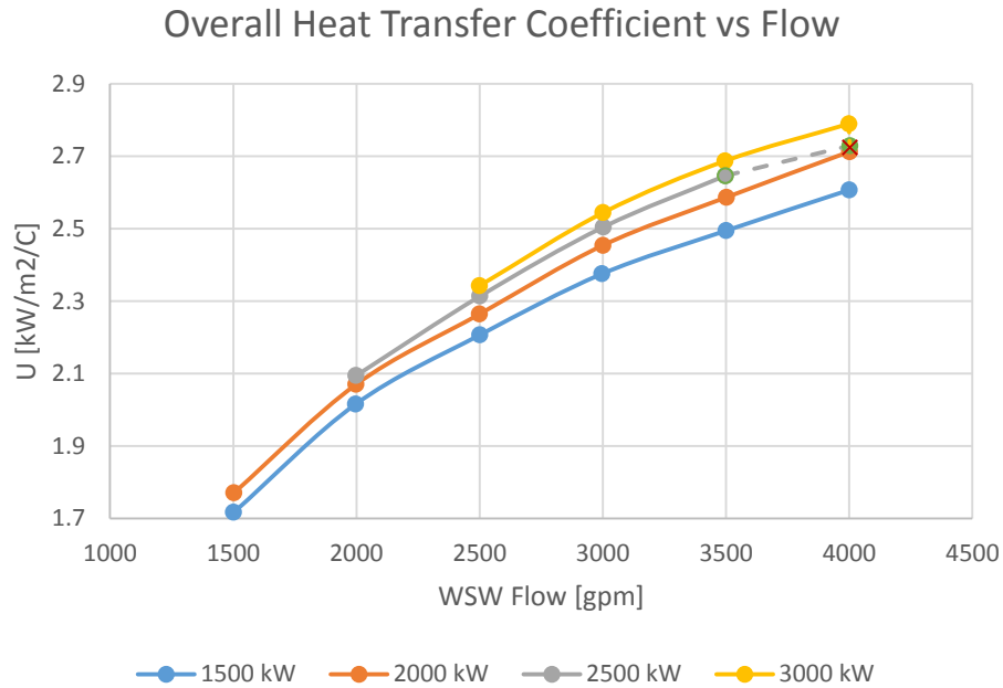
Figure 3-10. Overall heat transfer coefficient
