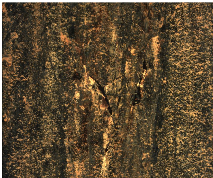
Figure 4-12. Corrosion product beginning to flake on a steel sample tested in the CSW MCIR.
