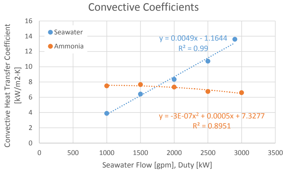
Figure 3-3. Ammonia and seawater convective heat transfer coefficients fitting the equation 1/U = 1/h_{sw} + dx_w/k + 1/h_{NH3} solved for using the least-squares method.
