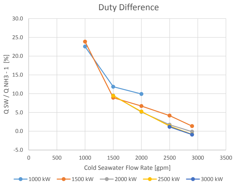
Figure 3-8. Difference between ammonia duty and seawater duty
