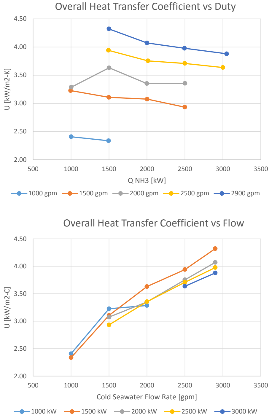
Figure 3-2. Condenser overall heat transfer coefficient
