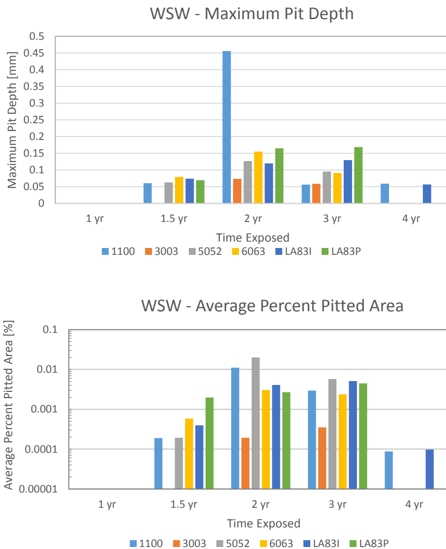
Figure 4-1. Maximum pit depth and average percent pitted area (per alloy, per exposure time) for samples exposed to WSW. There are no scan data for 1-yr exposure samples of Alloys 1100, 3003, 5052, LA83I and LA83P.
