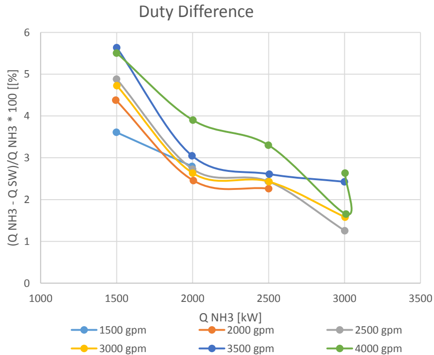
Figure 3-16. Difference between ammonia duty and seawater duty
