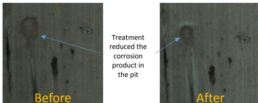
Figure 4-14. Before and after sulfamic treatment. Corrosion product buildup was lessened in this pit, but result was not observed for all pits.
