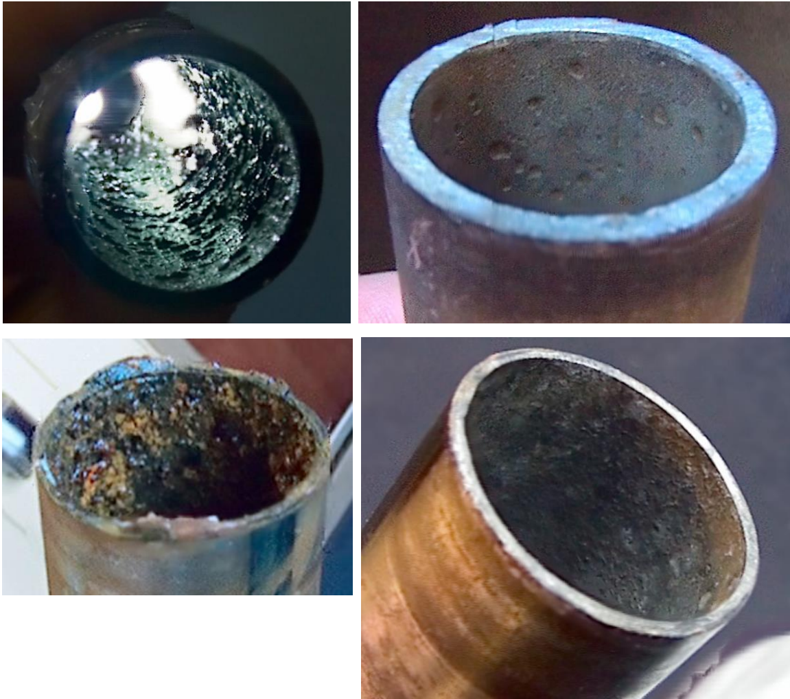
Figure 4-11. Certified steel sample after six months in CSW post-removal (top left) and post-processing (top right). Non-certified steel sample after one year in CSW post-removal (bottom left) and post-processing (bottom right). Post-processing reveals a relatively smooth wall with large shallow pits in the certified steel sample and a rough wall with few visible pits in the non-certified steel sample.
