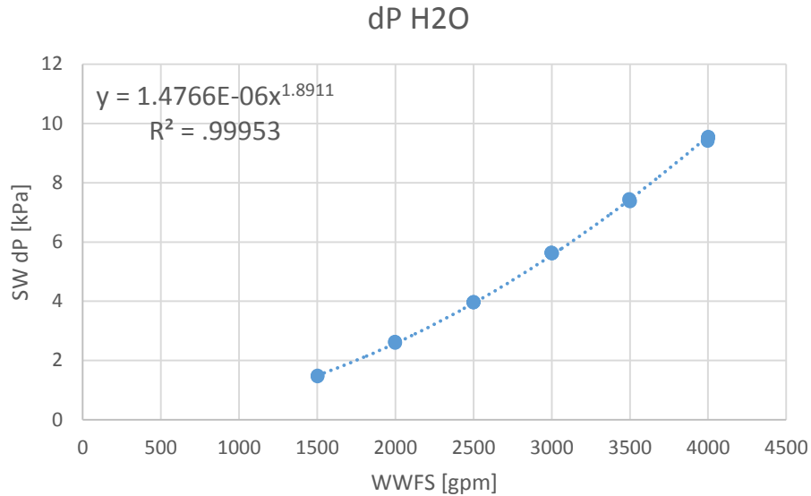
Figure 3-12. Seawater-side pressure drop
