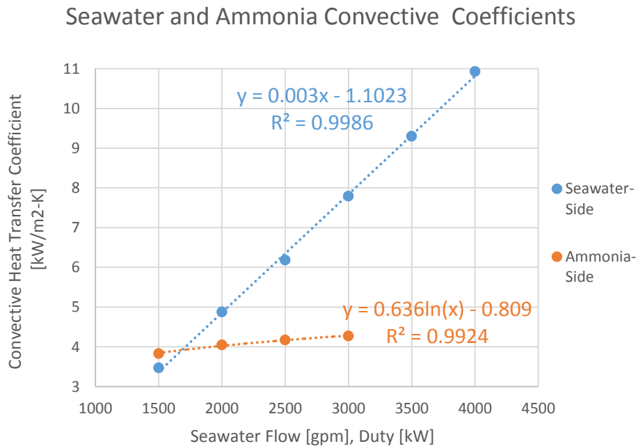
Figure 3-11. Ammonia and seawater convective heat transfer coefficients fitting the equation 1/U = 1/h_{sw} + dx_w/k + 1/h_{NH3} solved for using the least-squares method.
