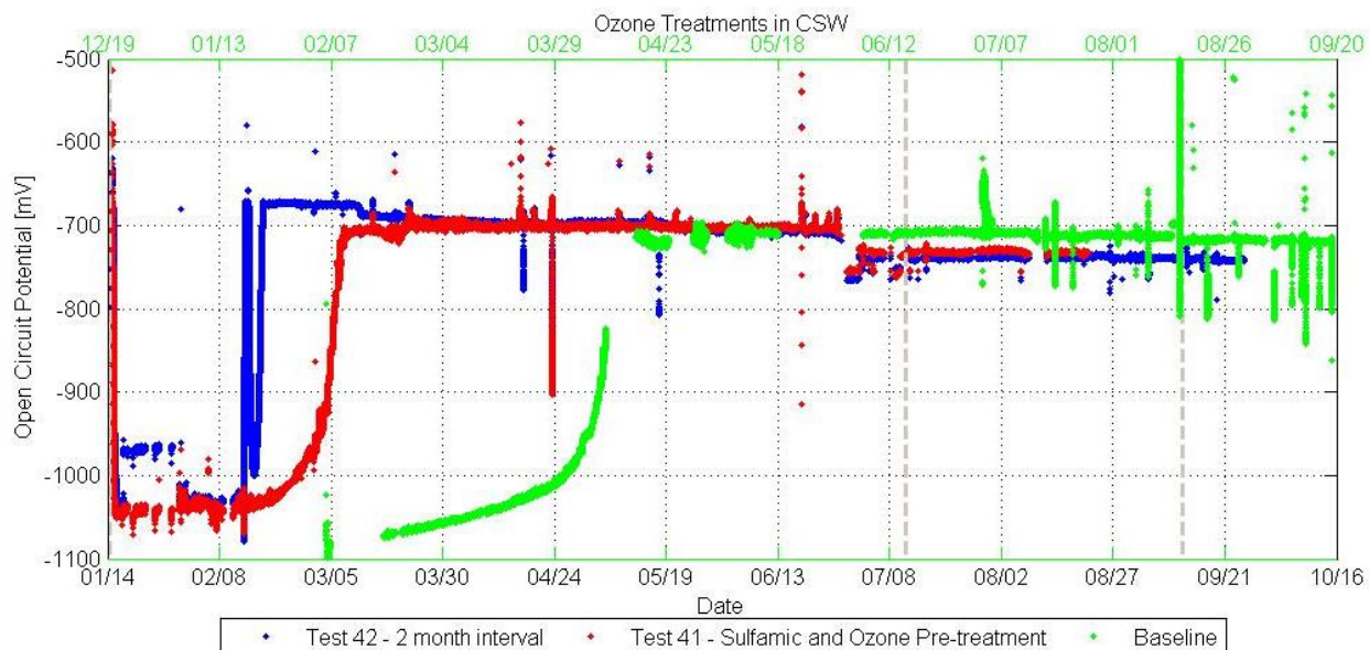
Figure 4-18. OCP of ozone treated samples reached steady-state 70 days (Test 41) and 90 days (Test 42) before the baseline sample. Ozone treatment dates for Test 42 are indicated by vertical gray lines. Treatments were planned but not performed on 3/10/2014 and 5/13/2014. Small pits were observed on 2/25/2014. Only first 275 days of exposure are shown for the baseline coupon (actual date is on upper x-axis in green). Test 41 was removed on 8/20/2014 and Test 42 was removed on 9/24/14.
