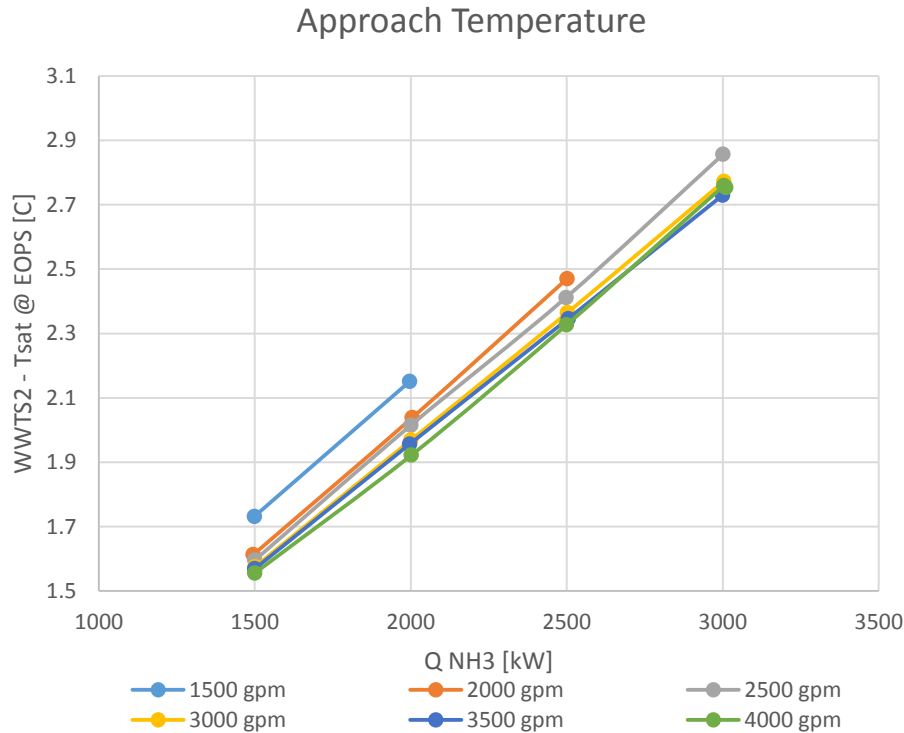
Figure 3-17. Approach temperature
