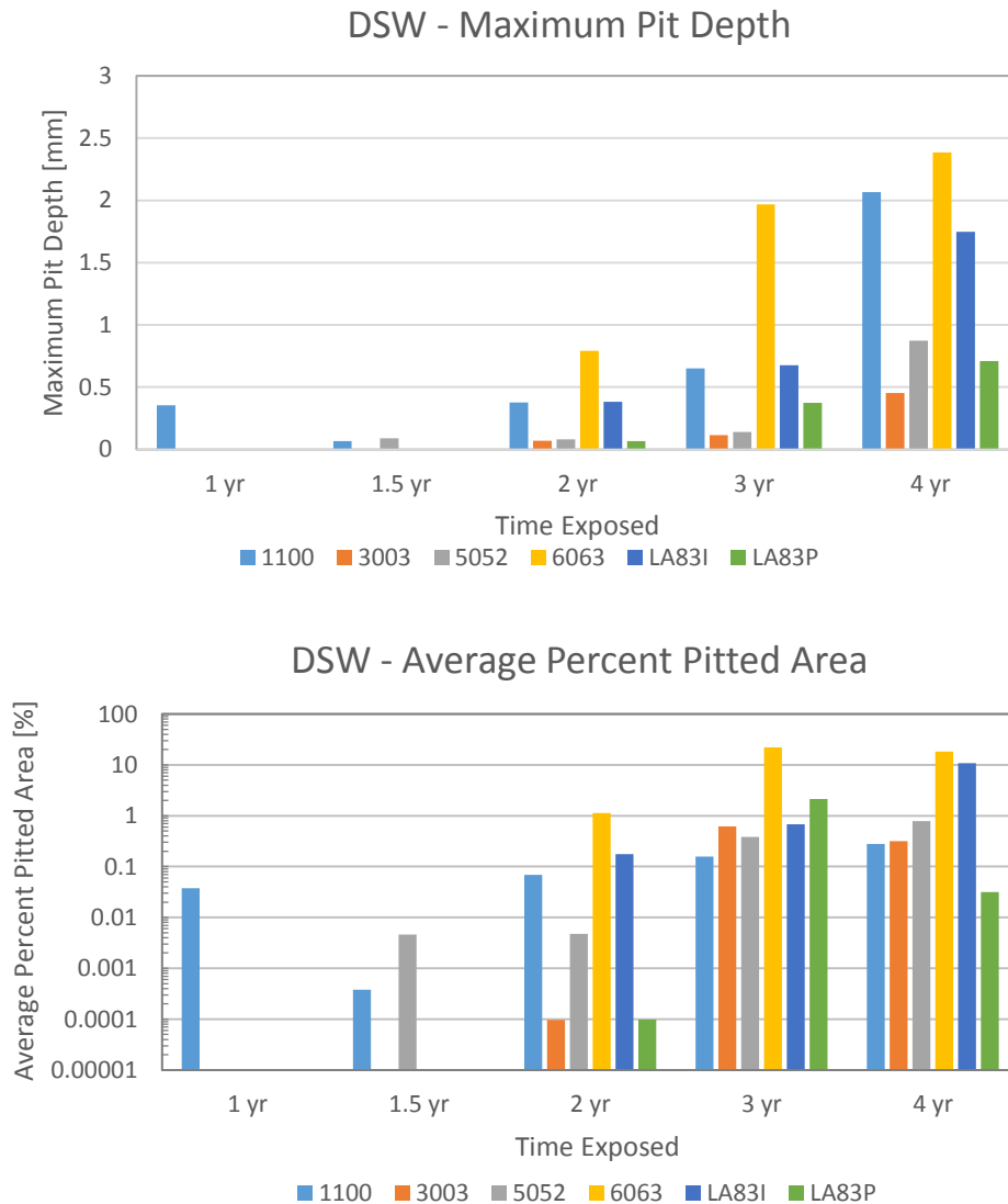
Figure 4-7. Maximum pit depth and average percent pitted area (per alloy, per exposure time) for samples exposed to DSW. Pits were prevalent on DSW samples. Only Alloy 1100 1-year samples were scanned. No profilometer data is reported for the 1-year samples of the other alloys. (No pits were observed, only two of Alloy 5052 samples had small blisters but no pit craters). Many of the 4-year samples had pits on the edges and sides of the coupon that could not be captured in the profilometer scans.
