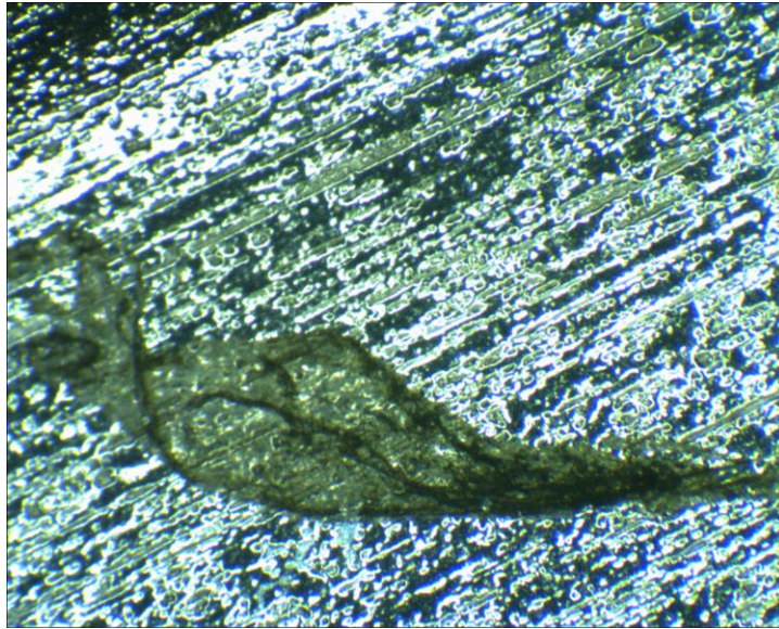
Figure 4-3. Pitted area identified in profilometer scan on LA83I-35. Under microscope inspection, the area does not display characteristics of pitting, rather the surface appears gouged or eroded.
