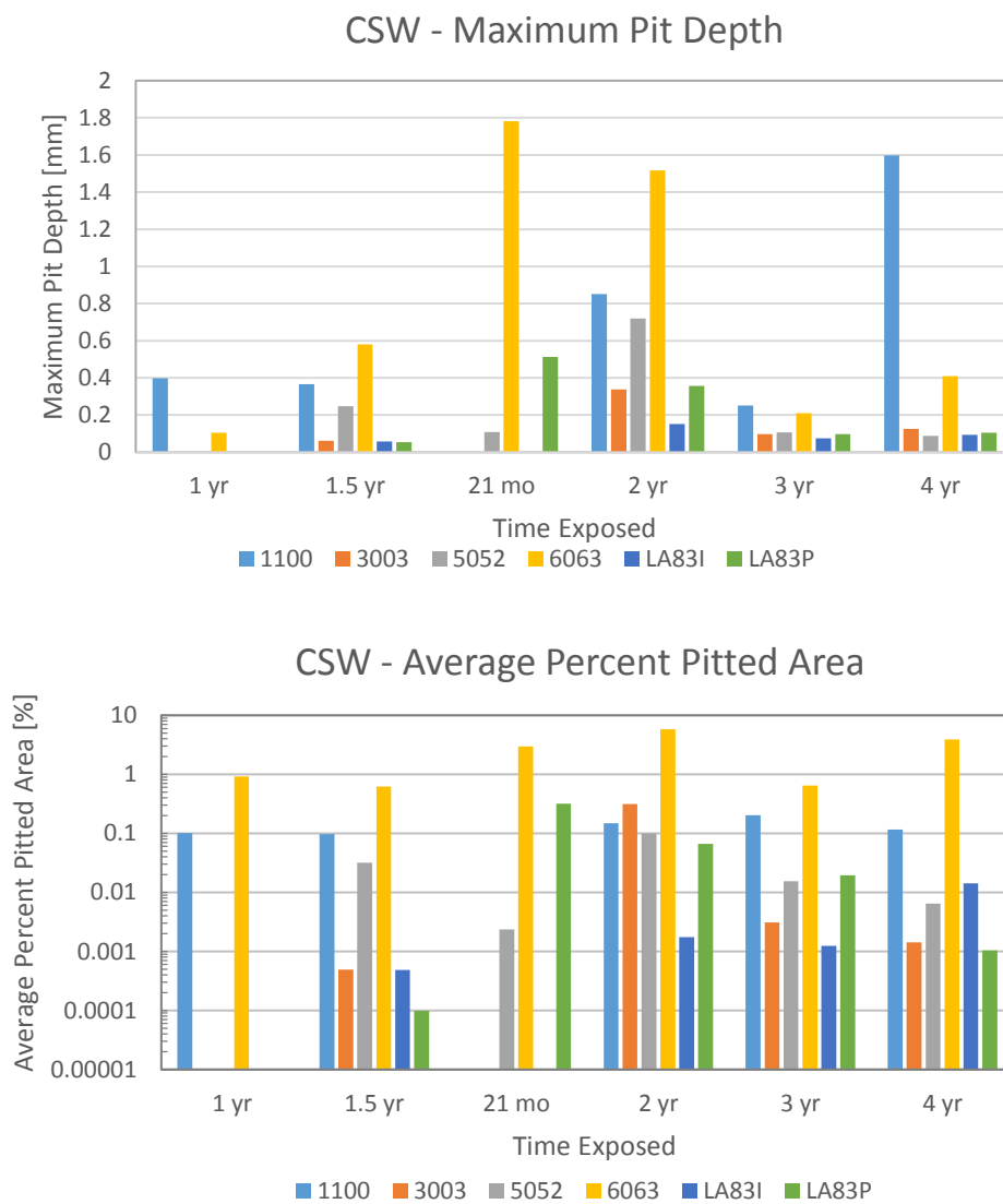
Figure 4-4. Maximum pit depth and average percent pitted area (per alloy, per exposure time) for samples exposed to CSW. There are no scan data for 1-yr exposure of Alloys 3003, 5052, LA83I, and LA83P and 21-month exposure of Alloys 1100, 3003, and LA83I.
