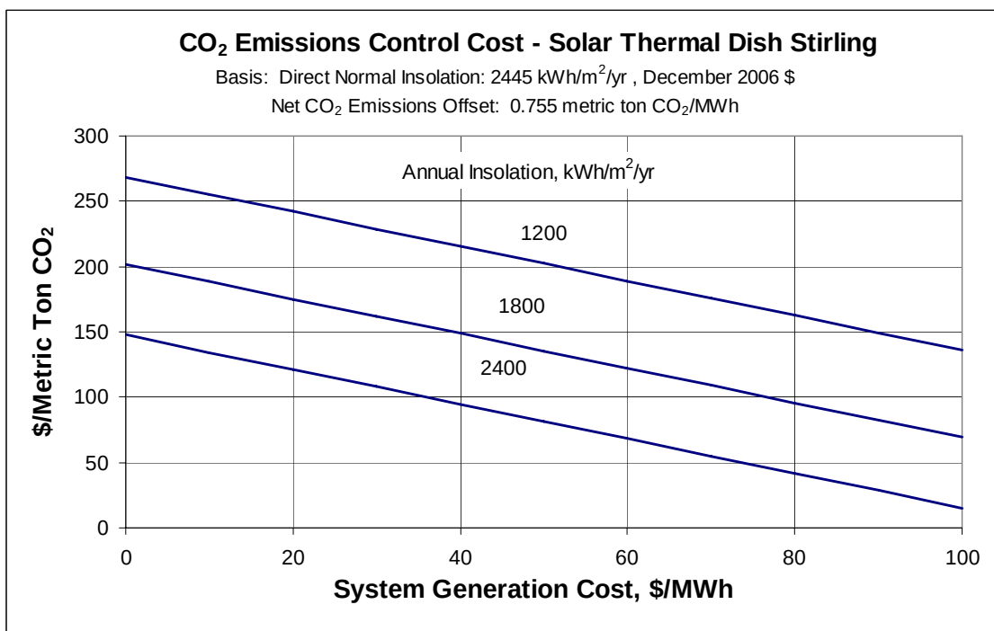
Figure 11-9 Levelized CO 2 Emissions Control Cost vs. Annual Insolation (Top) and System Generation Cost (Bottom) for an 80-MW Solar Thermal Dish Stirling Engine Power Plant (Dec-06 $)
