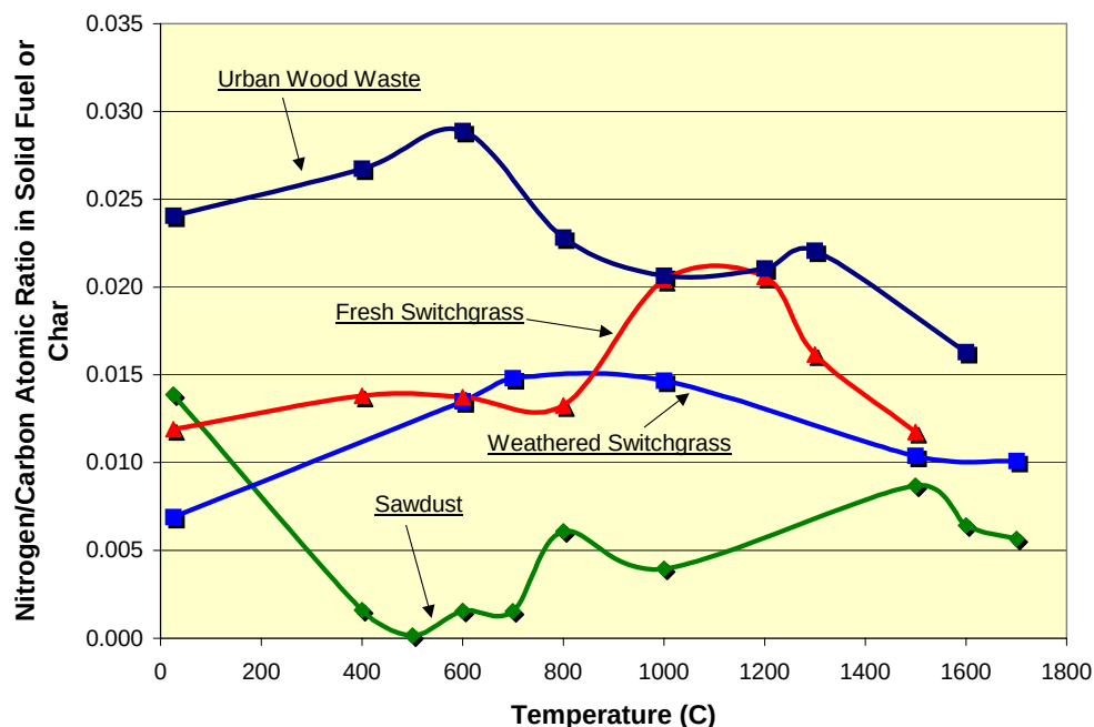
Figure 4-18 Nitrogen/Carbon Atomic Ratios for Biomass Chars Formed During DTR Pyrolysis at Various Temperatures
