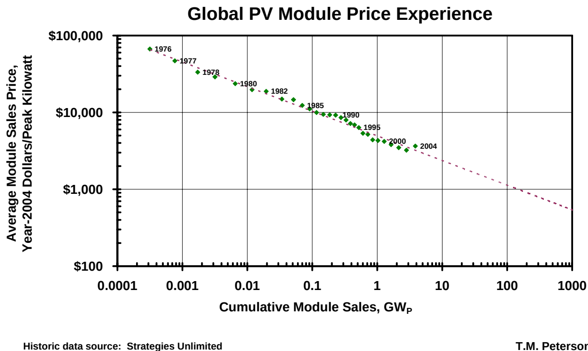
Figure 5-2 Worldwide Average PV Module Selling Price vs. Cumulative Sales
