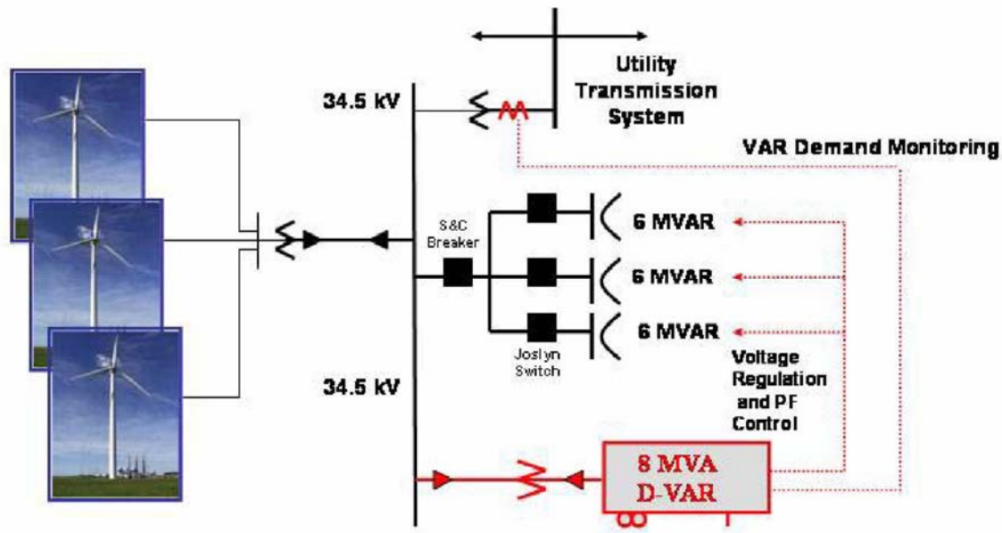
Figure 10-13 Conceptual Layout of a Dynamic VAR Device and Switched Capacitors Supporting a Wind Farm (Source: American Superconductor)
