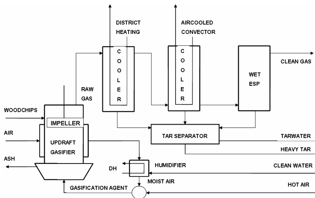
Figure 4-34 Process Flow Diagram for the Vølund Gasifier at Harboøre
