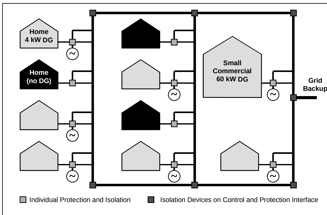
Figure 5-3 Schematic of a Simple Microgrid System
