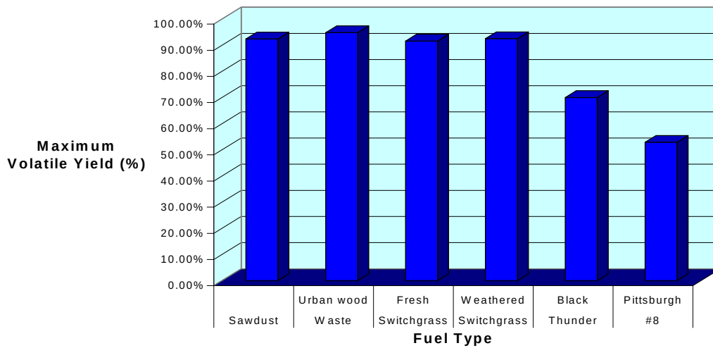
Figure 4-1 Maximum Volatile Yield of Biomass Fuels Compared to Reference Coals (sources: Johnson et al., 2001; Johnson et al., 2002)
