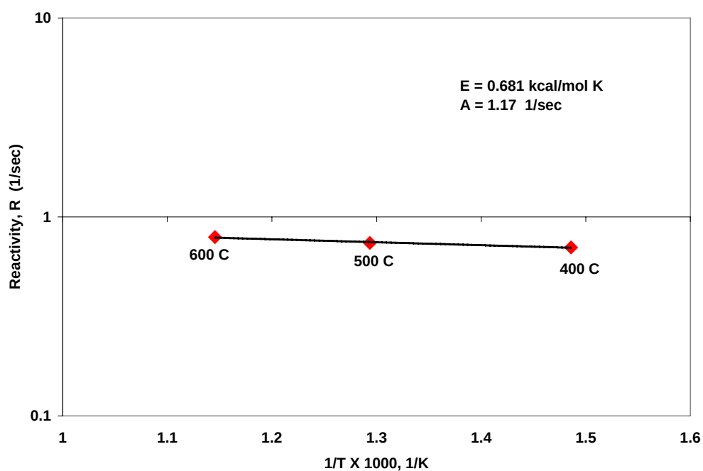
Figure 4-2 Low-Temperature Devolatilization Kinetics for Fresh Sawdust (Source: Johnson et al., 2001)
