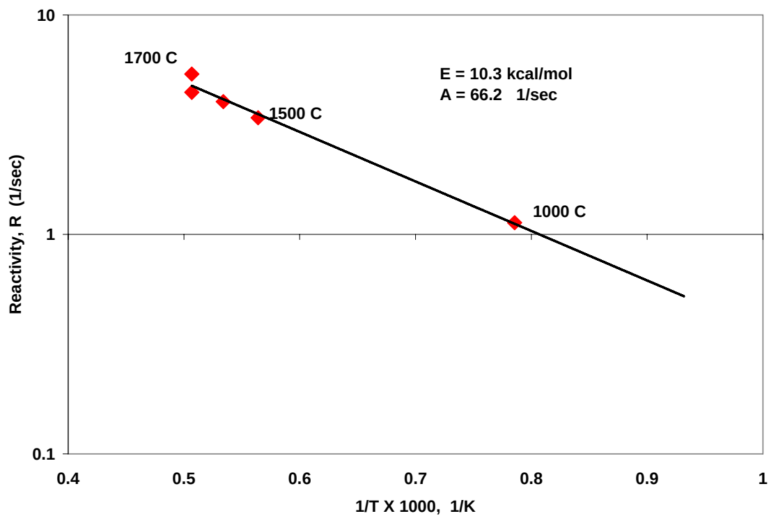
Figure 4-8 Devolatilization Kinetics for Pittsburgh Seam #8 Coal (Source: Johnson et al., 2001)
