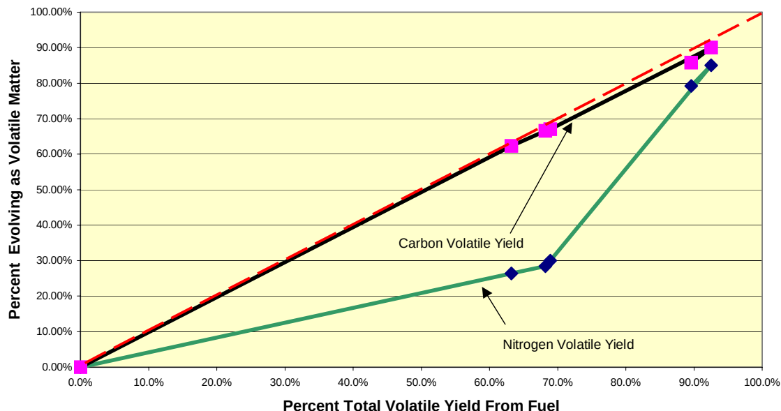
Figure 4-17 Nitrogen and Carbon Volatile Evolution from Weathered Switchgrass Normalized to Total Volatile Evolution
