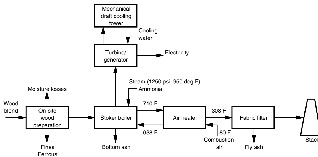
Figure 4-29 Schematic of Biomass-Fired Stoker Boiler Power Plant
