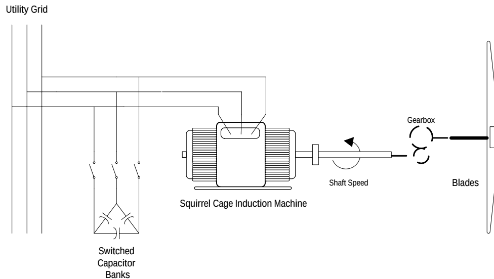
Figure 10-2 Constant-Speed Induction Machine-Connected Wind Turbine Generator with Gear Box
