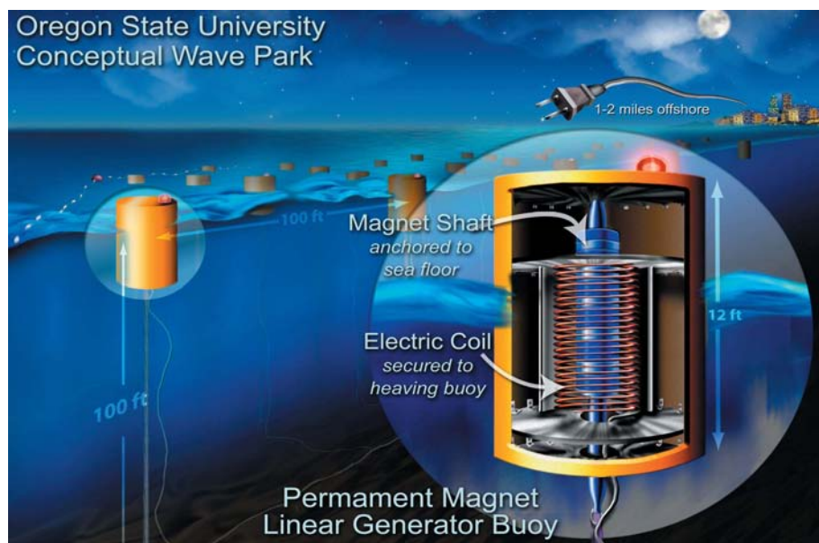
Figure 9-14 Permanent Magnet Linear Generator in a Conceptual Wave Park Vision
