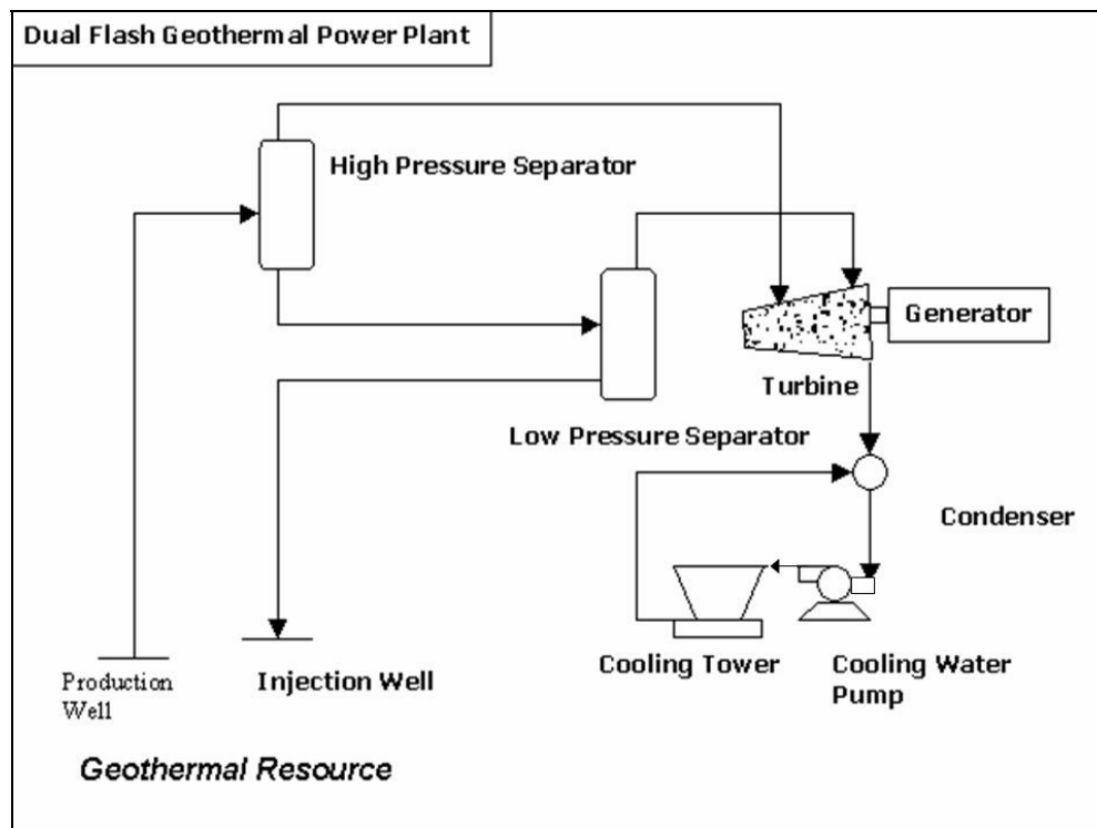
Figure 6-4 Dual-Flash (two-flash) Geothermal Power Plant
