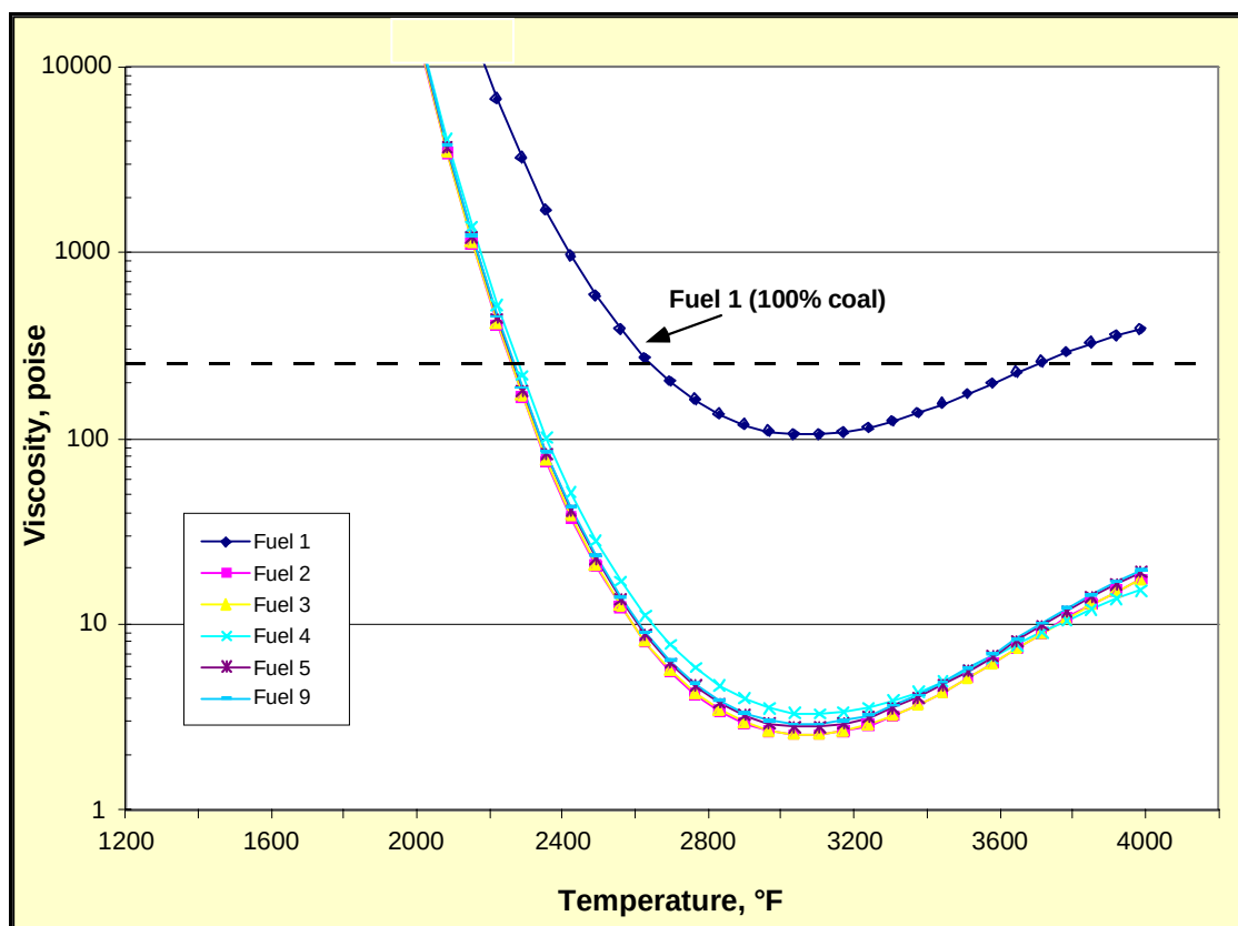
Figure 4-25 The Influence of Cofiring on Slag Viscosity. Fuels 2 to 9 are various cofiring scenarios using woody biomass, herbaceous biomass, and animal manures with eastern bituminous coals (Source: Miller et al., 2002).
