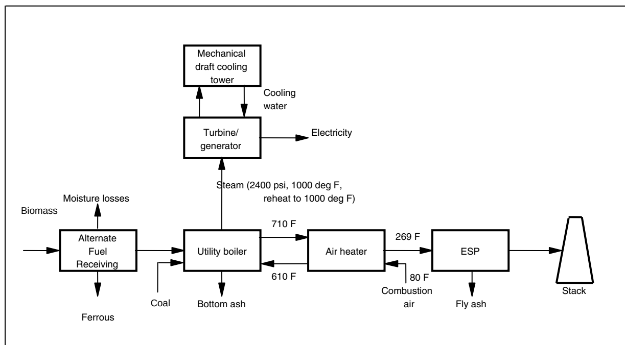
Figure 4-20 Schematic of Biomass Cofiring with Coal in a Utility Boiler
