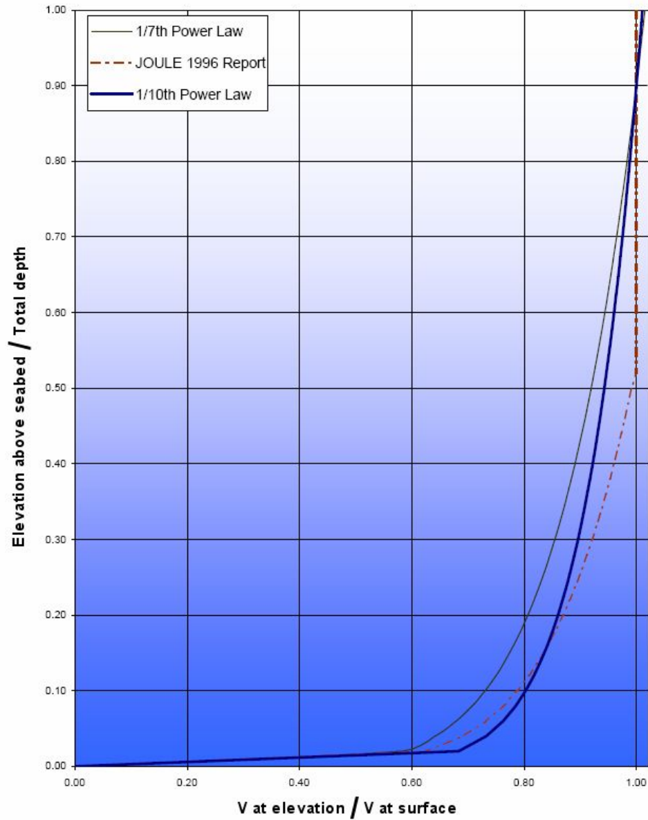
Figure 8-16 Alternative Profile Formulations of Velocity Variability with Depth (1/10th-Power Law used)
