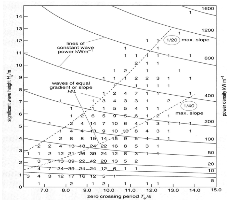
Figure 9-10 Statistical Wave Distribution Matrix and Lines of Constant Wave Power and Gradient
