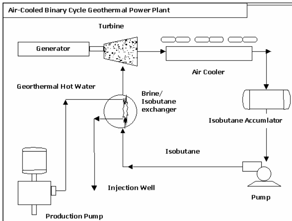
Figure 6-5 Binary Cycle Geothermal Power Plant (air-cooled design)
