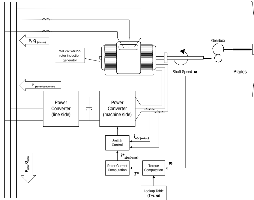
Figure 10-4 Variable-Speed Doubly-Fed Induction Machine Connected WTG with Gear Box
