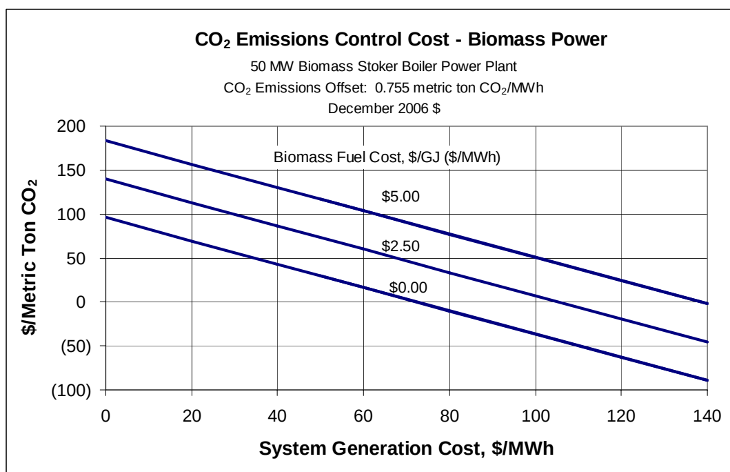
Figure 11-5 Levelized CO 2 Emissions Control Cost vs. Delivered Fuel Cost (Top) and System Generation Cost (Bottom) for a 50-MW Stoker Boiler Biomass Power Plant (Dec-2006 $)
