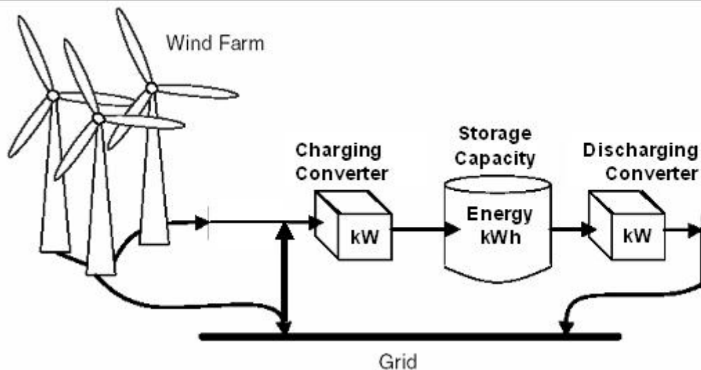
Figure 10-18 Model for Evaluation of Energy Storage with Wind Power
