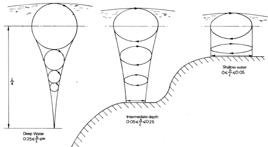
Figure 9-2 Particle Motion in Different Water Depths
