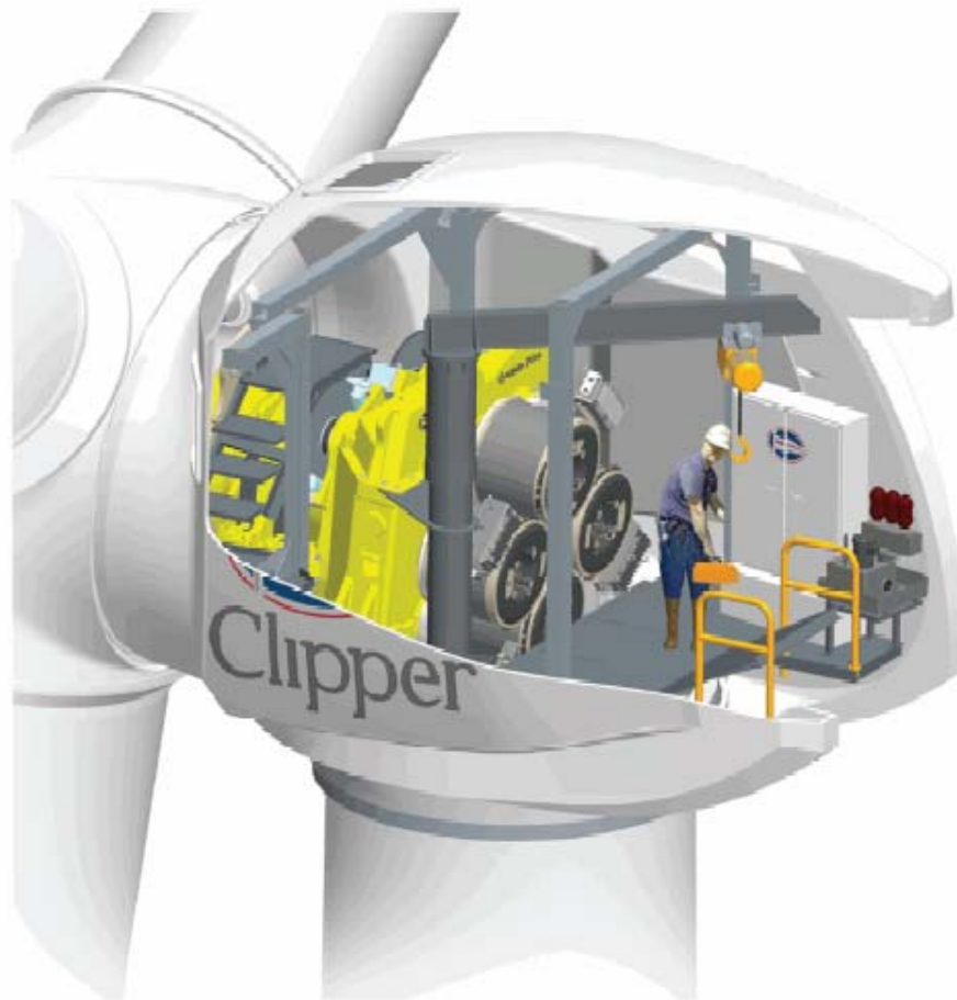
Figure 3-6 Clipper Windpower's 2.5 MW Liberty Series Wind Turbine Nacelle, with Four Modular Permanent-Magnet Generators and Integral (Source: Clipper Windpower Inc.)
