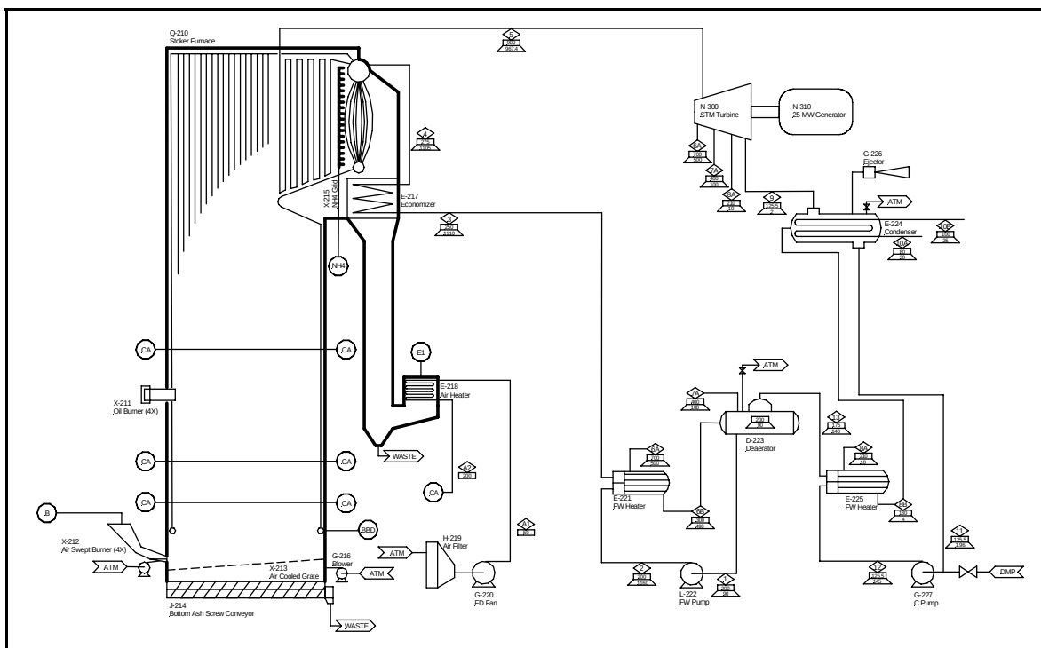
Figure 4-30 Typical Boiler and Turbine-Generator Approach
