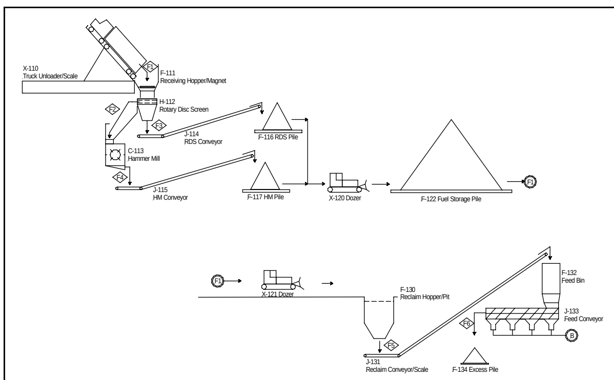
Figure 4-28 Representative Wood Fuel Handling System
