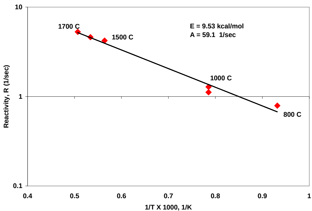
Figure 4-7 Devolatilization Kinetics for Black Thunder PRB Coal (Source: Johnson et al., 2001)
