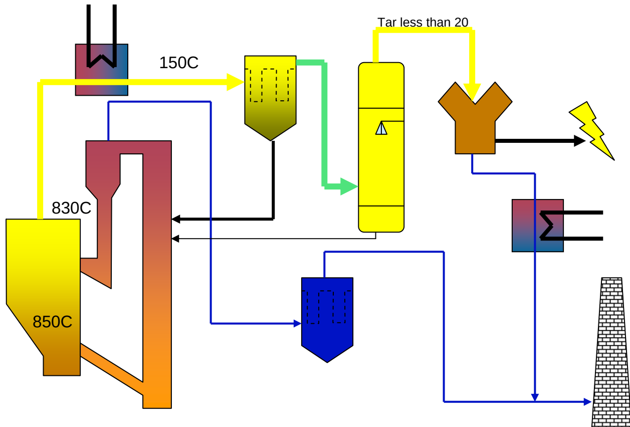
Figure 4-33 Schematic of Biomass Gasification Application for Combined Heat and Power
