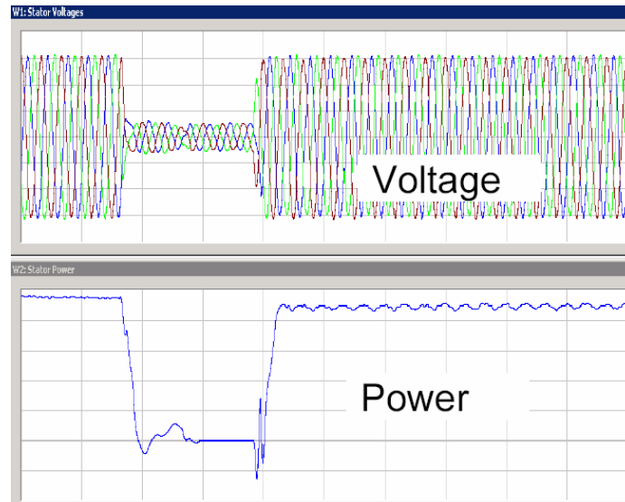
Figure 10-8 A Severe Voltage Sag to Less Than 30% Voltage Remaining Voltage for 100 ms (Upper Trace) and Wind Turbine with LVRT Recovering After the Event (Lower Trace)
