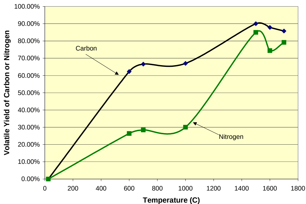
Figure 4-15 Volatile Nitrogen and Carbon Evolution from Weathered Switchgrass
