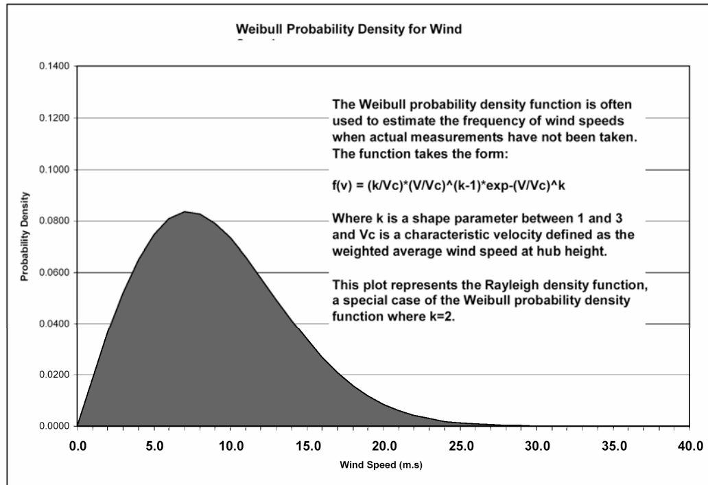
Figure 3-4 Rayleigh Probability Density Function for Wind Speed
