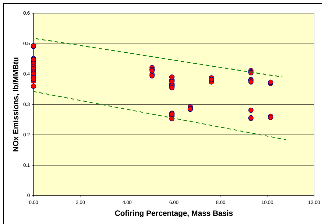
Figure 4-27 \text{NO}_x Reduction at the Albright Generating Station Test Program
