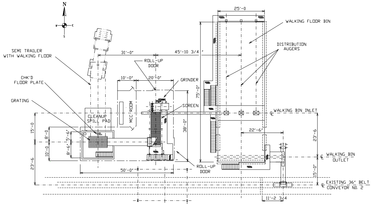
Figure 4-21 Plan View of the Willow Island Biomass Cofiring System
