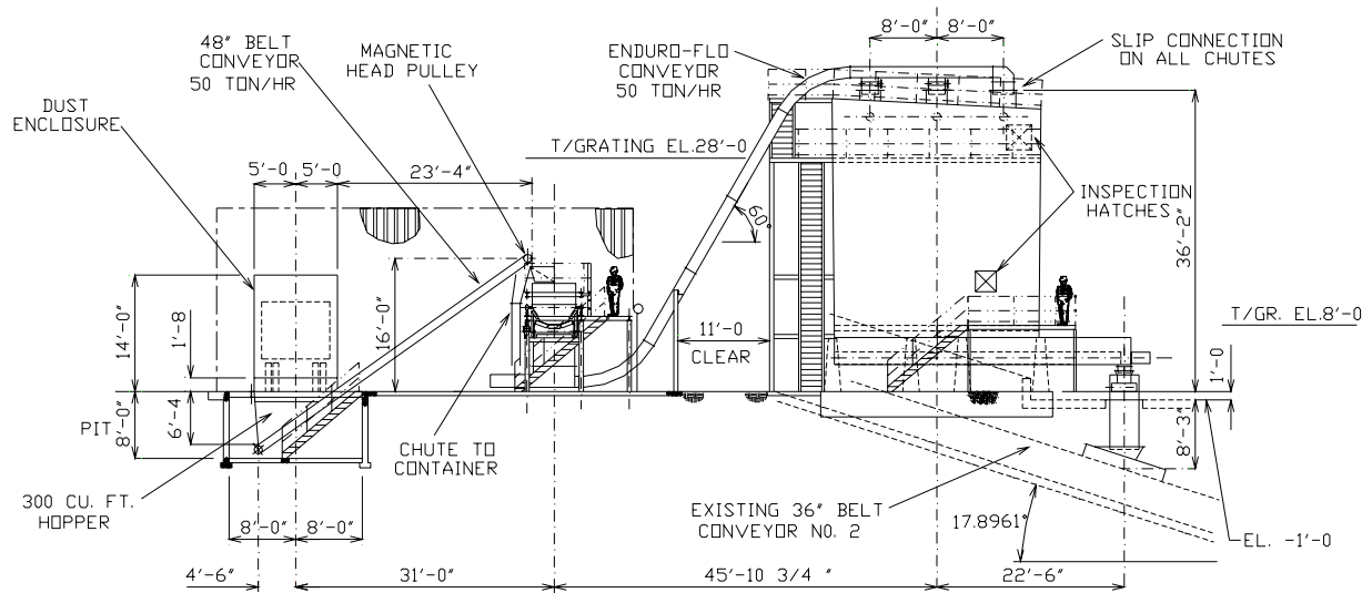
Figure 4-22 Elevation View of the Willow Island Biomass Cofiring System
