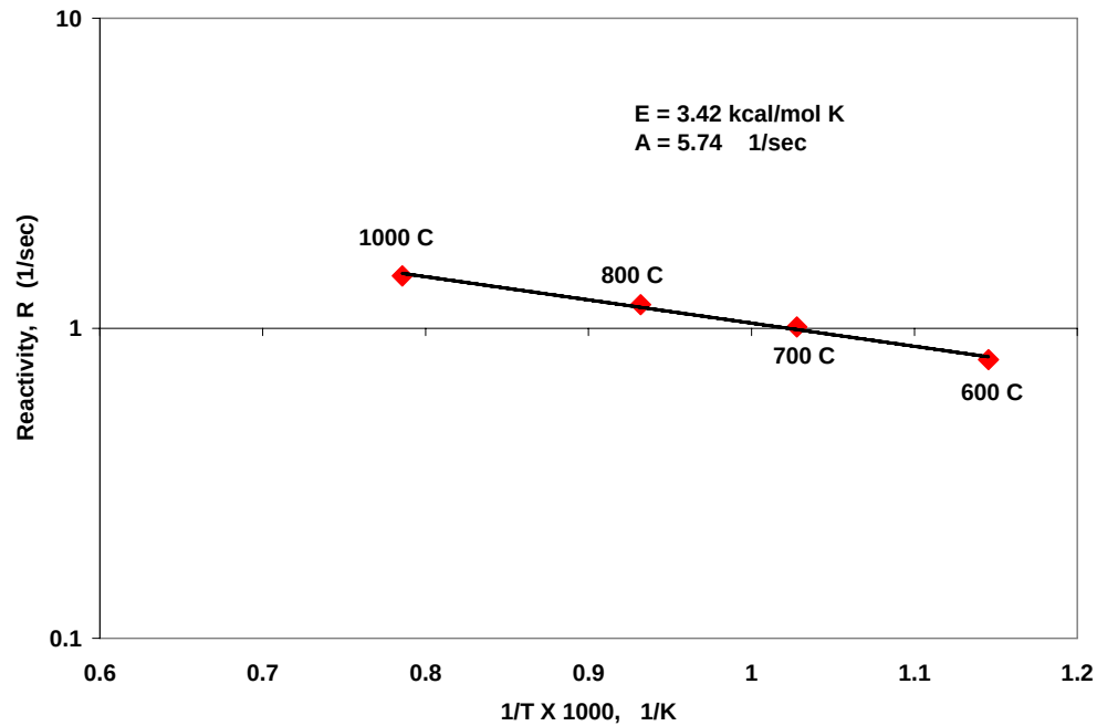
Figure 4-3 High-Temperature Devolatilization Kinetics for Fresh Sawdust (Source: Johnson et al., 2001)
