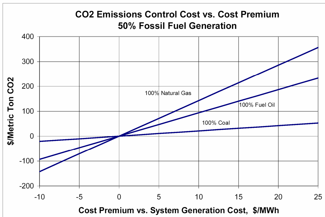
Figure 11-3 Levelized CO 2 Emissions Control Cost vs. Cost Premium and Fossil Fuel Mix at 50% Generation from Fossil Fuels
