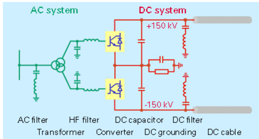
Figure 10-7 One Leg, Single-Line Diagram of 12-Pulse HVDC System (Source: Siemens)
