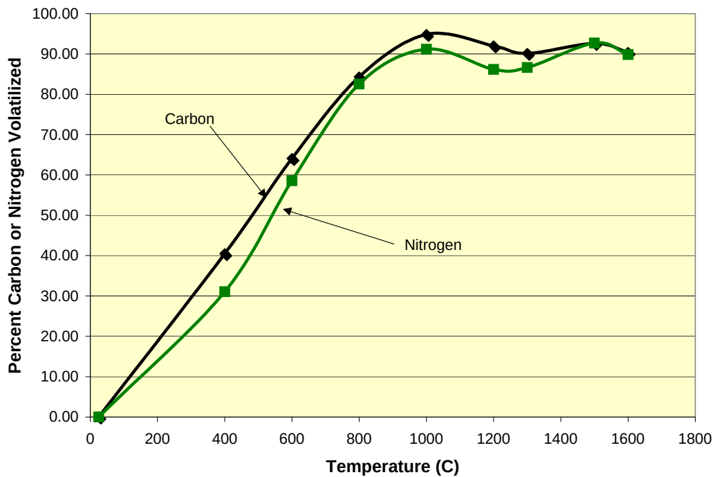
Figure 4-14 Volatile Nitrogen and Carbon Evolution from Fresh Switchgrass
