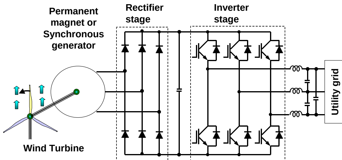
Figure 10-6 Direct-Drive Synchronous Generator with Simple Rectifier at the WTG and Voltage-Source Converter Interface With the Utility Grid
