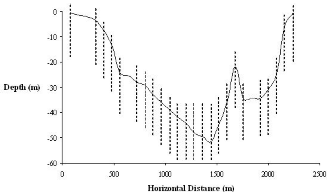
Figure 8-17 Cross-Section of Tidal Channel (dotted lines show section boundaries)
