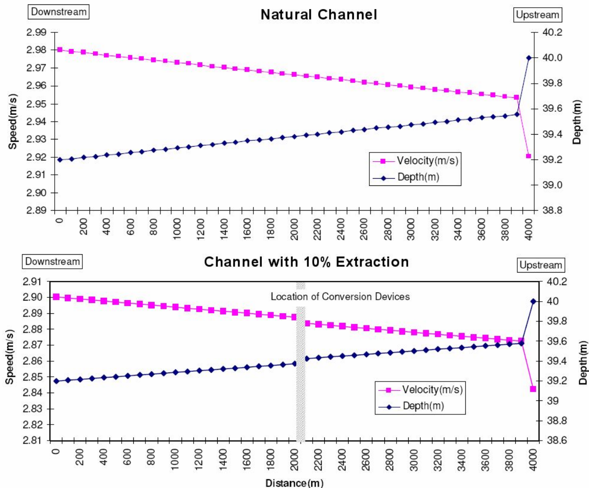
Figure 8-20 Influence of Energy Extraction on Flow in a Tidal Channel
