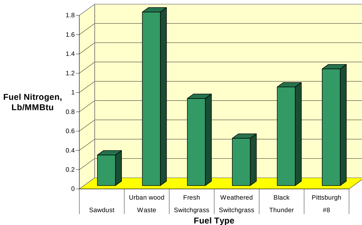
Figure 4-9 Fuel Nitrogen Concentrations for the Fuel Samples Analyzed in Detail (Source: Johnson et al., 2001; Johnson et al., 2002)
