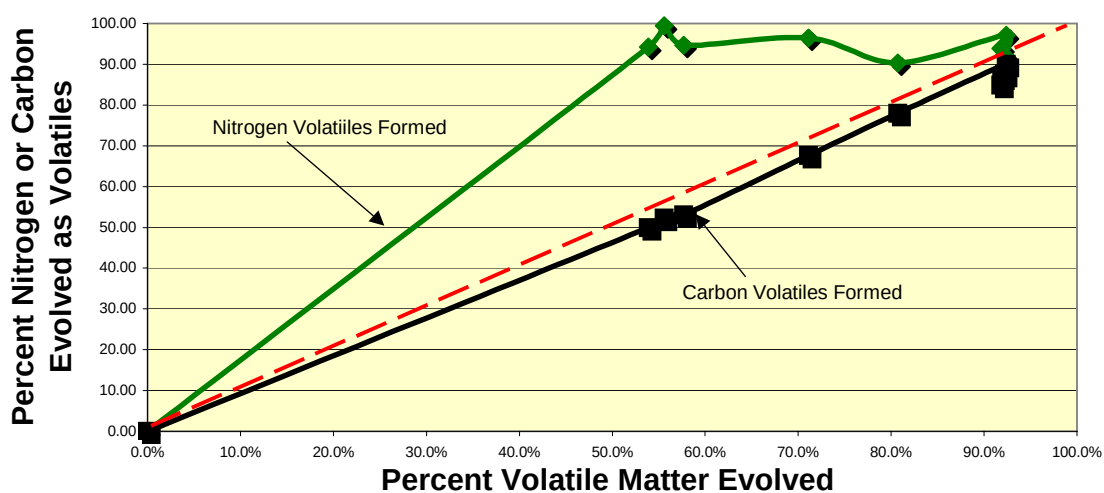
Figure 4-16 Nitrogen and Carbon Volatilization Normalized to Total Volatiles Formed from Sawdust
