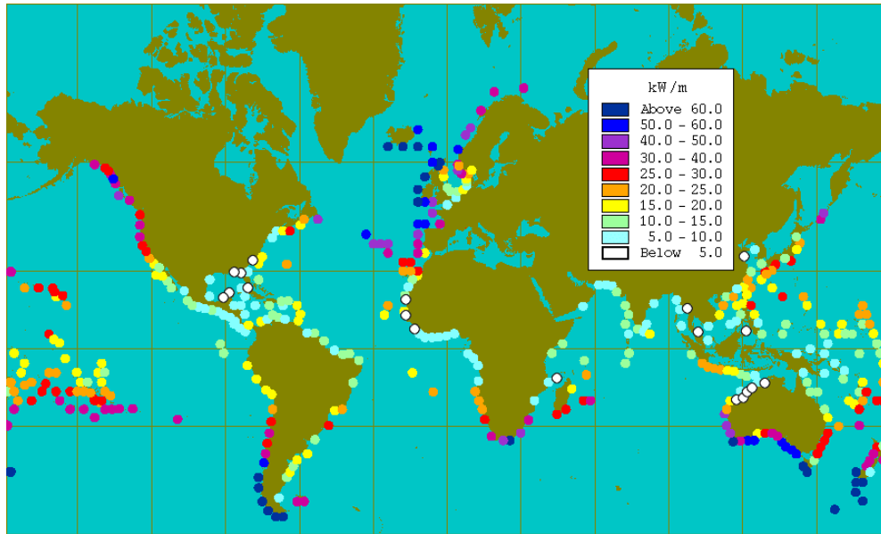
Figure 9-12 Annual Wave Power Averages Worldwide in kW/m Wave Front
