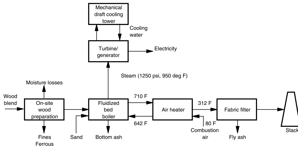
Figure 4-31 Schematic of Biomass-Fired Atmospheric Fluidized Boiler Power Plant
