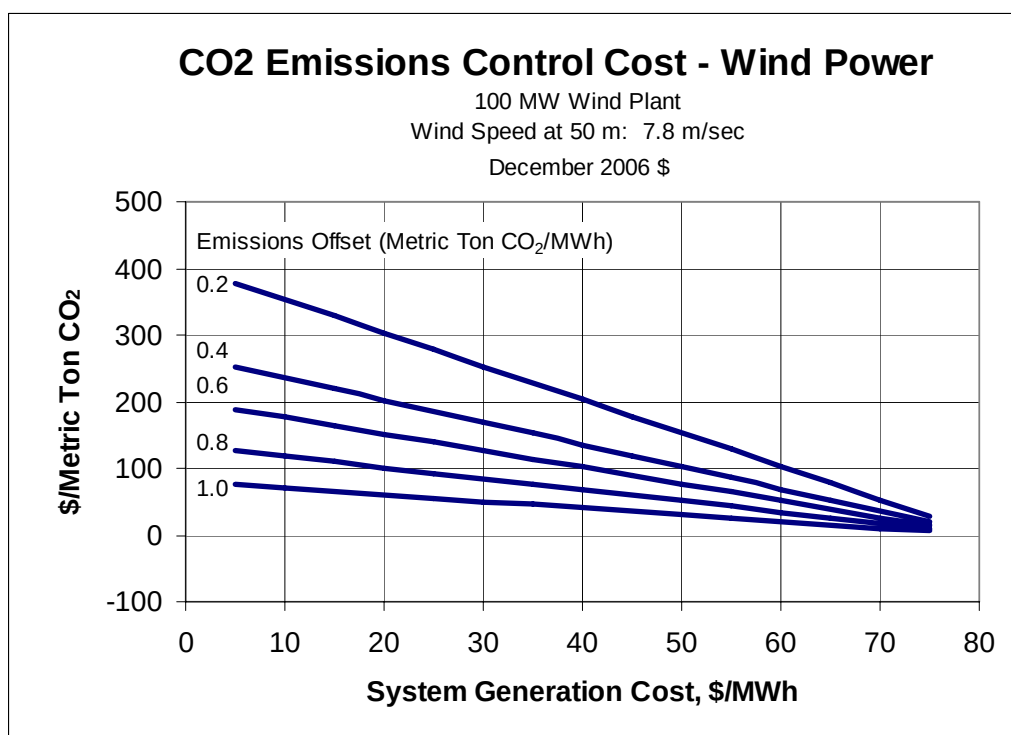
Figure 11-4 Levelized CO 2 Emissions Control Cost vs. Average Wind Speed at 50 m (top) and System Generation Cost (Bottom) for a 100-MW Wind Plant (Dec 2006 $)
