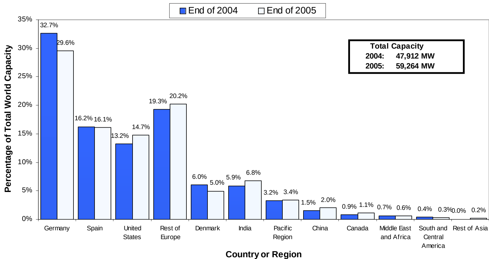
Figure 3-2 End-of-Year Operating Wind Capacity by Country and Region: 2004 and 2005 (Source: BTM Consult ApS, March 2005).
