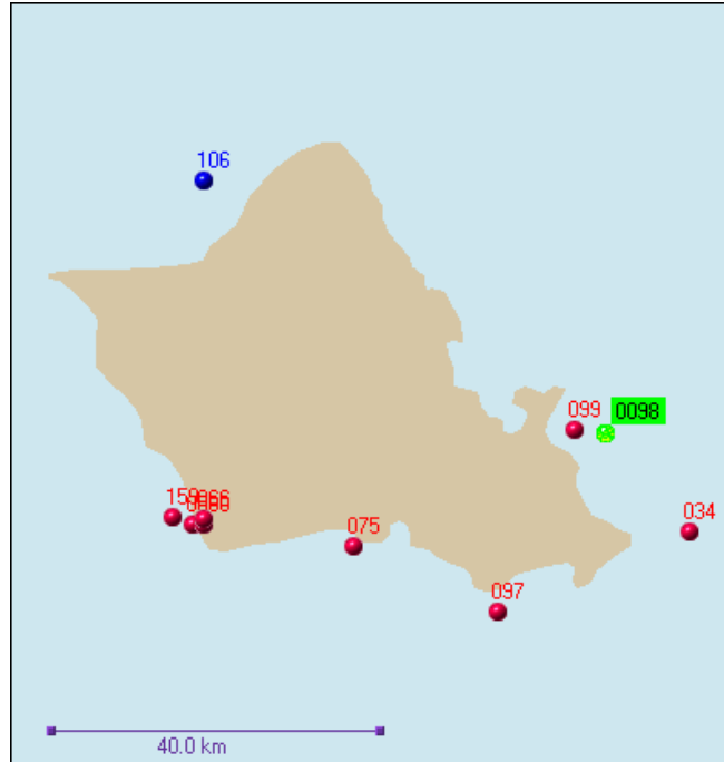
Figure 9-6 Oahu HI Reference Station, (CDIP 0098 is green circle)
