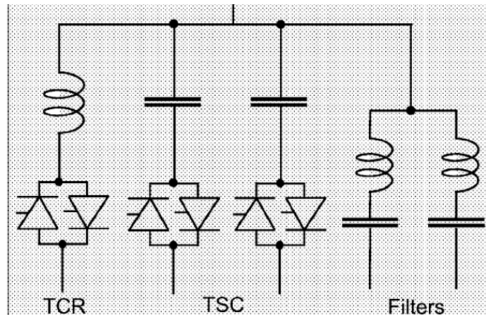
Figure 10-14 Simplified Schematic of a Static VAR (SVC) or Distribution Static Var Compensator (DSVC)
