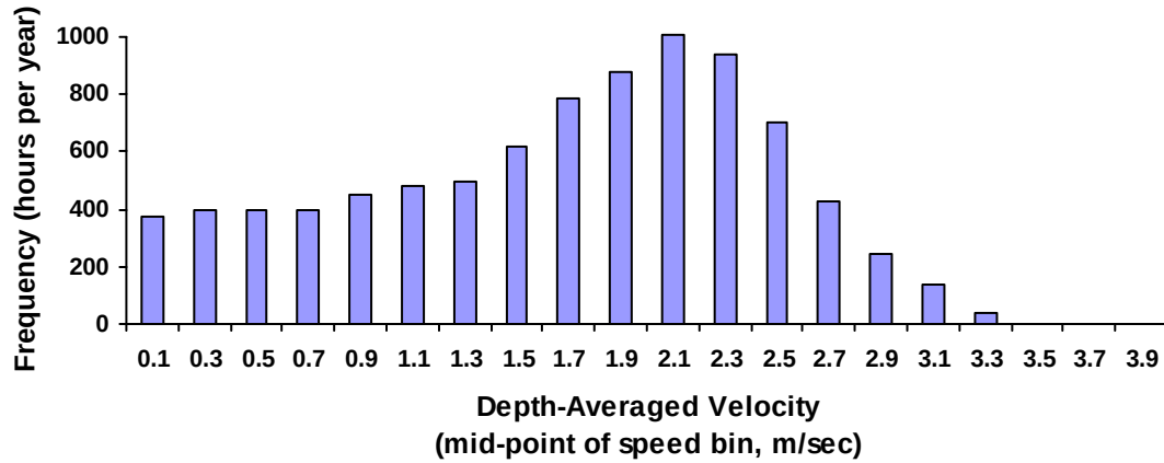
Figure 8-12 Annual Average Tidal Current Speed Probability Distributions for Dog Island transect, Western Passage, ME (East Coast)
