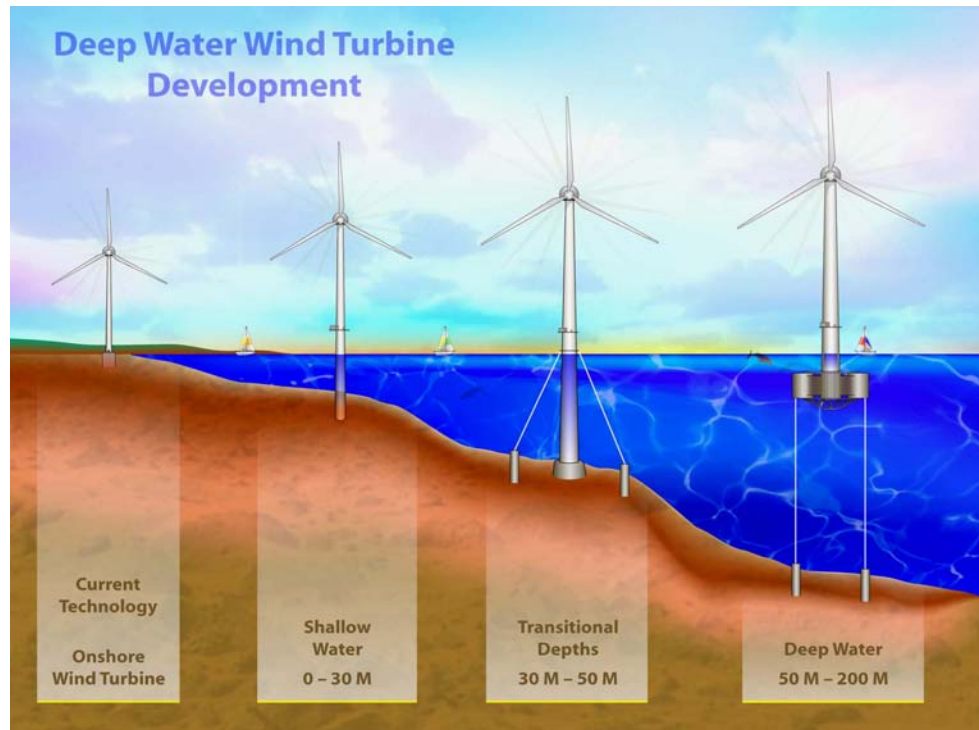
Figure 3-15 Progression of Expected Wind Turbine Evolution to Deeper Water (Source: Musial and Butterfield, NREL/U.S. DOE, 2004)
