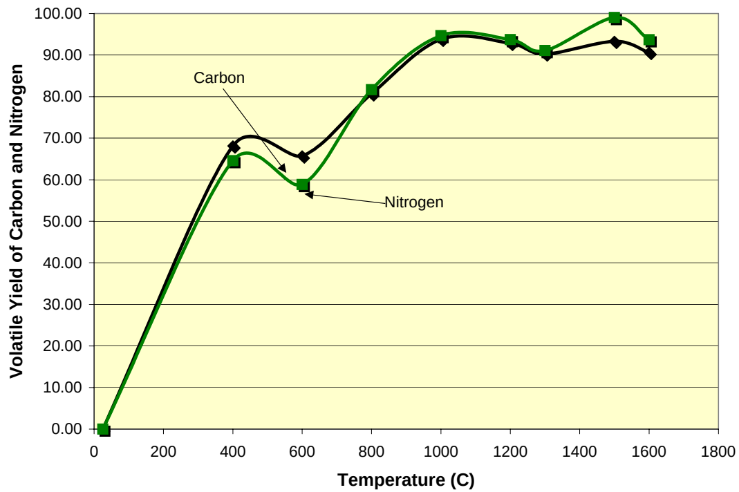
Figure 4-13 Volatile Nitrogen and Carbon Evolution from Urban Wood Waste
