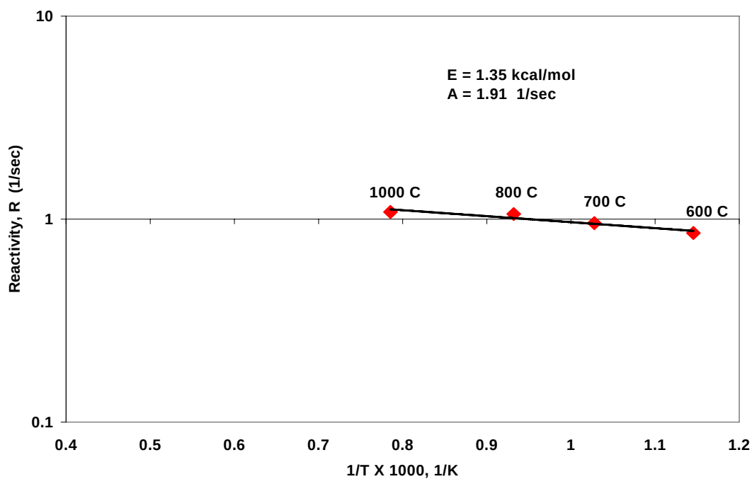
Figure 4-6 Devolatilization Kinetics for Weathered Switchgrass (Source: Johnson et al., 2001)
