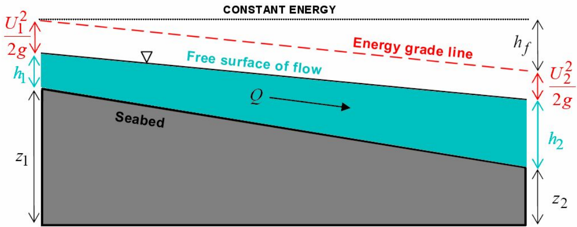
Figure 8-15 Open-Channel Flow Theory: Energy Equation and Definition Sketch
