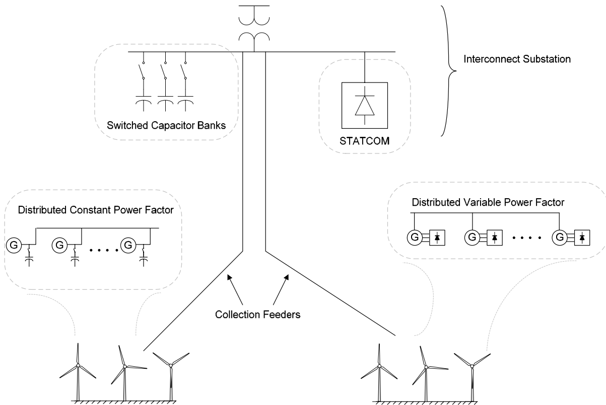
Figure 10-10 Illustration of Various Reactive Compensation and Voltage Control Mechanisms for Wind Farm Applications
