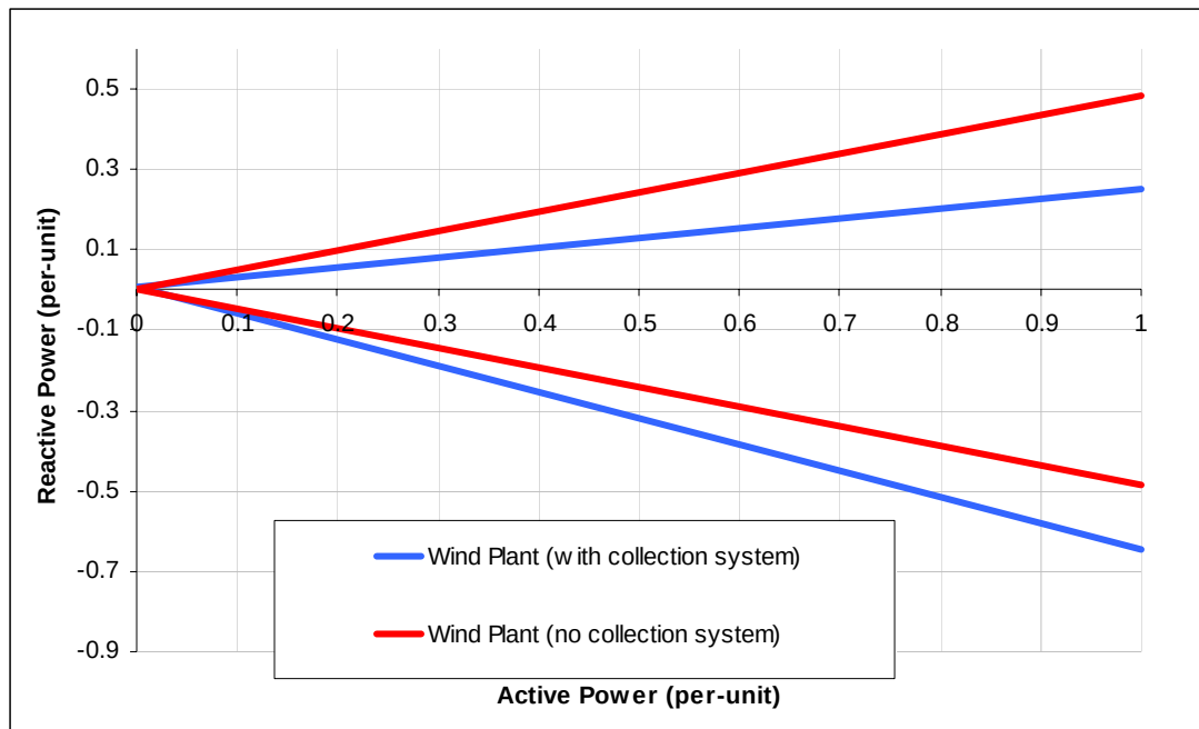
Figure 10-11 Power Factor Curves for Example Wind Plant
