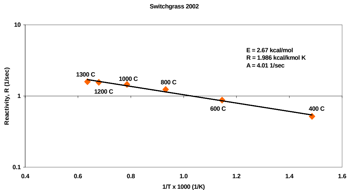
Figure 4-5 Devolatilization Kinetics for Fresh Switchgrass (Source: Johnson et al., 2002)
