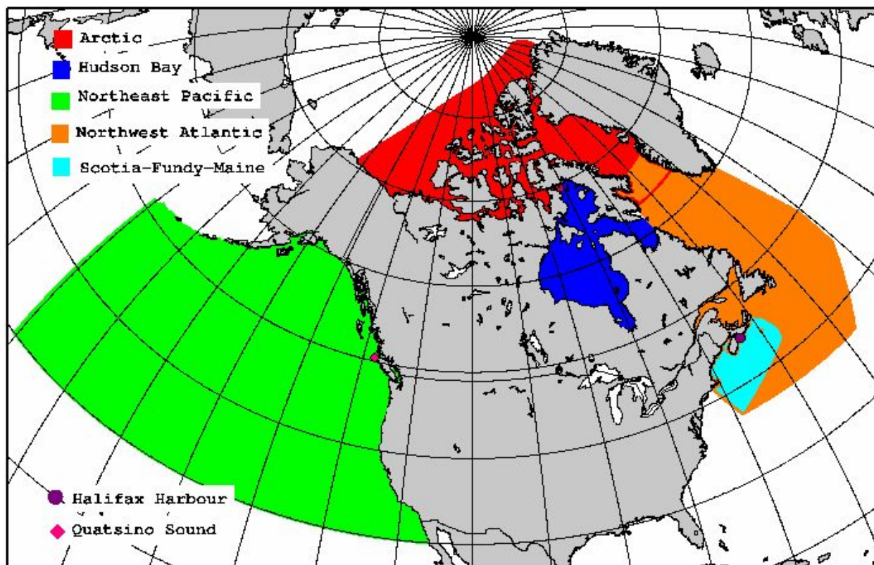
Figure 8-10 WebTide Ocean Model Regions
