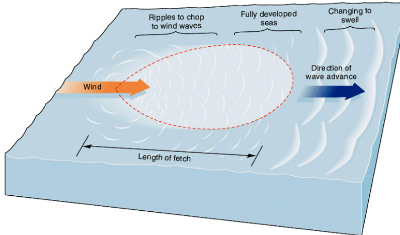
Figure 9-1 Wind Blowing Over Fetch of Water Produces Waves
