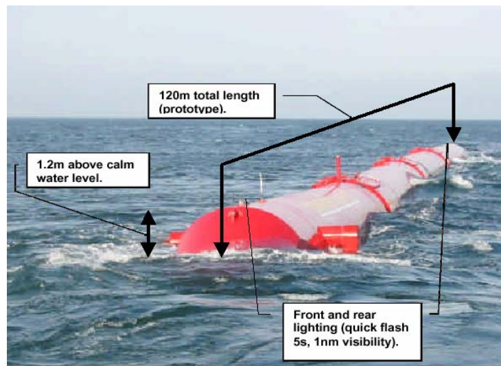
Figure 9-15 Preproduction Prototype Pelamis
