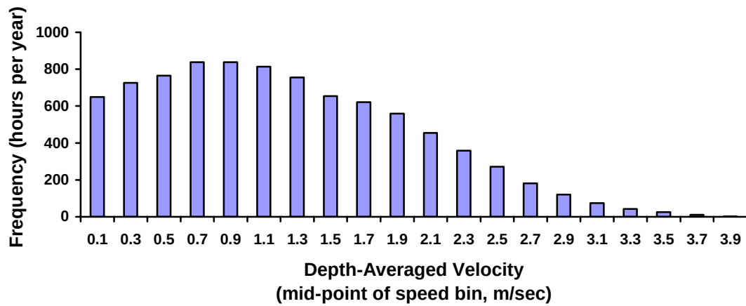
Figure 8-13 Annual Average Tidal Current Speed Probability Distributions for Point Evans Transect, Tacoma Narrows, WA (West Coast)
