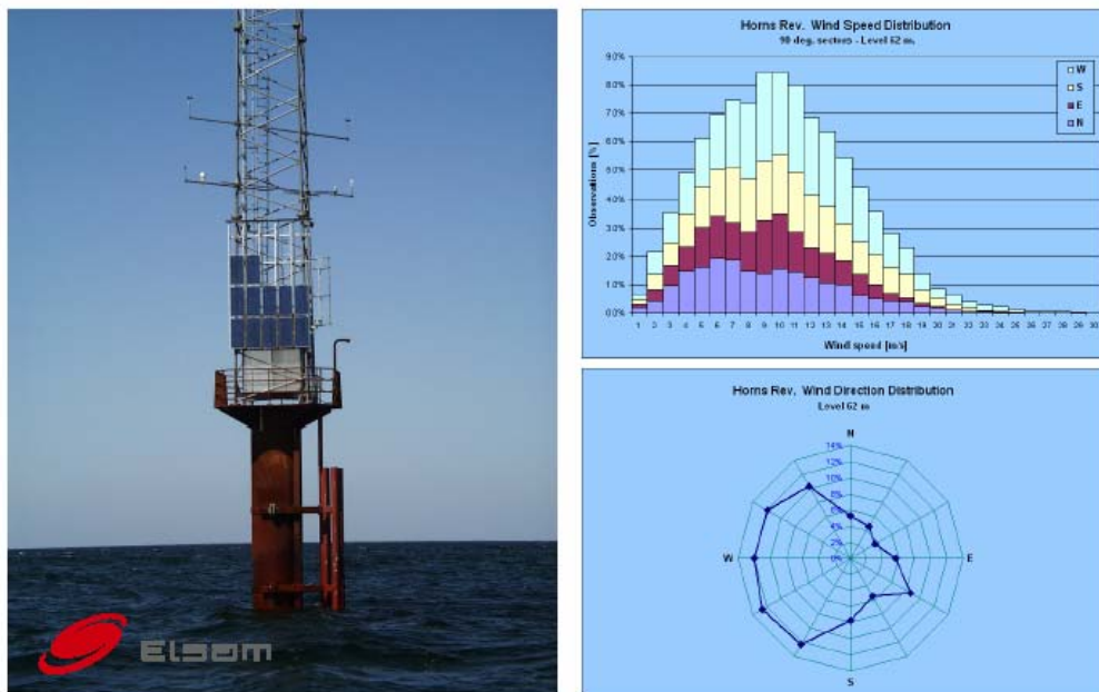
Figure 3-14 Meteorological Tower and Wind Speed Frequency Data from Horns Rev Site (EUREC, Elsam, and Risoe National Laboratory [60]).
