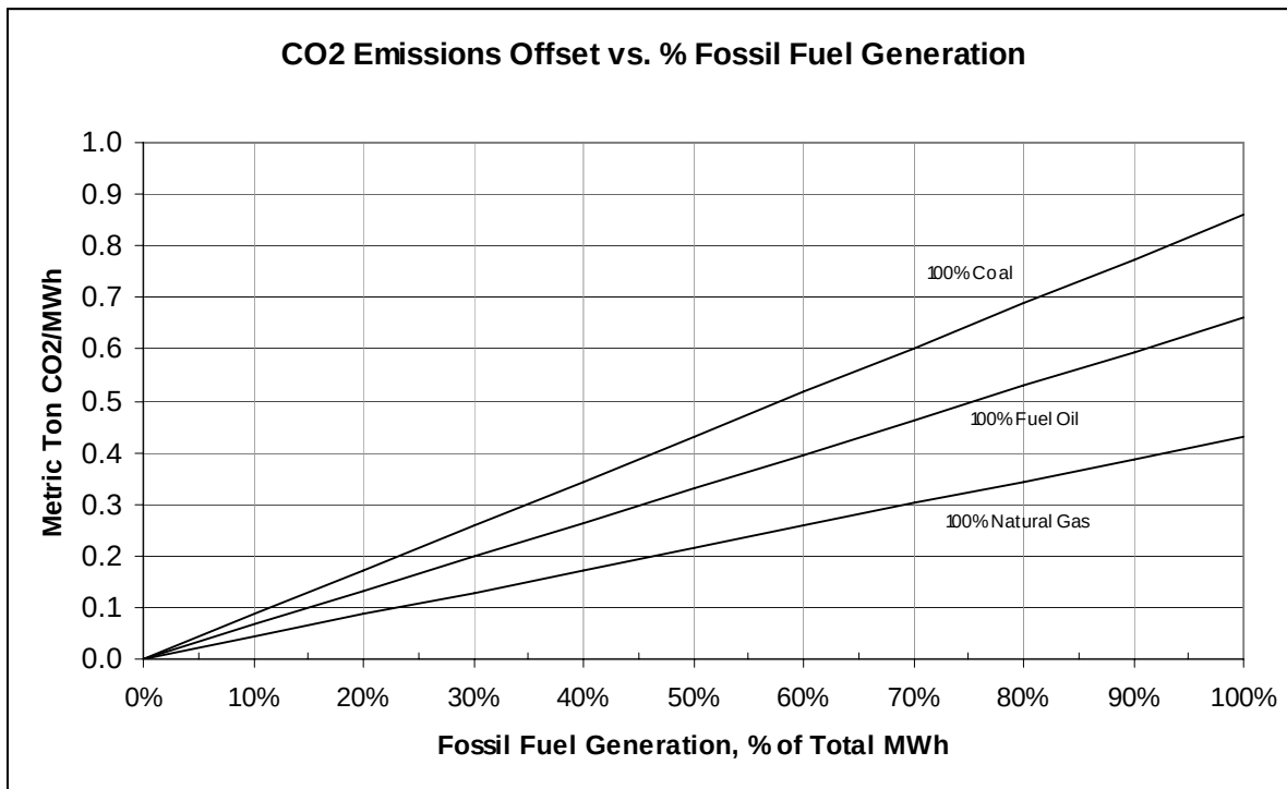
Figure 11-1 Levelized CO 2 Emissions Offset vs. % Fossil Fuel Generation
