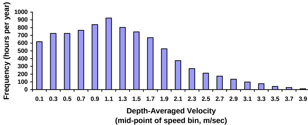
Figure 8-14 Annual-Average Tidal Current Speed Probability Distributions for Cairn Point Transect, Knik Arm, AK (West Coast)
