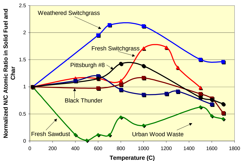
Figure 4-19 Normalized Nitrogen/Carbon Atomic Ratios for Biomass Solid Fuel and Char, Compared to Pittsburgh #8 Bituminous Coal and Black Thunder Powder River Basin Subbituminous Coal
