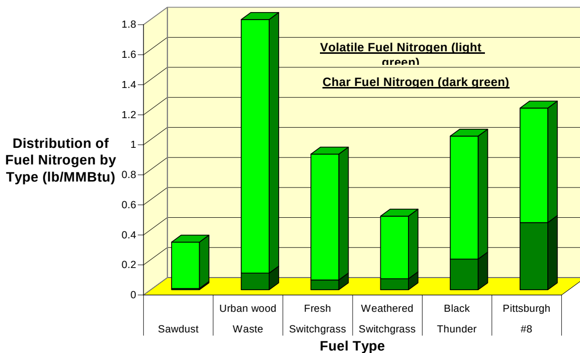
Figure 4-10 Distribution of Volatile and Char Fuel Nitrogen in Selected Biomass and Reference Coal Samples (Source: Johnson et al., 2001; Johnson et al., 2002)
