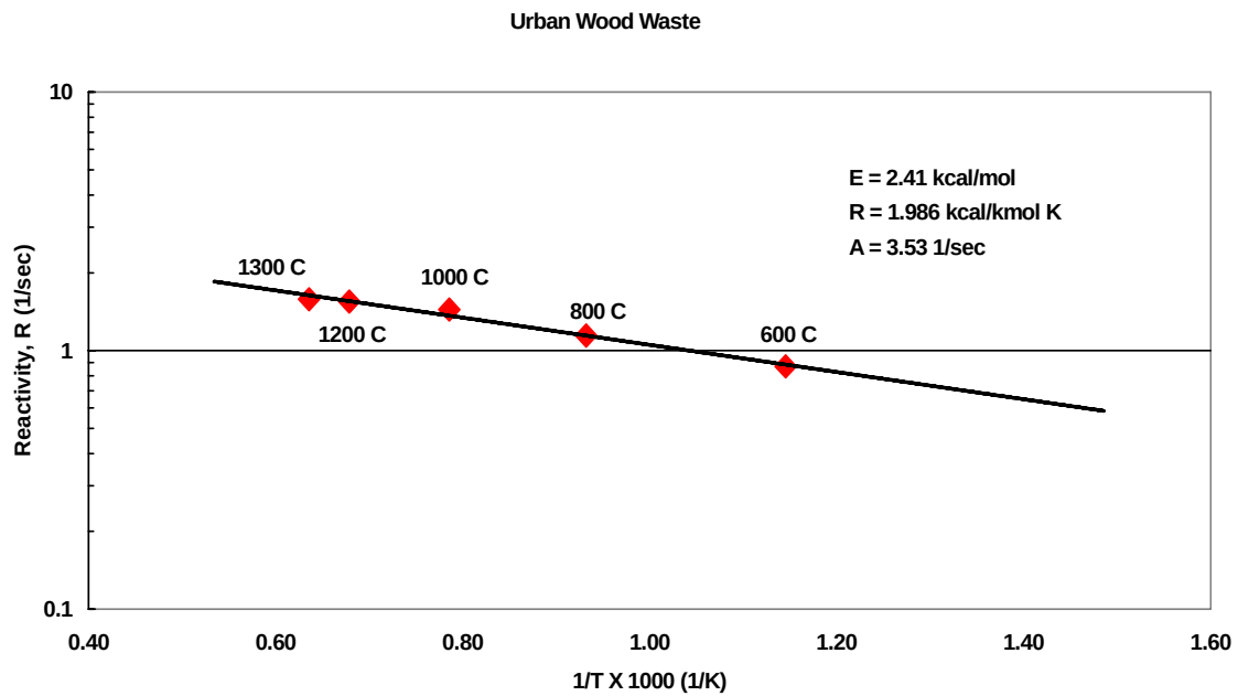
Figure 4-4 Devolatilization Kinetics for Urban Wood Waste (Source: Johnson et al., 2002)
