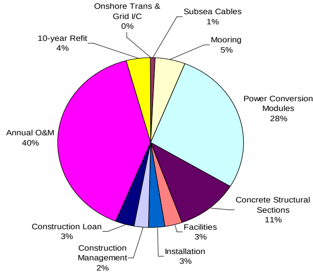
Figure 9-20 Commercial Scale COE Breakdown—Oregon Example
