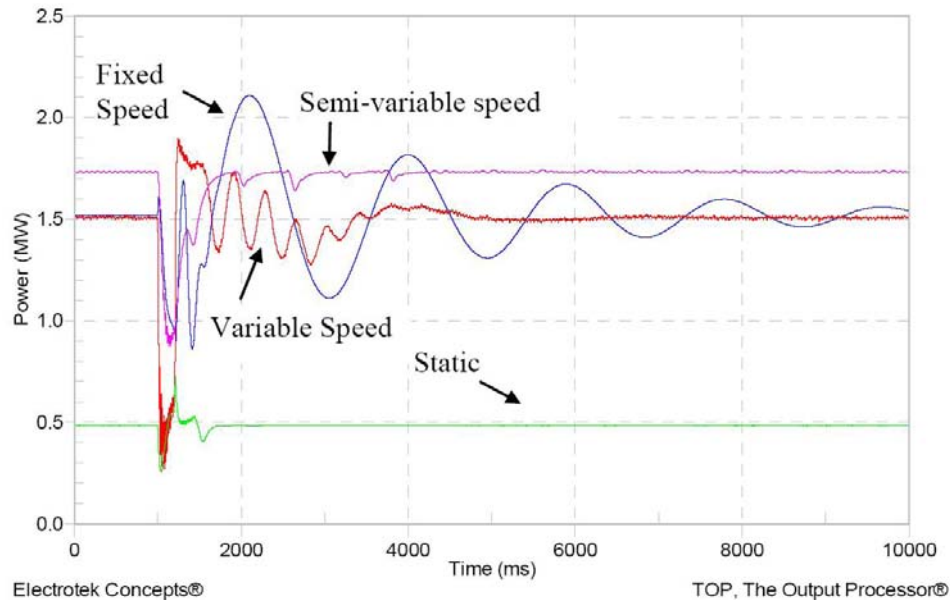
Figure 10-9 Response of Four Commercially Available Wind Turbine Generators to a Large Voltage Sag
