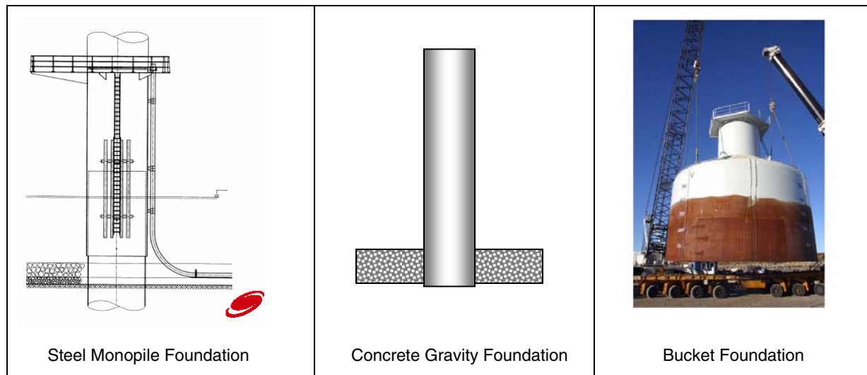
Figure 3-11 Steel Monopile, Concrete Gravity, and Bucket Foundations for Offshore Wind Turbines in Shallow Water Less than 30-m Depth (EUREC and Risoe National Laboratory [60])
