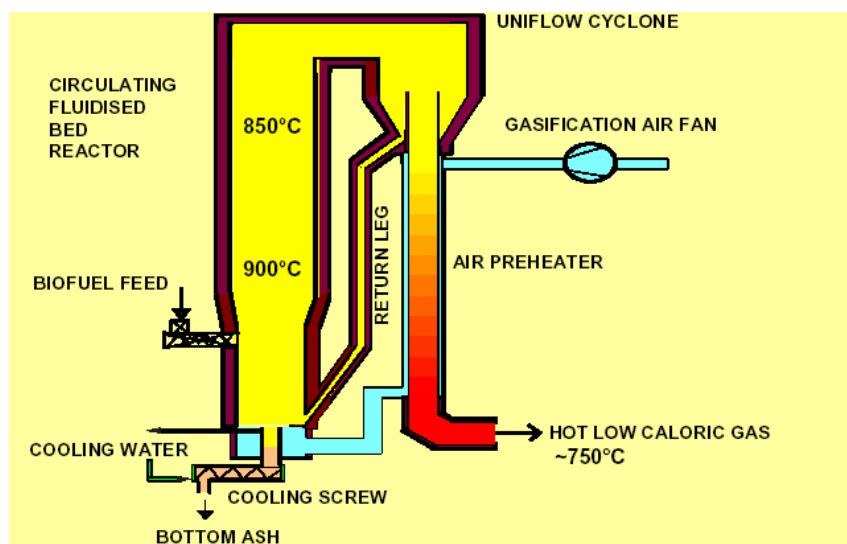
Figure 4-36 Overall Configuration of the Biomass Gasifier at Ruien
