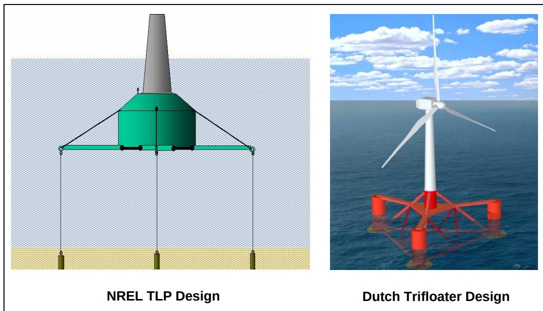
Figure 3-16 NREL TLP and Dutch Trifloater Design Concepts for Floating Wind Turbine Platforms (Source: Musial and Butterfield, NREL/U.S. DOE, 2004)
