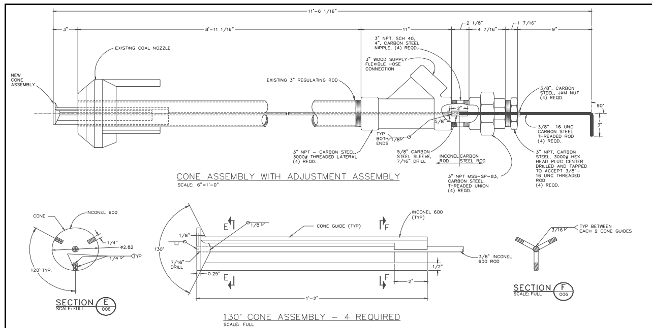
Figure 4-26 Design of the Sawdust Injection System at Seward Generating Station
