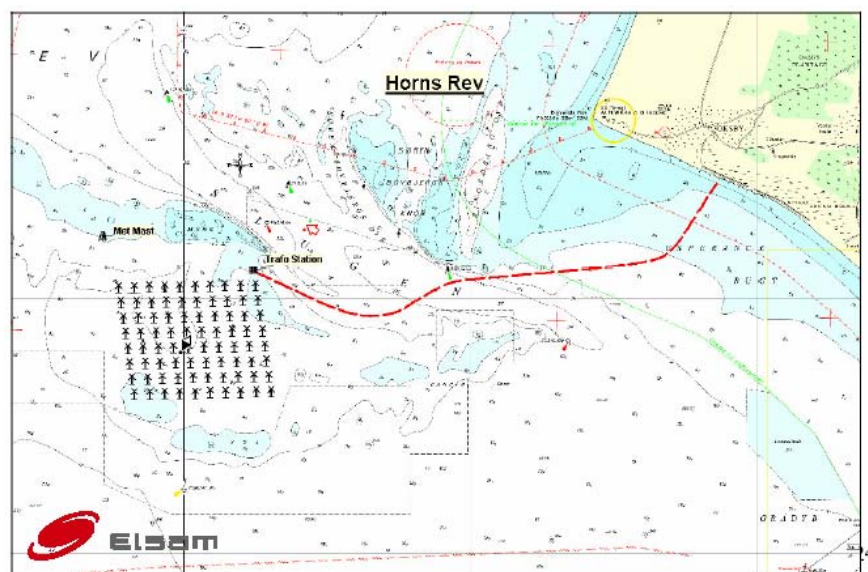
Figure 3-12 Location of 80 2-MW wind turbines at Horns Rev Offshore Wind Project (EUREC, Elsam, and Risoe National Laboratory [60])
