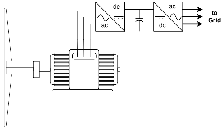
Figure 10-5 Variable-Speed, Direct-Drive Asynchronous Machine Converter-Connected WTG (no gear box)
