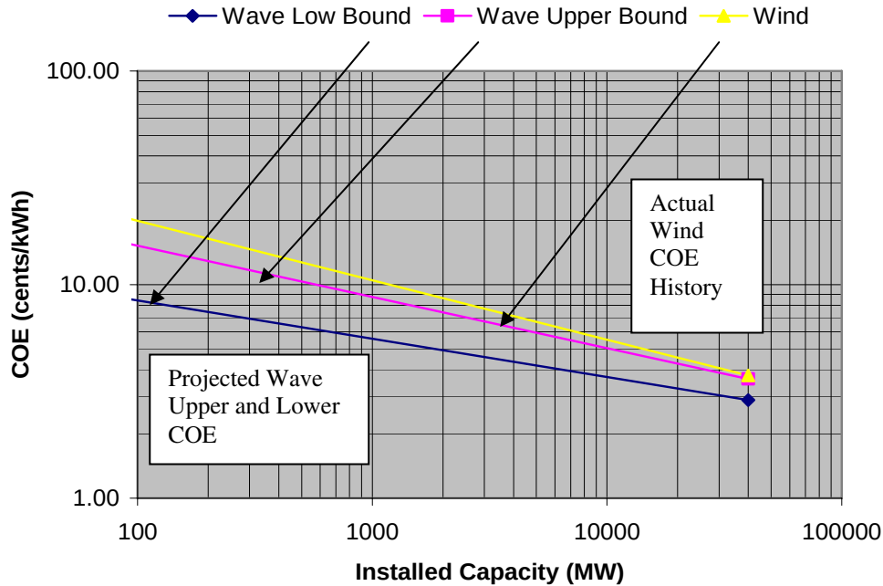
Figure 9-21 Levelized COE Comparison to Wind–Oregon Example
