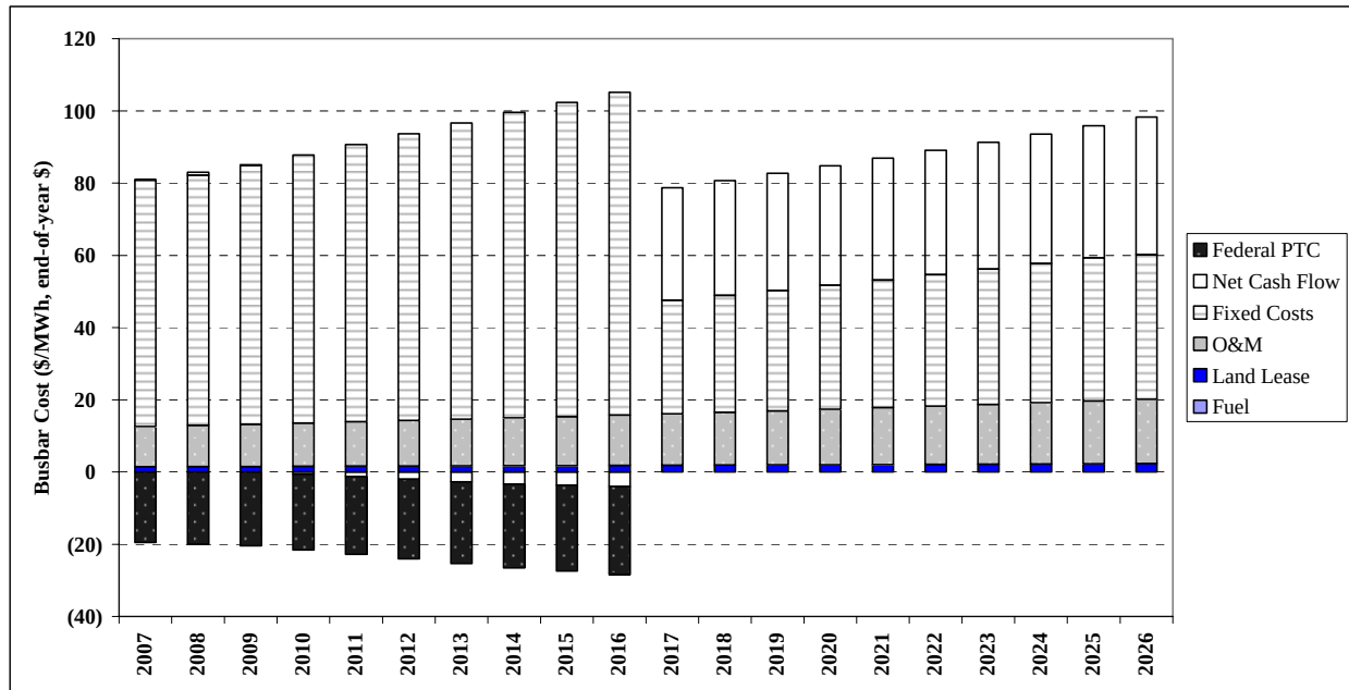
Figure 2-3 Components of Busbar Cost for Example 100-MW Wind Generation Plant
