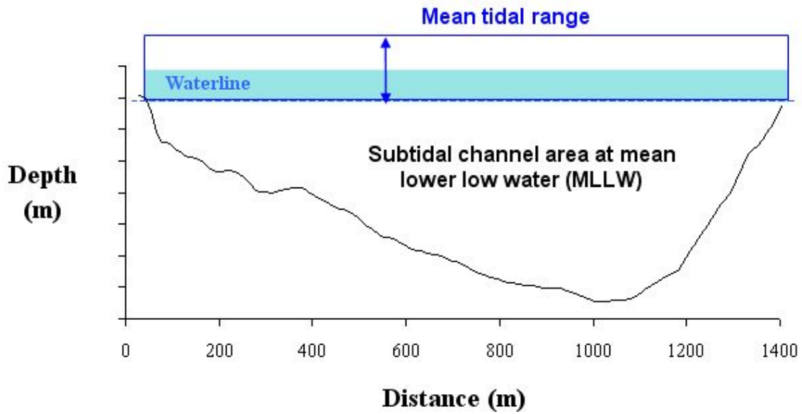
Figure 8-18 Accounting for Tidal Range in Cross-Sectional Area Calculation
