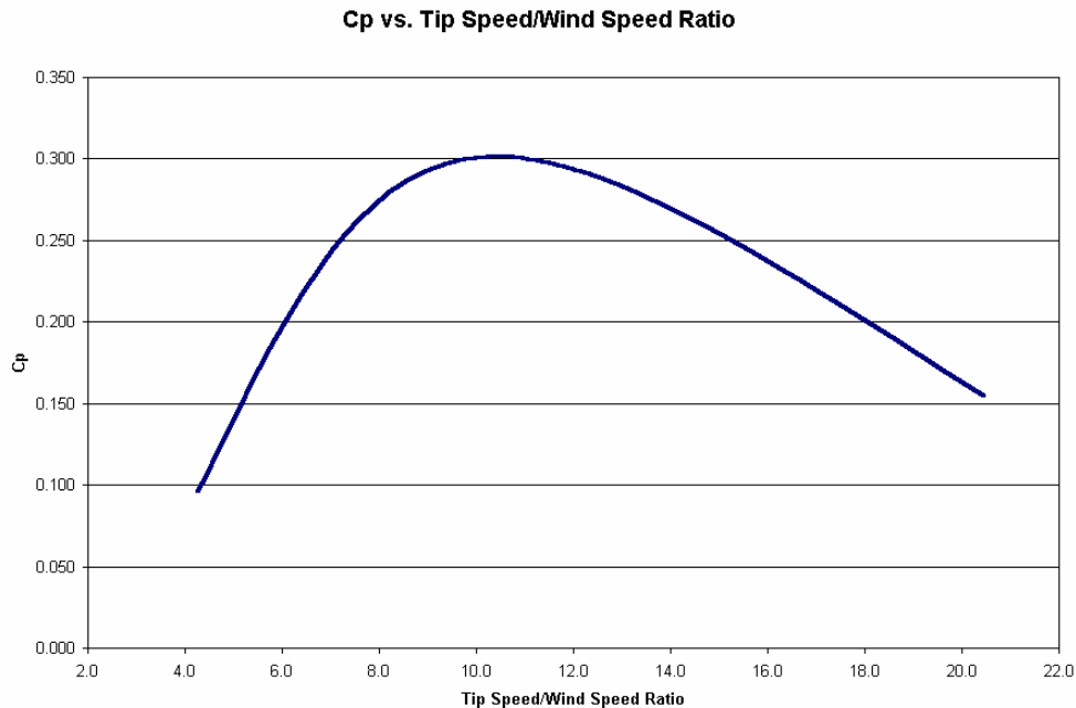
Figure 3-5 Coefficient of Performance ( C_p ) vs. Tip Speed/Wind Speed Ratio
