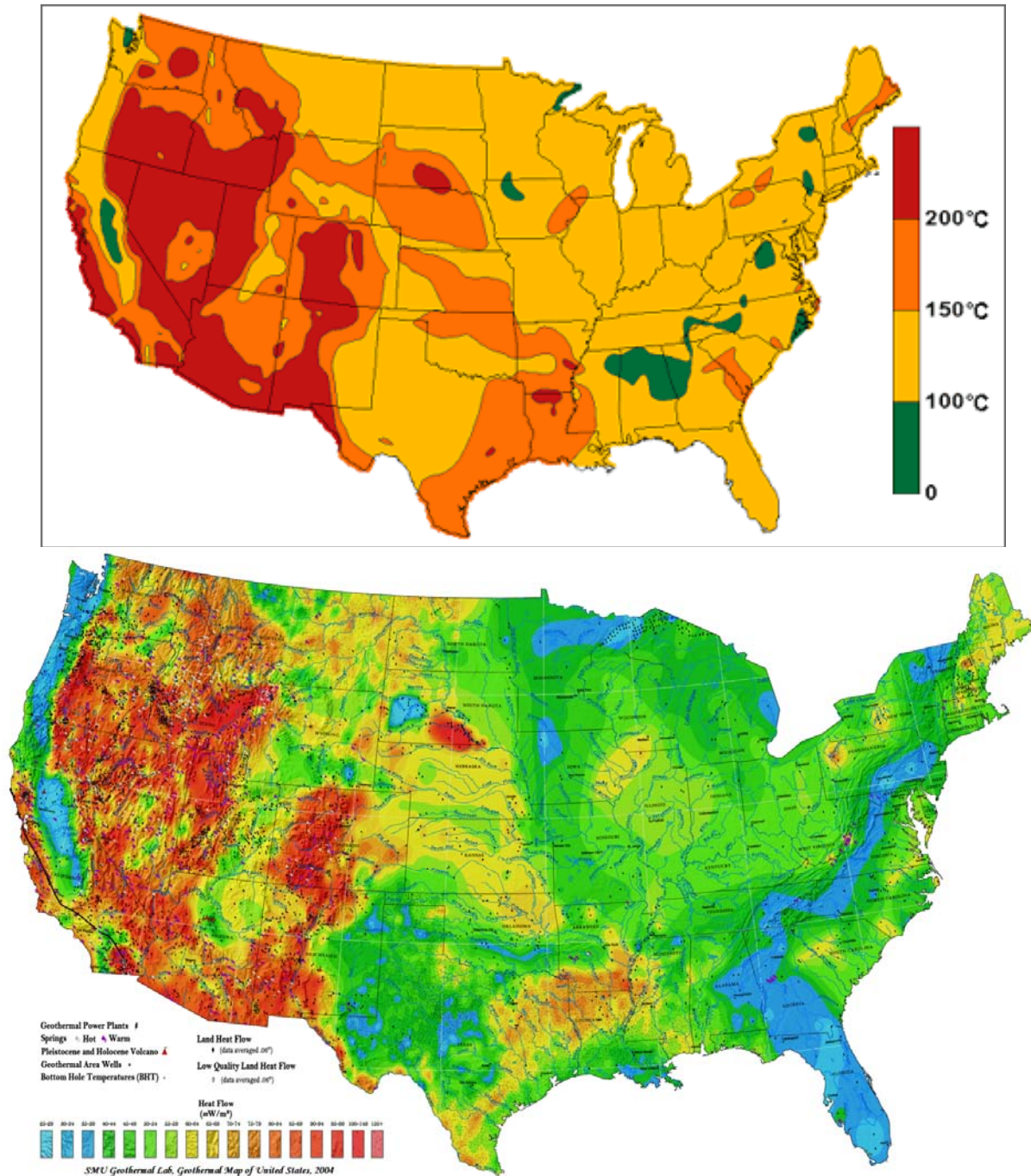
Figure 6-1 Map of U.S. Geothermal Resource Potential Map [Estimated Temperatures (°C) at 6 km Depth] (top), 2004 SMU Heat Flow Assessment (bottom)
