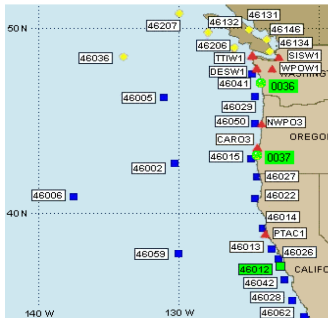
Figure 9-5 West Coast Reference Stations (NDBC 46012 is green square; CDIP 0036 and 0037 are green circles)
