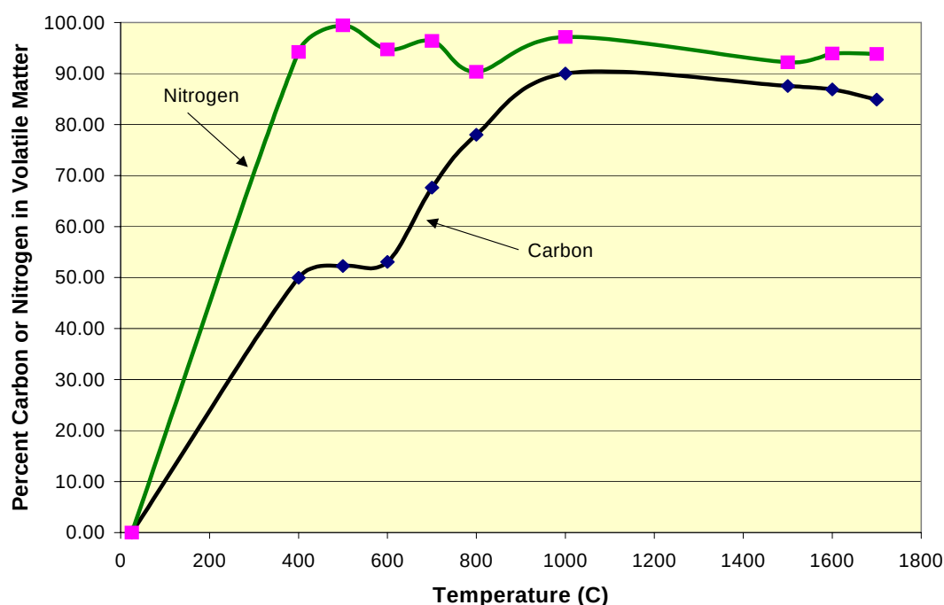
Figure 4-12 Volatile Nitrogen and Carbon Evolution from Fresh Sawdust
