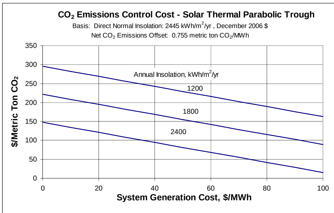
Figure 11-8 Levelized CO 2 Emissions Control Cost vs. Annual Insolation (Top) and System Generation Cost (Bottom) for an 80-MW Solar Thermal Parabolic Trough Power Plant (Dec-06 $)
