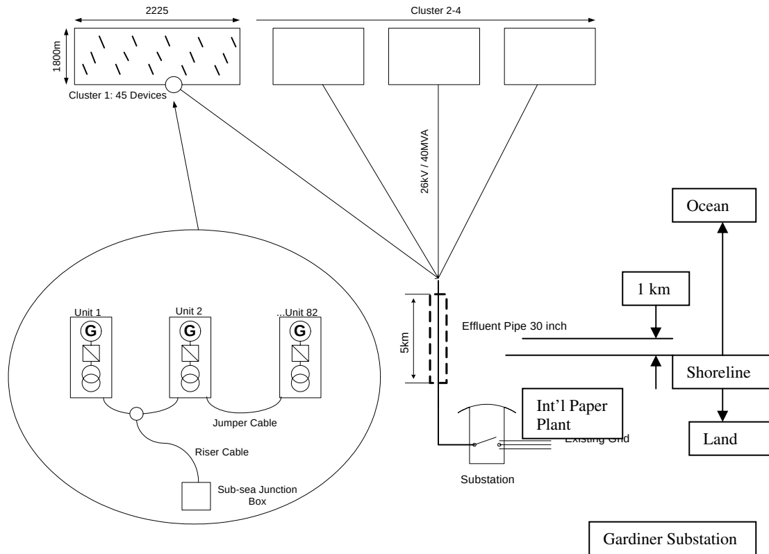
Figure 9-19 Electrical Interconnection of a Commercial-Scale Pelamis Plant—Oregon Example
