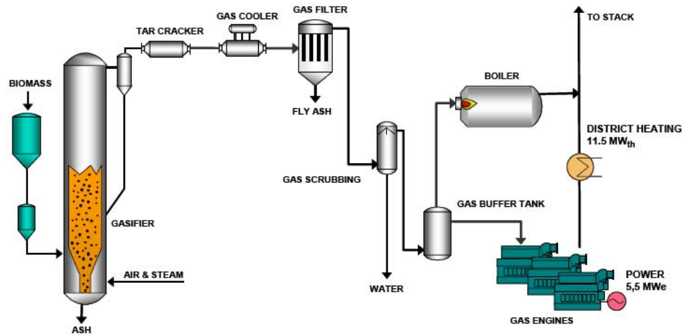
Figure 4-35 Fjernvarme Process Flow Diagram for Coproduction of 6 MW electric and 10 MW thermal.
