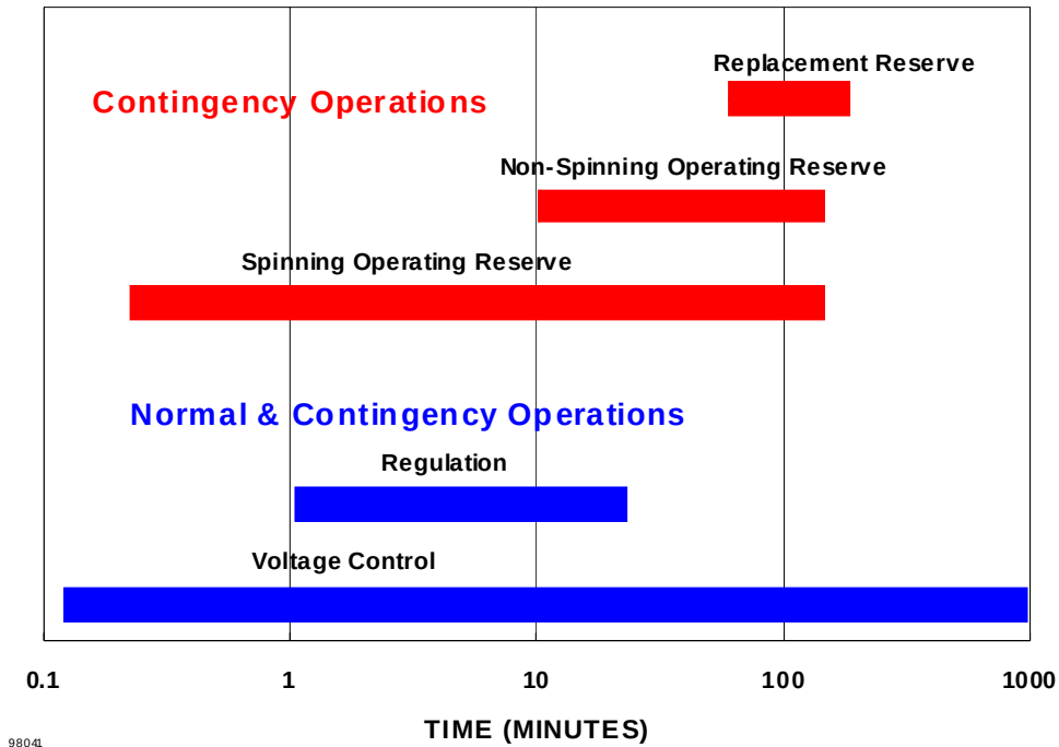
Figure 10-1 Ancillary Services Are Distinguished by Their Deployment Times and Durations
