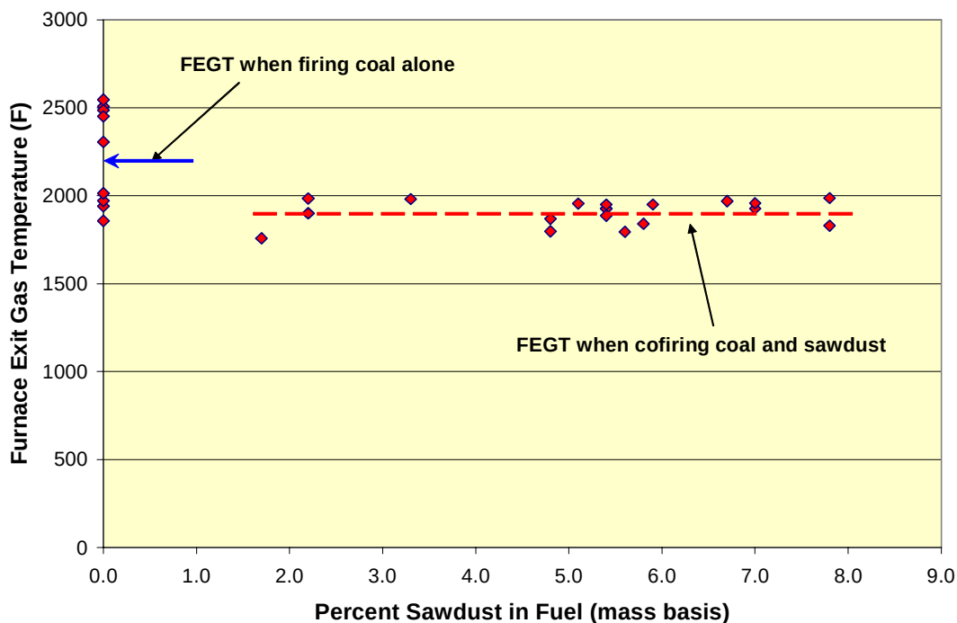
Figure 4-24 Influence of Cofiring in Cyclone Boilers on Furnace Exit Gas Temperature (Source: Tillman and Payette, 2004)
