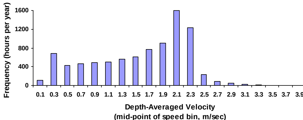
Figure 8-11 Annual Average Tidal Current Speed Probability Distributions for Cape Blomidon transect, Minas Passage, NS (East Coast)
