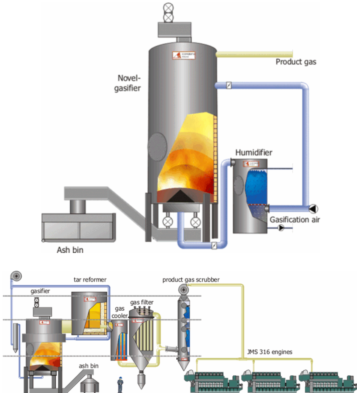
Figure 4-37 Schematic of Biomass Gasification and Power Generation System at Kokomäki.
