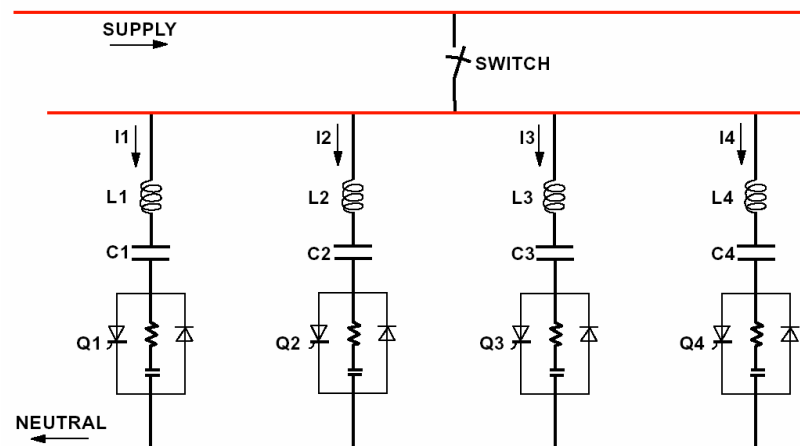
Figure 10-15 Configuration of Commercially Available DSVC Source: S&C Electric
