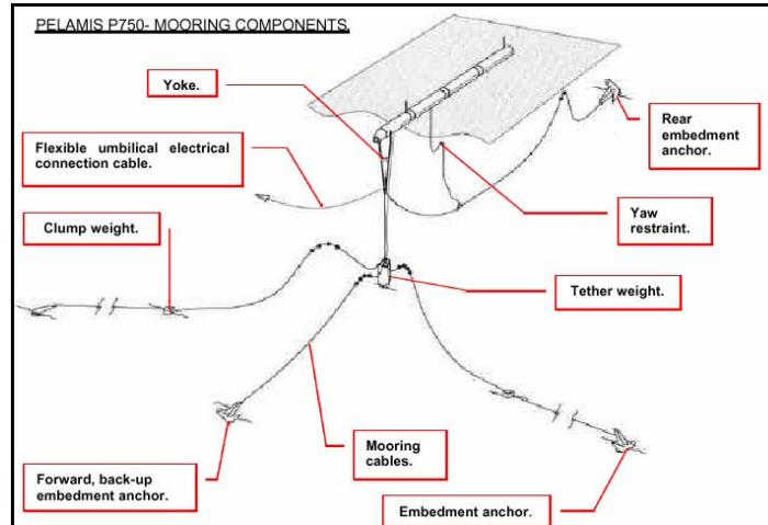
Figure 9-16 Mooring Arrangement of the Prototype Pelamis Design
