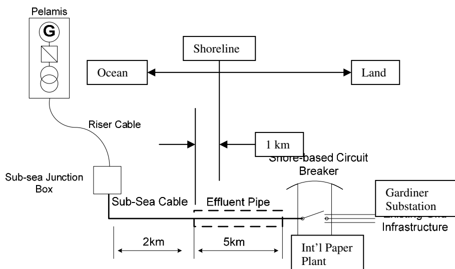
Figure 9-18 Electrical Interconnection of a Single Unit Pelamis Plant–Oregon Example
