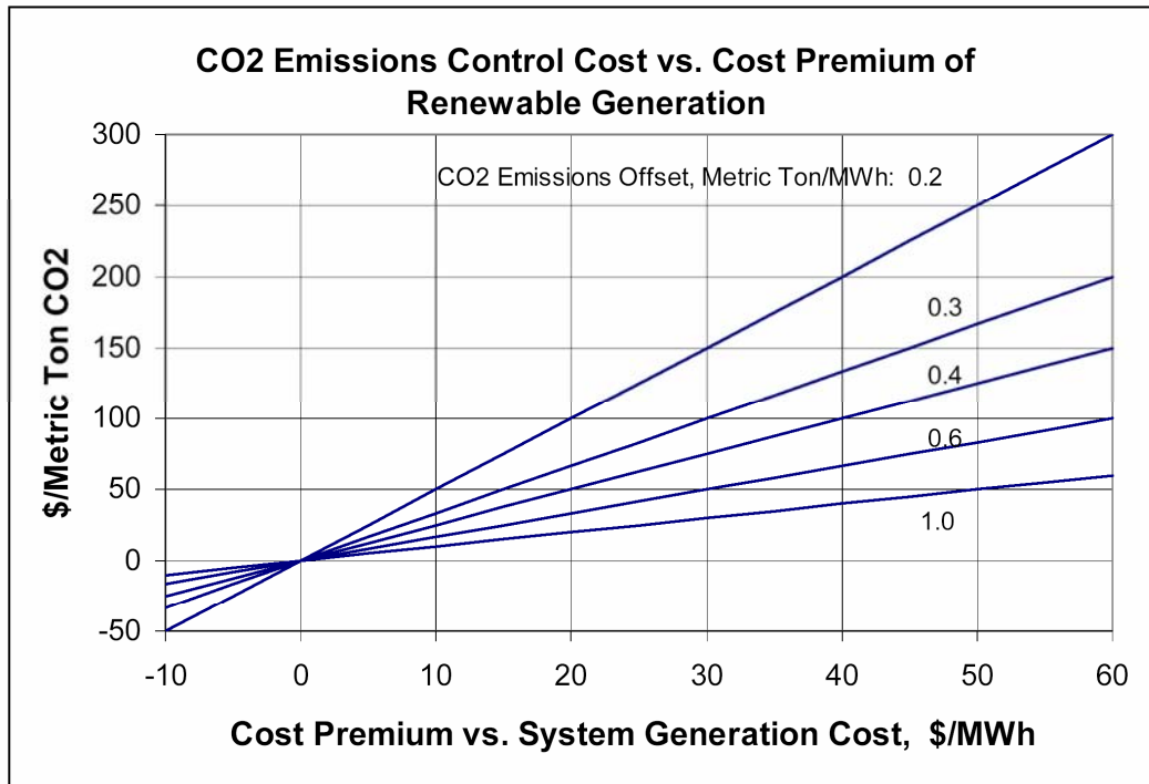
Figure 11-2 Levelized CO 2 Emissions Control Cost vs. Cost Premium and CO 2 Emissions Offset
