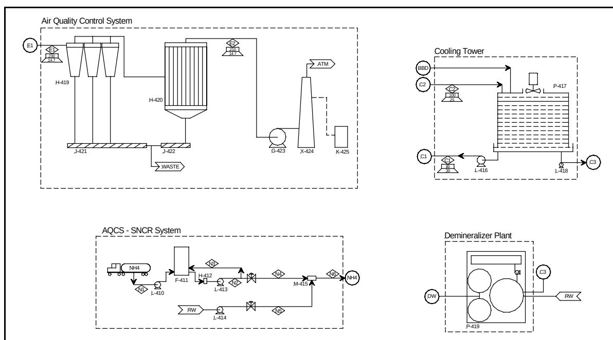
Figure 4-32 Air Pollution Control System, Cooling Tower, and Demineralizer for a Typical Wood Waste-Fired Plant
