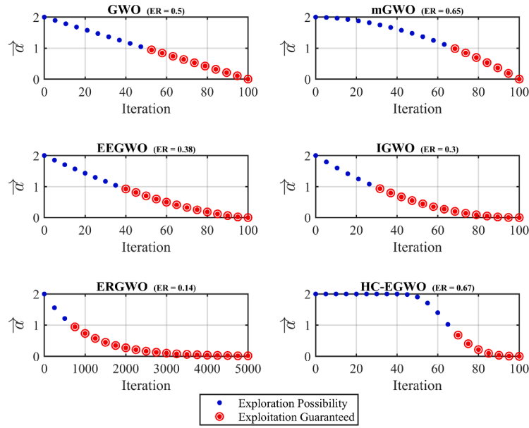
Fig. 10. The evolution of \vec{a} value during the optimization process for the six evaluated GWO methods in this study, and their Exploration Ratio (ER).
