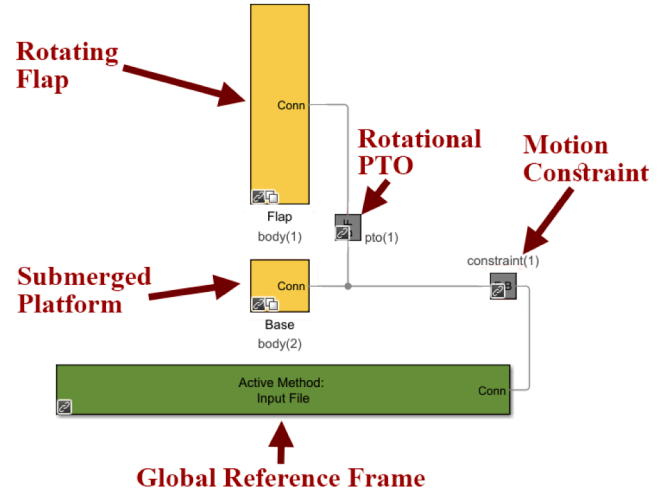
Fig. 12. OSWEC's Simulink model in WEC-Sim [33].
