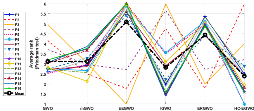
Fig. A.21. Average performance rank of the HC-EGWO compared with other five variants of GWOs over the 16 benchmarks using the Friedman test.
