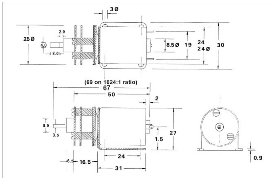
Figure 25. Motor and gearbox dimensions [mm].
