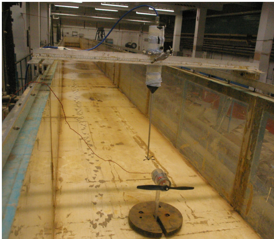
Figure 32. Velocity meter setting.
