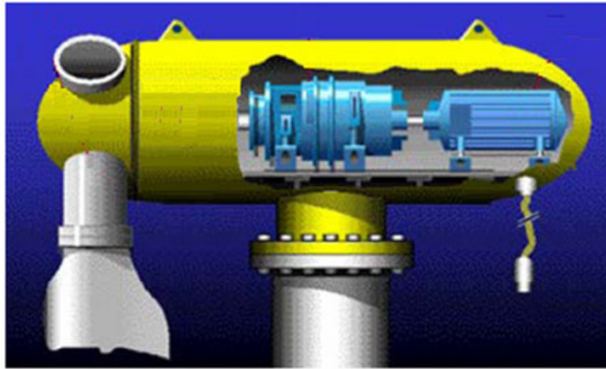
Figure 8. Inside view of marine current turbine nacelle. (Source: tidevannsenenergi.com)
