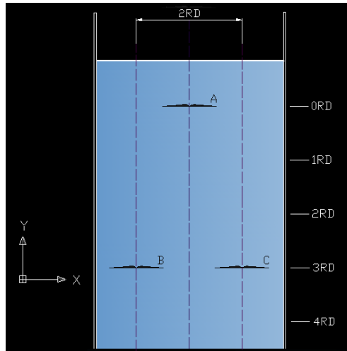
Figure 45 and 46. Array configuration 1-1 and turbine performance.
