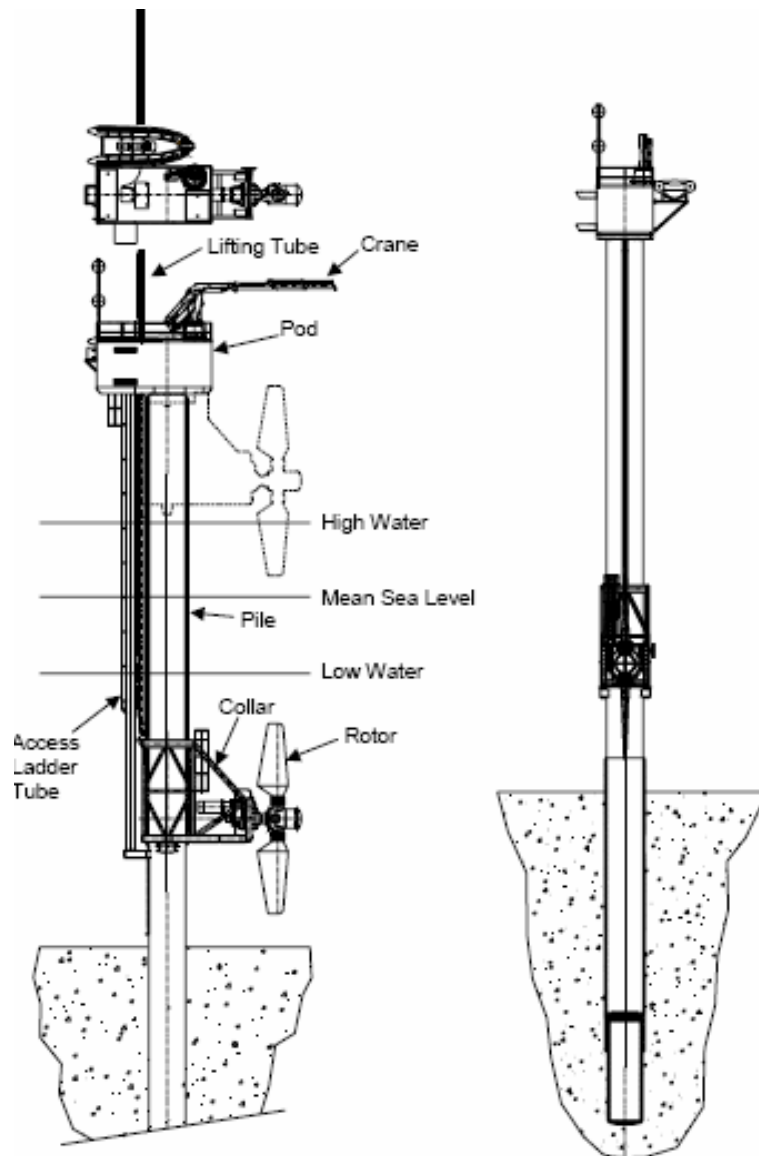
Figure 7. Marine current turbine arrangement. [15]
