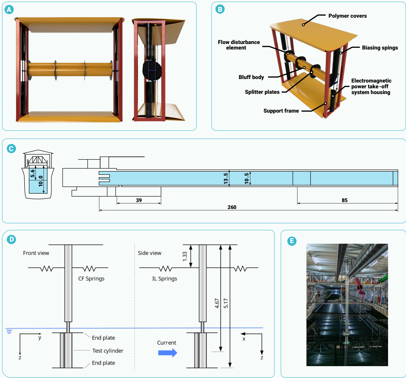
Figure 1. (A) & (B) Overview of the VIMEC device concept And experimental verification of VIMEC oscillator: (C) details of the towing tank and, (D) schematic and (E) photograph of the pendulum test rig allowing tracking the 2DOF VIV response.
