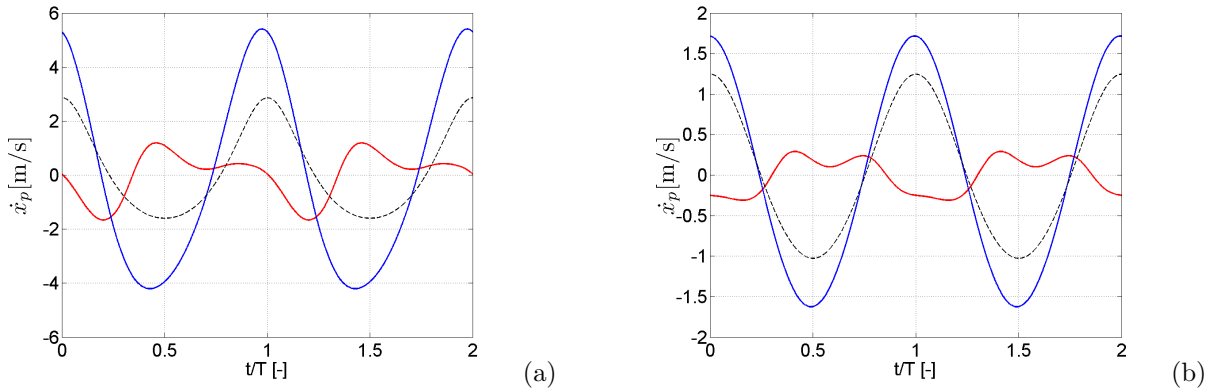
Figure 6: The plate velocity. Figure (a): Case #1, figure (b): Case #2. — Plate A, — Plate B, - - Horizontal surface velocity, u .
