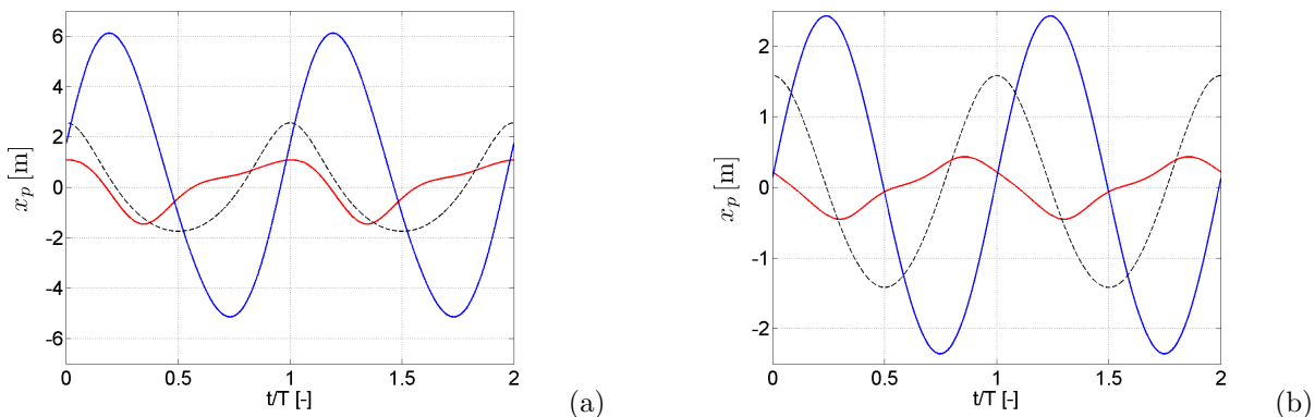
Figure 5: Plate oscillations as a function of time with reference to the incident wave cf. table 1. Figure (a): Case #1, figure (b): Case #2. — Plate A, — Plate B, - - Surface elevation \eta .
