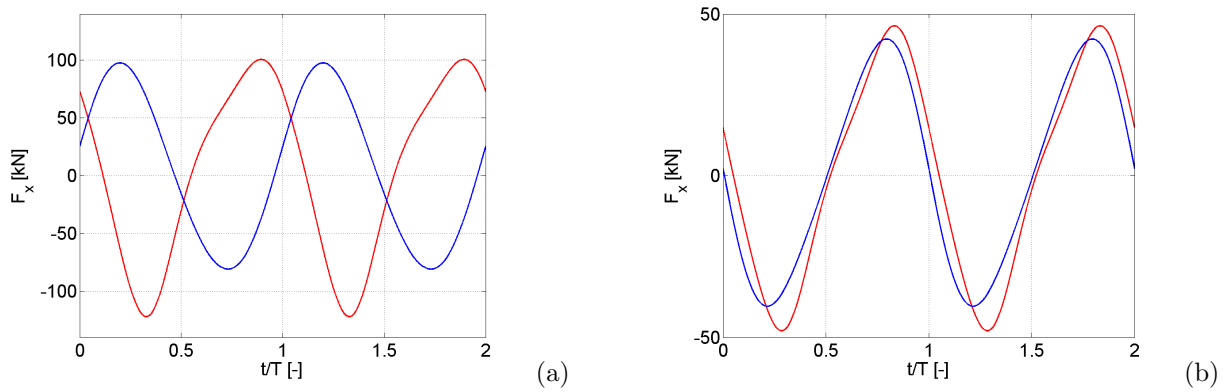
Figure 8: The total force F_x . Figure (a): Case #1, figure (b): Case #2. — Plate A, — Plate B.
