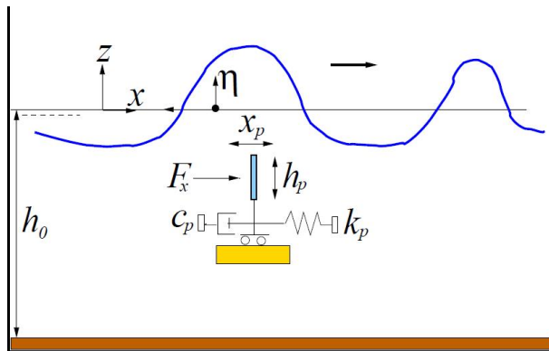
Figure 4: Problem set-up. Wave past a thin plate.
