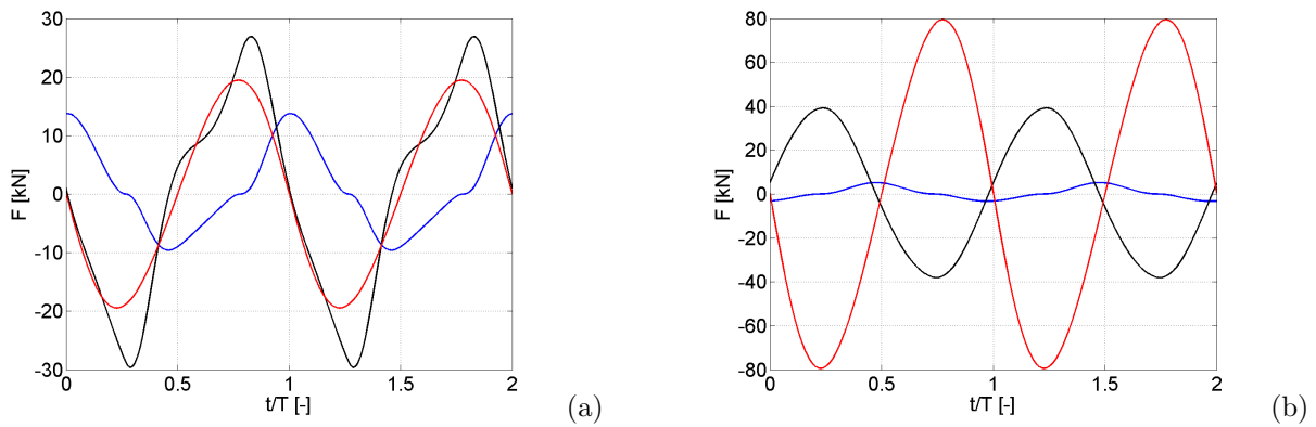
Figure 10: The force contributions for case #2. Figure (a): Plate A, figure (b): Plate B. Force ID: — Froude-Krylov force, — Drag force, — Hydrodynamic mass force.
