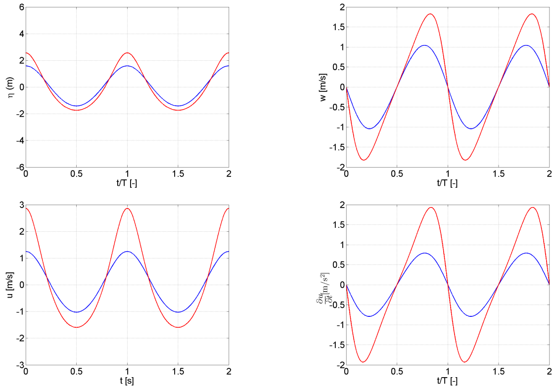
Figure 3: Free-surface solution based on Stream Function theory. — Case #1, — Case #2.
