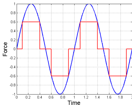
Figure 2: Plate contribution to the power-generation. In this report it is assumed that the plate contribute over the whole wave period (—). In the WavePiston-system the plate only contributes to the power generation when the force has obtained a certain value and is then constant (—).
