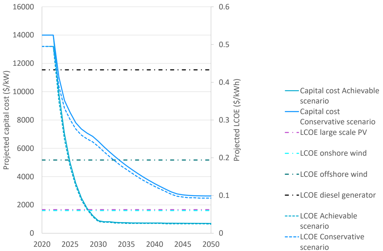
Figure 20 Projected modelled capital cost and LCOEs under the Achievable and Conservative scenarios
