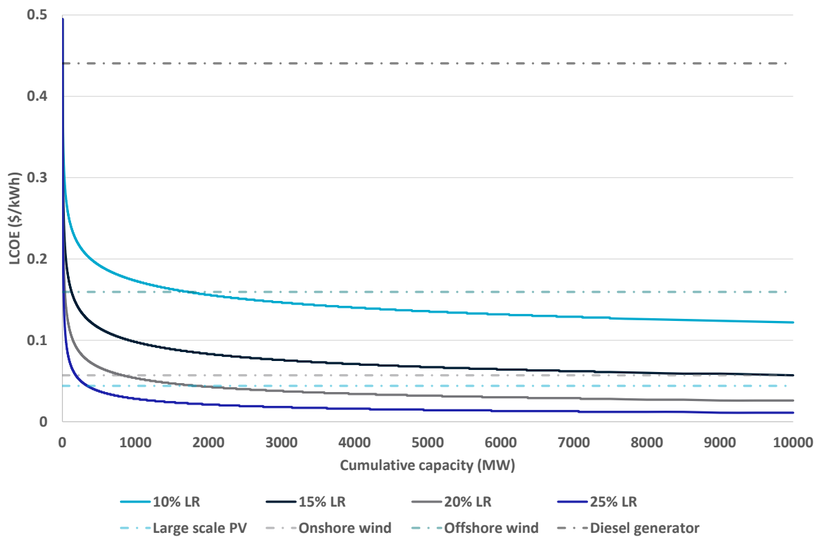
Figure 13 Projected LCOE of WSE's WEC at various LR and as a function of cumulative capacity and the 2030 LCOE of other technologies
