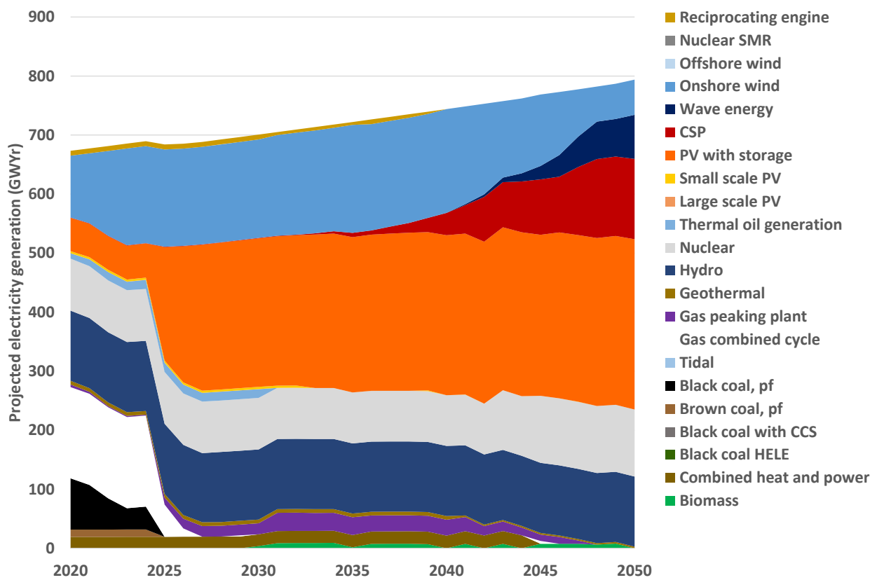
Figure 19 Projected North American electricity generation under the Conservative scenario
