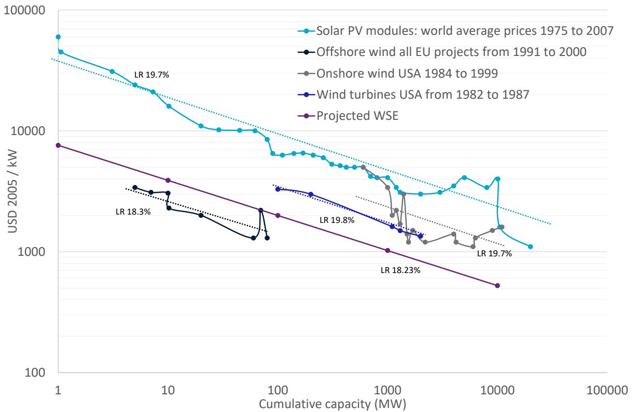
Figure 8 Projected capital cost with an increasing cumulative capacity
