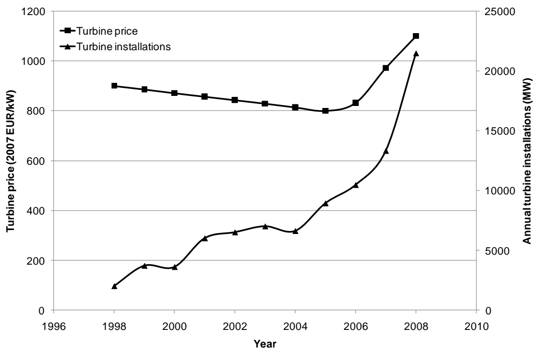
Figure 5 Wind turbine price and annual installations in IEA countries (Hayward and Graham, 2011)
