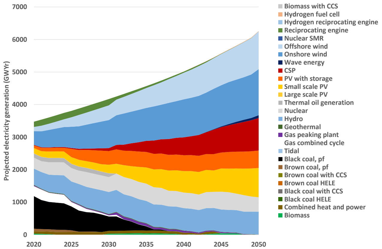
Figure 18 Projected global electricity generation under the Conservative scenario
