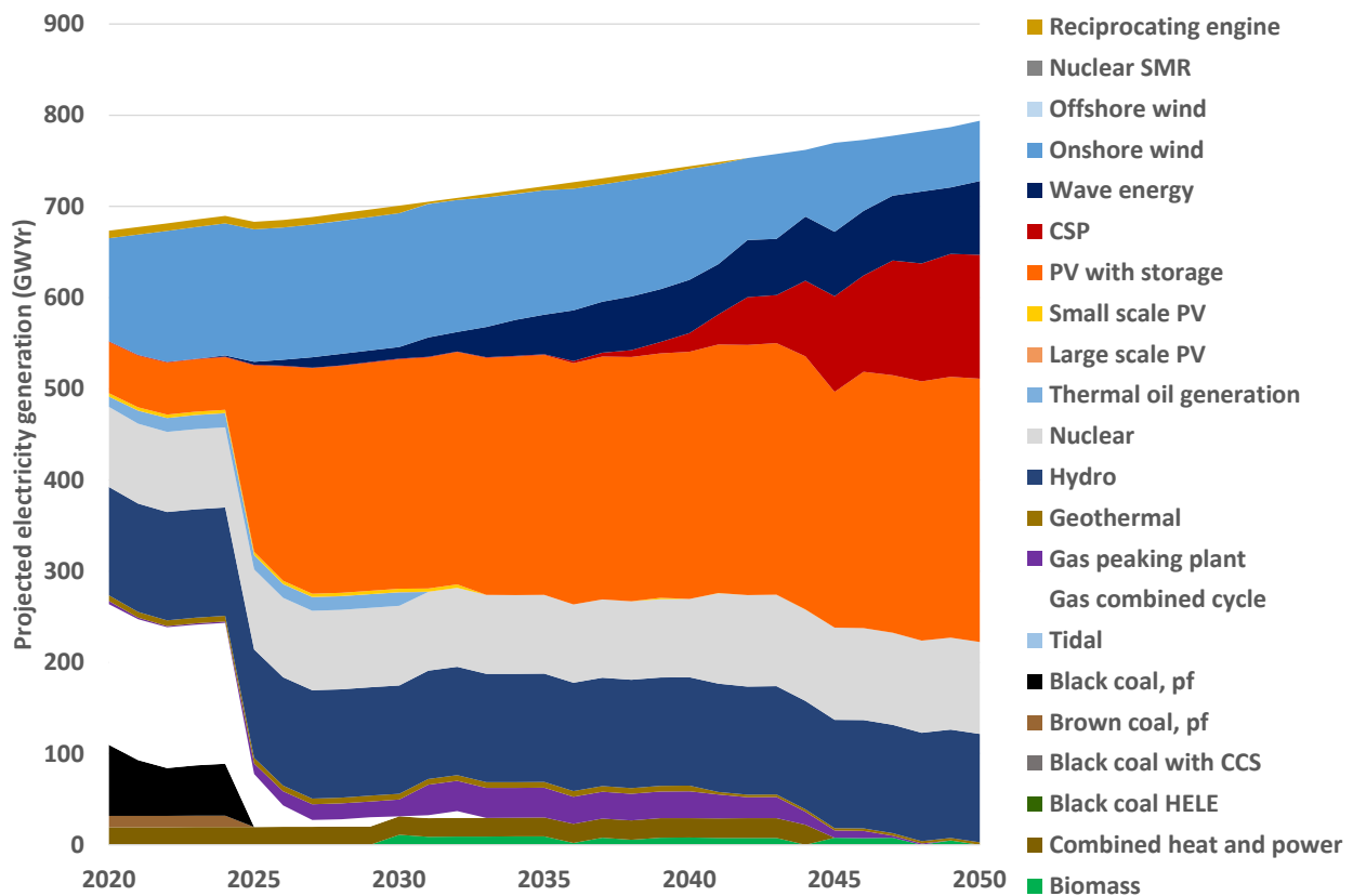
Figure 17 Projected North American electricity generation under the Achievable scenario
