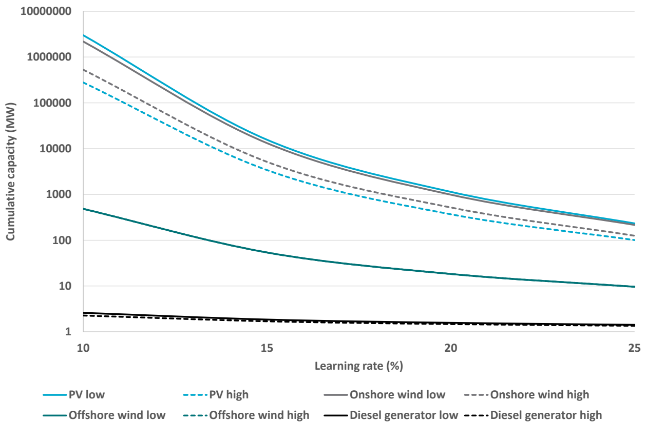
Figure 10 LR and cumulative capacity where the projected LCOE of WSE’s WEC is equivalent to that of other technologies in 2020
