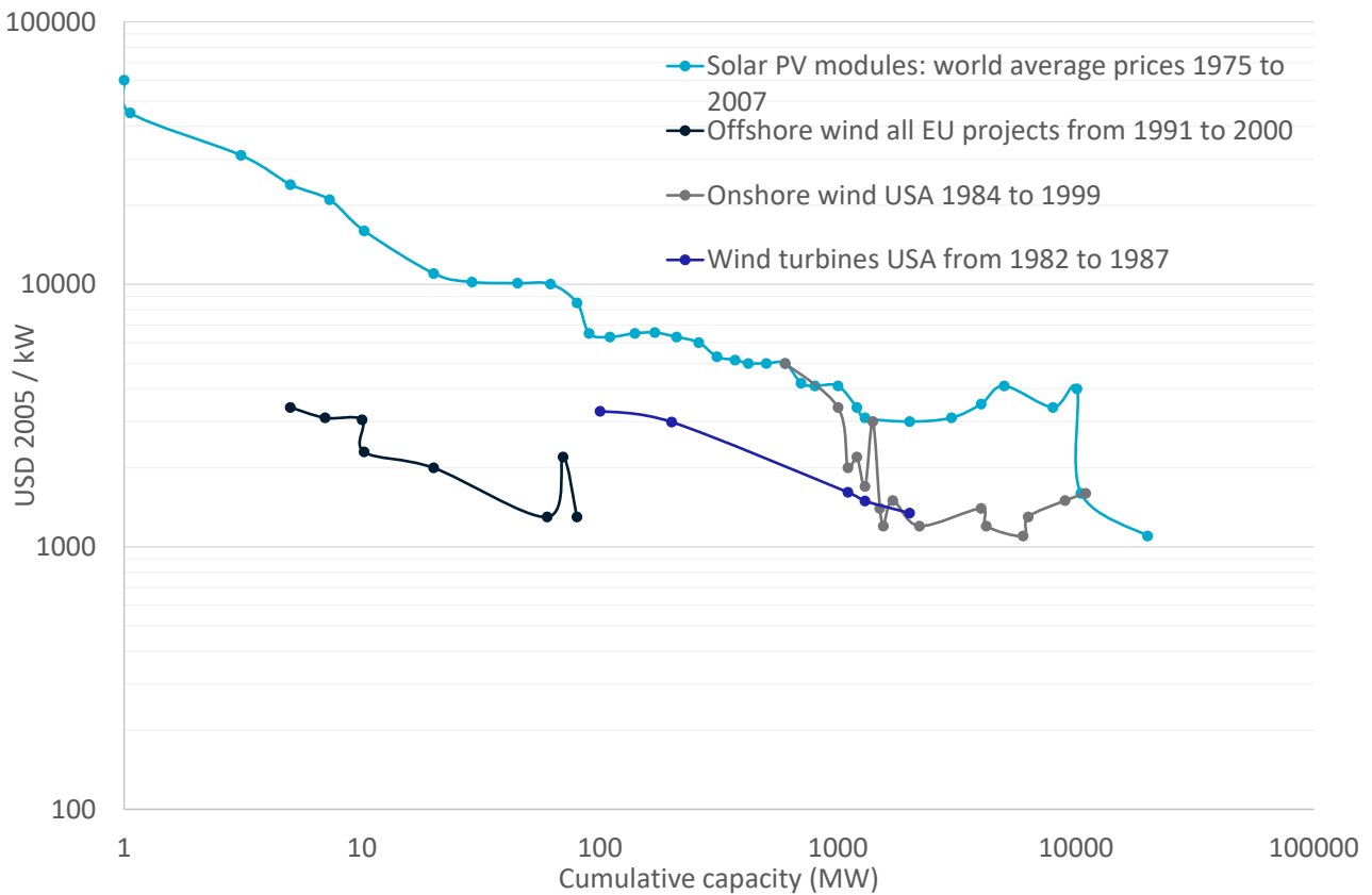
Figure 1 Historical technology costs versus deployment illustrating learning-by-doing. Source of data GEA (2012). PV=photovoltaics, EU=European Union, LR=learning rate, USA=United States of America, USD=United States Dollar. Wind turbines refer to just the component and onshore wind refers to onshore wind farms.
