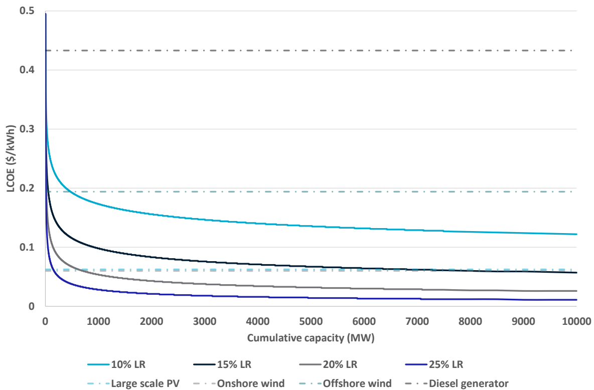
Figure 12 Projected LCOE of WSE's WEC at various LR and as a function of cumulative capacity and the 2020 LCOE of other technologies
