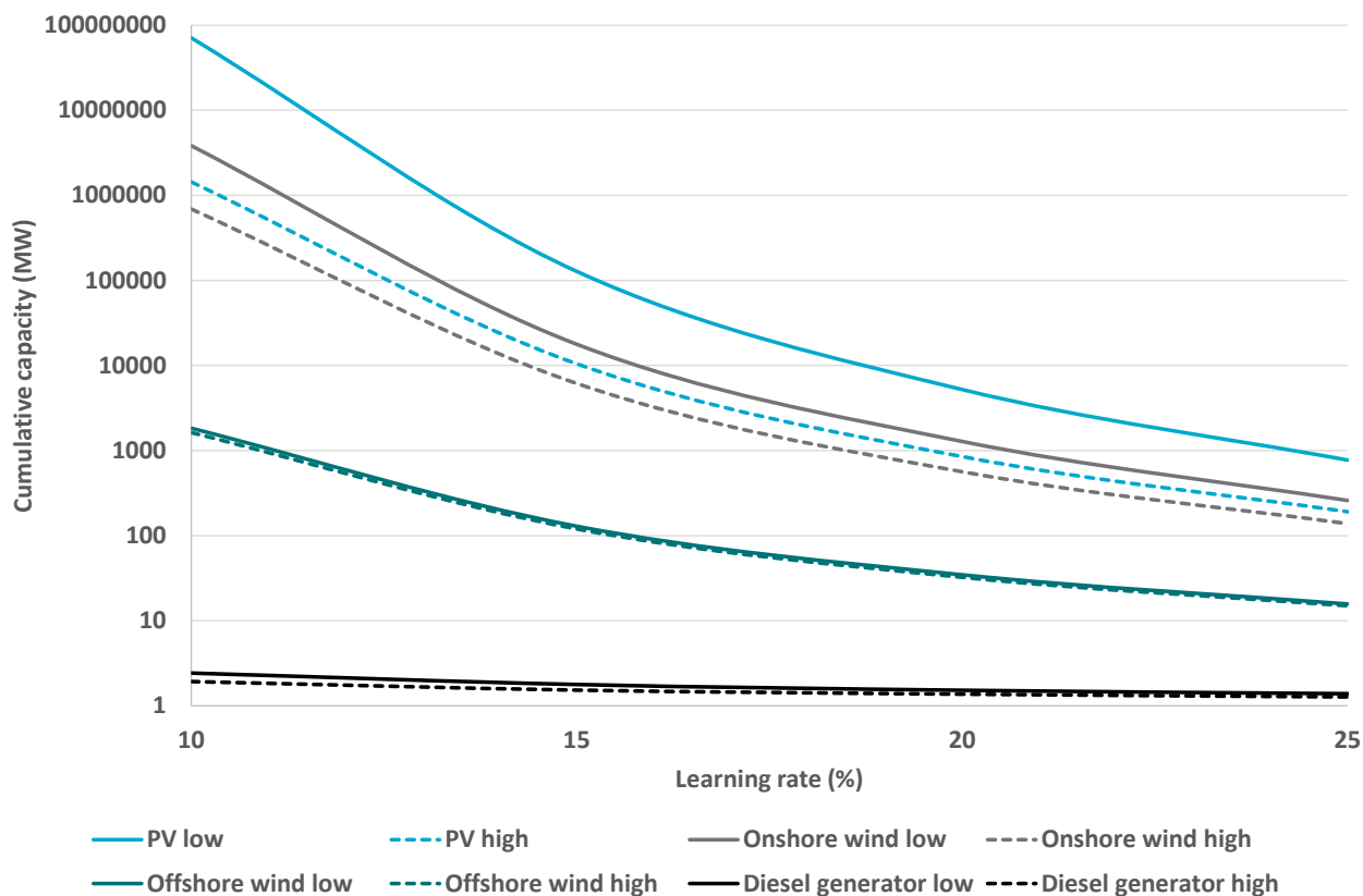
Figure 11 LR and cumulative capacity where the projected LCOE of WSE’s WEC is equivalent to that of other technologies in 2030
