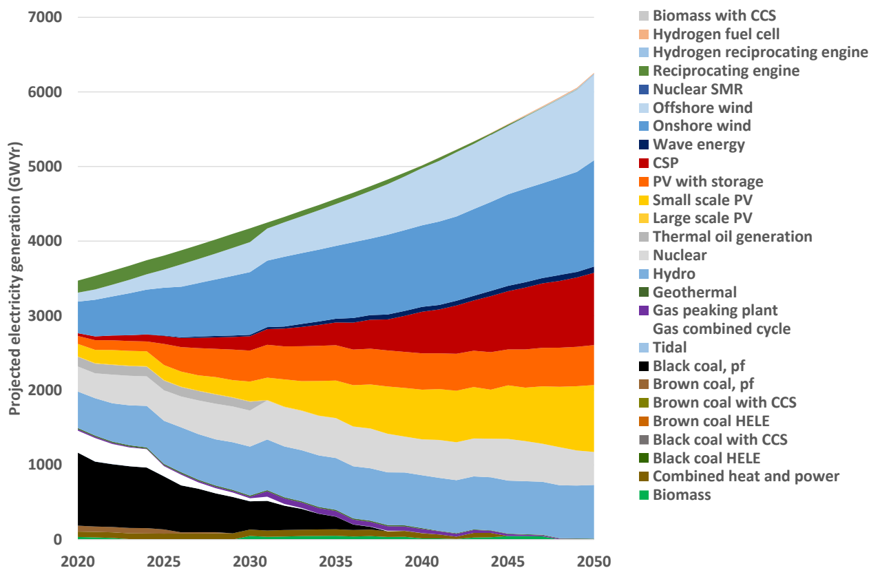
Figure 16 Projected global electricity generation under the Achievable scenario
