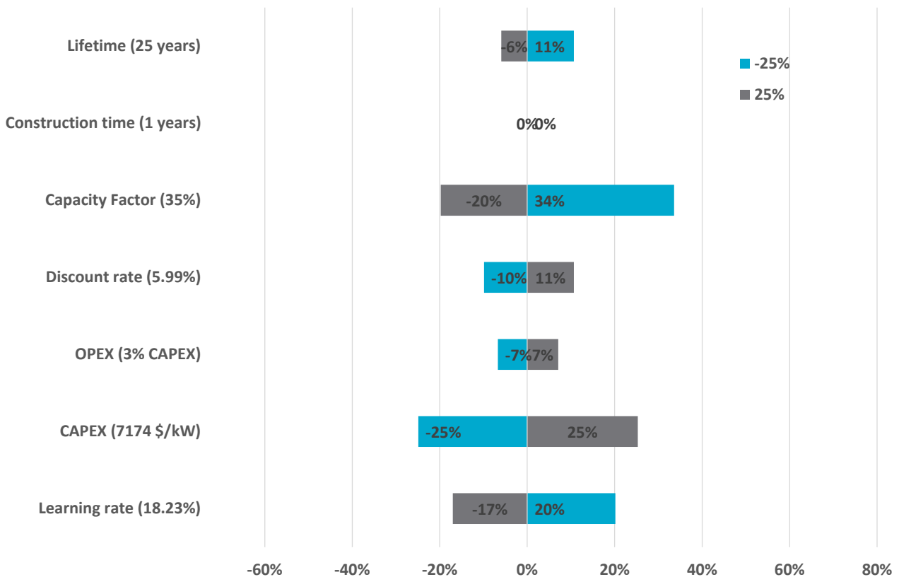
Figure 14 Projected sensitivity of the LCOE to changes in assumptions at 10 MW of cumulative capacity
