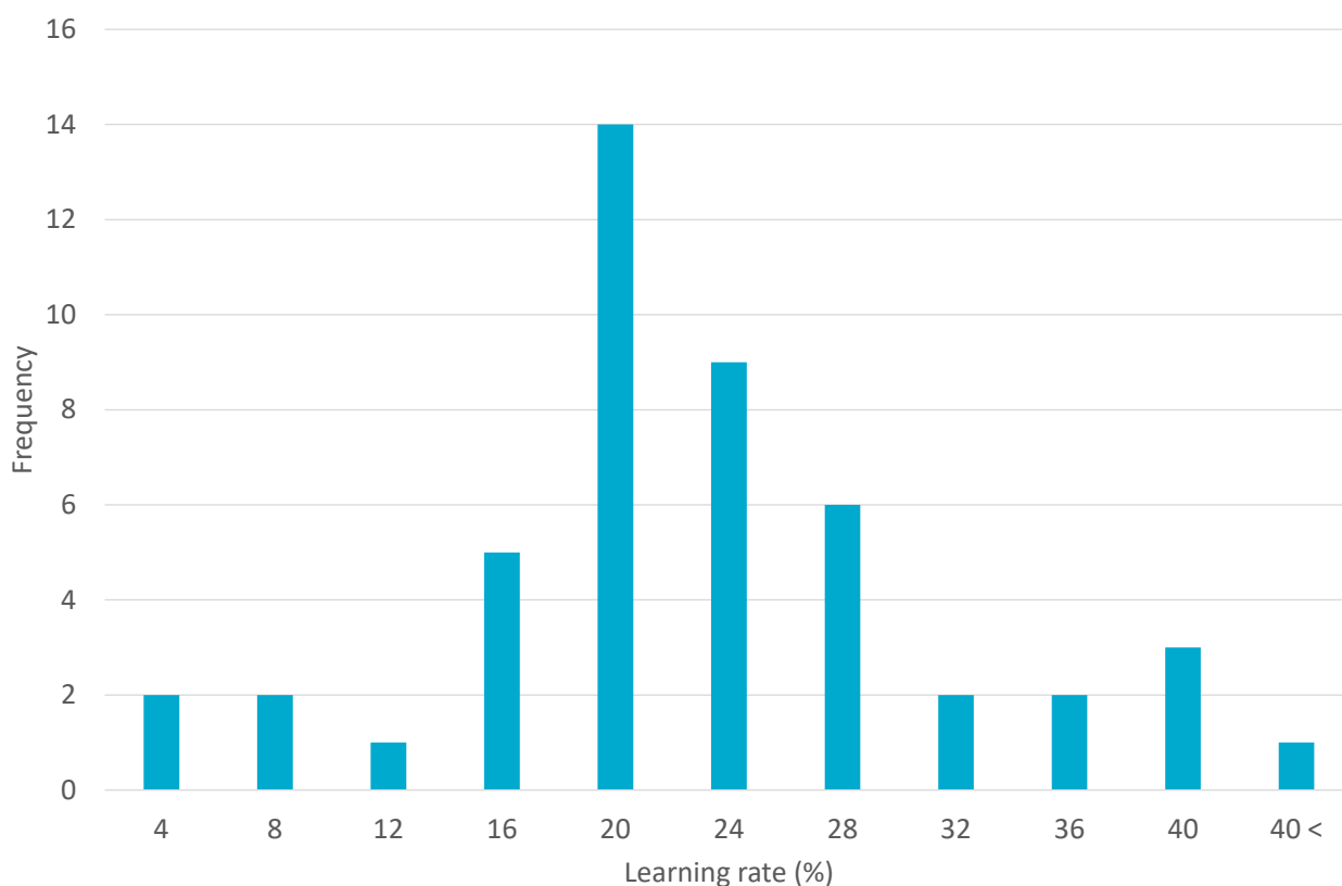
Figure 4 Histogram of 47 emerging technology LR's
