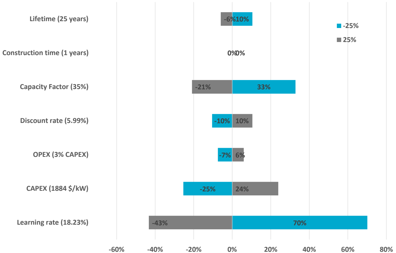
Figure 15 Projected sensitivity of the LCOE to changes in assumptions at 1000 MW of cumulative capacity
