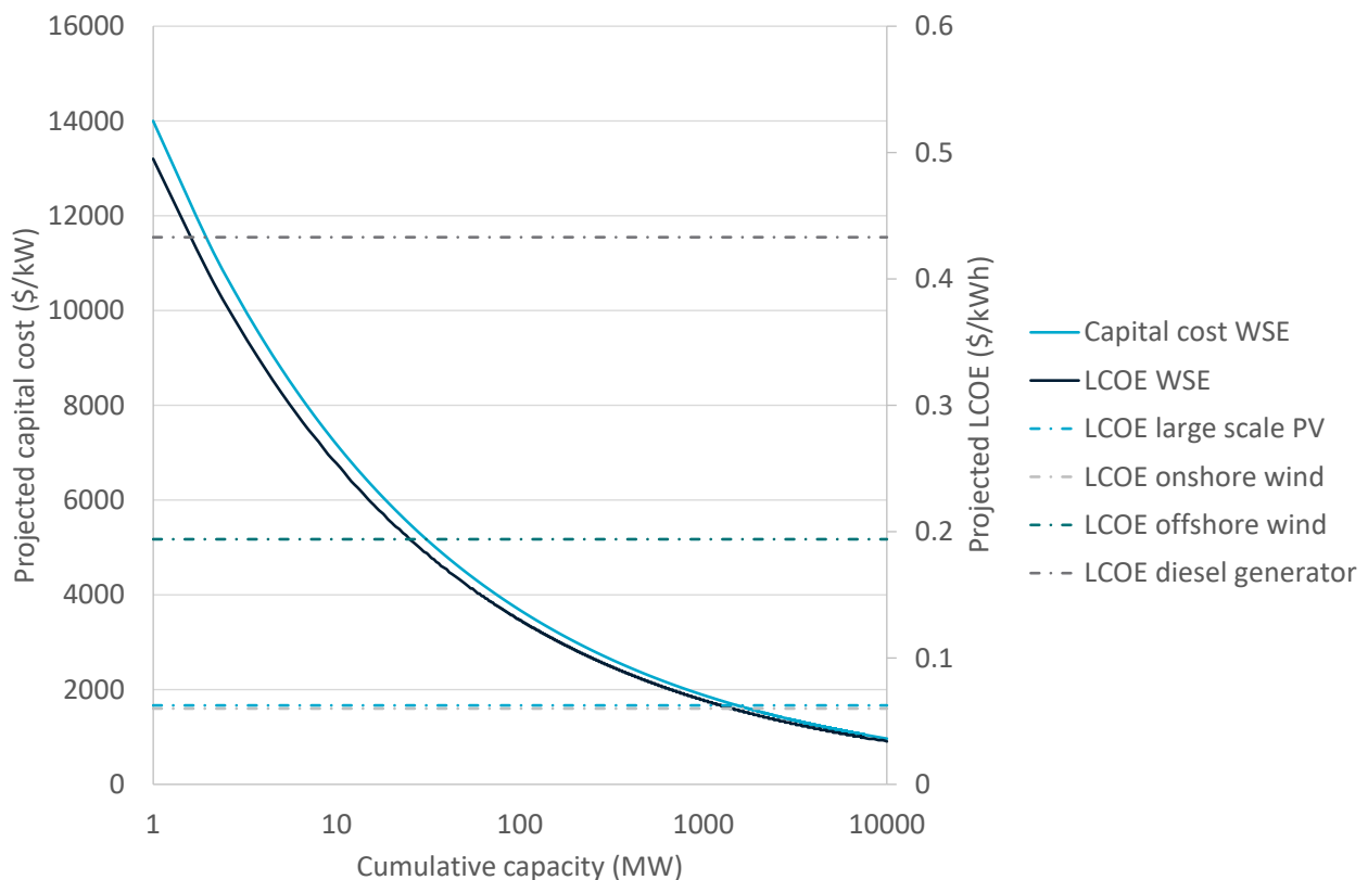
Figure 9 Projected capital cost and LCOE of WSE’s WEC with increasing cumulative capacity along with the current LCOEs of various technologies
