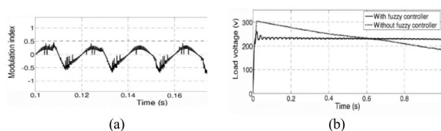
FIGURE 30. Control: (a) Modulation index control and (b) waveforms.
