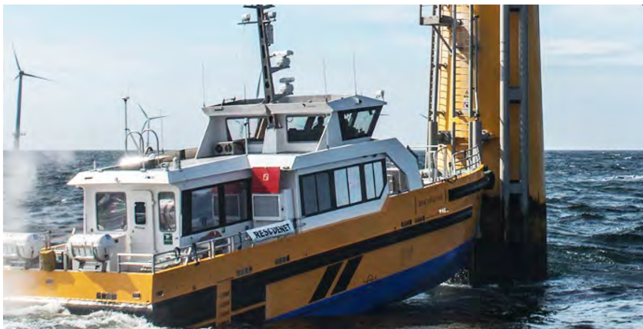
Figure 2.6 Windfarm service workboat and vertical access ladder. Note biofouling above the water line.
