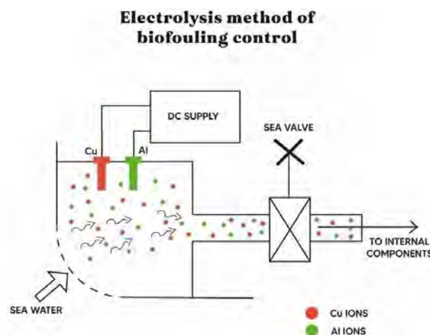
Figure 3.4 Sea chest arrangement for electrolytic biofouling control system.
