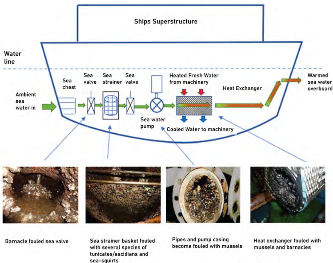
Figure A4 Common seawater cooling system components. Source: David Smith.
