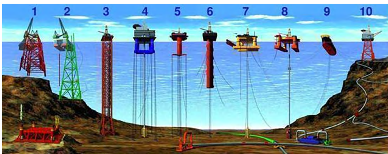
Figure 4.29 Types of offshore oil and gas structures include: 1), 2) conventional fixed platforms, shown here as a jacket foundation (deepest: Shell's Bullwinkle in 1991 at 412 m/1,353 ft GOM); 3) compliant tower (deepest: ChevronTexaco's Petronius in 1998 at 534 m/1,754 ft GOM); 4), 5) vertically moored tension leg and mini-tension leg platform (deepest: ConocoPhillips' Magnolia in 2004 1,425 m/4,674 ft GOM); 6) Spar (deepest: Dominion's Devil's Tower in 2004, 1,710 m/5,610 ft GOM); 7), 8) Semi-submersibles (deepest: Shell's NaKika in 2003, 1,920 m/6,300 ft GOM); 9) Floating production, storage and offloading facility (deepest: 2005, 1,345 m/4,429 ft Brazil); 10) Sub-sea completion and tie-back to host facility (deepest: Shell's Coulomb tie to NaKika 2004, 2,307 m/ 7,570 ft). All records from 2005 data.
