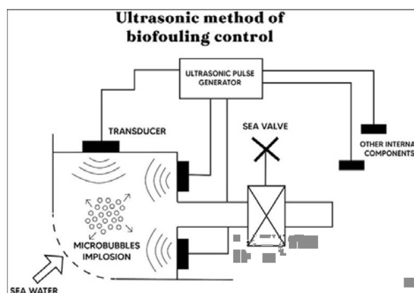
Figure 3.5 Ultrasonic biofouling control.
