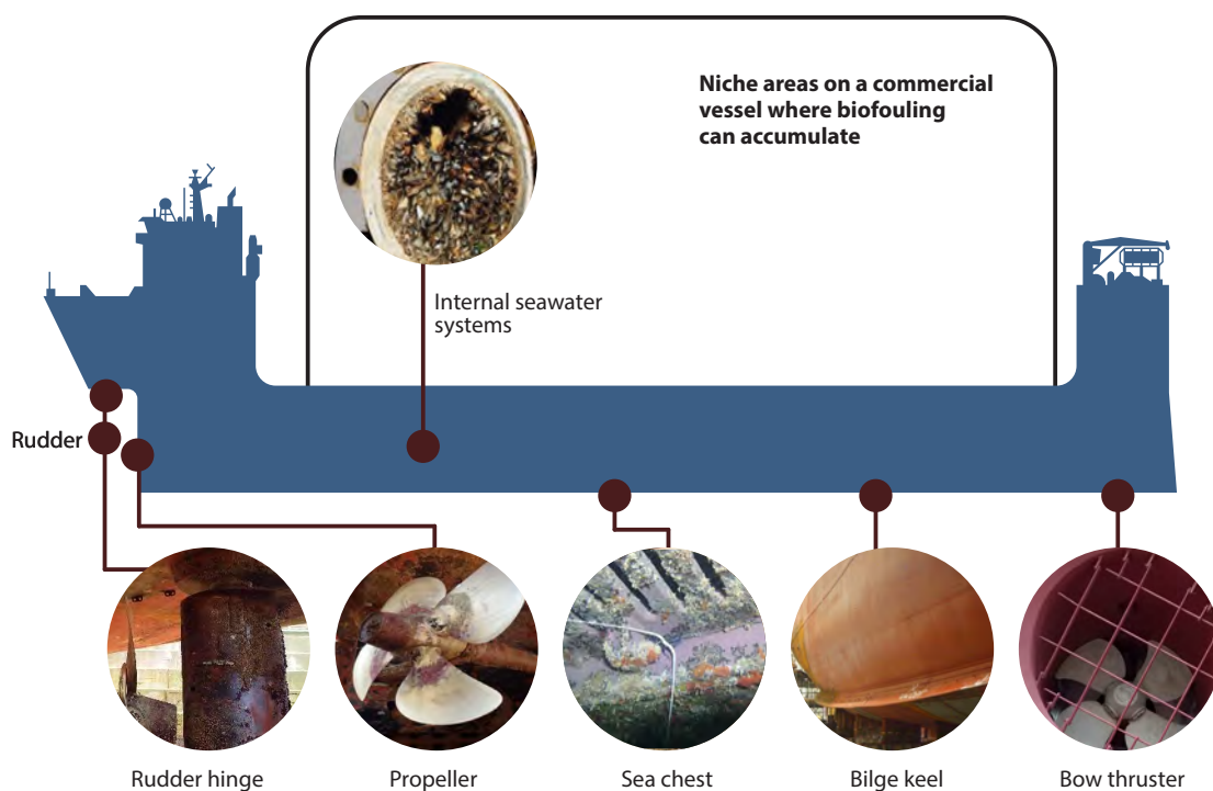
Figure 4.4 Niche areas on commercial vessels.
