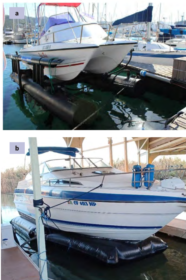
Figure 4.22 a) A motorized recreational boat suspended onto a floating system to prevent biofouling and b) the presence of biofouling on the structure
