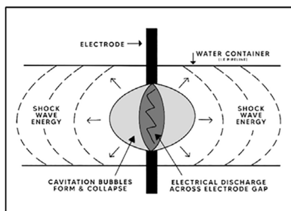
Figure 3.6 Acoustic sparker transducer in a water filled pipeline.
