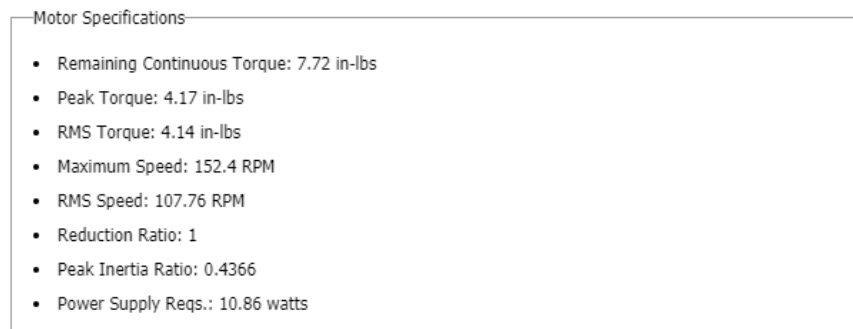
Figure 8: Motor Specifications for Tolomatic ERD Actuator
