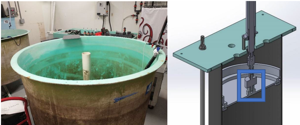
Figure 4: MCRL Wet Lab flow-through tank; Right: Device under test with load cell framed in blue
