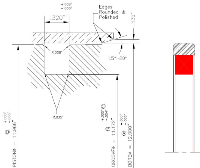
Figure 12: Dynamic Seal Drawing - AHPS C-12686S
