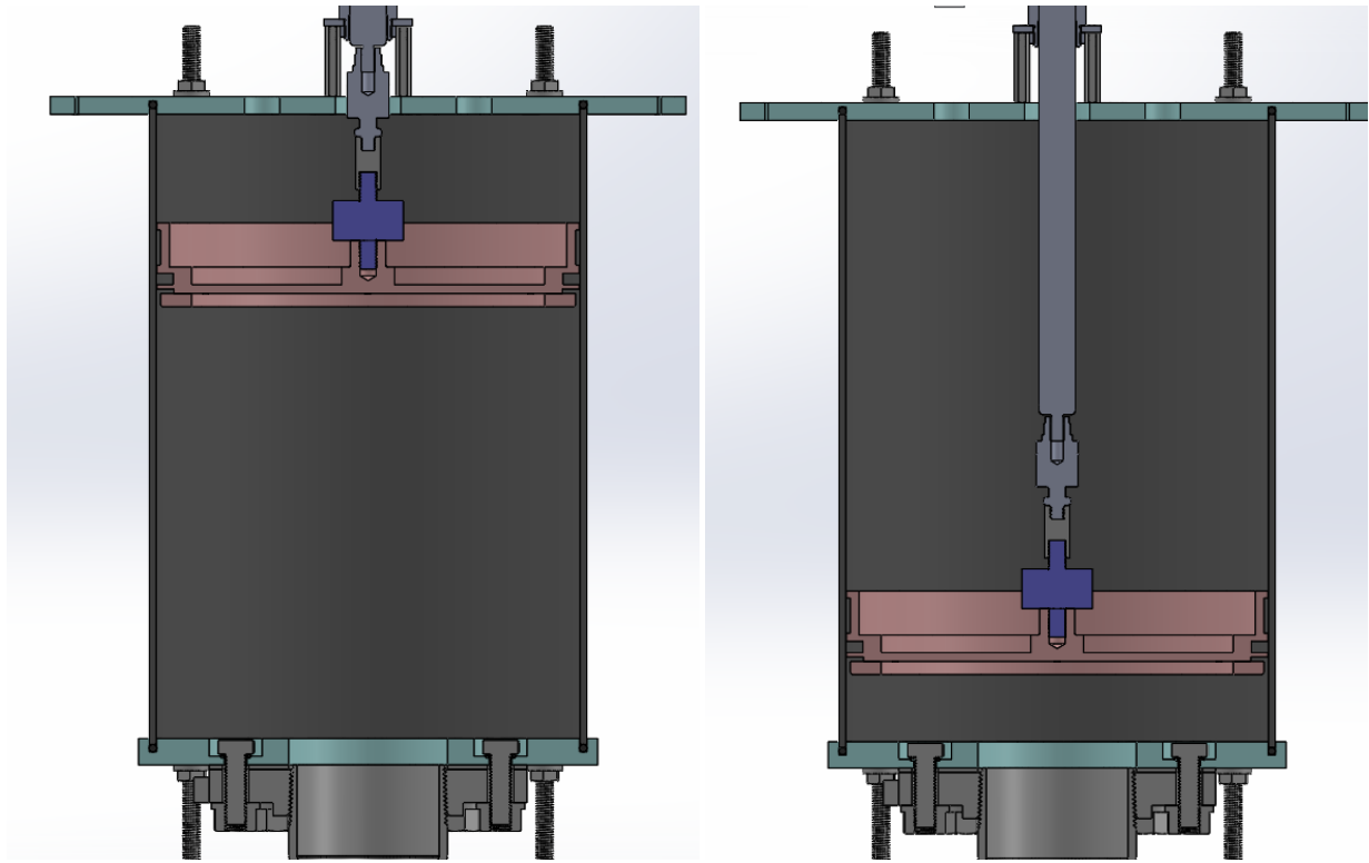
Figure 13: Stroke of actuator during test
