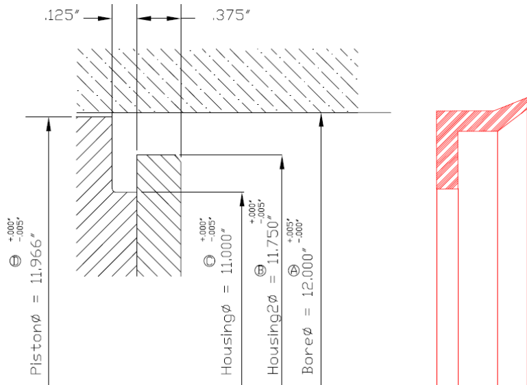
Figure 10: Wiper Seal Drawing - AHPS C-12686WP
