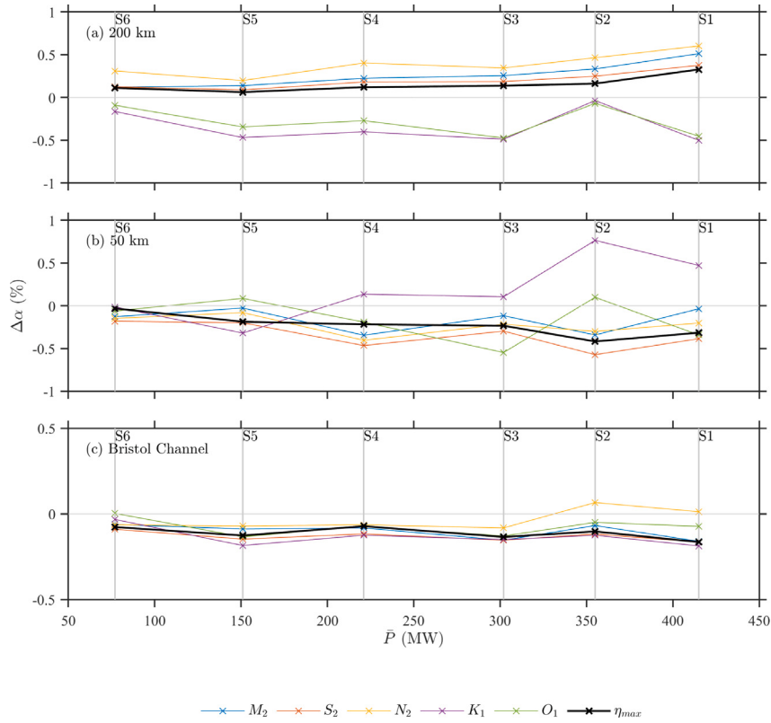
Fig. 7. The percentage change in amplitude \Delta\alpha of tidal constituents (and \overline{\eta_{max}} ) averaged over various areas: (a) \approx 200 km, and (b) \approx 50 km in radius from each lagoon, and (c) the Bristol Channel (BC) region (shown in Fig. 5a). In each calculation, changes inside the lagoon impoundment are omitted. To reduce the effects of local extremes, which especially occur over inter-tidal regions, the 1 \times 1 km grids were used for these calculations. Mean power output \bar{P} is calculated over the 30-day simulation period.
