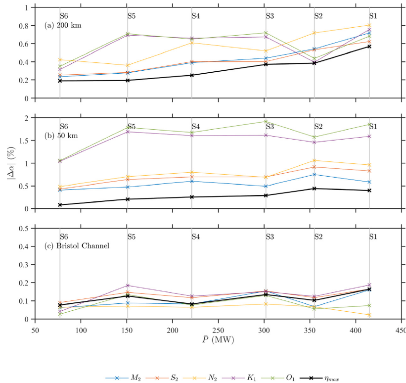
Fig. 8. Same as Fig. 7, but instead showing the absolute percentage change in amplitude |\Delta\alpha| .
